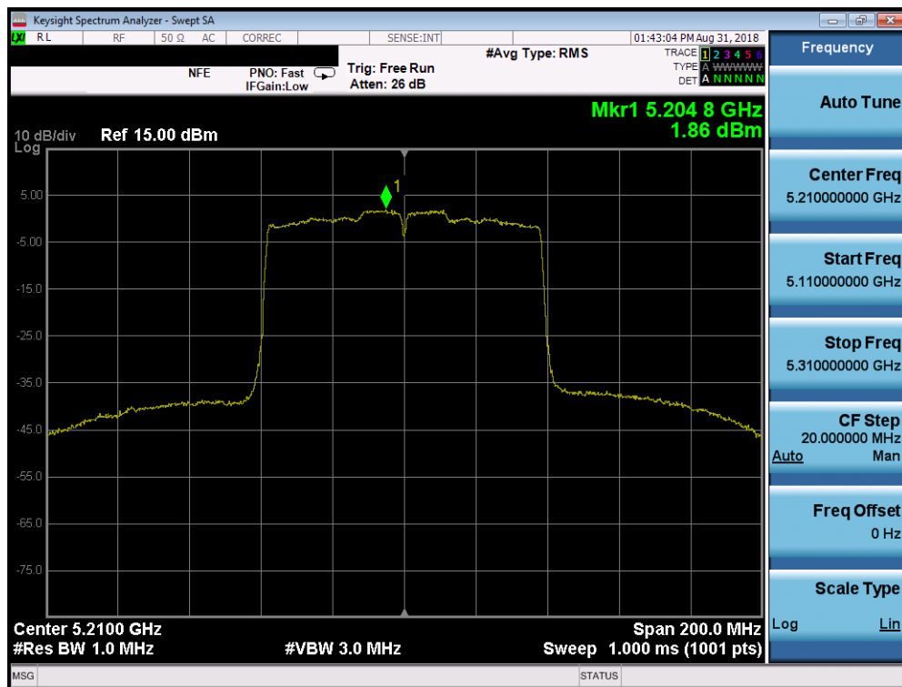
Plot 7-84. Power Spectral Density Plot SISO CORE1 (80MHz BW 802.11ac (UNII Band 1) – Ch. 42)
