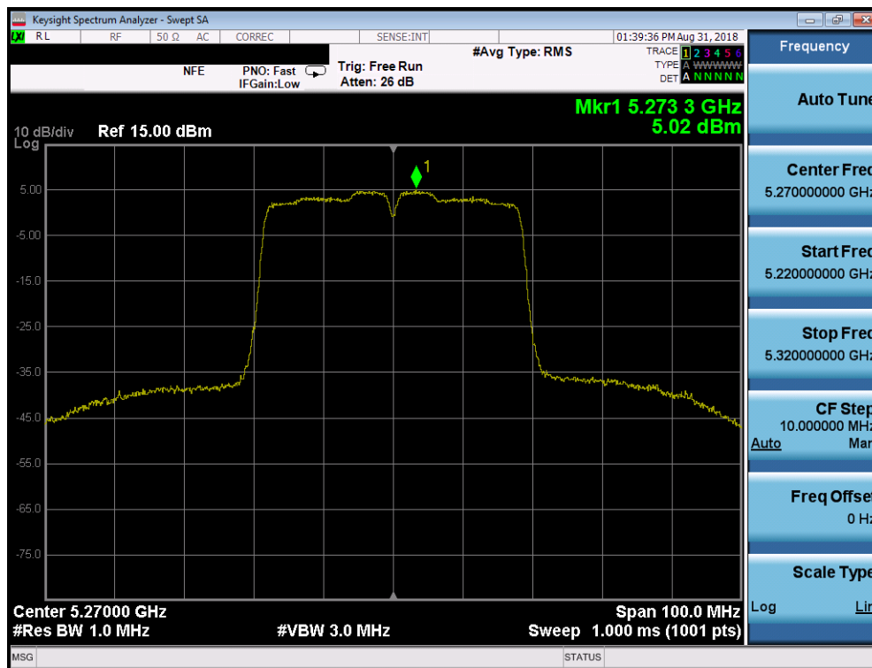
Plot 7-88. Power Spectral Density Plot SISO CORE1 (40MHz BW 802.11n (UNII Band 2A) – Ch. 54)
