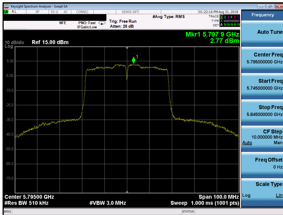
Plot 7-77. Power Spectral Density Plot SISO CORE0 (40MHz BW 802.11n (UNII Band 3) – Ch. 159)
