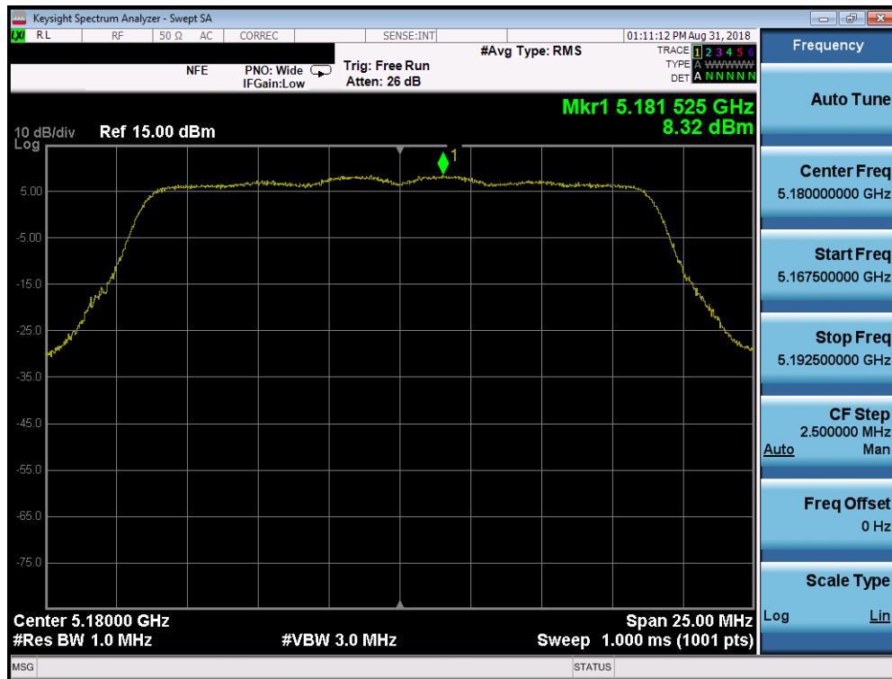
Plot 7-53. Power Spectral Density Plot SISO CORE0 (20MHz BW 802.11n (UNII Band 1) – Ch. 36)
