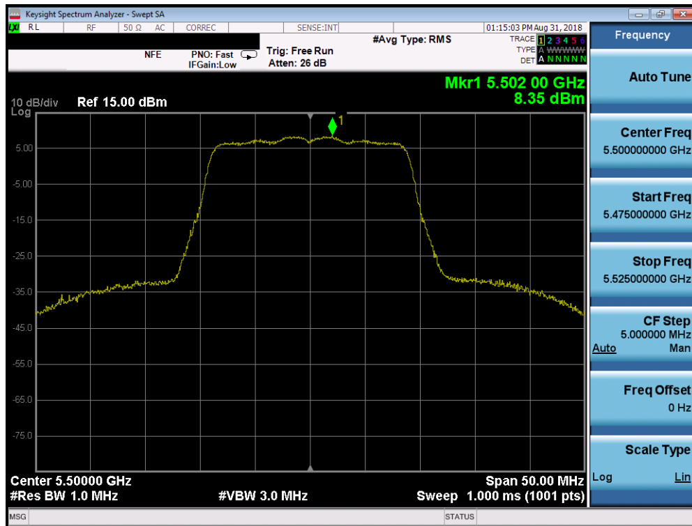
Plot 7-65. Power Spectral Density Plot SISO CORE0 (20MHz BW 802.11n (UNII Band 2C) – Ch. 100)
