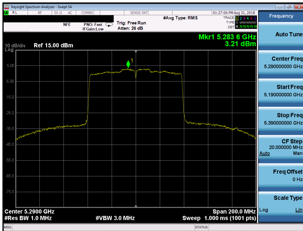
Plot 7-64. Power Spectral Density Plot SISO CORE0 (80MHz BW 802.11ac (UNII Band 2A) – Ch. 58)
