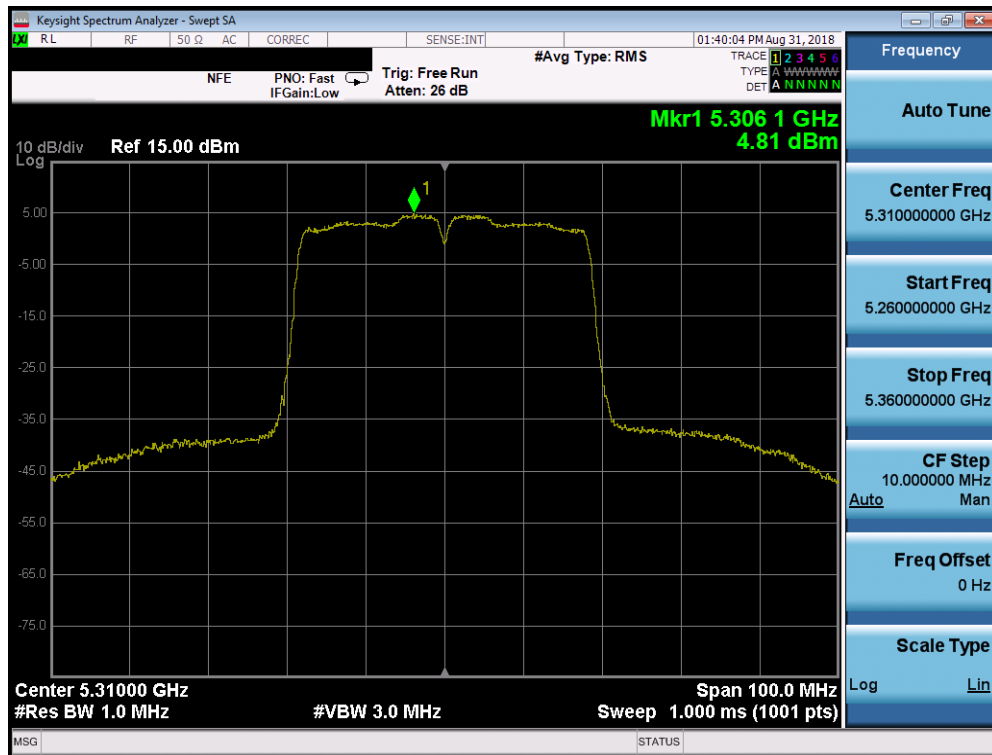
Plot 7-89. Power Spectral Density Plot SISO CORE1 (40MHz BW 802.11n (UNII Band 2A) – Ch. 62)
