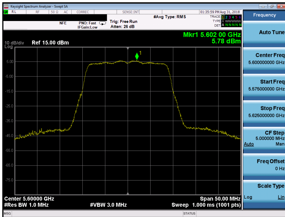
Plot 7-92. Power Spectral Density Plot SISO CORE1 (20MHz BW 802.11n (UNII Band 2C) – Ch. 120)
