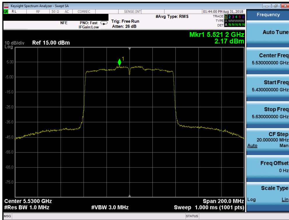
Plot 7-97. Power Spectral Density Plot SISO CORE1 (80MHz BW 802.11ac (UNII Band 2C) – Ch. 106)
