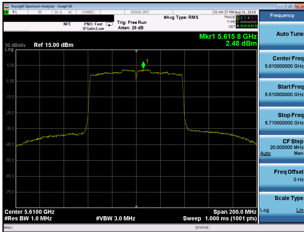
Plot 7-98. Power Spectral Density Plot SISO CORE1 (80MHz BW 802.11ac (UNII Band 2C) – Ch. 122)
