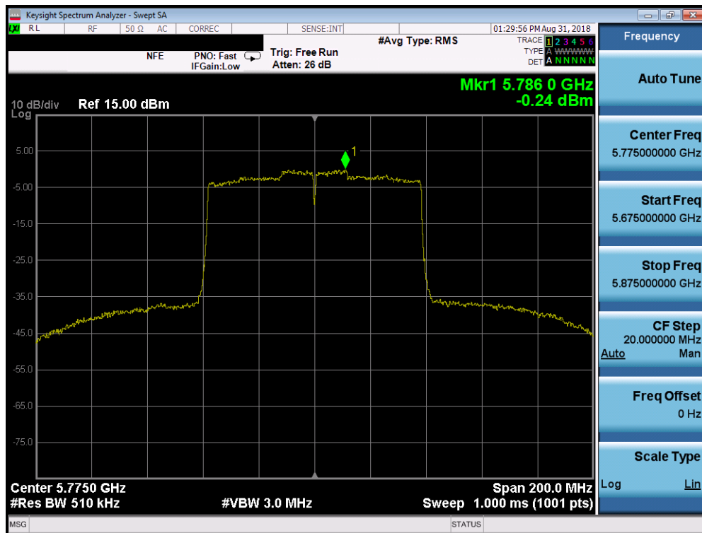
Plot 7-78. Power Spectral Density Plot SISO CORE0 (80MHz BW 802.11ac (UNII Band 3) – Ch. 155)
