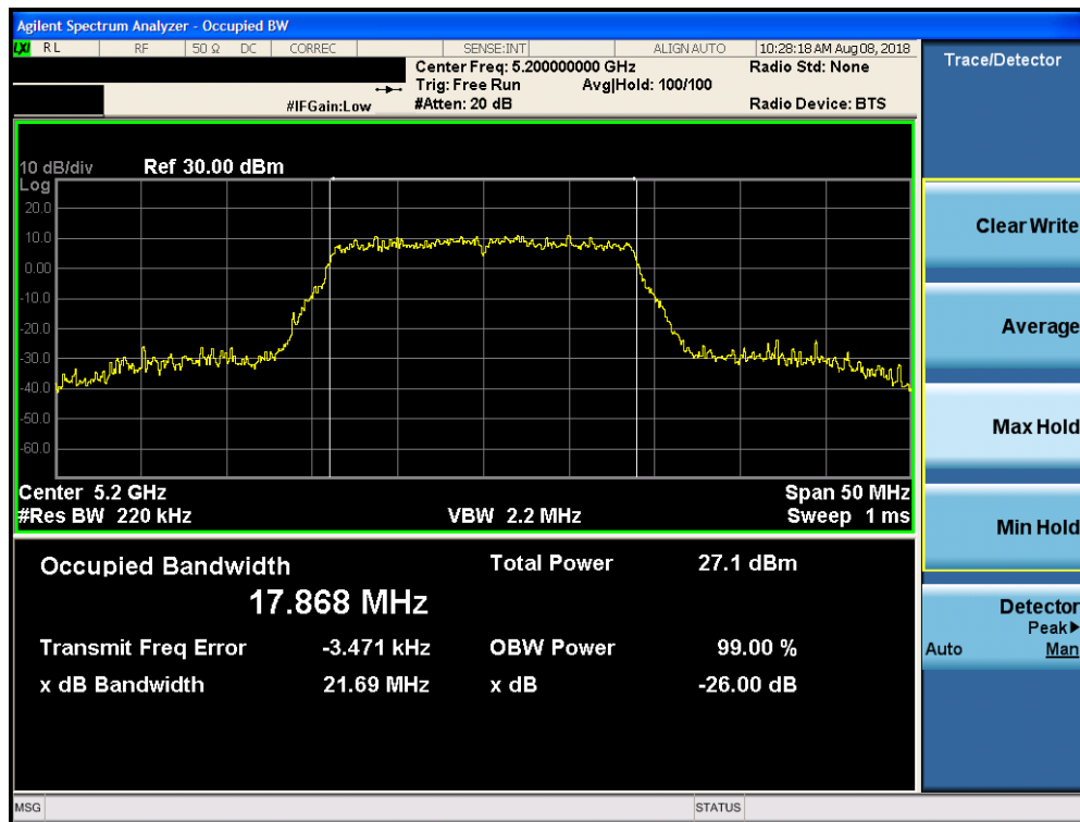
Plot 7-2. 26dB Bandwidth Plot SISO CORE0 (20MHz BW 802.11n (UNII Band 1) – Ch. 40)
