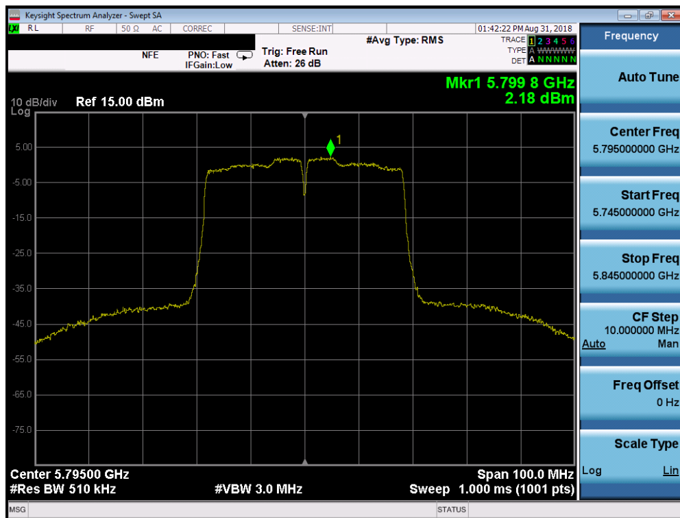
Plot 7-103. Power Spectral Density Plot SISO CORE1 (40MHz BW 802.11n (UNII Band 3) – Ch. 159)
