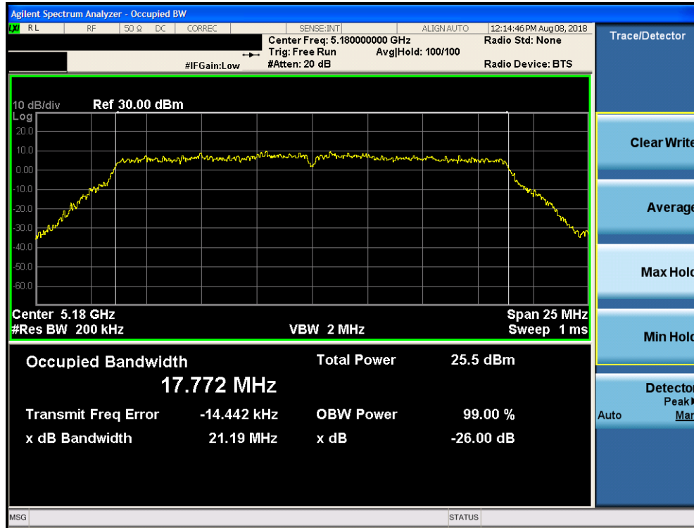
Plot 7-21. 26dB Bandwidth Plot SISO CORE1 (20MHz BW 802.11n (UNII Band 1) – Ch. 36)
