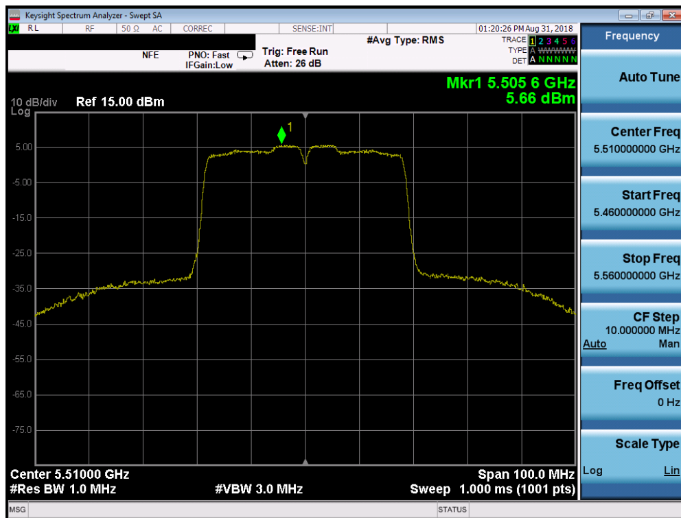
Plot 7-68. Power Spectral Density Plot SISO CORE0 (40MHz BW 802.11n (UNII Band 2C) – Ch. 102)
