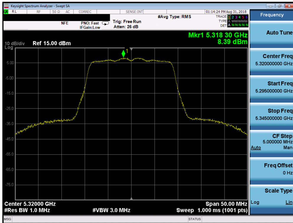
Plot 7-61. Power Spectral Density Plot SISO CORE0 (20MHz BW 802.11n (UNII Band 2A) – Ch. 64)
