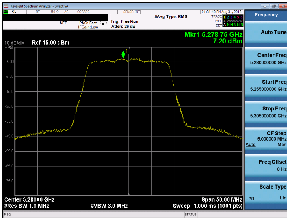
Plot 7-86. Power Spectral Density Plot SISO CORE1 (20MHz BW 802.11n (UNII Band 2A) – Ch. 56)
