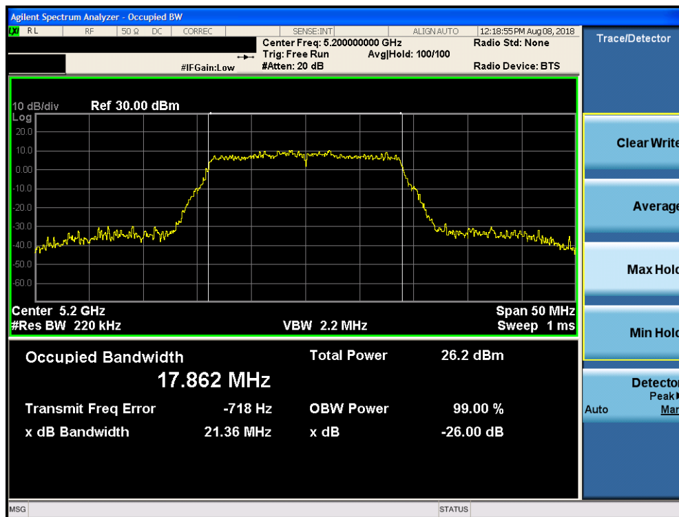
Plot 7-22. 26dB Bandwidth Plot SISO CORE1 (20MHz BW 802.11n (UNII Band 1) – Ch. 40)
