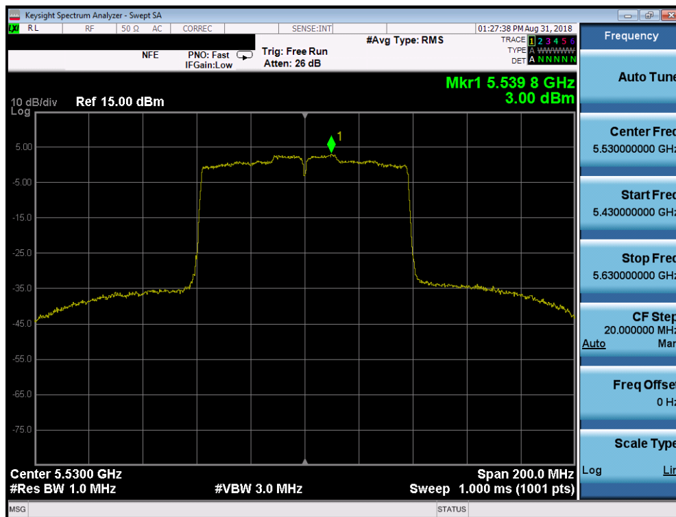
Plot 7-71. Power Spectral Density Plot SISO CORE0 (80MHz BW 802.11ac (UNII Band 2C) – Ch. 106)
