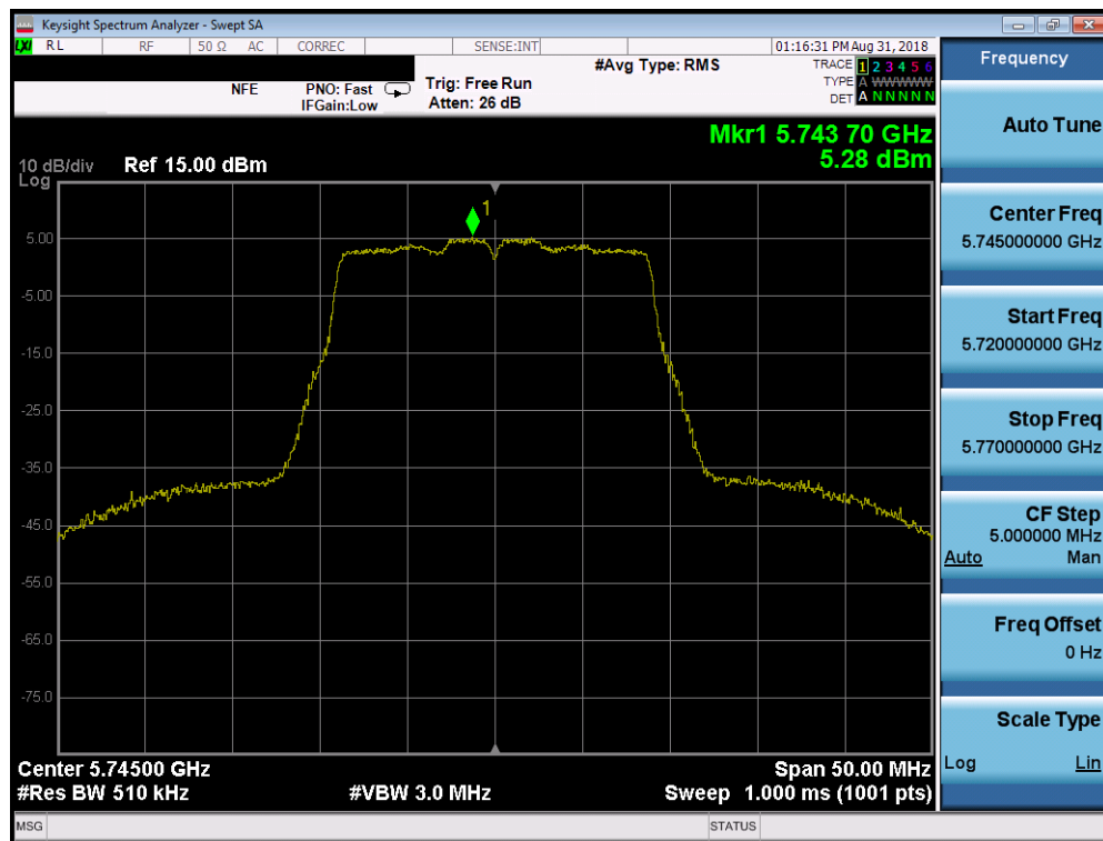
Plot 7-73. Power Spectral Density Plot SISO CORE0 (20MHz BW 802.11n (UNII Band 3) – Ch. 149)
