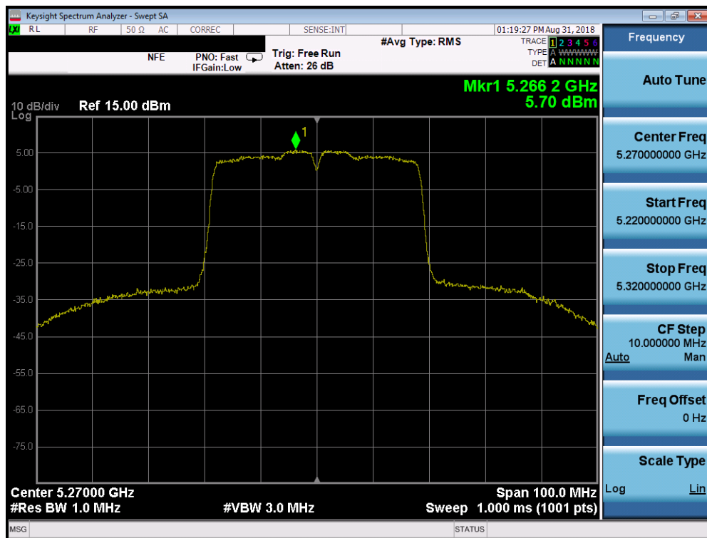
Plot 7-62. Power Spectral Density Plot SISO CORE0 (40MHz BW 802.11n (UNII Band 2A) – Ch. 54)
