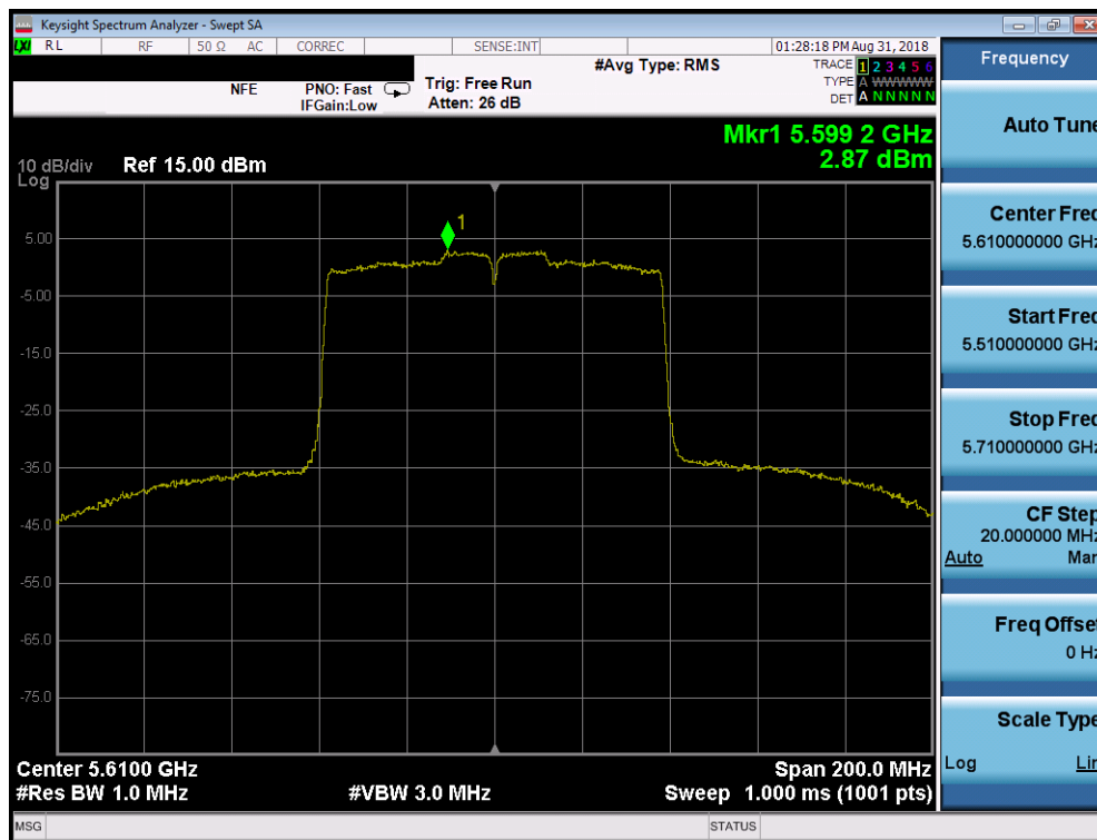
Plot 7-72. Power Spectral Density Plot SISO CORE0 (80MHz BW 802.11ac (UNII Band 2C) – Ch. 122)
