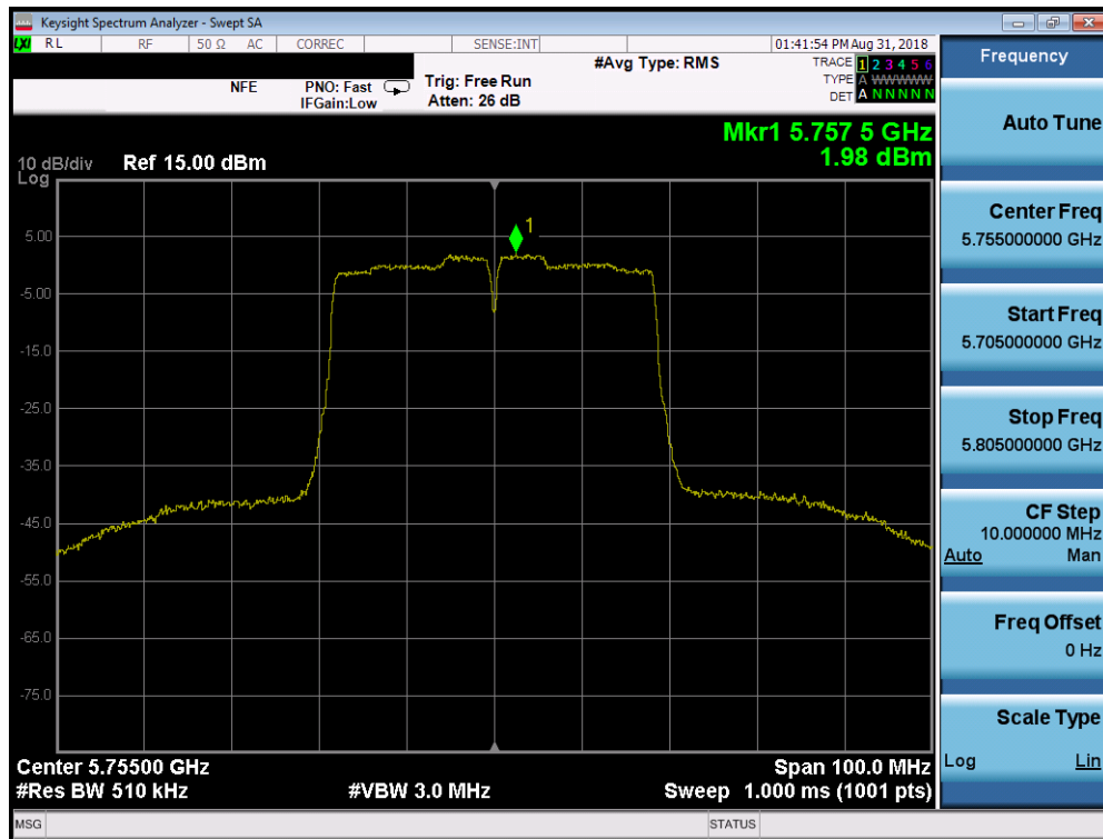
Plot 7-102. Power Spectral Density Plot SISO CORE1 (40MHz BW 802.11n (UNII Band 3) – Ch. 151)
