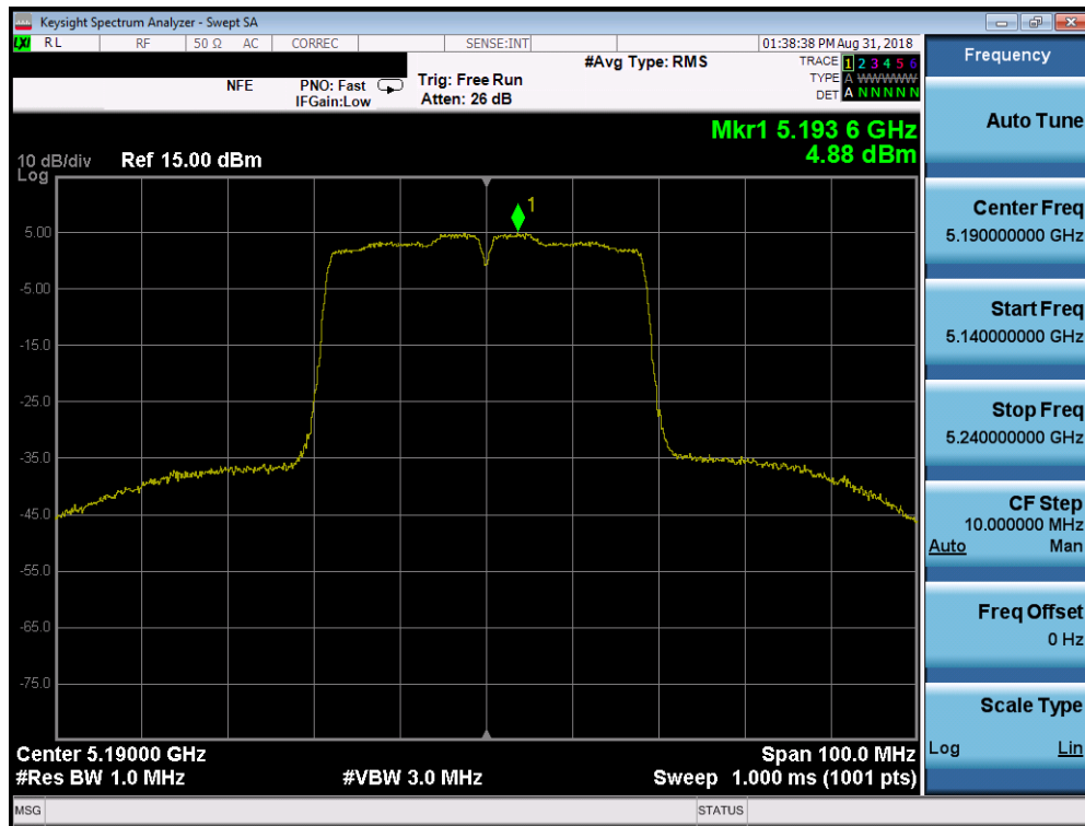
Plot 7-82. Power Spectral Density Plot SISO CORE1 (40MHz BW 802.11n (UNII Band 1) – Ch. 38)
