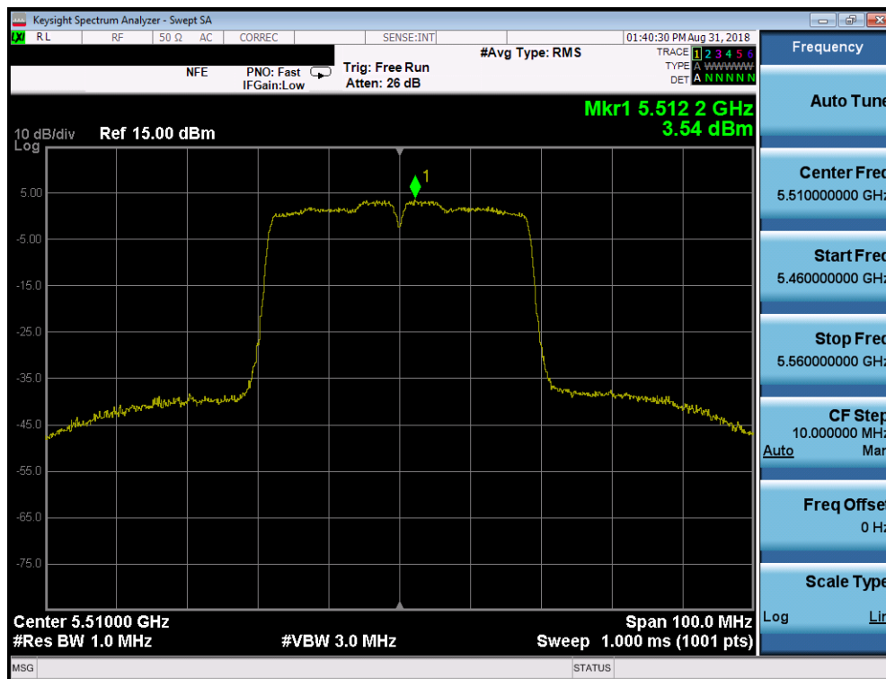
Plot 7-94. Power Spectral Density Plot SISO CORE1 (40MHz BW 802.11n (UNII Band 2C) – Ch. 102)
