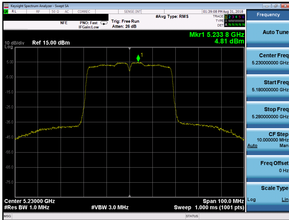
Plot 7-83. Power Spectral Density Plot SISO CORE1 (40MHz BW 802.11n (UNII Band 1) – Ch. 46)
