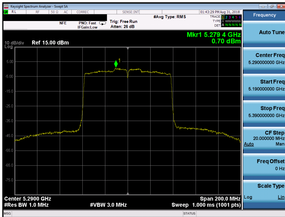
Plot 7-90. Power Spectral Density Plot SISO CORE1 (80MHz BW 802.11ac (UNII Band 2A) – Ch. 58)
