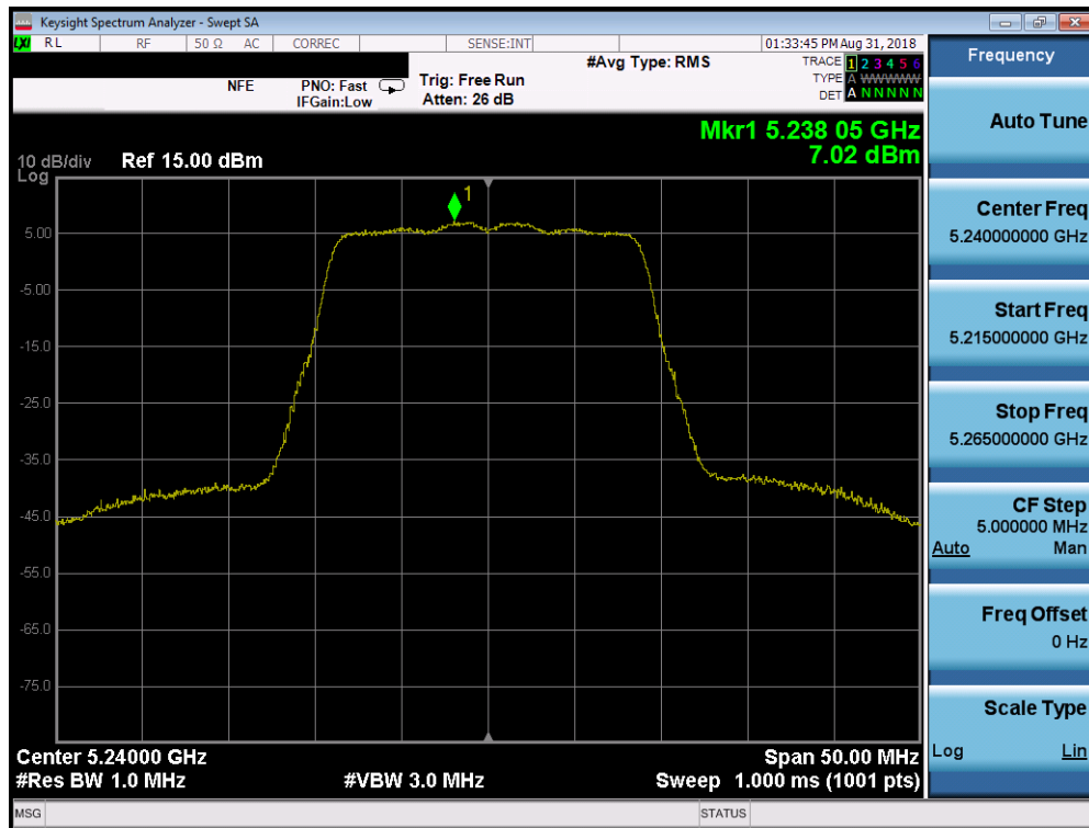
Plot 7-81. Power Spectral Density Plot SISO CORE1 (20MHz BW 802.11n (UNII Band 1) – Ch. 48)
