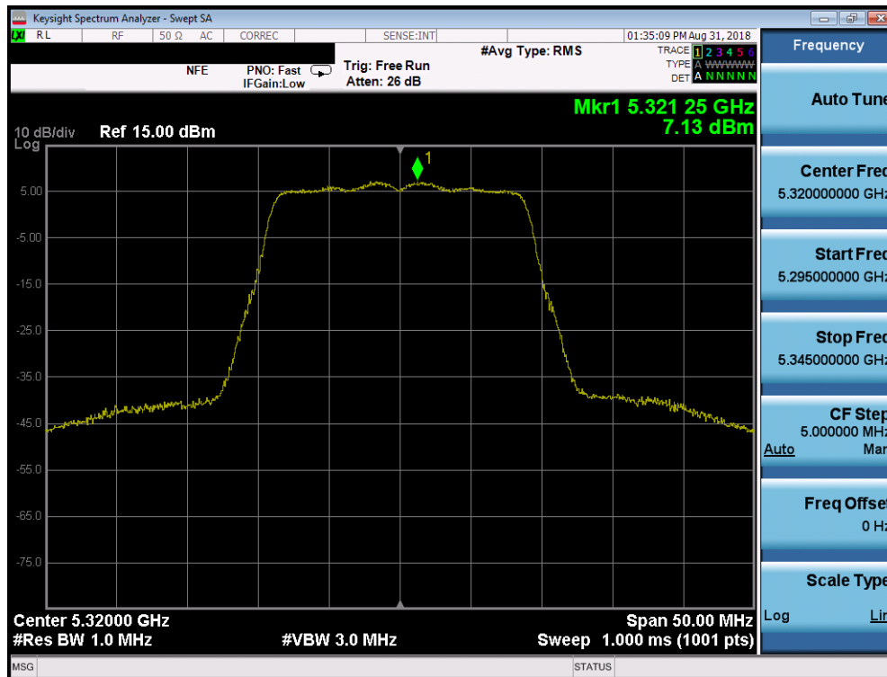
Plot 7-87. Power Spectral Density Plot SISO CORE1 (20MHz BW 802.11n (UNII Band 2A) – Ch. 64)
