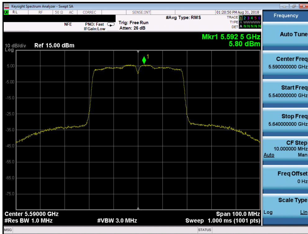
Plot 7-69. Power Spectral Density Plot SISO CORE0 (40MHz BW 802.11n (UNII Band 2C) – Ch. 118)
