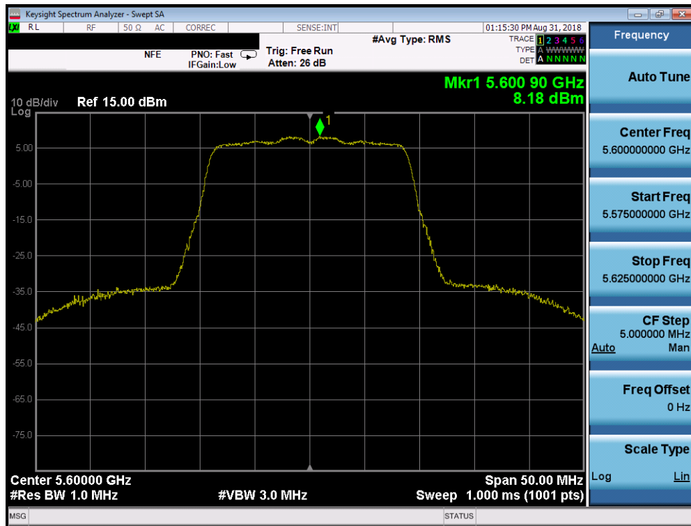
Plot 7-66. Power Spectral Density Plot SISO CORE0 (20MHz BW 802.11n (UNII Band 2C) – Ch. 120)
