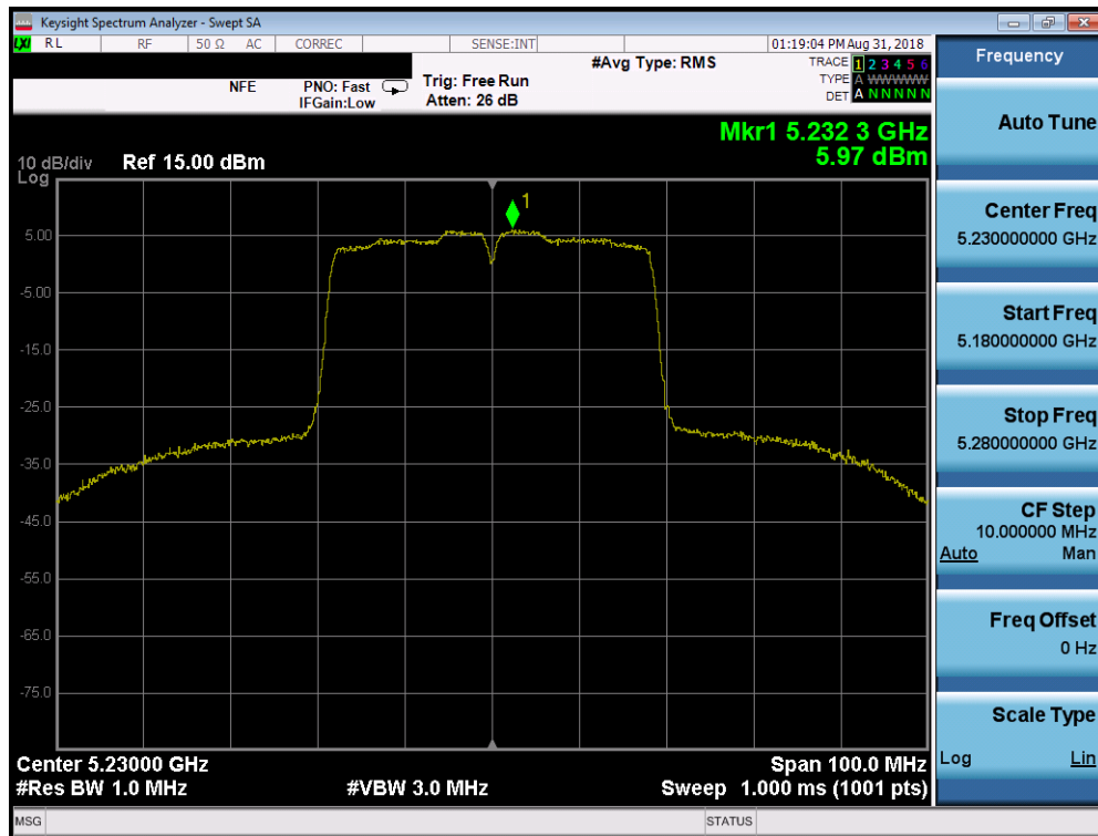
Plot 7-57. Power Spectral Density Plot SISO CORE0 (40MHz BW 802.11n (UNII Band 1) – Ch. 46)
