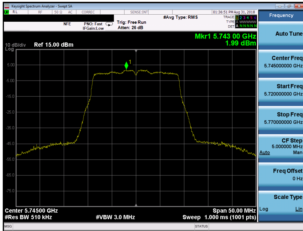
Plot 7-99. Power Spectral Density Plot SISO CORE1 (20MHz BW 802.11n (UNII Band 3) – Ch. 149)
