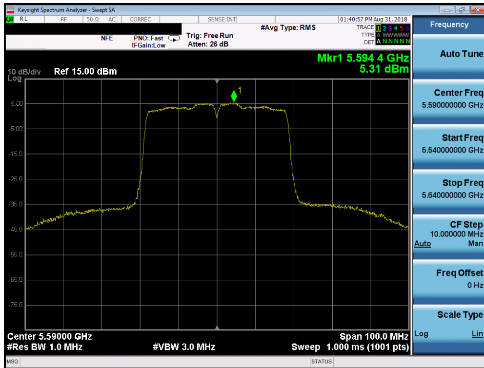
Plot 7-95. Power Spectral Density Plot SISO CORE1 (40MHz BW 802.11n (UNII Band 2C) – Ch. 118)
