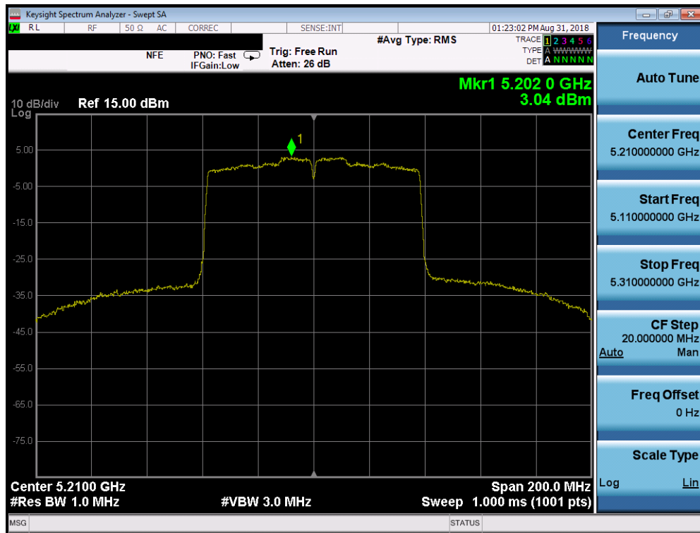
Plot 7-58. Power Spectral Density Plot SISO CORE0 (80MHz BW 802.11ac (UNII Band 1) – Ch. 42)
