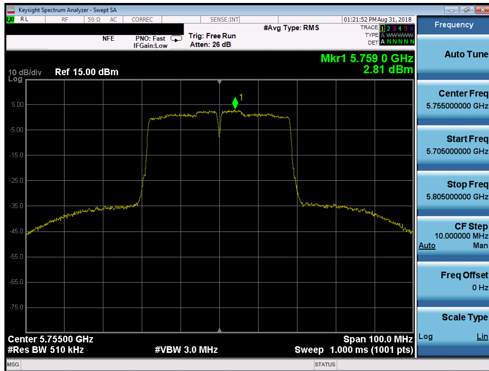
Plot 7-76. Power Spectral Density Plot SISO CORE0 (40MHz BW 802.11n (UNII Band 3) – Ch. 151)
