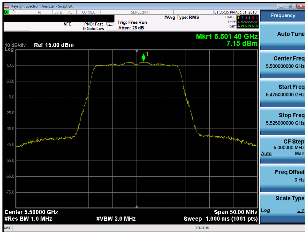
Plot 7-91. Power Spectral Density Plot SISO CORE1 (20MHz BW 802.11n (UNII Band 2C) – Ch. 100)
