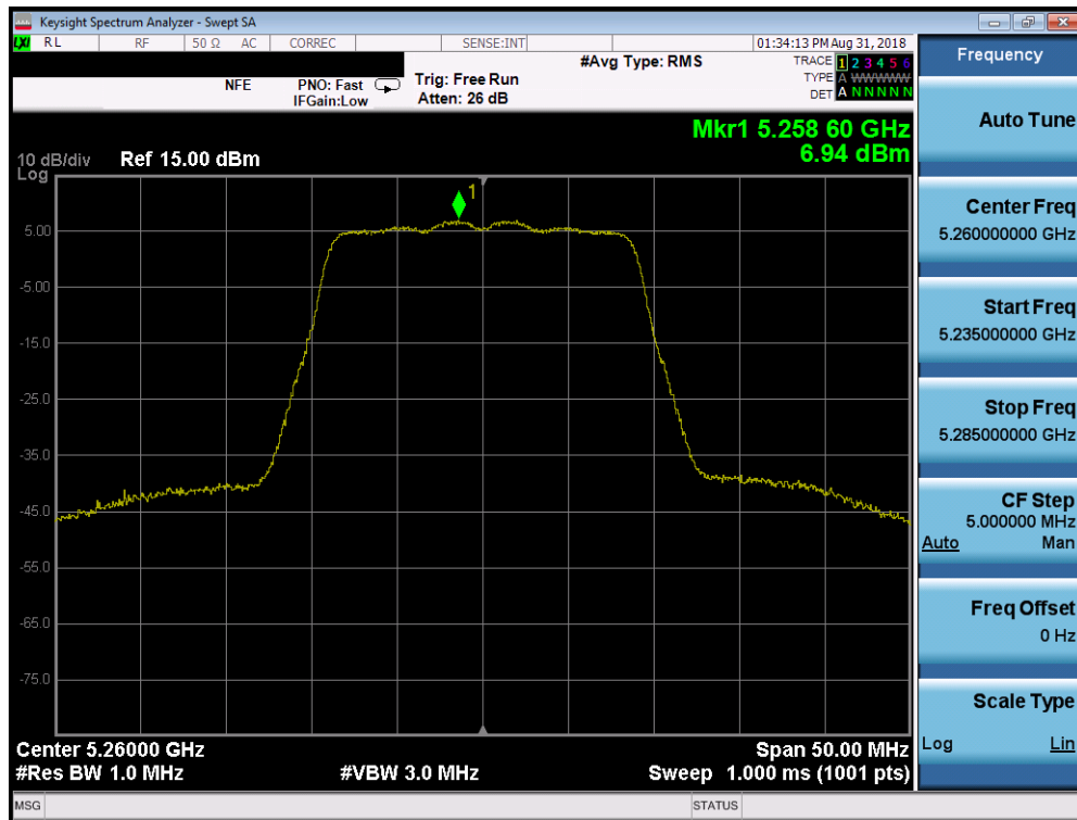
Plot 7-85. Power Spectral Density Plot SISO CORE1 (20MHz BW 802.11n (UNII Band 2A) – Ch. 52)
