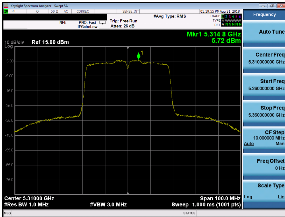
Plot 7-63. Power Spectral Density Plot SISO CORE0 (40MHz BW 802.11n (UNII Band 2A) – Ch. 62)
