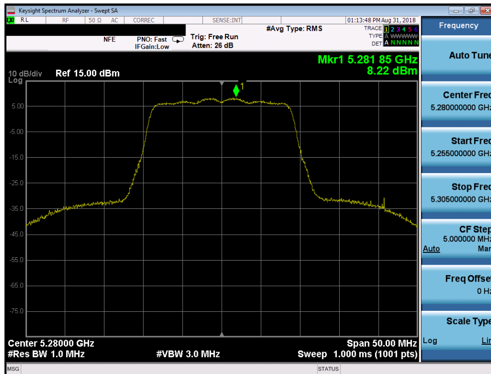
Plot 7-60. Power Spectral Density Plot SISO CORE0 (20MHz BW 802.11n (UNII Band 2A) – Ch. 56)
