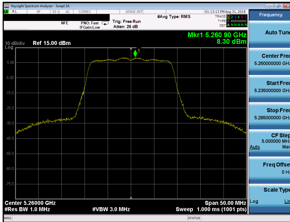
Plot 7-59. Power Spectral Density Plot SISO CORE0 (20MHz BW 802.11n (UNII Band 2A) – Ch. 52)
