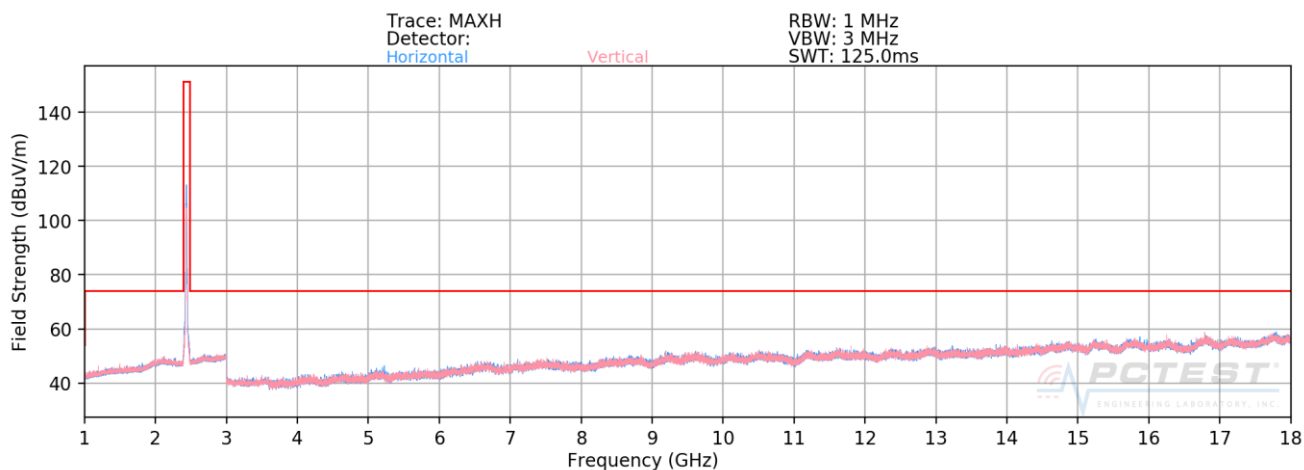
Plot 7-116. Radiated Spurious Plot above 1GHz SISO CORE0 (802.11b – Ch. 6)
