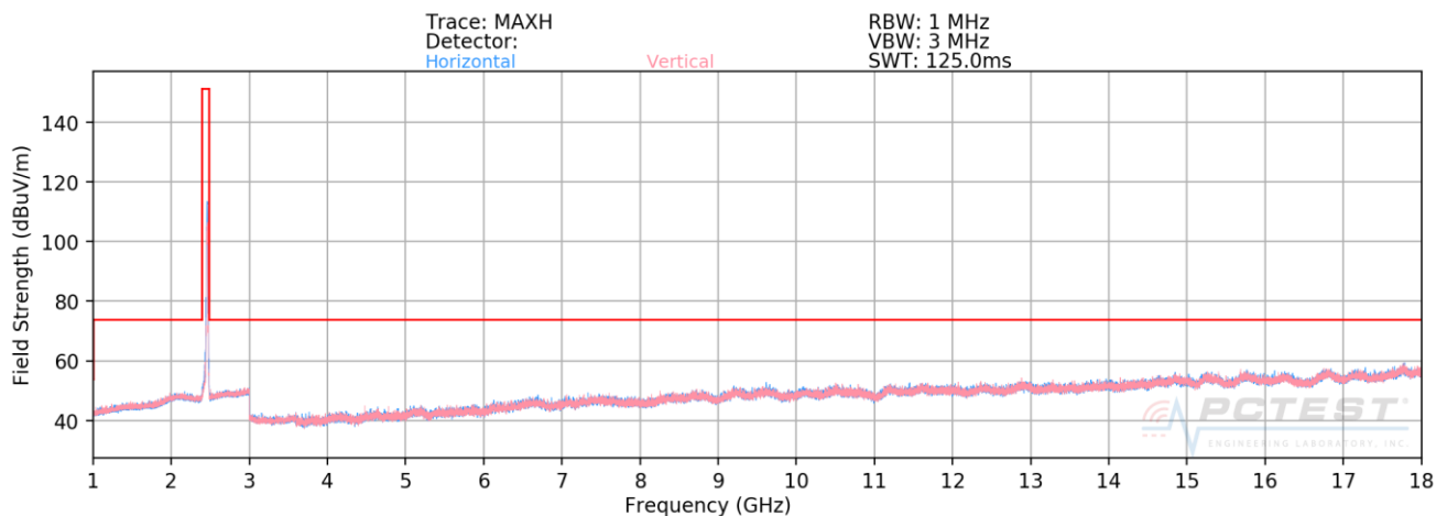
Plot 7-117. Radiated Spurious Plot above 1GHz SISO CORE0 (802.11b – Ch. 11)
