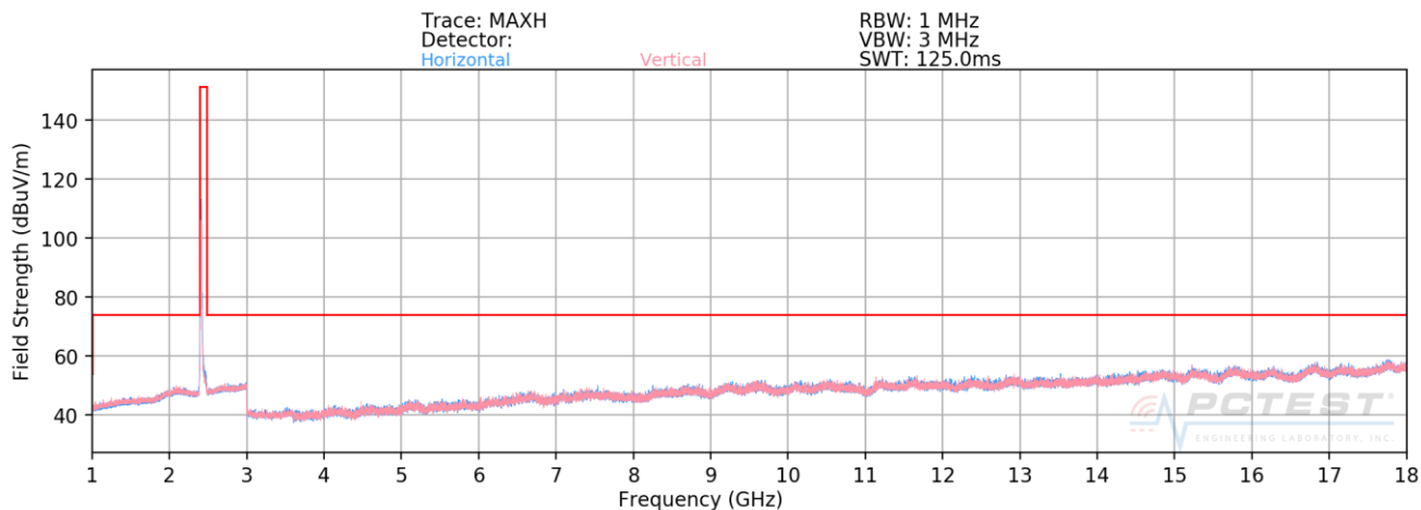
Plot 7-115. Radiated Spurious Plot above 1GHz SISO CORE0 (802.11b – Ch. 1)
