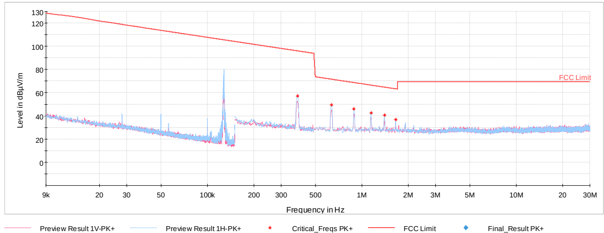
Plot 7-3. Radiated Spurious Plot from 9kHz – 30MHz (Loop Antenna X & Y)
