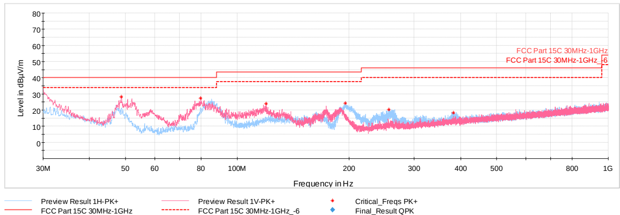
Plot 7-4. Radiated Spurious Plot above 30MHz (Pol. H & V)
