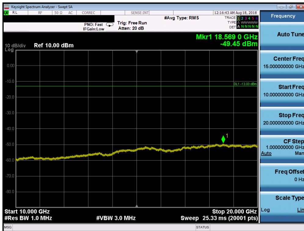
Plot 7-43. Conducted Spurious Plot (AWS WCDMA Mode - High Channel)
