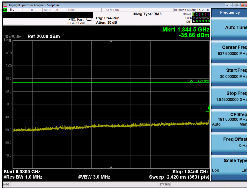
Plot 7-17. Conducted Spurious Plot (PCS GPRS Mode - Low Channel)
