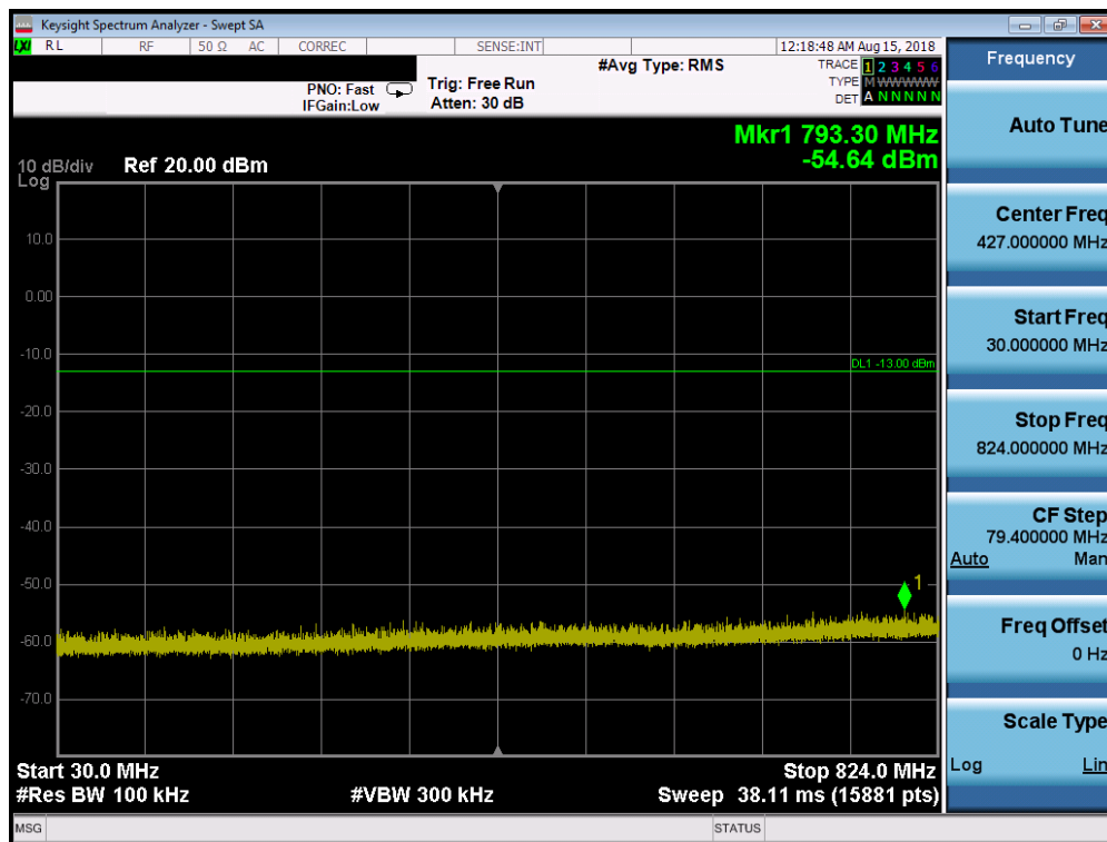
Plot 7-14. Conducted Spurious Plot (Cellular GPRS Mode - High Channel)
