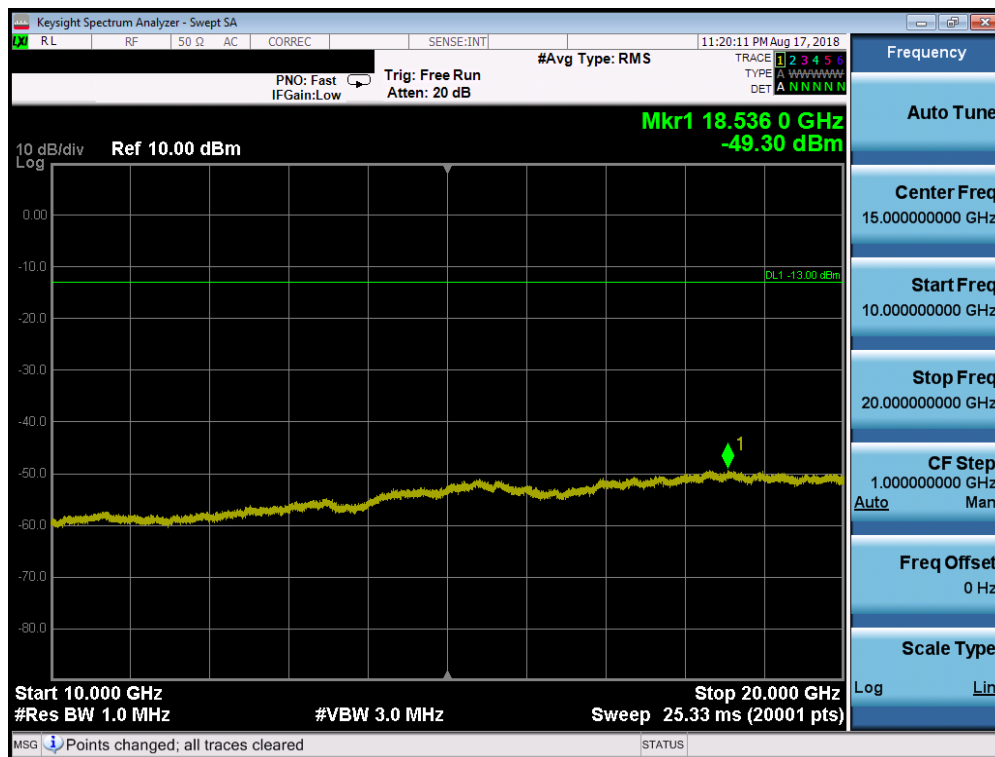
Plot 7-52. Conducted Spurious Plot (PCS WCDMA Mode - High Channel)
