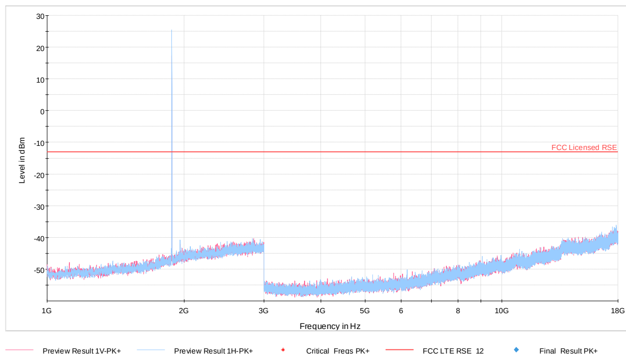
Plot 7-79. Radiated Spurious Data (PCS GPRS Mode)
