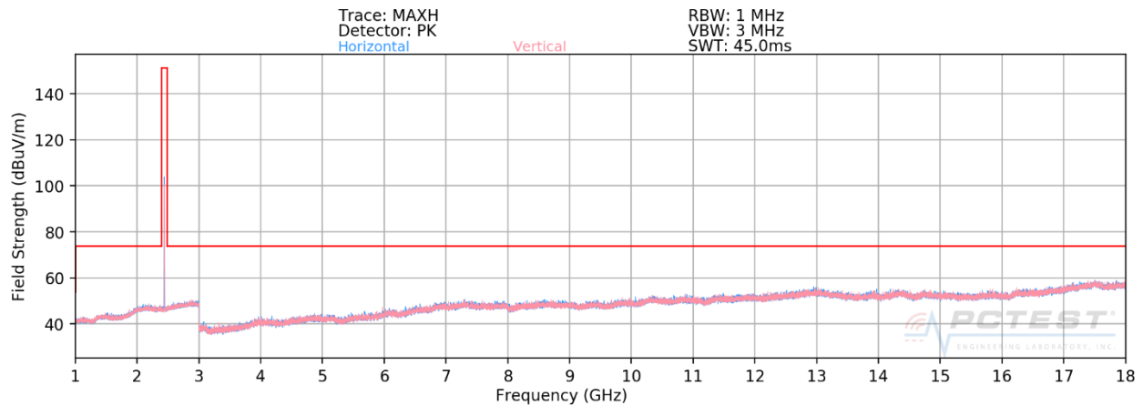
Plot 7-92. Radiated Spurious Plot Above 1GHz ANT1 (4Mbps, HDR4 ePA – Ch. 38, Ant. Pol. H & V)
