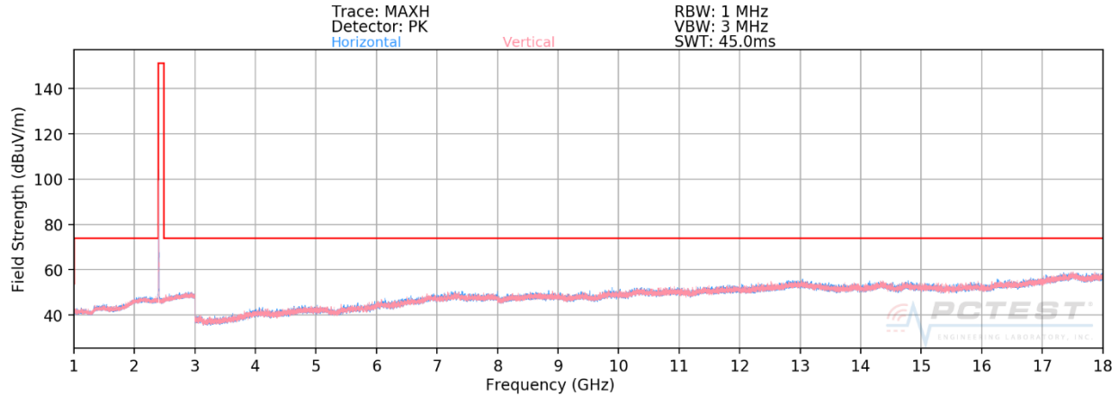
Plot 7-88. Radiated Spurious Plot ANT0 (8Mbps, HDR8, ePA – Ch. 1, Ant. Pol. H & V)
