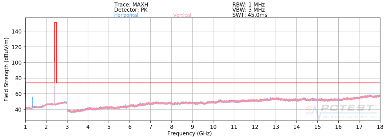
Plot 7-91. Radiated Spurious Plot Above 1GHz ANT1 (4Mbps, HDR4 ePA – Ch. 1, Ant. Pol. H & V)
