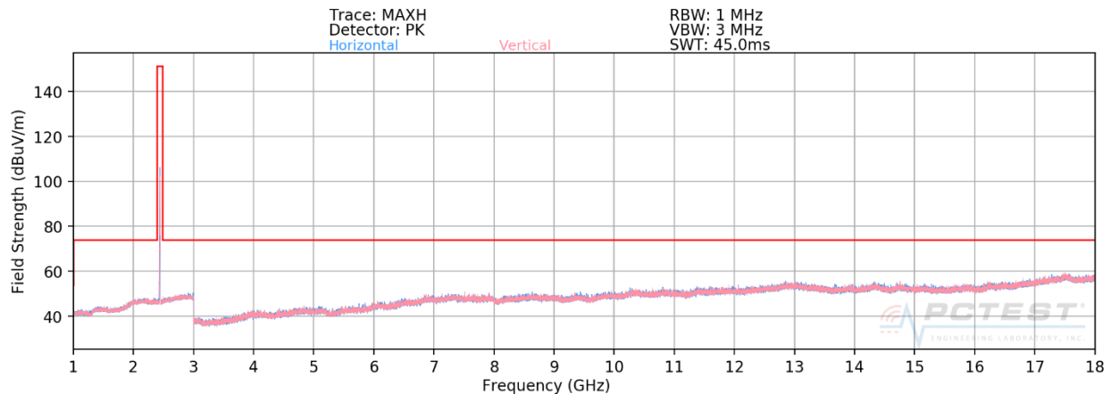
Plot 7-89. Radiated Spurious Plot ANT0 (8Mbps, HDR8, ePA – Ch. 38, Ant. Pol. H & V)
