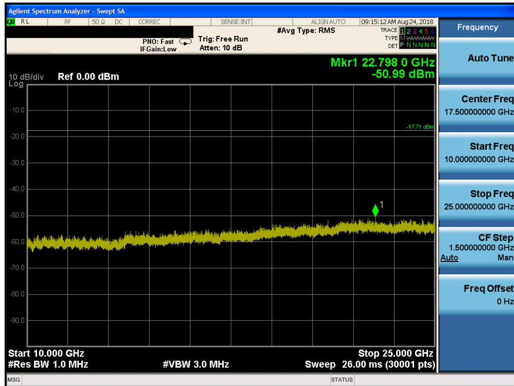
Plot 7-84. Conducted Spurious Plot ANT2 (Bluetooth (HDR4, ePA), 4Mbps – Ch. 75)
