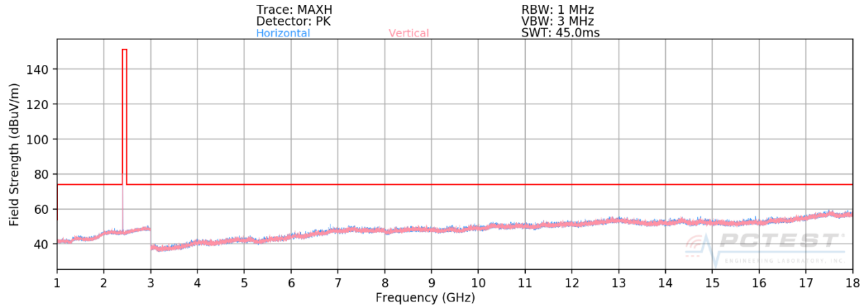
Plot 7-100. Radiated Spurious Plot Above 1GHz ANT2 (8Mbps, HDR8 ePA – Ch. 1, Ant. Pol. H & V)
