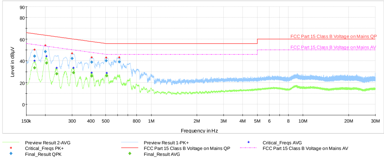
Plot 7-119. Line Conducted Plot with Bluetooth HDR4 Ch.38 ANT0 (N, with AC/DC Adapter)
