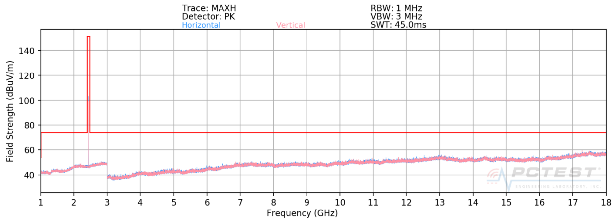
Plot 7-86. Radiated Spurious Plot ANT0 (4Mbps, HDR4, ePA – Ch. 38, Ant. Pol. H & V)
