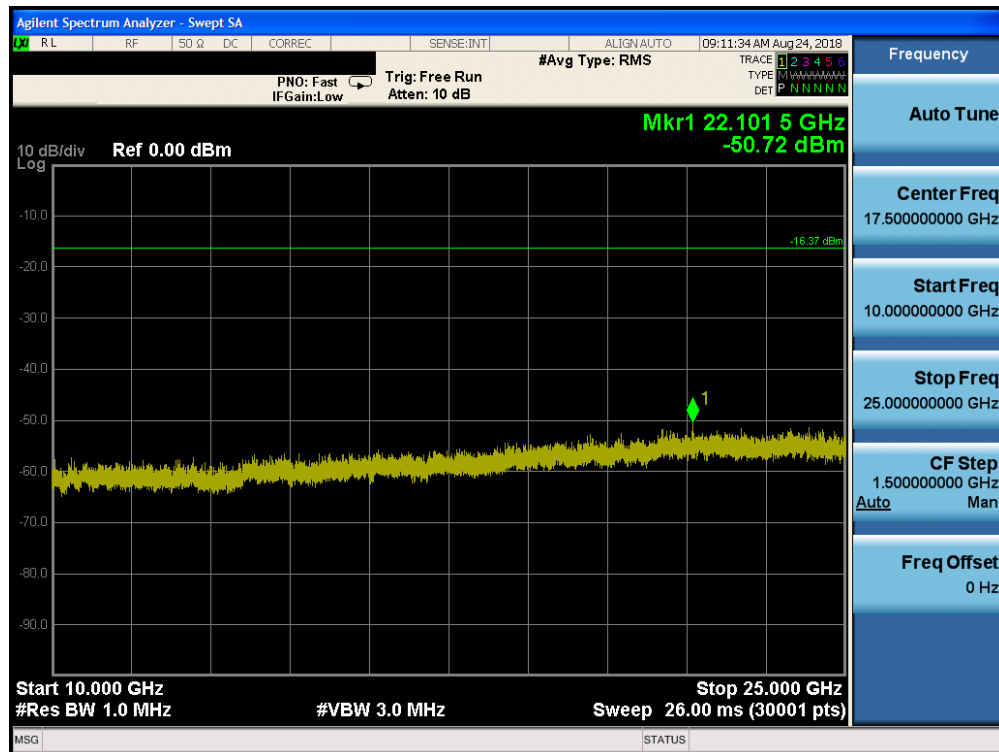
Plot 7-82. Conducted Spurious Plot ANT2 (Bluetooth (HDR4, ePA), 4Mbps – Ch. 38)
