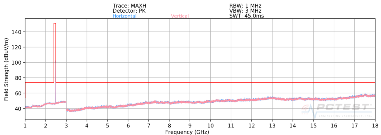
Plot 7-93. Radiated Spurious Plot Above 1GHz ANT1 (4Mbps, HDR4 ePA – Ch. 75, Ant. Pol. H & V)
