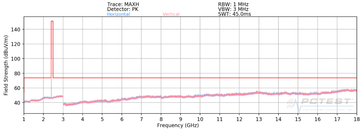
Plot 7-85. Radiated Spurious Plot ANT0 (4Mbps, HDR4, ePA – Ch. 1, Ant. Pol. H & V)
