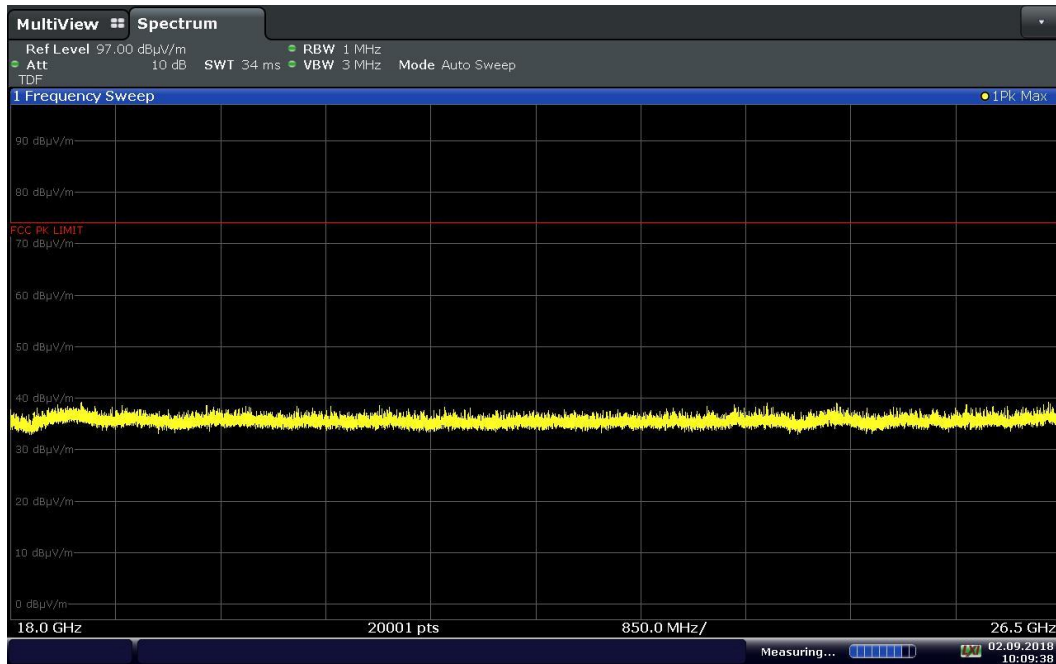
Plot 7-104. Radiated Spurious Plot above 18GHz ANT0 (8Mbps, HDR8 ePA – Ch. 38, Pol. V)
