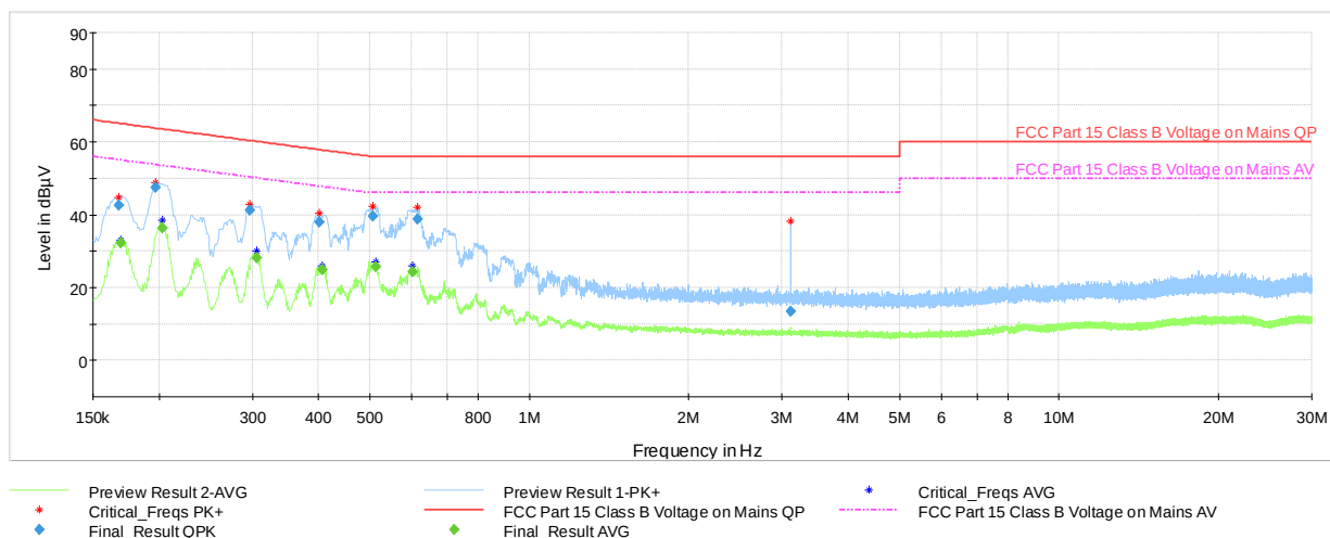
Plot 7-118. Line Conducted Plot with Bluetooth HDR4 Ch.38 ANT0 (L1, with AC/DC Adapter)
