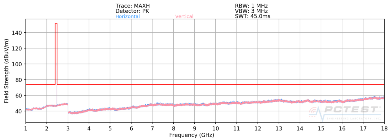
Plot 7-87. Radiated Spurious Plot ANT0 (4Mbps, HDR4, ePA – Ch. 75, Ant. Pol. H & V)
