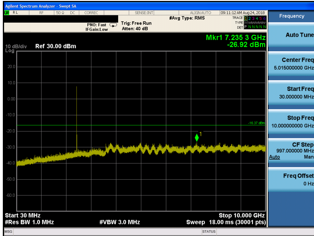
Plot 7-81. Conducted Spurious Plot ANT2 (Bluetooth (HDR4, ePA), 4Mbps – Ch. 38)
