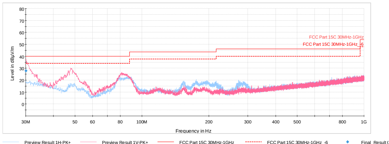
Plot 7-117. Radiated Spurious Plot below 1GHz ANT0 (HDR4, ePA, Ch.38 Pol. H & V, with AC/DC Adapter)
