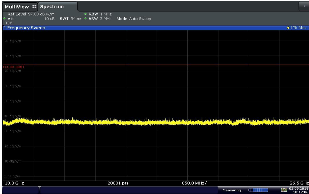
Plot 7-103. Radiated Spurious Plot above 18GHz ANT0 (8Mbps, HDR8 ePA – Ch. 38, Pol. H)
