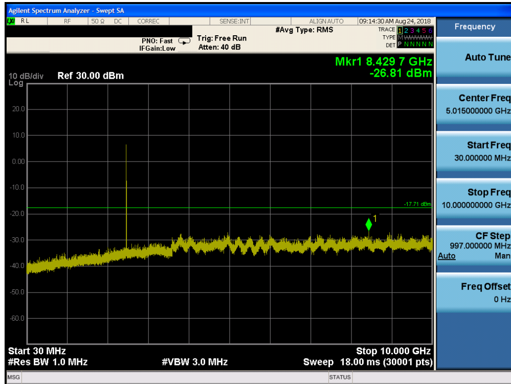
Plot 7-83. Conducted Spurious Plot ANT2 (Bluetooth (HDR4, ePA), 4Mbps – Ch. 75)
