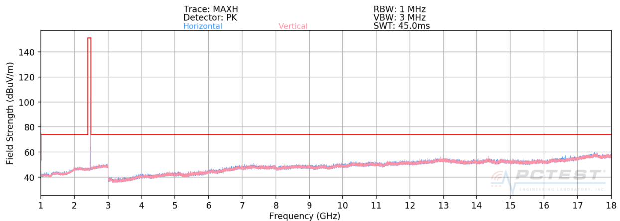
Plot 7-90. Radiated Spurious Plot ANT0 (8Mbps, HDR8, ePA – Ch. 75, Ant. Pol. H & V)
