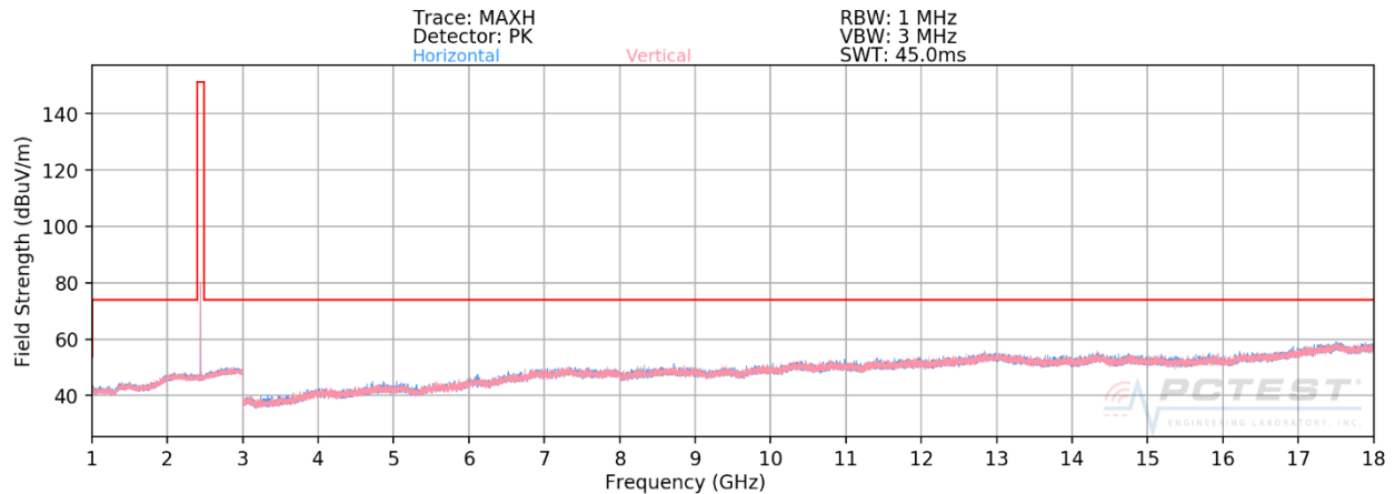
Plot 7-101. Radiated Spurious Plot Above 1GHz ANT2 (8Mbps, HDR8 ePA – Ch. 38, Ant. Pol. H & V)
