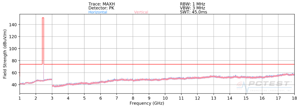
Plot 7-102. Radiated Spurious Plot Above 1GHz ANT2 (8Mbps, HDR8 ePA – Ch. 75, Ant. Pol. H & V)
