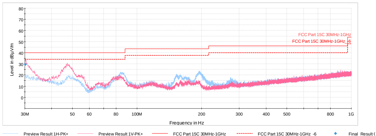
Plot 7-102. Radiated Spurious Plot below 1GHz ANT0 (1Mbps ePA, Ch. 19, Pol. H & V, AC/DC Adapter)
