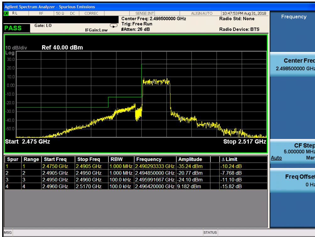
Plot 7-334. Lower ACP Plot (Band 41 – 5.0MHz QPSK – RB Size 25)
