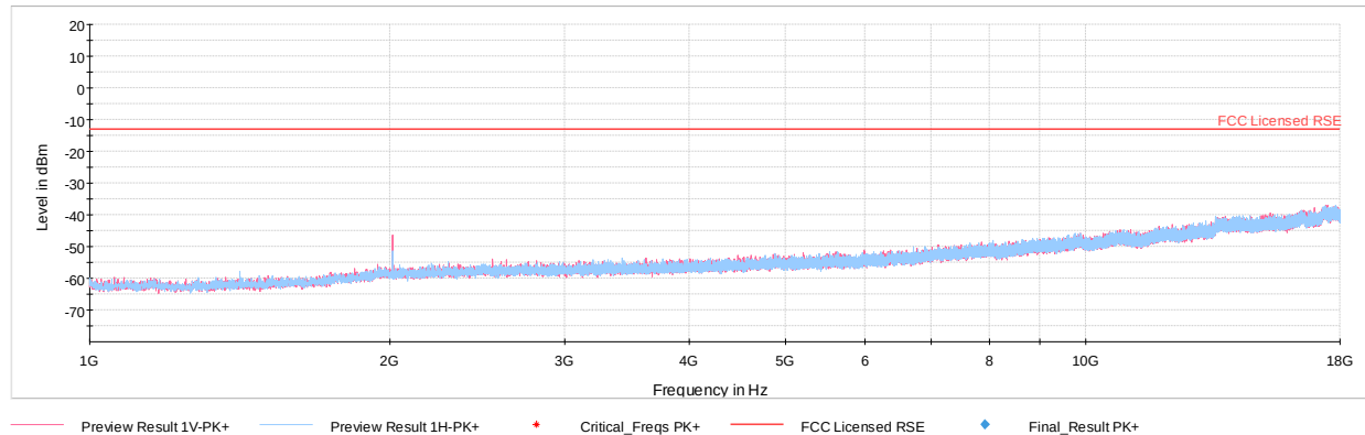
Plot 7-430. Radiated Spurious Plot above 1GHz (Band 71)
