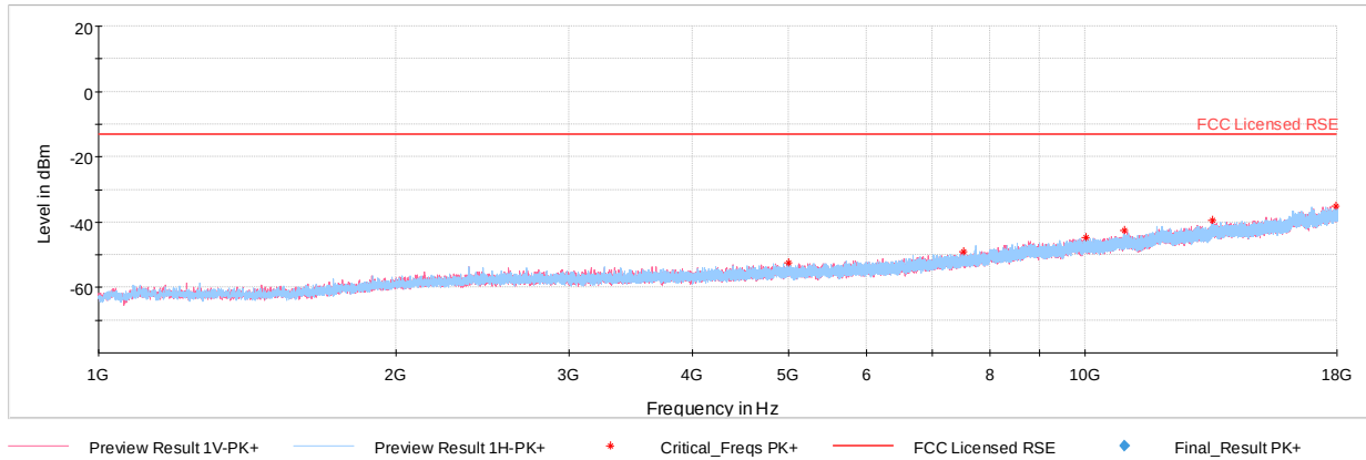
Plot 7-50. Radiated Spurious Plot above 1GHz (Band 14)
