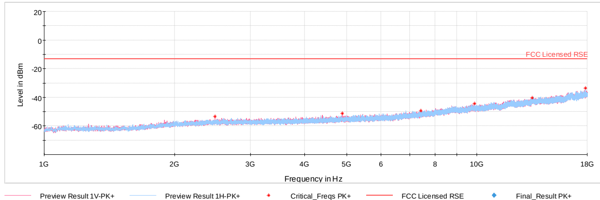
Plot 7-49. Radiated Spurious Plot above 1GHz (Band 26)
