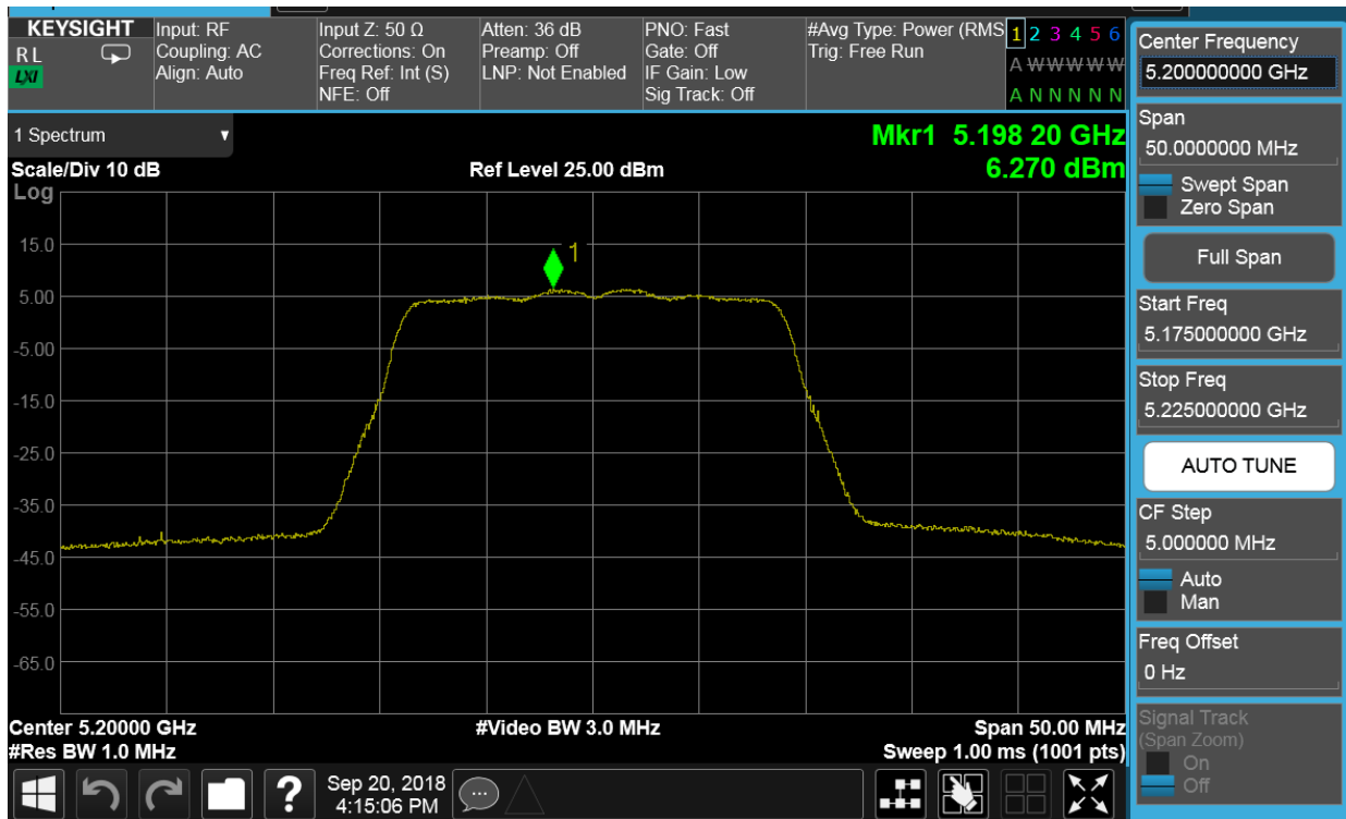
Plot 7-54. Power Spectral Density Plot SISO CORE0 (20MHz BW 802.11n (UNII Band 1) – Ch. 40)
