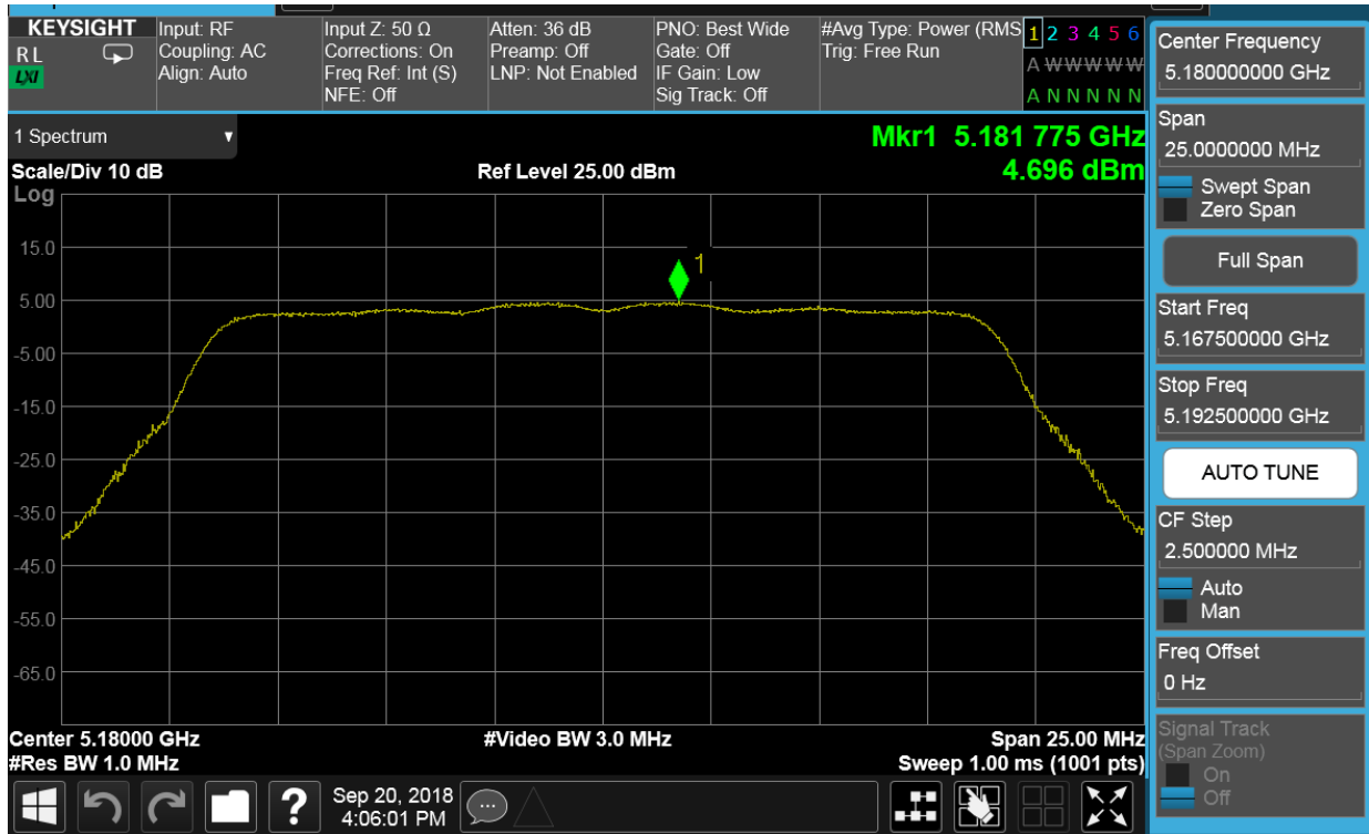
Plot 7-53. Power Spectral Density Plot SISO CORE0 (20MHz BW 802.11n (UNII Band 1) – Ch. 36)
