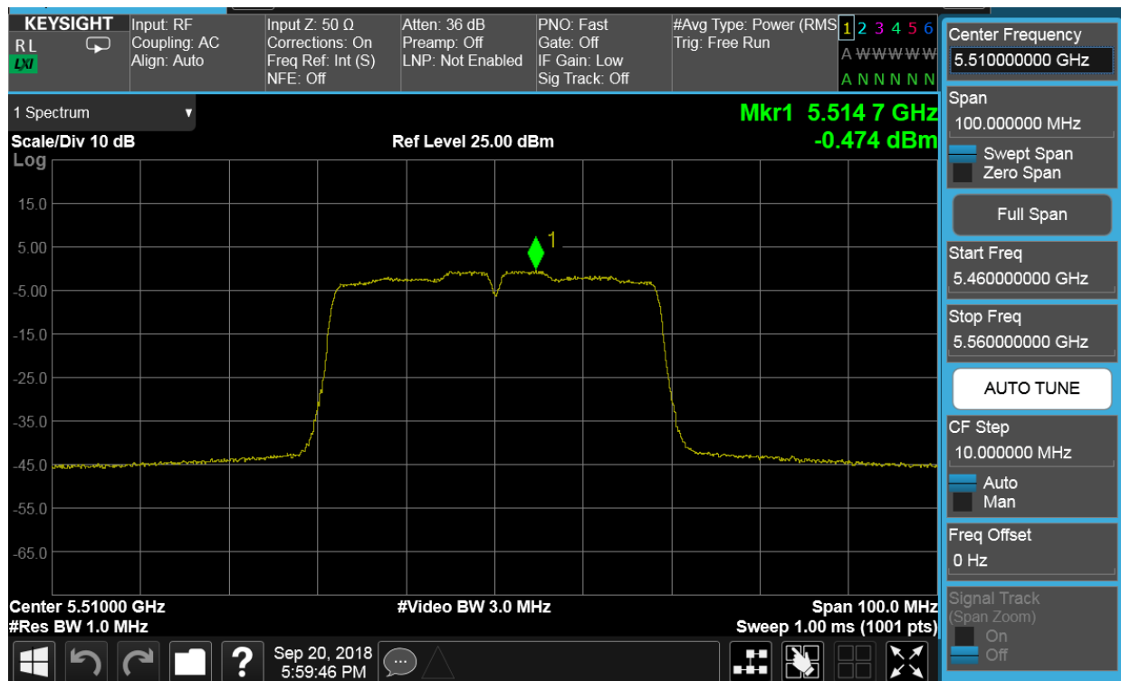
Plot 7-68. Power Spectral Density Plot SISO CORE0 (40MHz BW 802.11n (UNII Band 2C) – Ch. 102)
