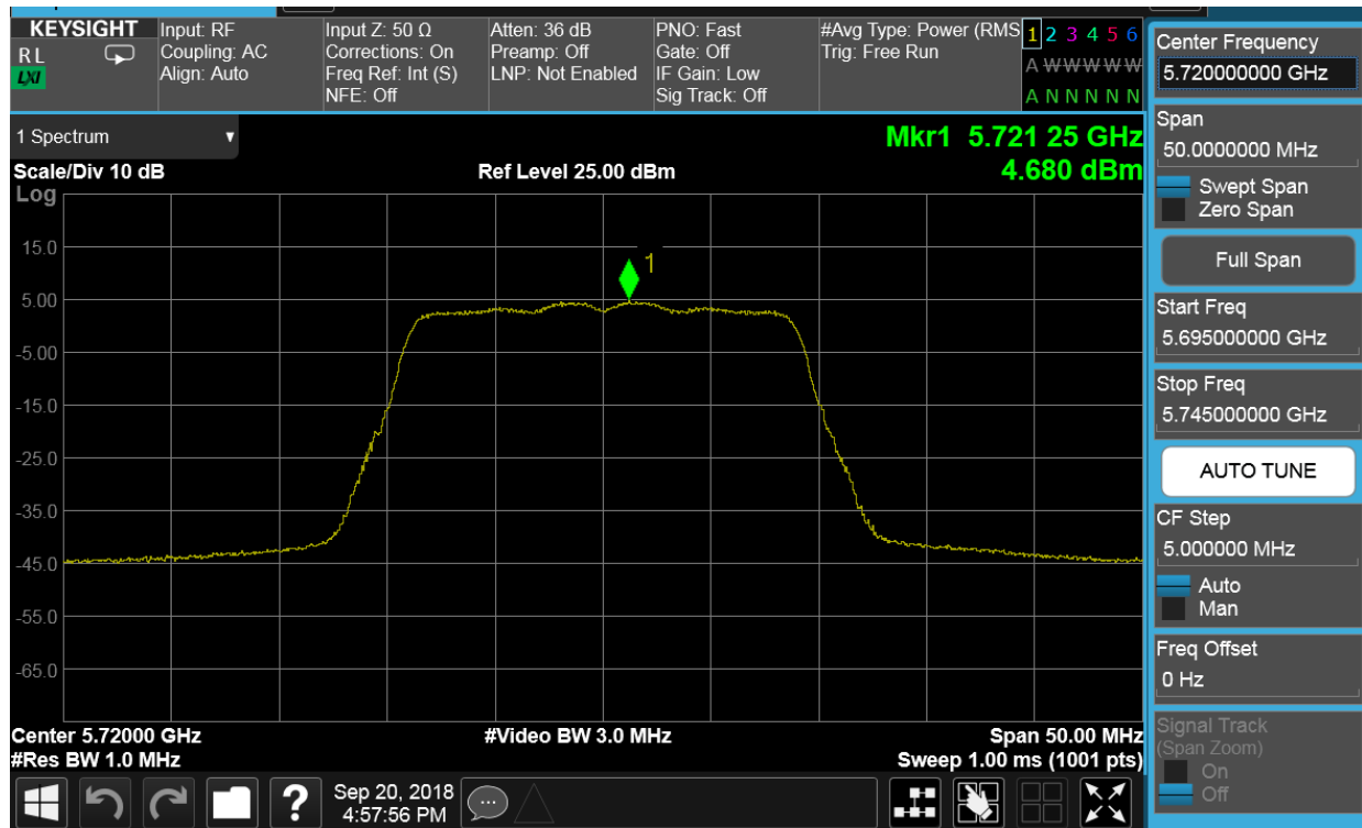
Plot 7-67. Power Spectral Density Plot SISO CORE0 (20MHz BW 802.11n (UNII Band 2C) – Ch. 144)
