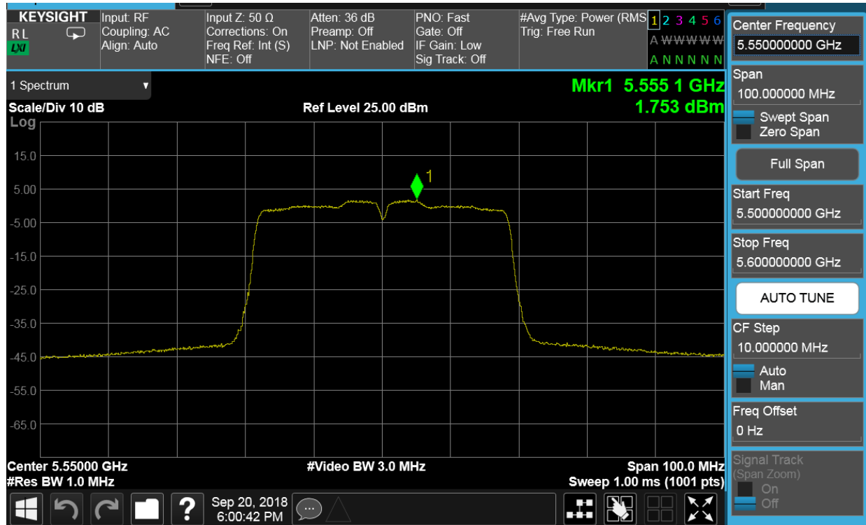
Plot 7-69. Power Spectral Density Plot SISO CORE0 (40MHz BW 802.11n (UNII Band 2C) – Ch. 110)
