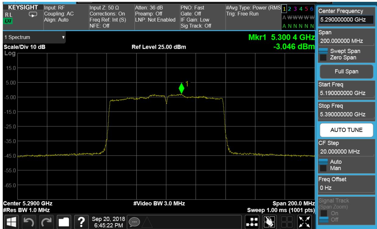
Plot 7-64. Power Spectral Density Plot SISO CORE0 (80MHz BW 802.11ac (UNII Band 2A) – Ch. 58)
