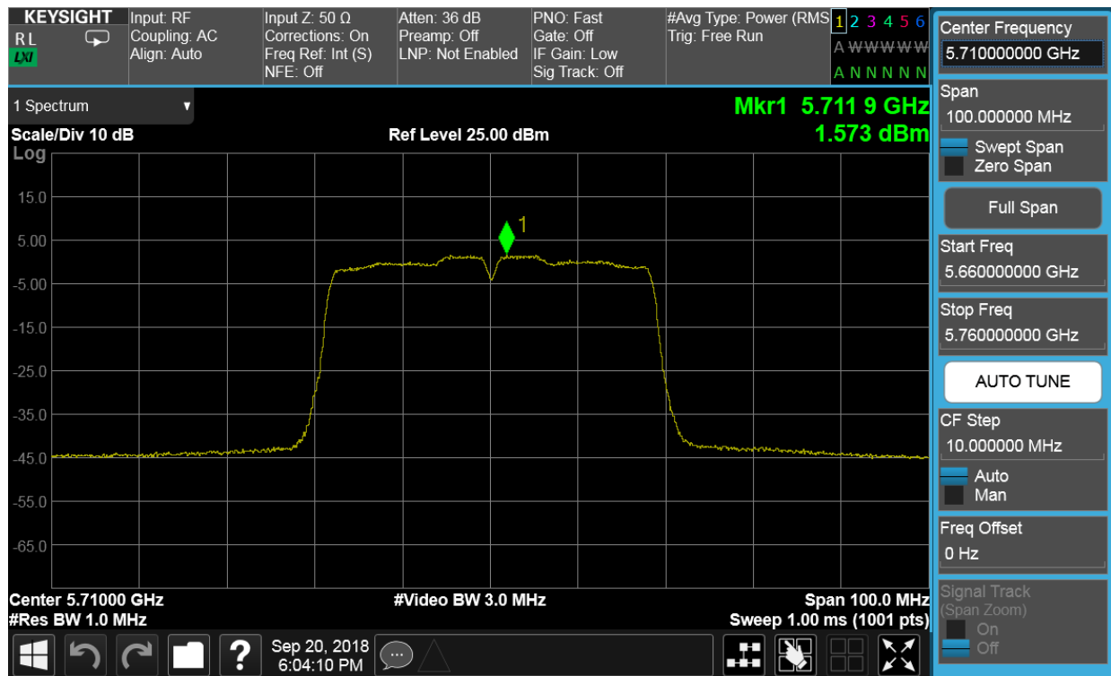
Plot 7-70. Power Spectral Density Plot SISO CORE0 (40MHz BW 802.11n (UNII Band 2C) – Ch. 142)
