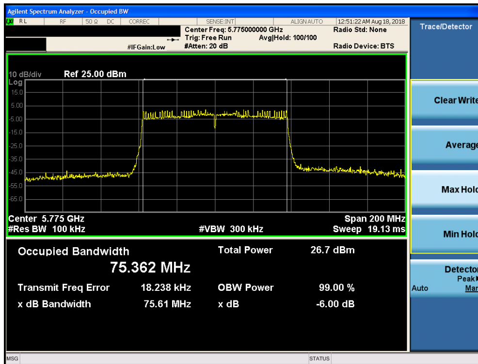
Plot 7-52. 6dB Bandwidth Plot SISO CORE1 (80MHz BW 802.11ac (UNII Band 3) – Ch. 155)
