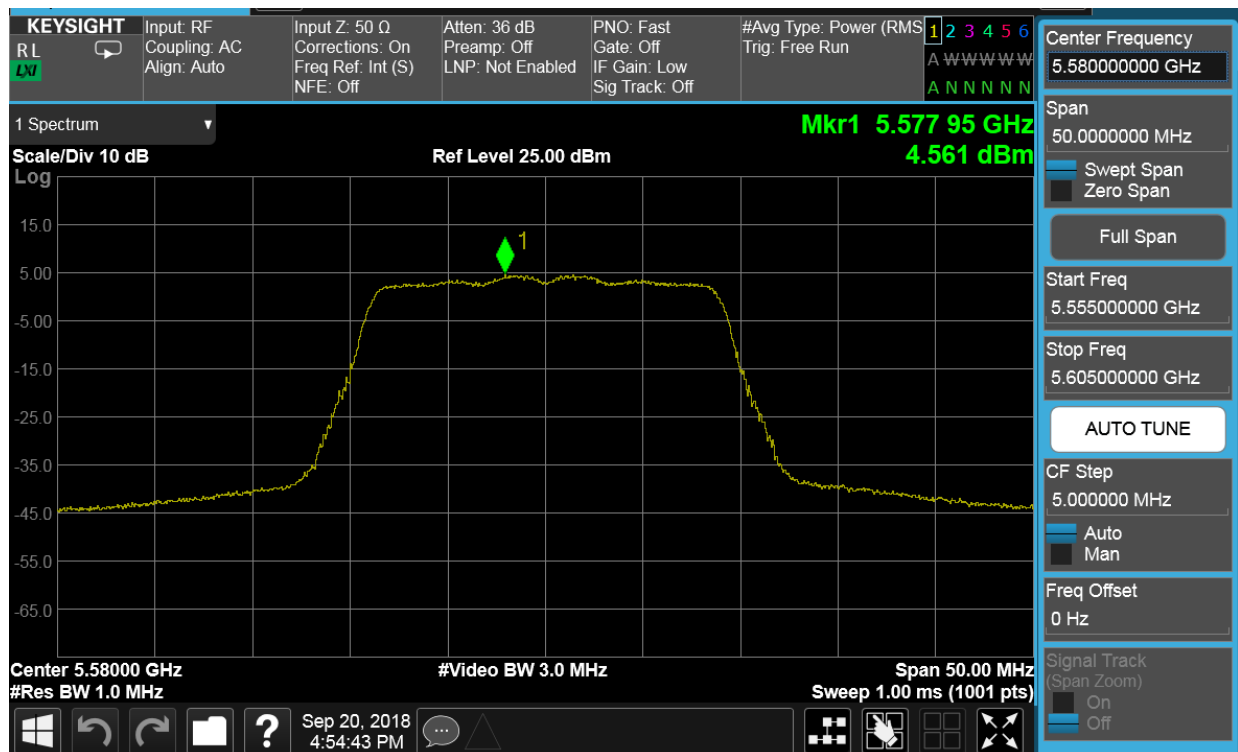
Plot 7-66. Power Spectral Density Plot SISO CORE0 (20MHz BW 802.11n (UNII Band 2C) – Ch. 116)
