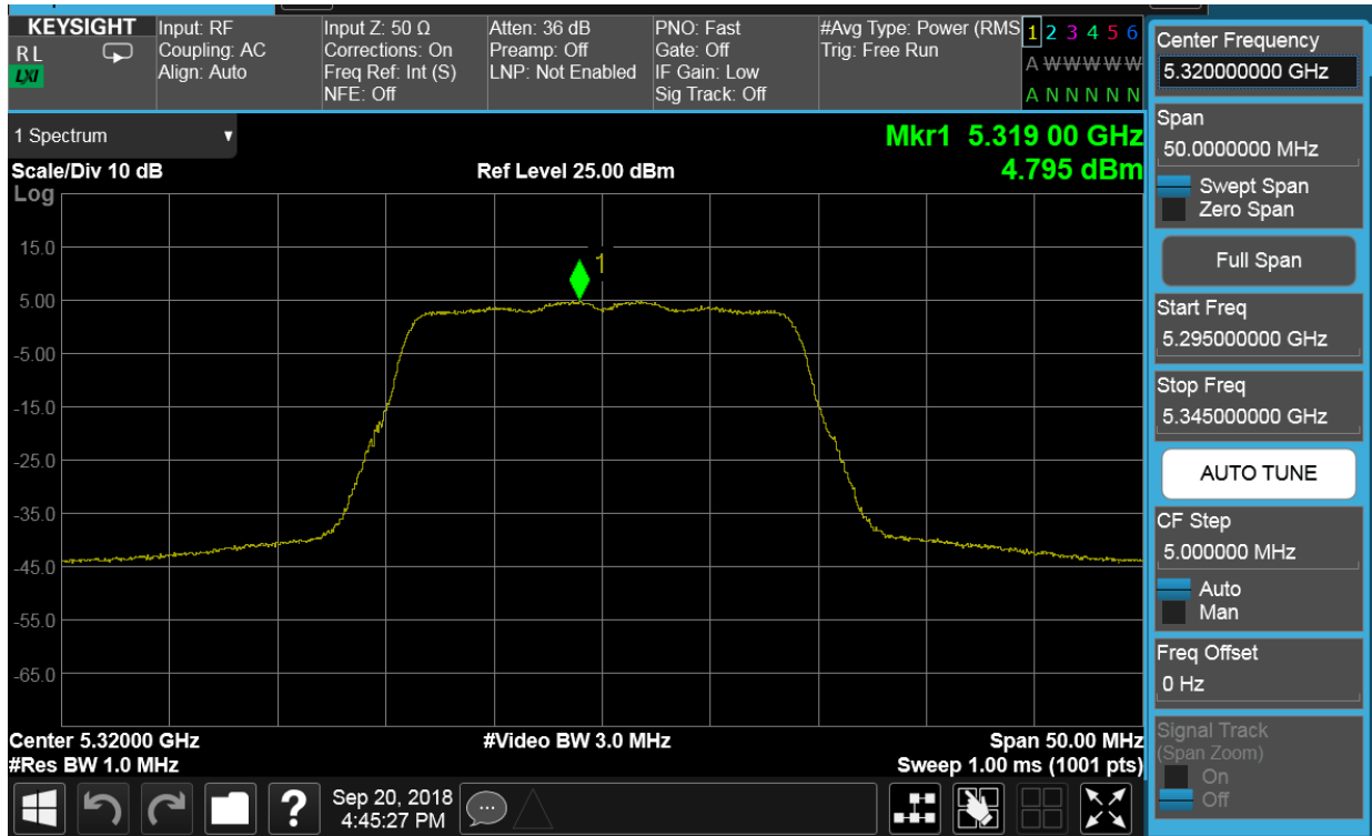
Plot 7-61. Power Spectral Density Plot SISO CORE0 (20MHz BW 802.11n (UNII Band 2A) – Ch. 64)
