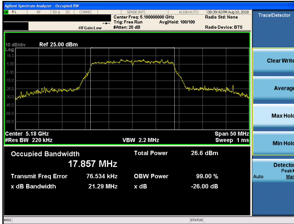
Plot 7-1. 26dB Bandwidth Plot SISO CORE0 (20MHz BW 802.11n (UNII Band 1) – Ch. 36)
