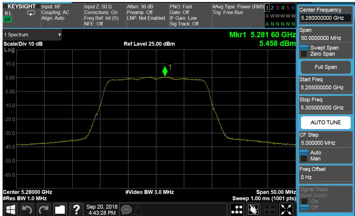
Plot 7-60. Power Spectral Density Plot SISO CORE0 (20MHz BW 802.11n (UNII Band 2A) – Ch. 56)
