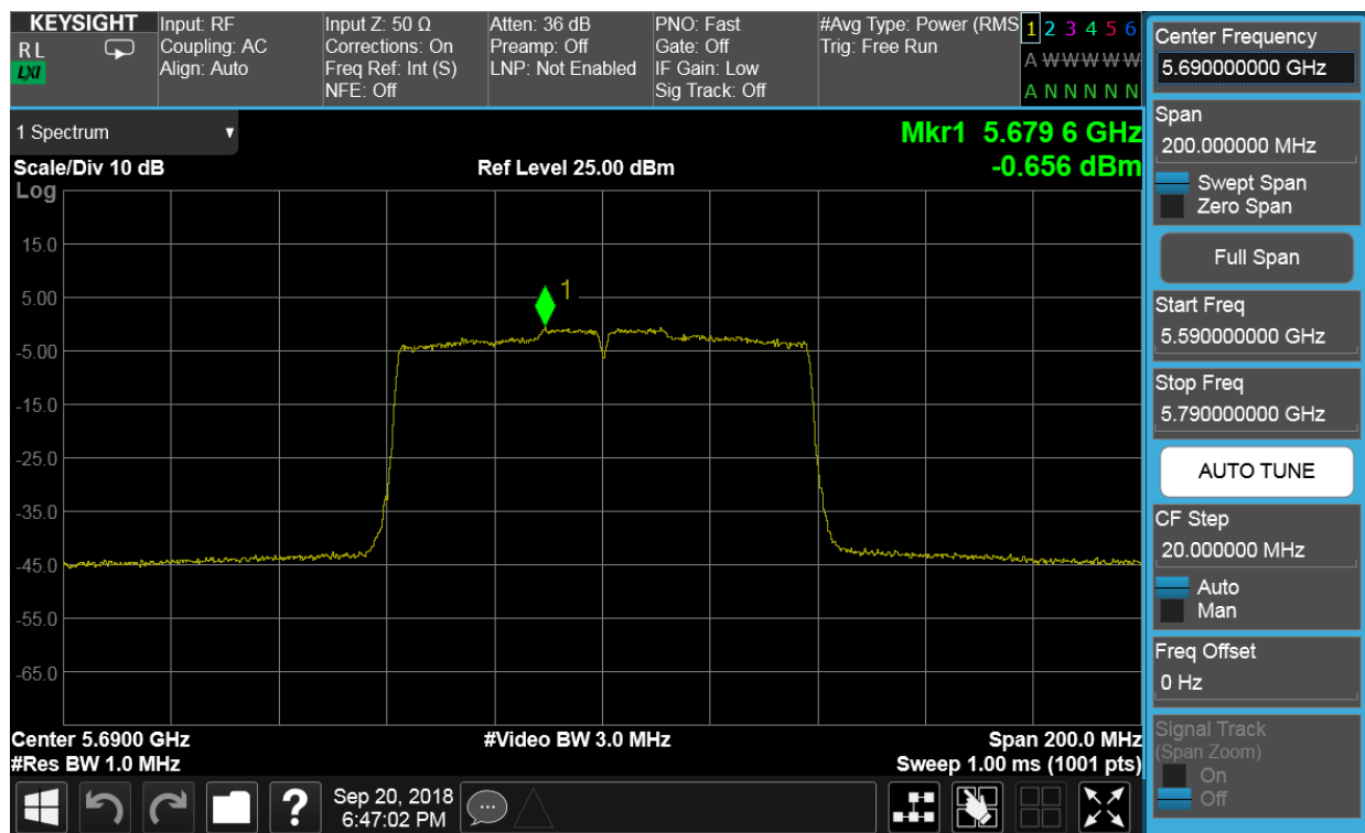
Plot 7-72. Power Spectral Density Plot SISO CORE0 (80MHz BW 802.11ac (UNII Band 2C) – Ch. 138)
