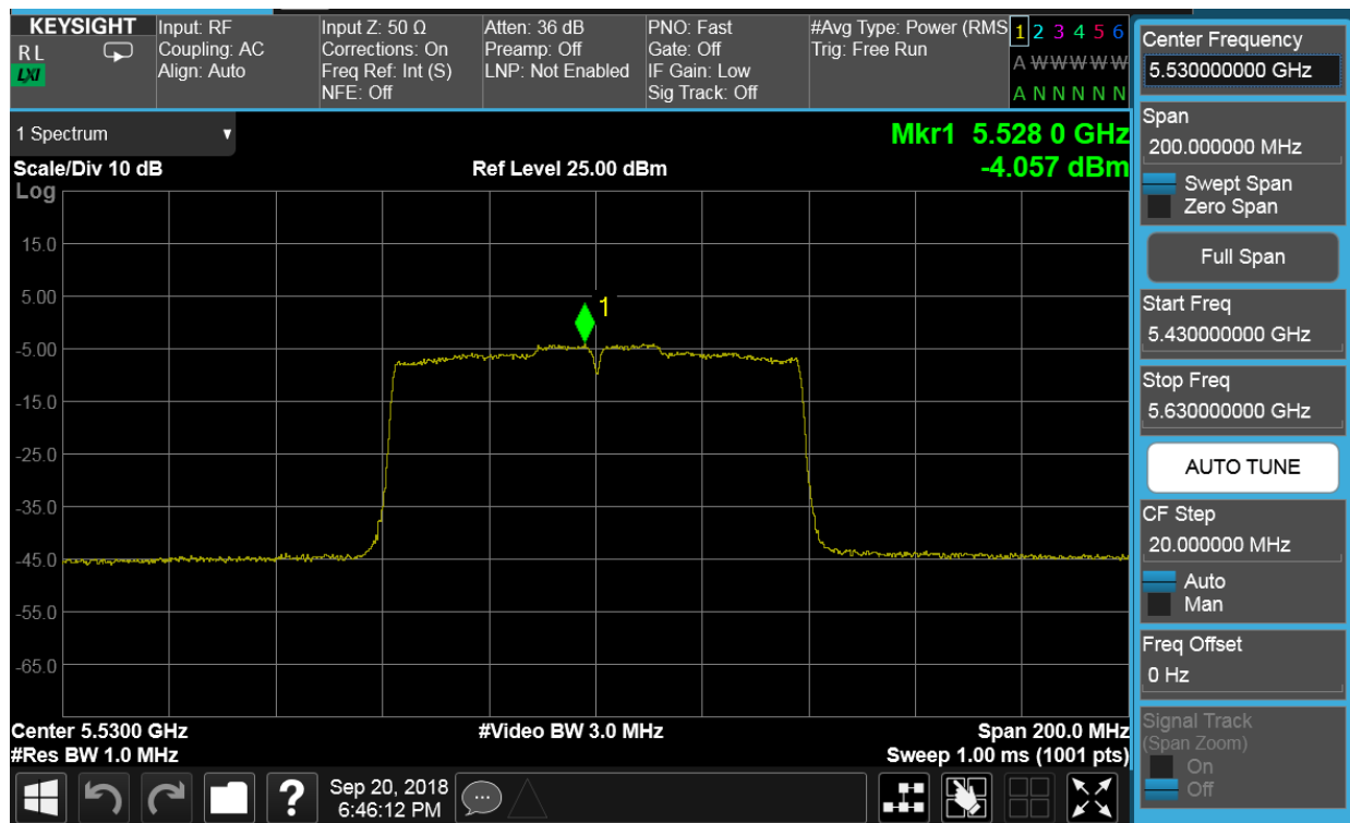
Plot 7-71. Power Spectral Density Plot SISO CORE0 (80MHz BW 802.11ac (UNII Band 2C) – Ch. 106)
