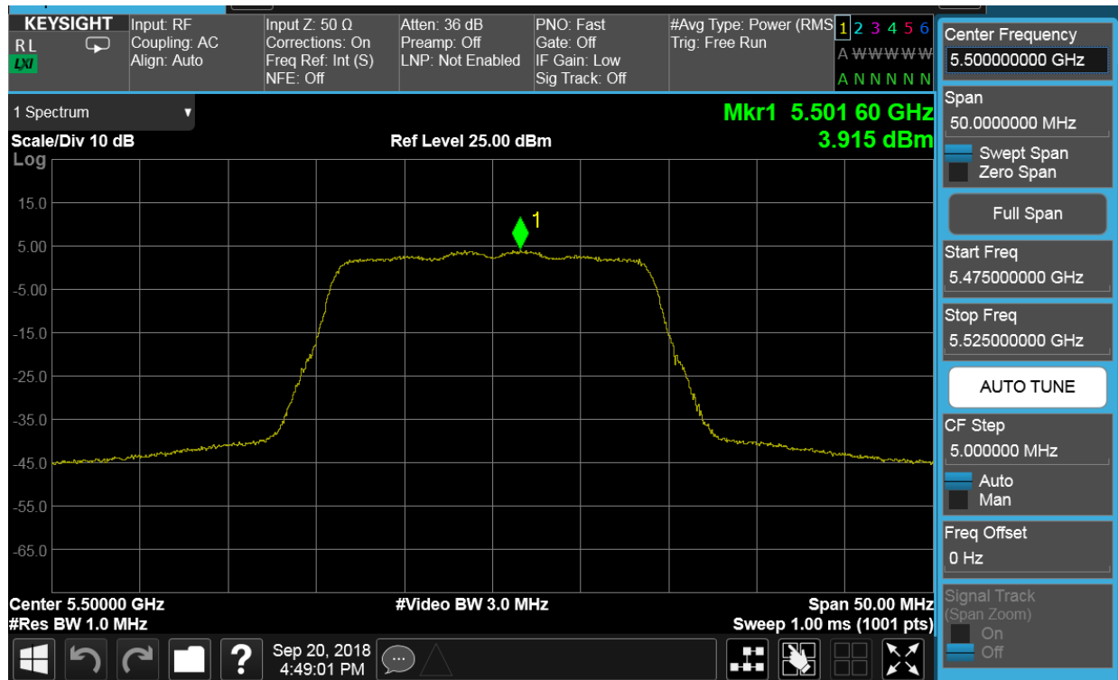
Plot 7-65. Power Spectral Density Plot SISO CORE0 (20MHz BW 802.11n (UNII Band 2C) – Ch. 100)
