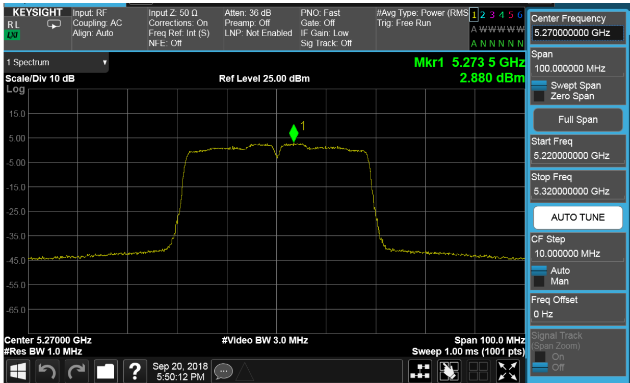
Plot 7-62. Power Spectral Density Plot SISO CORE0 (40MHz BW 802.11n (UNII Band 2A) – Ch. 54)
