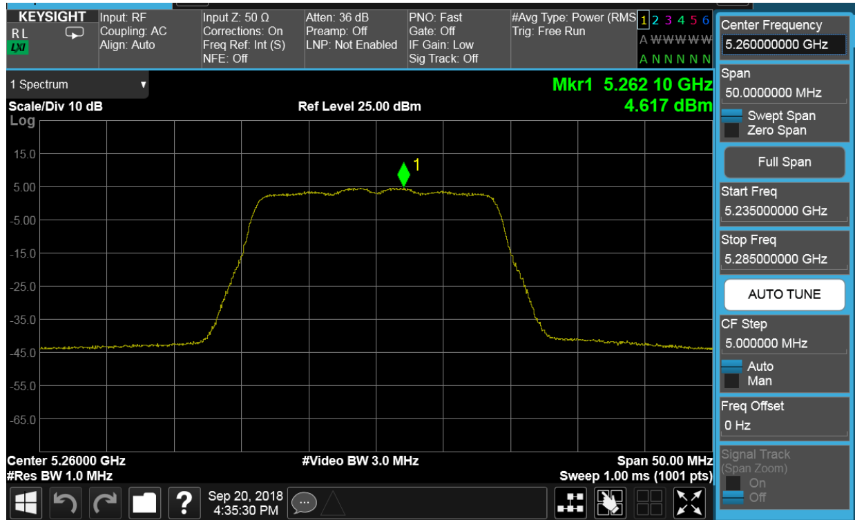
Plot 7-59. Power Spectral Density Plot SISO CORE0 (20MHz BW 802.11n (UNII Band 2A) – Ch. 52)
