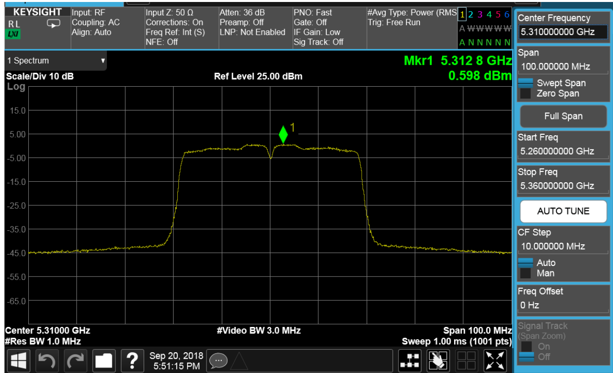
Plot 7-63. Power Spectral Density Plot SISO CORE0 (40MHz BW 802.11n (UNII Band 2A) – Ch. 62)
