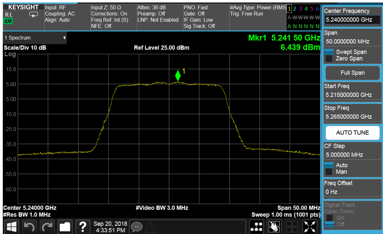
Plot 7-55. Power Spectral Density Plot SISO CORE0 (20MHz BW 802.11n (UNII Band 1) – Ch. 48)
