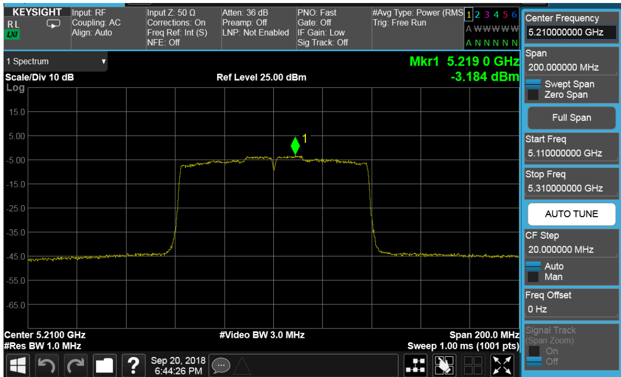
Plot 7-58. Power Spectral Density Plot SISO CORE0 (80MHz BW 802.11ac (UNII Band 1) – Ch. 42)
