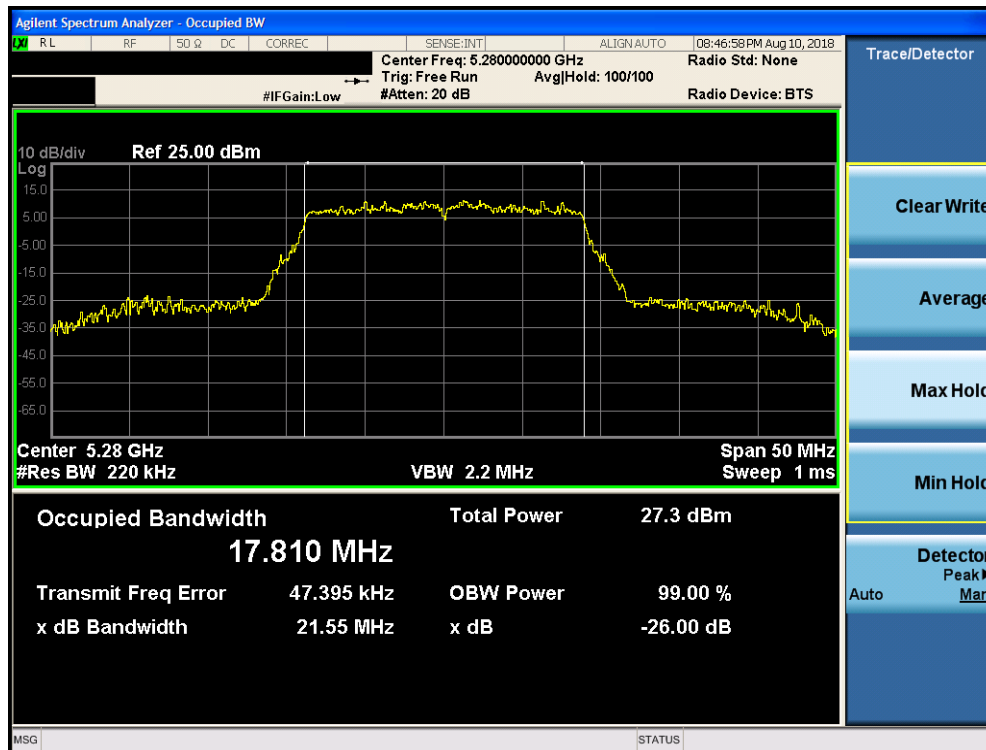
Plot 7-8. 26dB Bandwidth Plot SISO CORE0 (20MHz BW 802.11n (UNII Band 2A) – Ch. 56)
