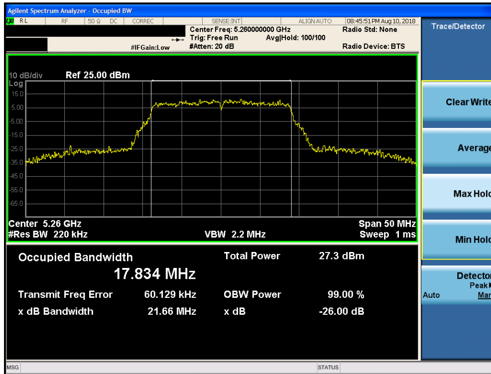
Plot 7-7. 26dB Bandwidth Plot SISO CORE0 (20MHz BW 802.11n (UNII Band 2A) – Ch. 52)
