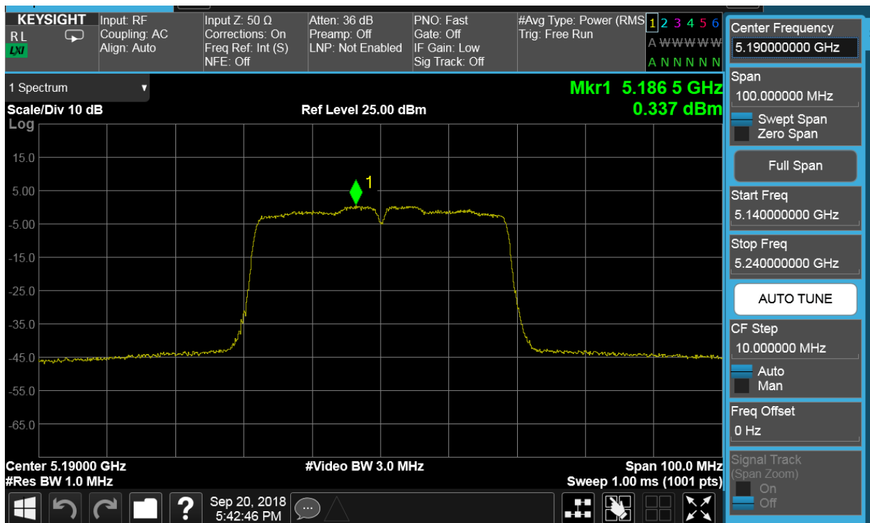
Plot 7-56. Power Spectral Density Plot SISO CORE0 (40MHz BW 802.11n (UNII Band 1) – Ch. 38)
