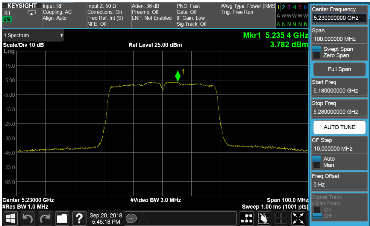
Plot 7-57. Power Spectral Density Plot SISO CORE0 (40MHz BW 802.11n (UNII Band 1) – Ch. 46)
