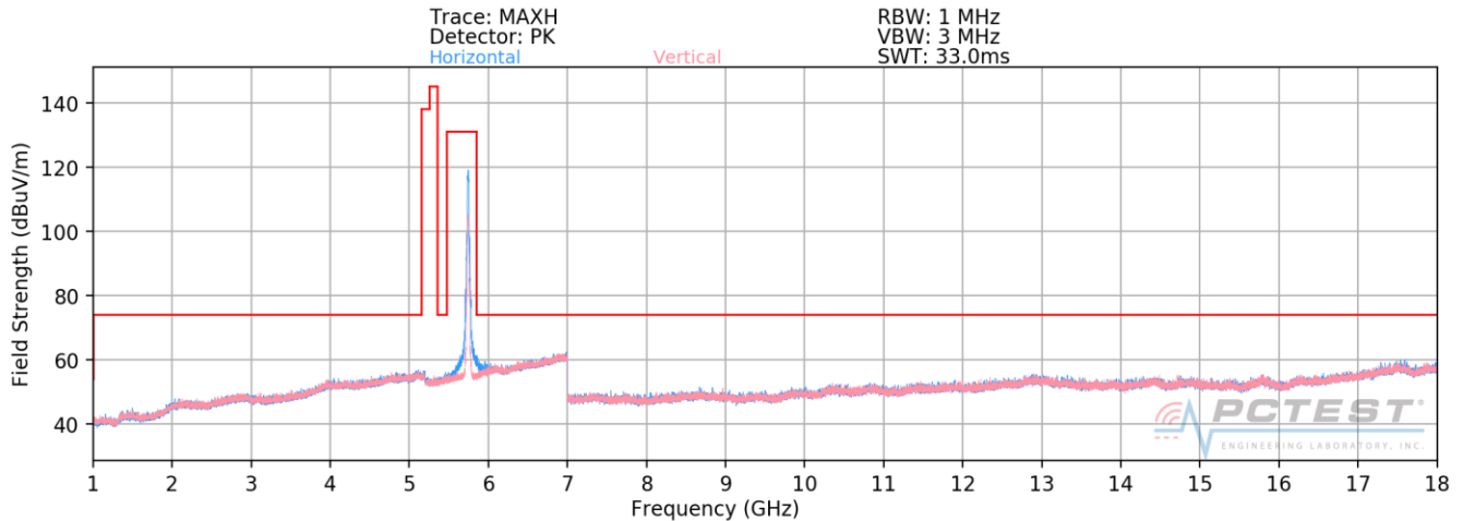
Plot 7-176. Radiated Spurious Plot above 1GHz SISO CORE0 (802.11n – U3 Ch. 149)
