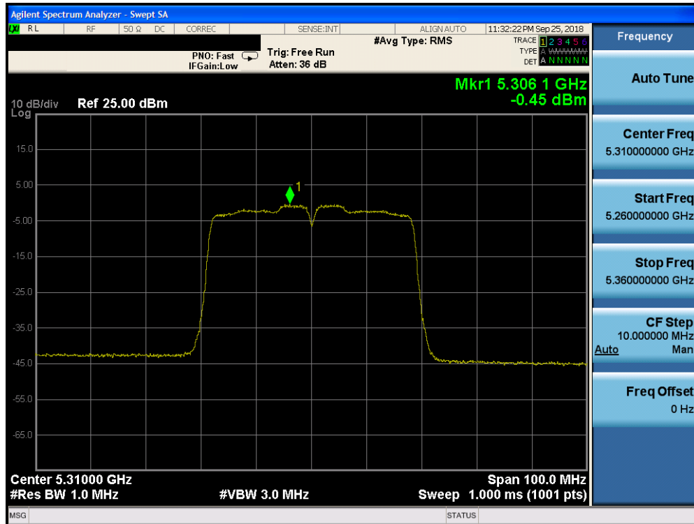
Plot 7-135. Power Spectral Density Plot CDD CORE 0 (40MHz BW 802.11n (UNII Band 2A) – Ch. 62)
