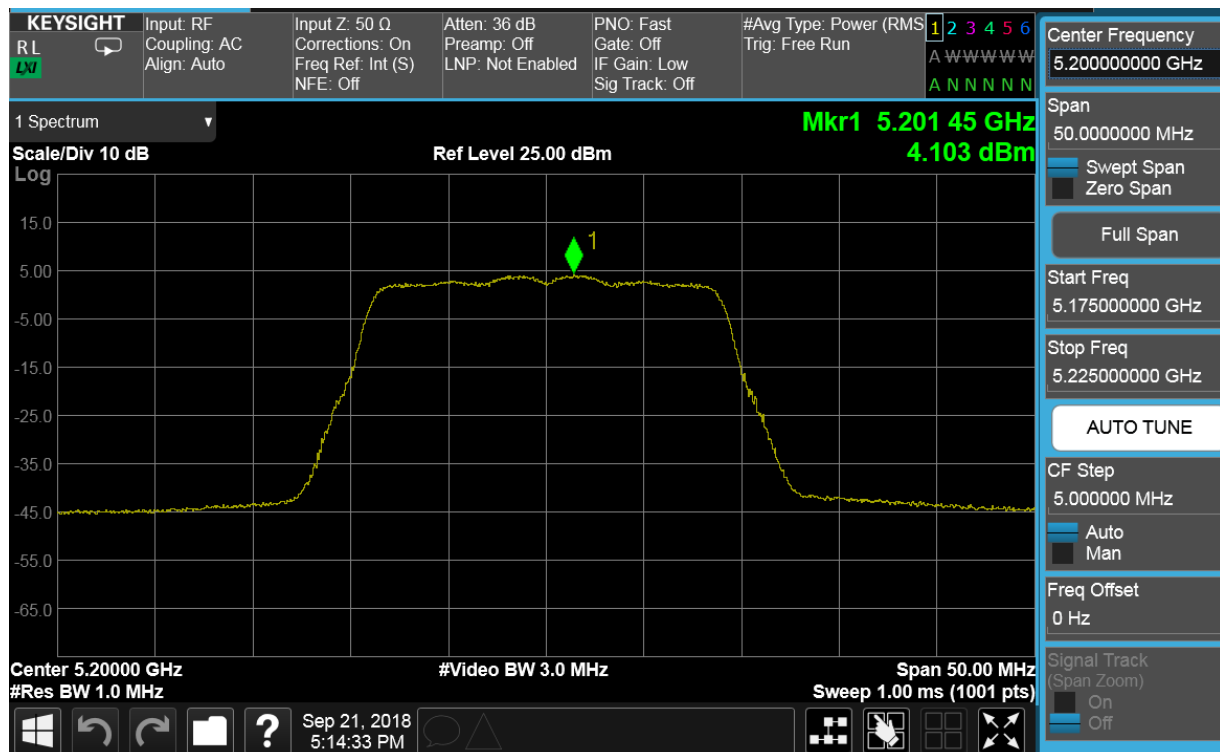
Plot 7-118. Power Spectral Density Plot CDD CORE 1 (20MHz BW 802.11n (UNII Band 1) – Ch. 40)
