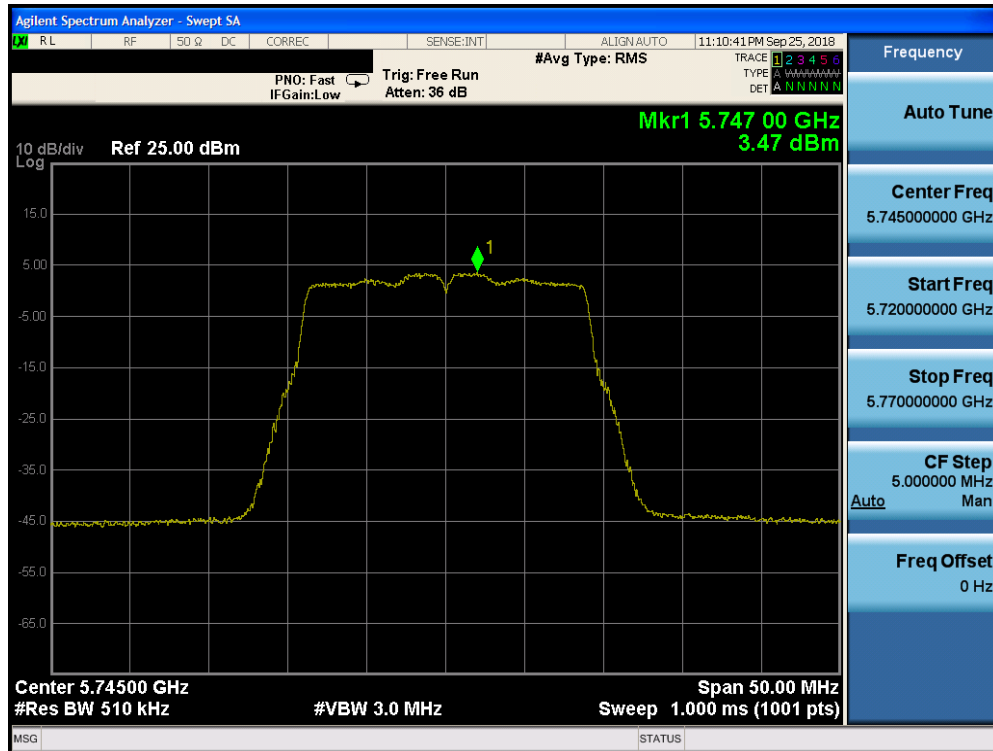
Plot 7-155. Power Spectral Density Plot CDD CORE 0 (20MHz BW 802.11n (UNII Band 3) – Ch. 149)
