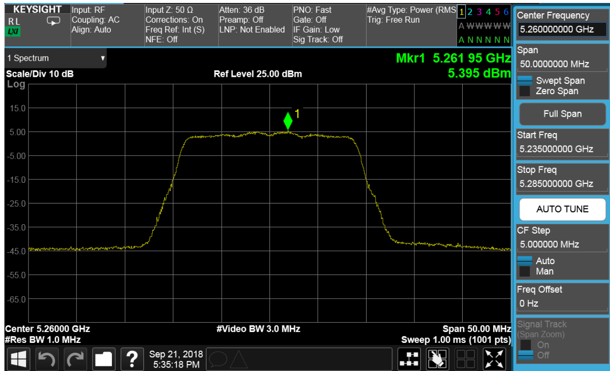
Plot 7-128. Power Spectral Density Plot CDD CORE 1 (20MHz BW 802.11n (UNII Band 2A) – Ch. 52)
