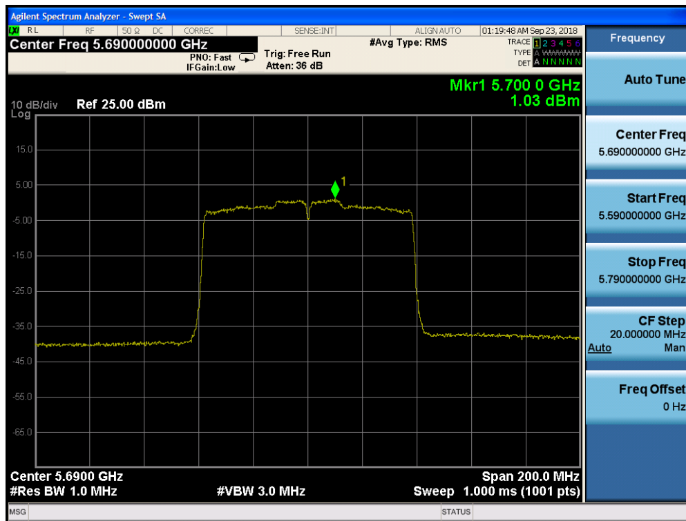
Plot 7-154. Power Spectral Density Plot CDD CORE 1 (80MHz BW 802.11ac (UNII Band 2C) – Ch. 138)
