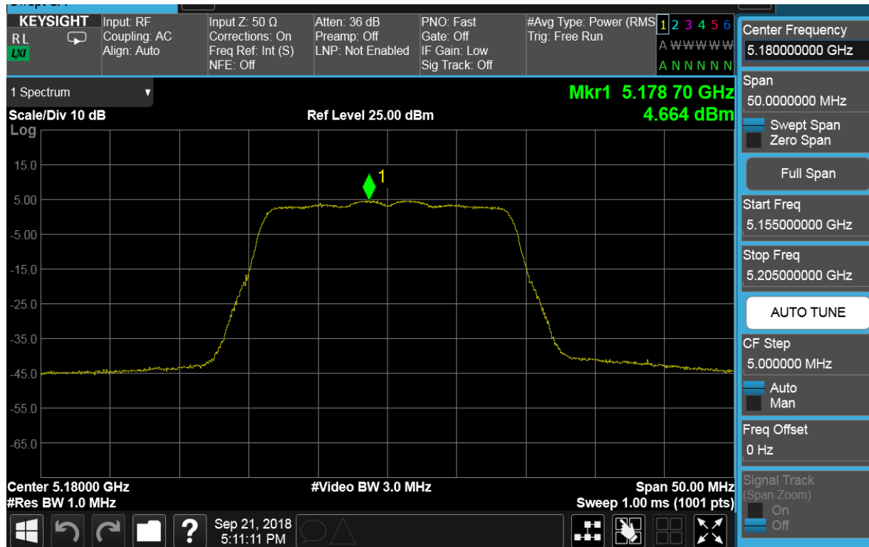
Plot 7-116. Power Spectral Density Plot CDD CORE 1 (20MHz BW 802.11n (UNII Band 1) – Ch. 36)
