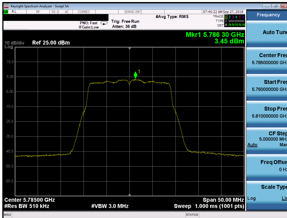
Plot 7-100. Power Spectral Density Plot SISO CORE1 (20MHz BW 802.11n (UNII Band 3) – Ch. 157)
