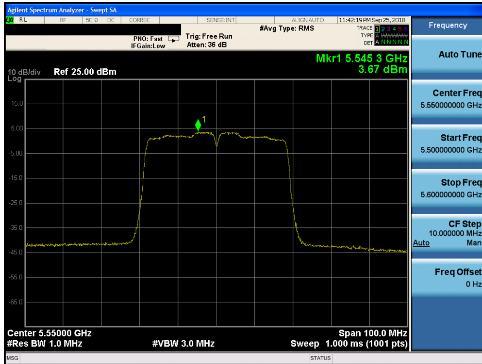
Plot 7-147. Power Spectral Density Plot CDD CORE 0 (40MHz BW 802.11n (UNII Band 2C) – Ch. 110)
