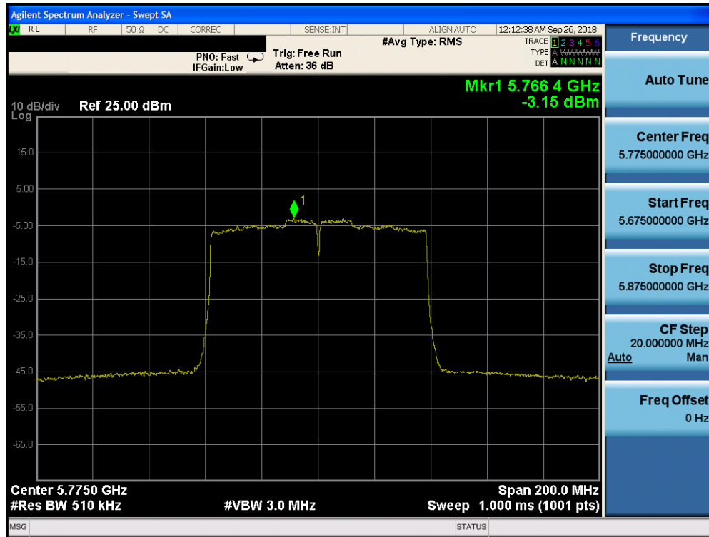
Plot 7-165. Power Spectral Density Plot CDD CORE 0 (80MHz BW 802.11ac (UNII Band 3) – Ch. 155)
