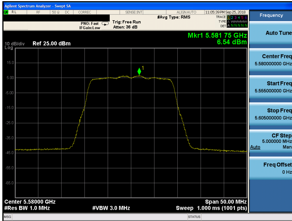
Plot 7-141. Power Spectral Density Plot CDD CORE 0 (20MHz BW 802.11n (UNII Band 2C) – Ch. 116)
