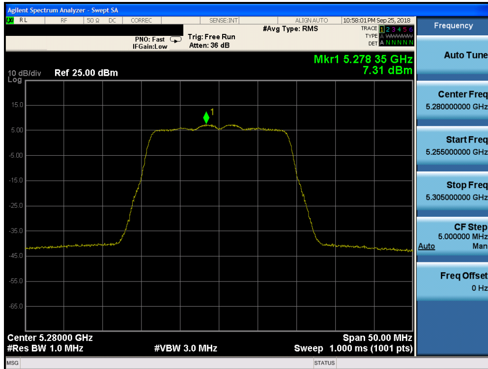
Plot 7-129. Power Spectral Density Plot CDD CORE 0 (20MHz BW 802.11n (UNII Band 2A) – Ch. 56)
