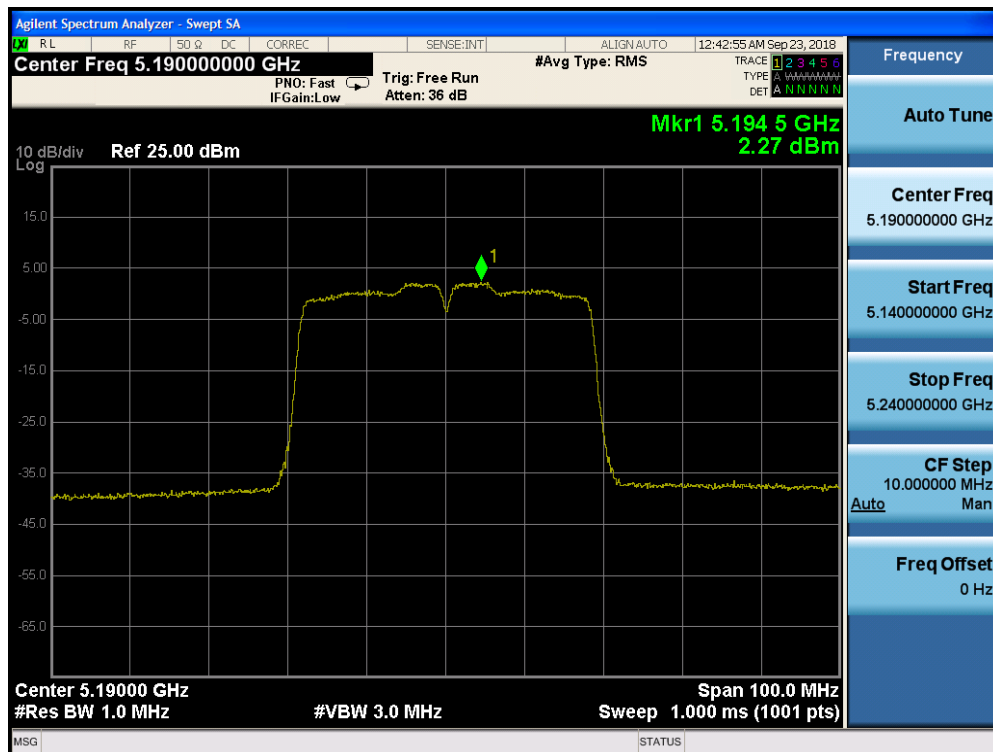
Plot 7-122. Power Spectral Density Plot CDD CORE 1 (40MHz BW 802.11n (UNII Band 1) – Ch. 38)
