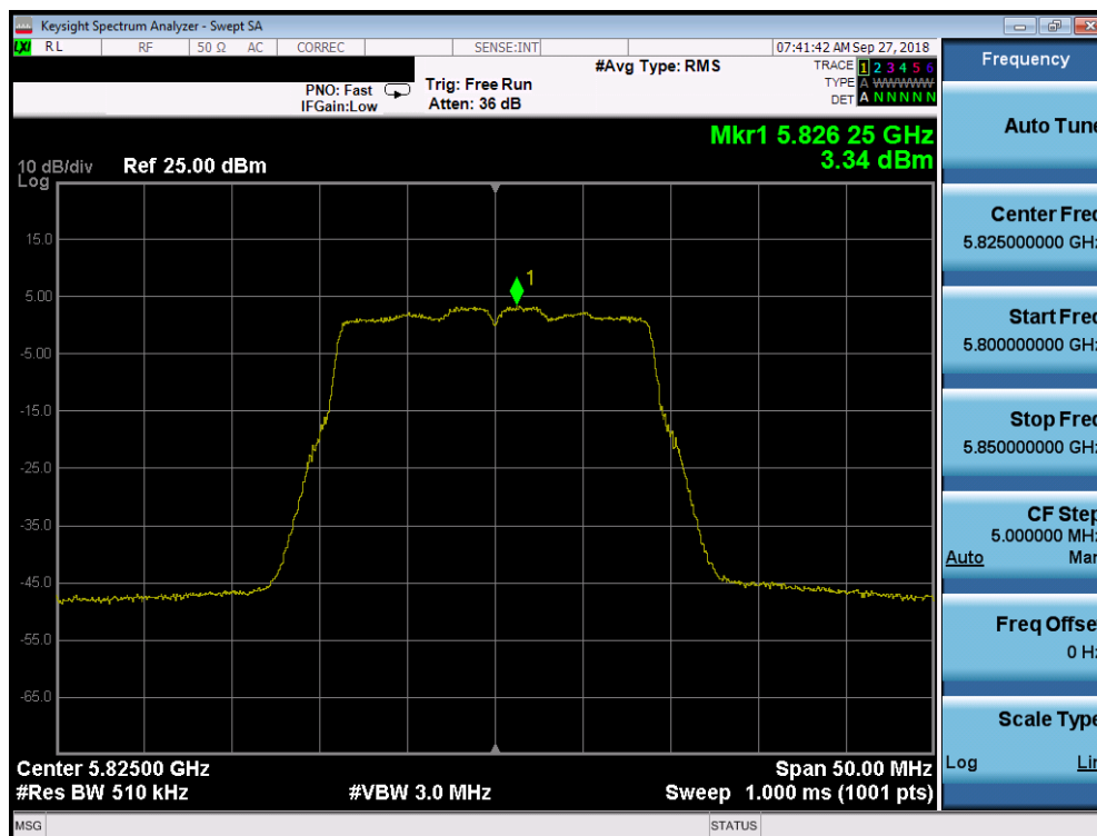
Plot 7-101. Power Spectral Density Plot SISO CORE1 (20MHz BW 802.11n (UNII Band 3) – Ch. 165)
