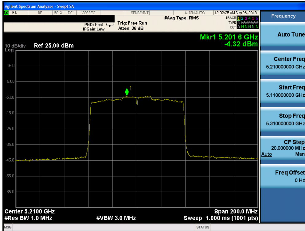
Plot 7-125. Power Spectral Density Plot CDD CORE 0 (80MHz BW 802.11ac (UNII Band 1) – Ch. 42)
