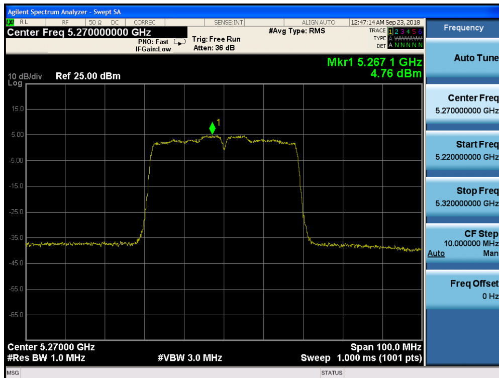
Plot 7-134. Power Spectral Density Plot CDD CORE 1 (40MHz BW 802.11n (UNII Band 2A) – Ch. 54)
