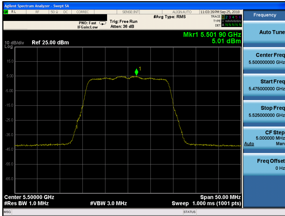
Plot 7-139. Power Spectral Density Plot CDD CORE 0 (20MHz BW 802.11n (UNII Band 2C) – Ch. 100)
