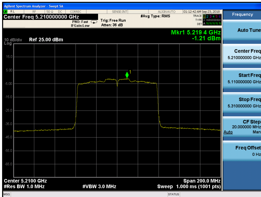
Plot 7-126. Power Spectral Density Plot CDD CORE 1 (80MHz BW 802.11ac (UNII Band 1) – Ch. 42)
