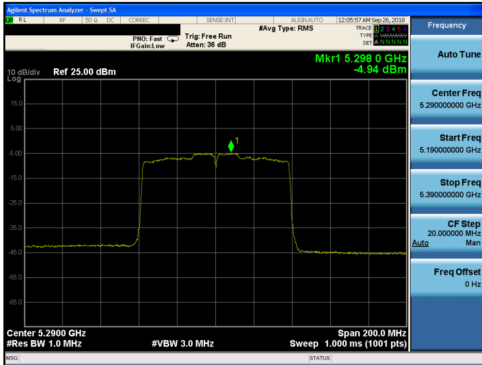
Plot 7-137. Power Spectral Density Plot CDD CORE 0 (80MHz BW 802.11ac (UNII Band 2A) – Ch. 58)
