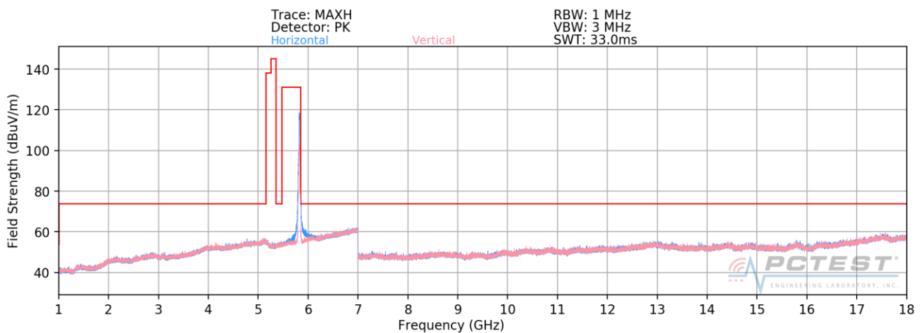
Plot 7-178. Radiated Spurious Plot above 1GHz SISO CORE0 (802.11n – U3 Ch. 165)
