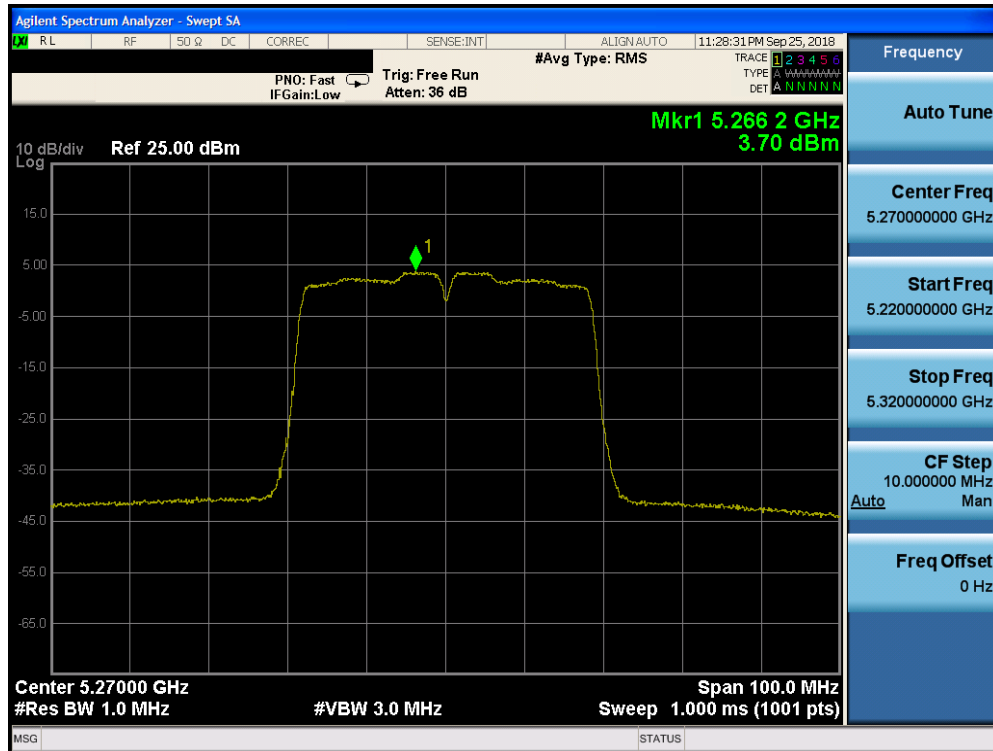
Plot 7-133. Power Spectral Density Plot CDD CORE 0 (40MHz BW 802.11n (UNII Band 2A) – Ch. 54)
