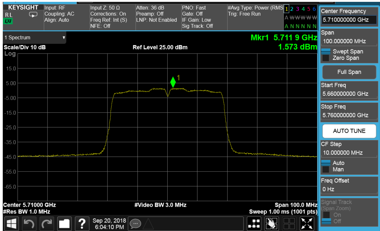
Plot 7-150. Power Spectral Density Plot CDD CORE 1 (40MHz BW 802.11n (UNII Band 2C) – Ch. 142)
