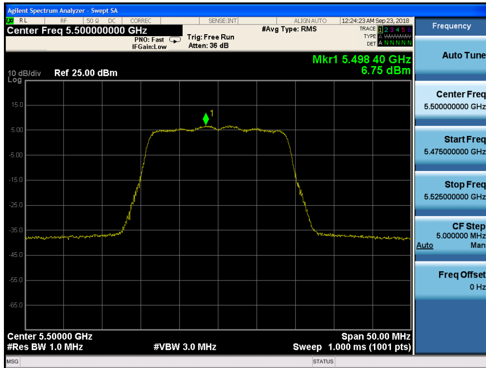
Plot 7-140. Power Spectral Density Plot CDD CORE 1 (20MHz BW 802.11n (UNII Band 2C) – Ch. 100)
