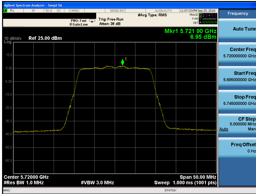
Plot 7-143. Power Spectral Density Plot CDD CORE 0 (20MHz BW 802.11n (UNII Band 2C) – Ch. 144)
