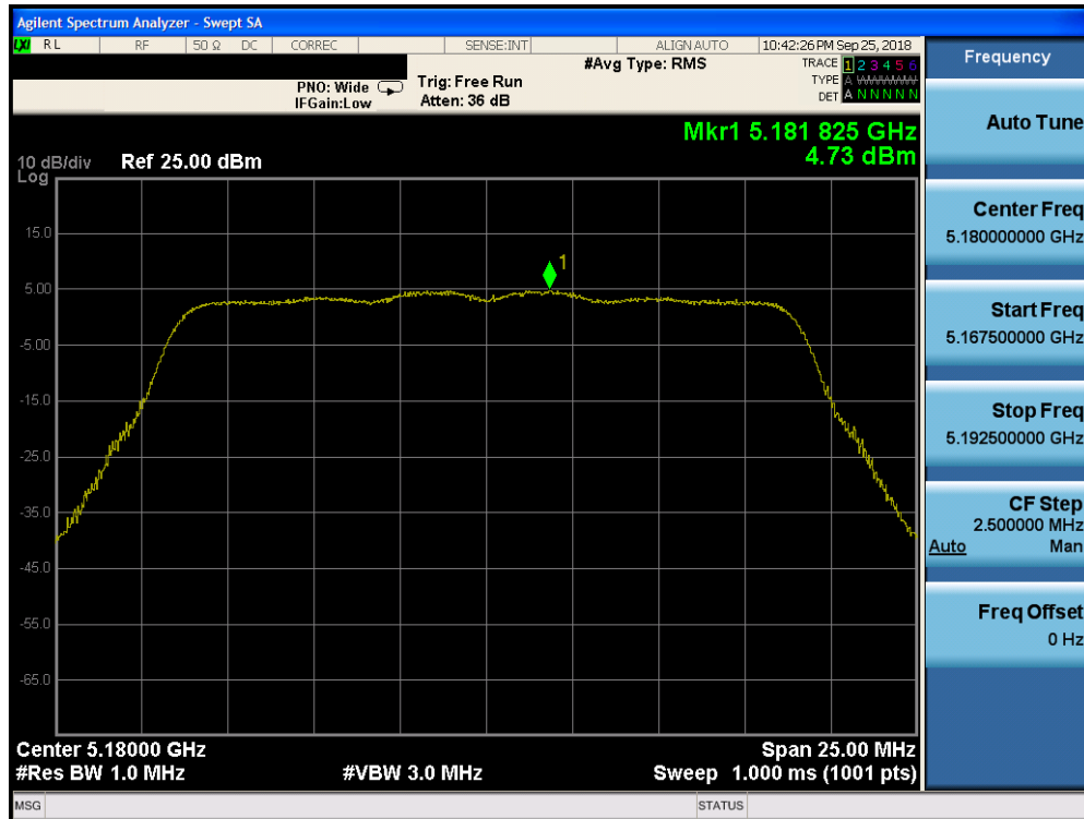
Plot 7-115. Power Spectral Density Plot CDD CORE 0 (20MHz BW 802.11n (UNII Band 1) – Ch. 36)
