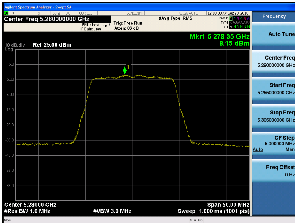
Plot 7-130. Power Spectral Density Plot CDD CORE 1 (20MHz BW 802.11n (UNII Band 2A) – Ch. 56)
