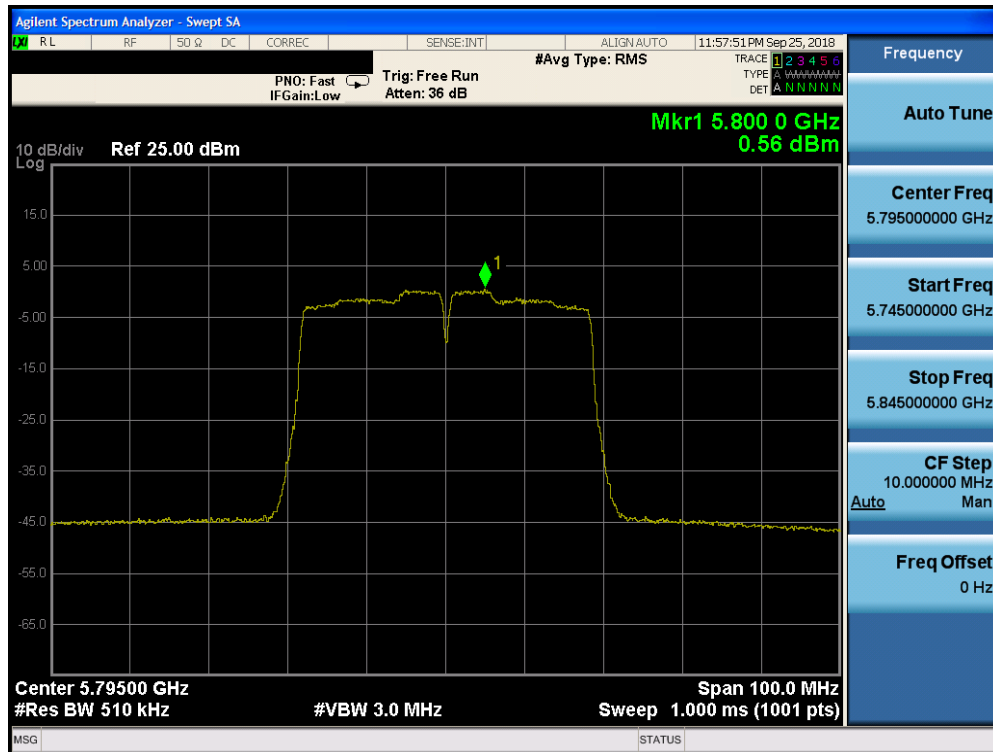
Plot 7-163. Power Spectral Density Plot CDD CORE 0 (40MHz BW 802.11n (UNII Band 3) – Ch. 159)
