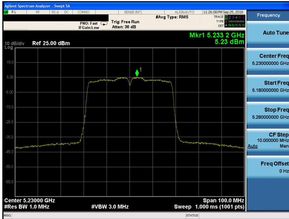
Plot 7-123. Power Spectral Density Plot CDD CORE 0 (40MHz BW 802.11n (UNII Band 1) – Ch. 46)
