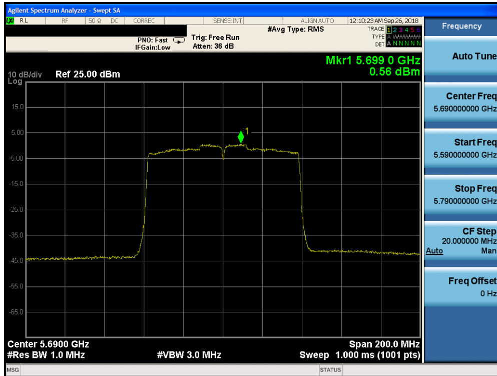
Plot 7-153. Power Spectral Density Plot CDD CORE 0 (80MHz BW 802.11ac (UNII Band 2C) – Ch. 138)
