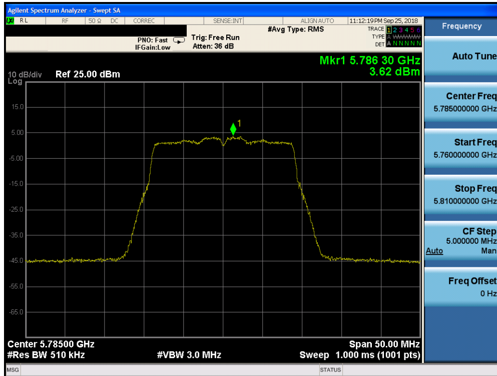
Plot 7-157. Power Spectral Density Plot CDD CORE 0 (20MHz BW 802.11n (UNII Band 3) – Ch. 157)
