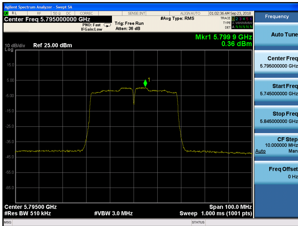
Plot 7-164. Power Spectral Density Plot CDD CORE 1 (40MHz BW 802.11n (UNII Band 3) – Ch. 159)
