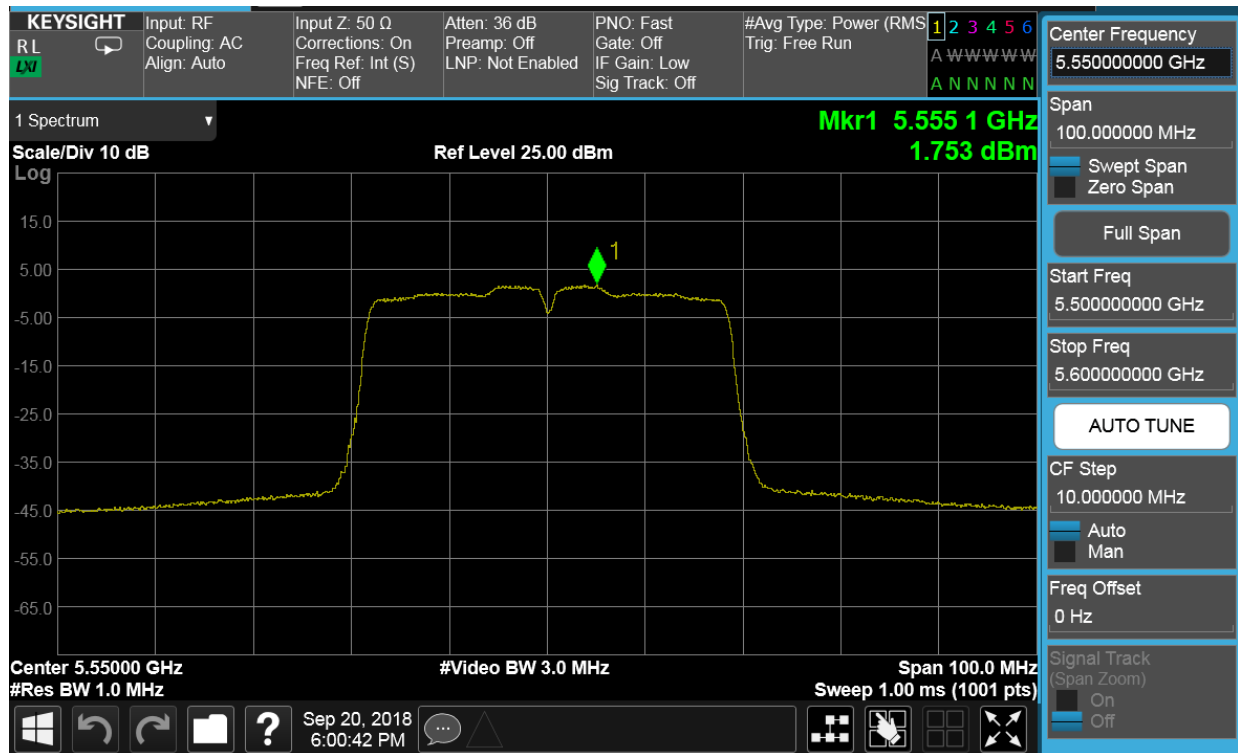
Plot 7-148. Power Spectral Density Plot CDD CORE 1 (40MHz BW 802.11n (UNII Band 2C) – Ch. 110)
