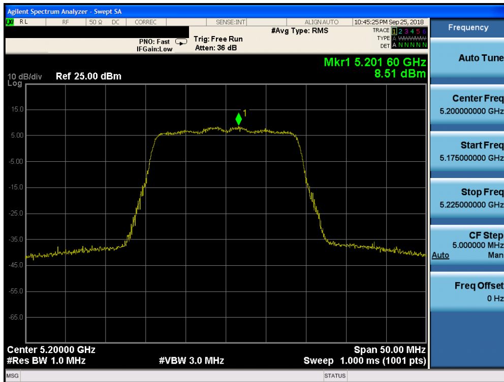
Plot 7-117. Power Spectral Density Plot CDD CORE 0 (20MHz BW 802.11n (UNII Band 1) – Ch. 40)
