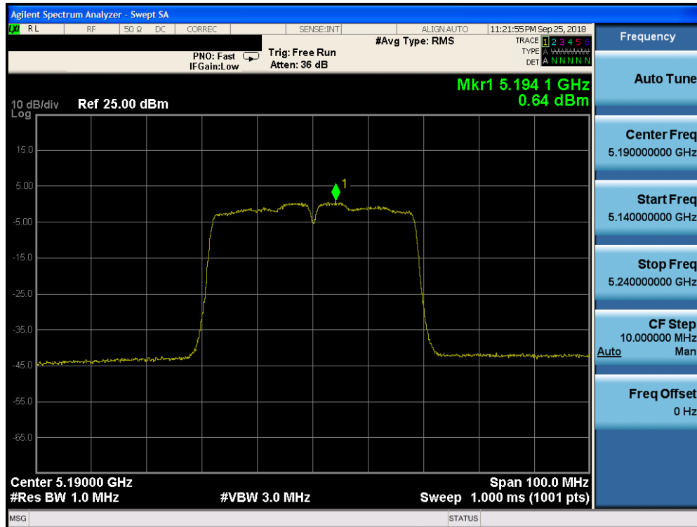
Plot 7-121. Power Spectral Density Plot CDD CORE 0 (40MHz BW 802.11n (UNII Band 1) – Ch. 38)
