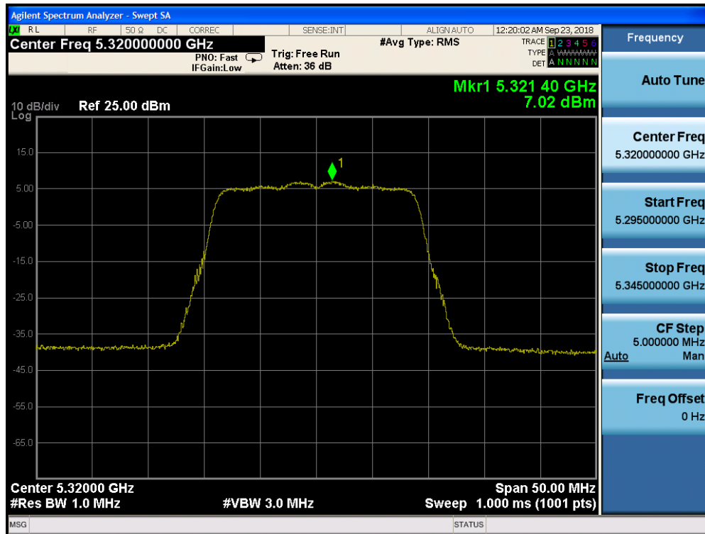
Plot 7-132. Power Spectral Density Plot CDD CORE 1 (20MHz BW 802.11n (UNII Band 2A) – Ch. 64)
