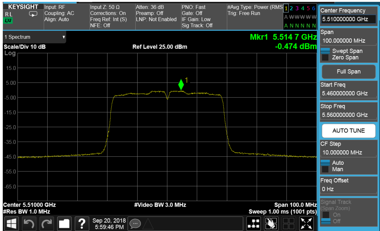
Plot 7-146. Power Spectral Density Plot CDD CORE 1 (40MHz BW 802.11n (UNII Band 2C) – Ch. 102)
