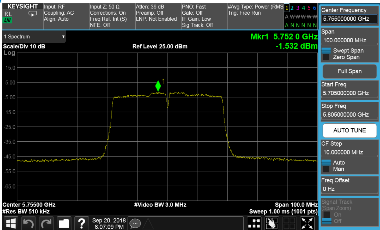
Plot 7-161. Power Spectral Density Plot CDD CORE 0 (40MHz BW 802.11n (UNII Band 3) – Ch. 151)
