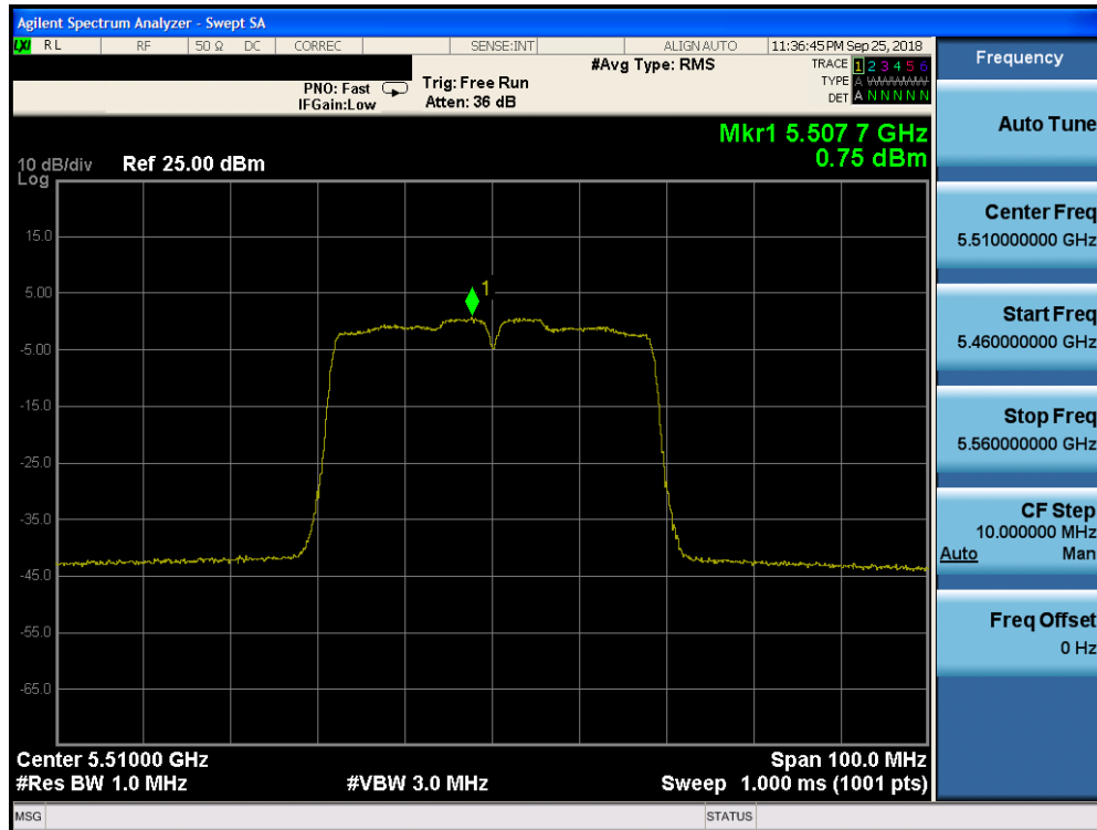
Plot 7-145. Power Spectral Density Plot CDD CORE 0 (40MHz BW 802.11n (UNII Band 2C) – Ch. 102)
