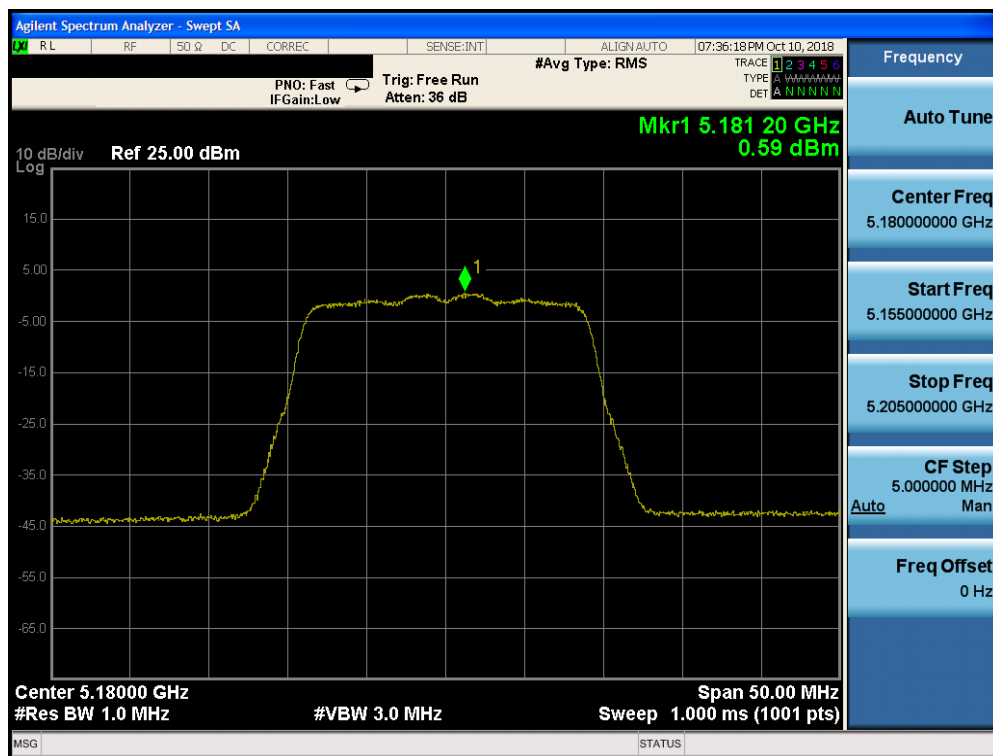
Plot 7-106. Power Spectral Density Plot CDD CORE 1 (20MHz BW 802.11n (UNII Band 1) – Ch. 36) - ISED
