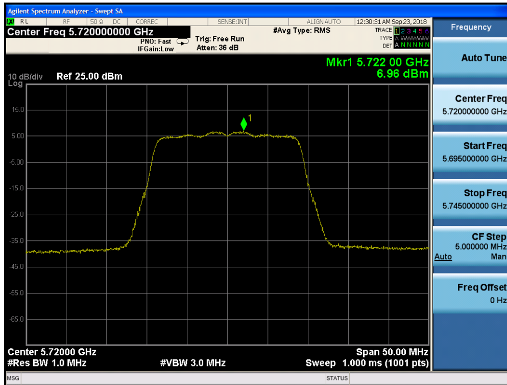
Plot 7-144. Power Spectral Density Plot CDD CORE 1 (20MHz BW 802.11n (UNII Band 2C) – Ch. 144)
