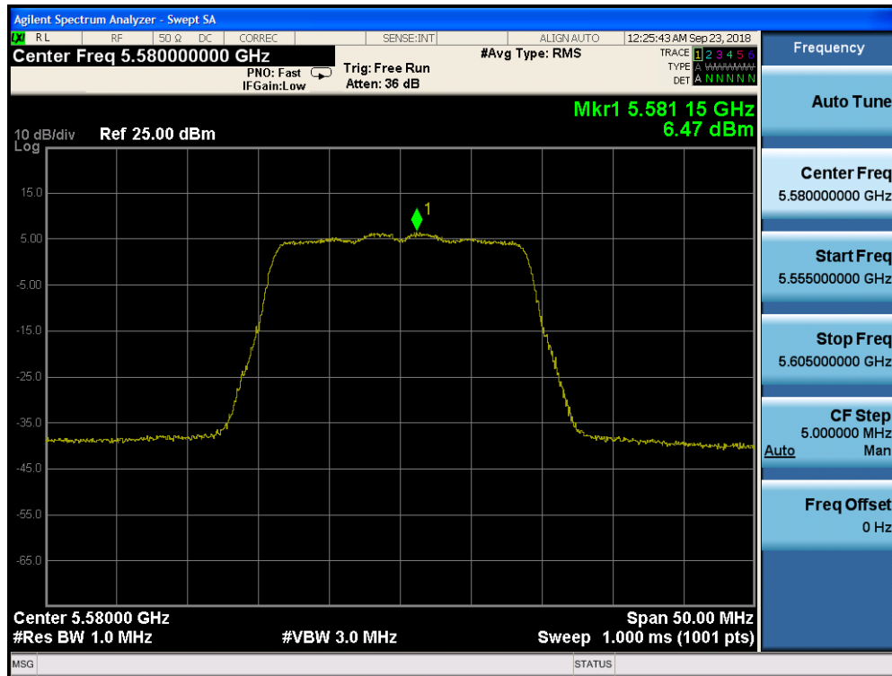
Plot 7-142. Power Spectral Density Plot CDD CORE 1 (20MHz BW 802.11n (UNII Band 2C) – Ch. 116)
