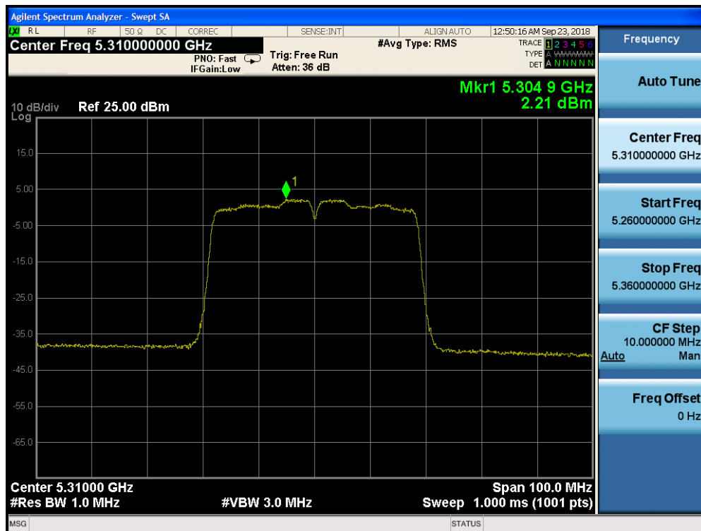
Plot 7-136. Power Spectral Density Plot CDD CORE 1 (40MHz BW 802.11n (UNII Band 2A) – Ch. 62)
