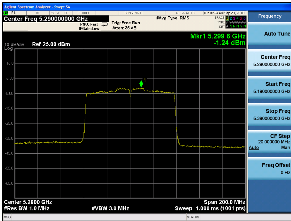
Plot 7-138. Power Spectral Density Plot CDD CORE 1 (80MHz BW 802.11ac (UNII Band 2A) – Ch. 58)
