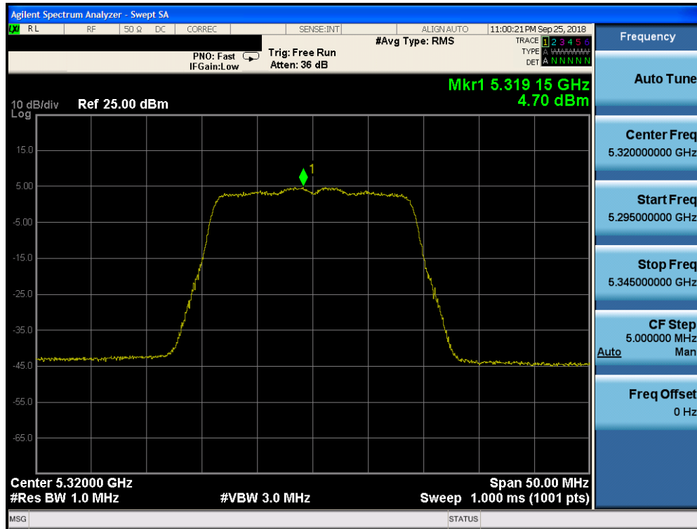
Plot 7-131. Power Spectral Density Plot CDD CORE 0 (20MHz BW 802.11n (UNII Band 2A) – Ch. 64)
