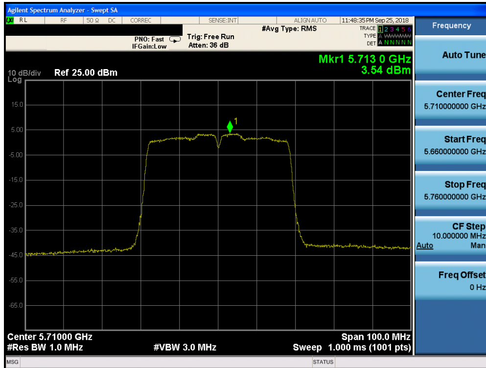
Plot 7-149. Power Spectral Density Plot CDD CORE 0 (40MHz BW 802.11n (UNII Band 2C) – Ch. 142)
