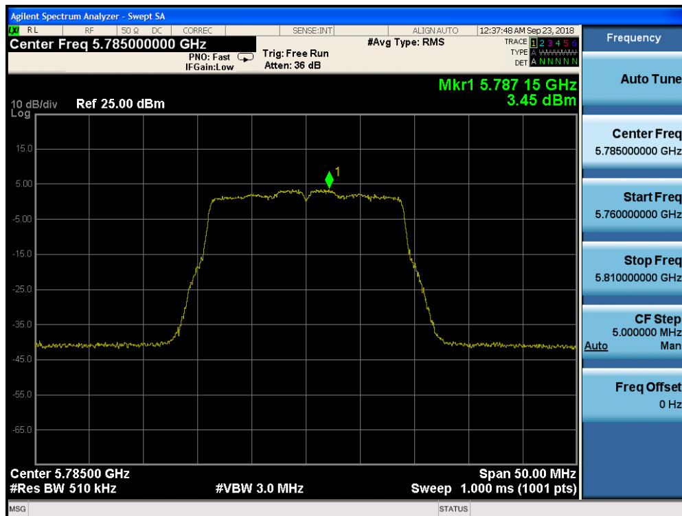
Plot 7-158. Power Spectral Density Plot CDD CORE 1 (20MHz BW 802.11n (UNII Band 3) – Ch. 157)
