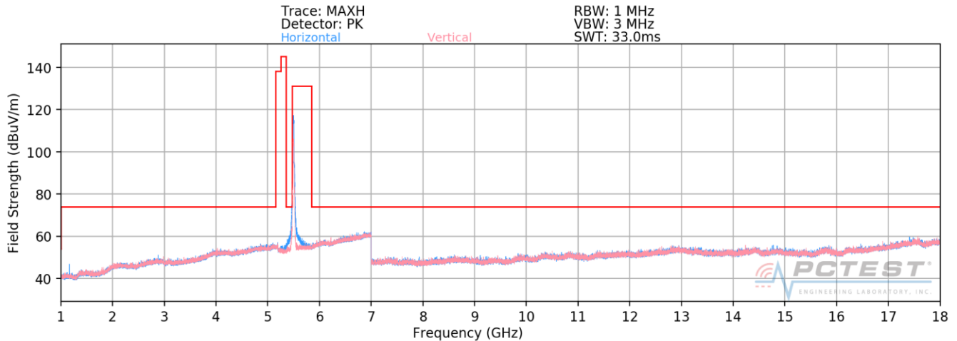
Plot 7-173. Radiated Spurious Plot above 1GHz SISO CORE0 (802.11n – U2C Ch. 100)
