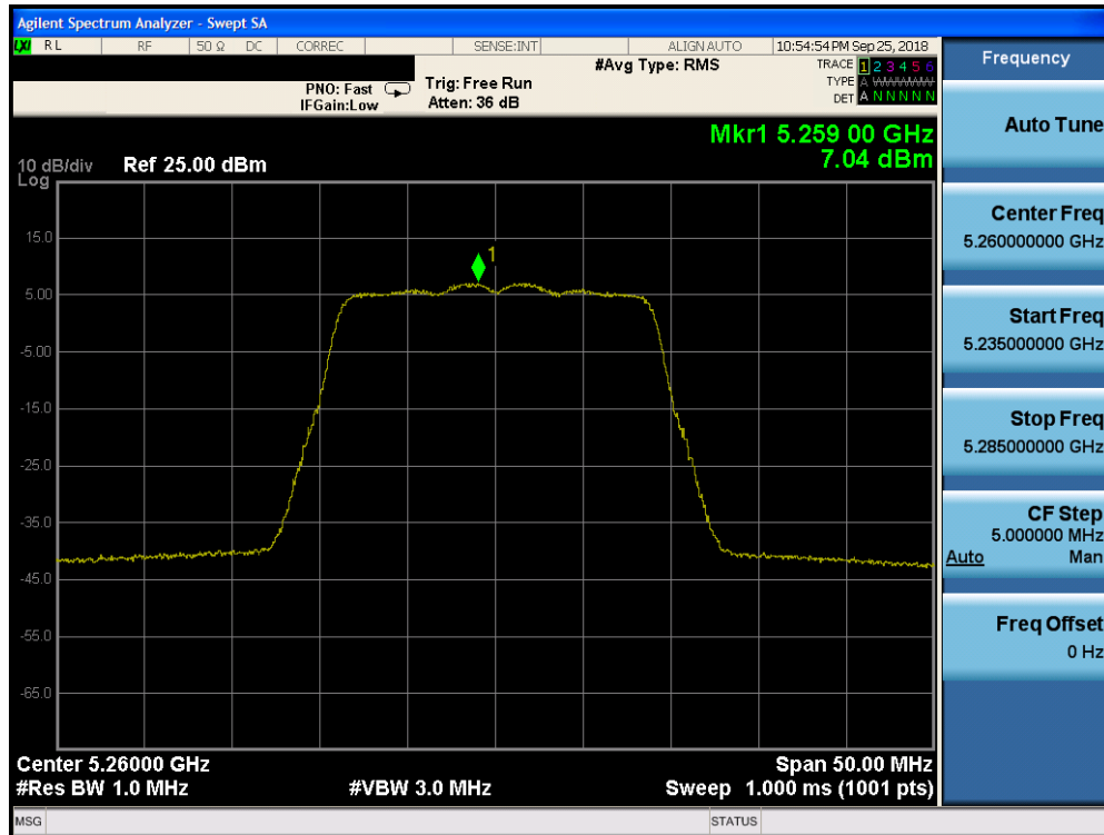
Plot 7-127. Power Spectral Density Plot CDD CORE 0 (20MHz BW 802.11n (UNII Band 2A) – Ch. 52)
