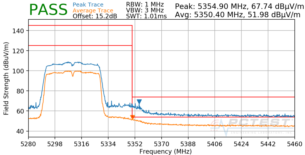
Plot 7-225. Radiated Upper Band Edge Plot SISO CORE0 (UNII Band 2A)
