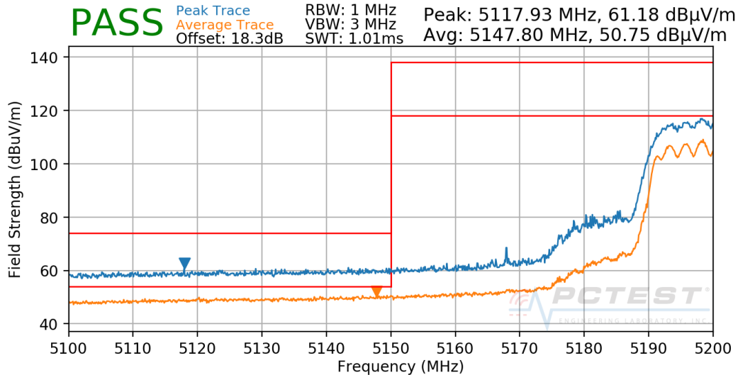
Plot 7-263. Radiated Lower Band Edge Plot CDD (UNII Band 1)
