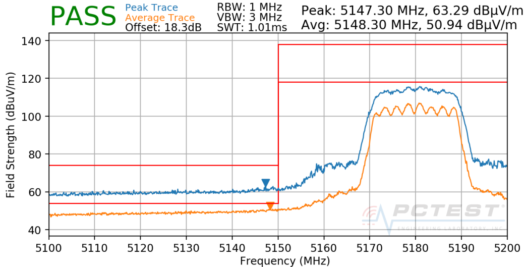
Plot 7-262. Radiated Lower Band Edge Plot CDD (UNII Band 1)
