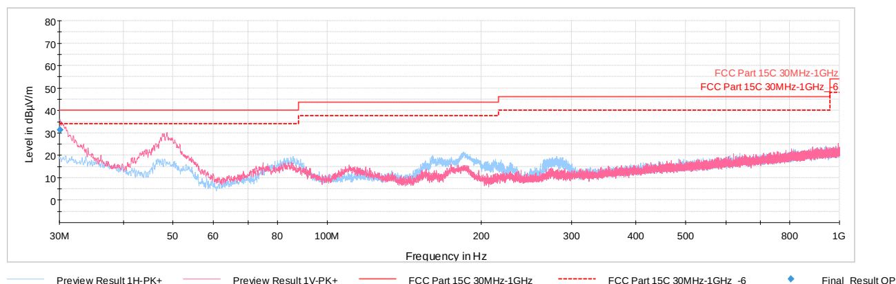
Plot 7-288. Radiated Spurious Plot below 1GHz CDD (802.11n – U3 Ch. 157, w/ AC/DC Charger)
