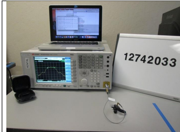
RF CONDUCTED
