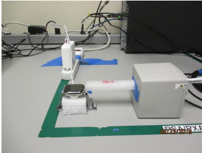
S2, RF EXPOSURE SETUP PHOTO @ 15 cm
