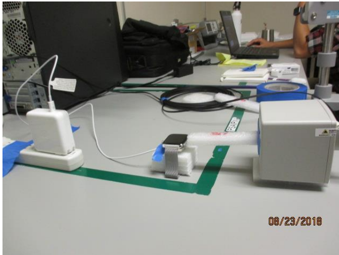
S3, RF EXPOSURE SETUP PHOTO @ 15 cm
