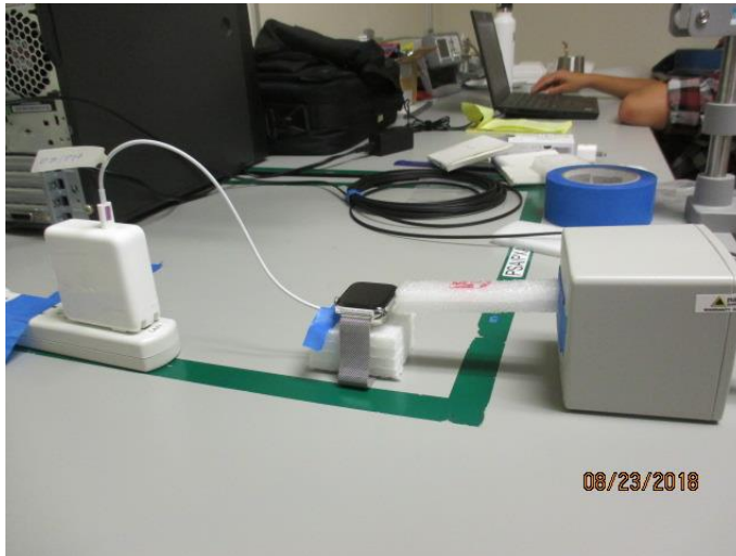
S3, RF EXPOSURE SETUP PHOTO @ 15 cm
