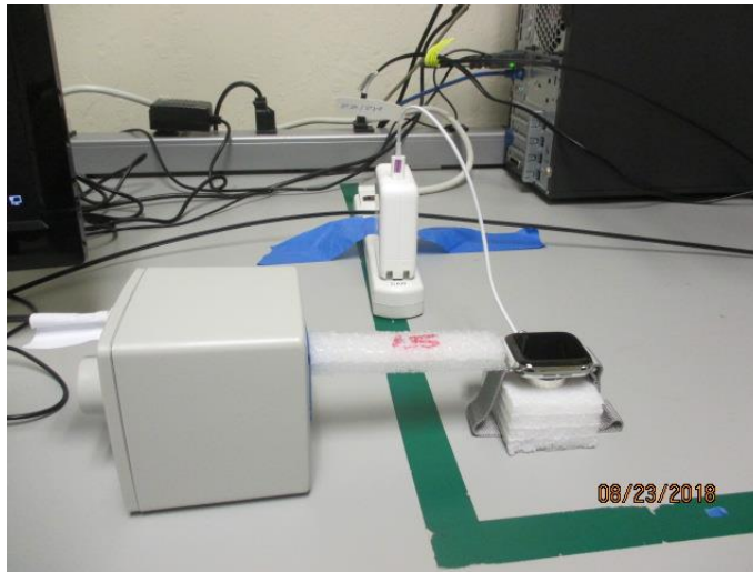
S4, RF EXPOSURE SETUP PHOTO @ 15 cm
