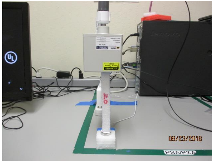
CENTER, RF EXPOSURE SETUP PHOTO @ 15 cm
