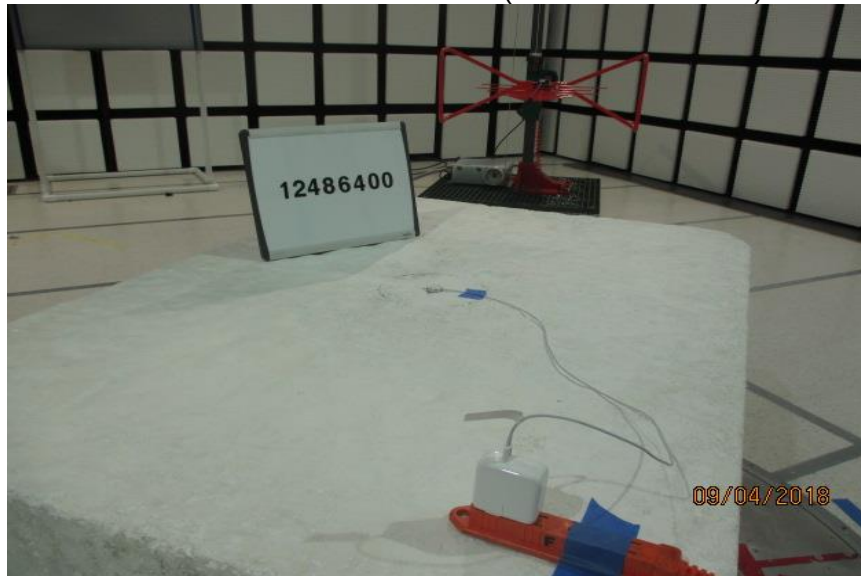
RADIATED EMISSIONS ABOVE 30 MHz (FRONT - STANDBY)
