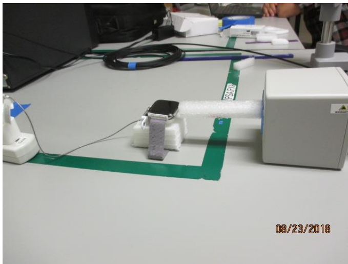
S3, RF EXPOSURE SETUP PHOTO (HORIZONTAL) 15cm
