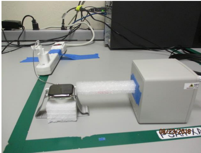
S2, RF EXPOSURE SETUP PHOTO (HORIZONTAL) 15cm
