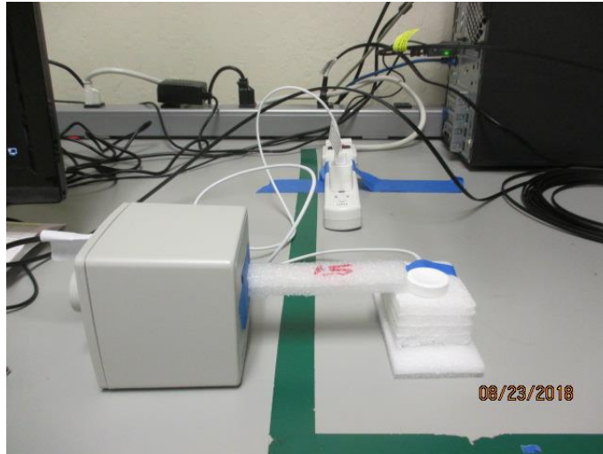
S4, RF EXPOSURE SETUP PHOTO 15cm
