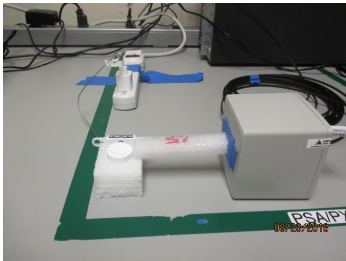
S2, RF EXPOSURE SETUP PHOTO 15cm
