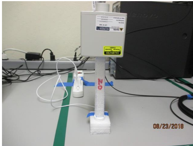
CENTER, RF EXPOSURE SETUP PHOTO 20cm
