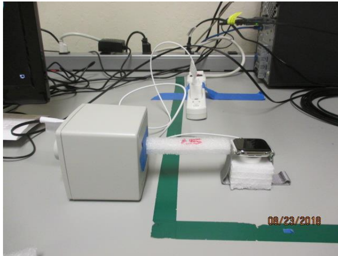
S4, RF EXPOSURE SETUP PHOTO (HORIZONTAL) 15cm
