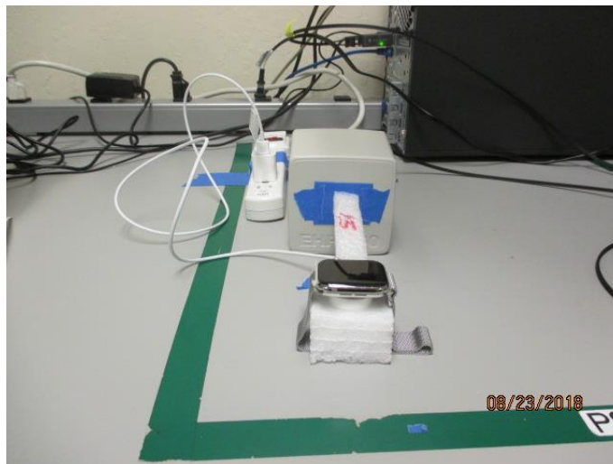
S1, RF EXPOSURE SETUP PHOTO (HORIZONTAL) 15cm
