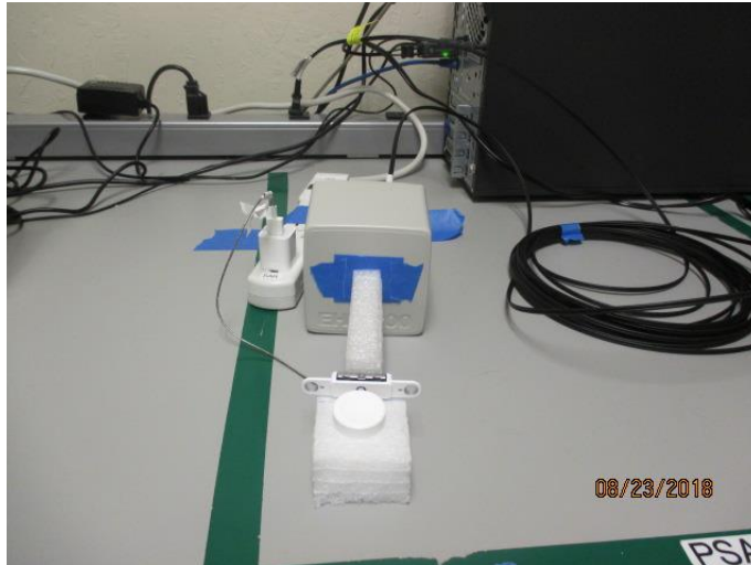
S1, RF EXPOSURE SETUP PHOTO 15cm
