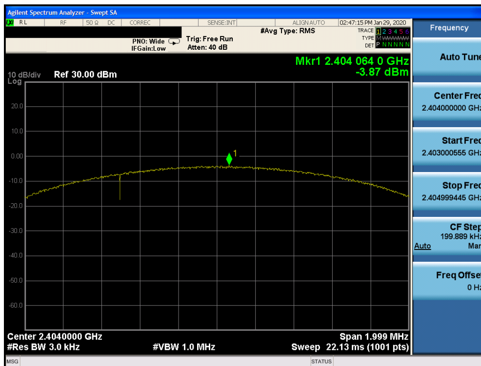
Plot 7-31. Power Spectral Density Plot Ant 2a (Bluetooth (LE), 2Mbps, ePA – Ch. 1)
