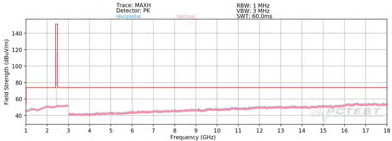
Plot 7-85. Radiated Spurious Plot Above 1GHz Ant 2a (1Mbps, ePA – Ch. 19)
