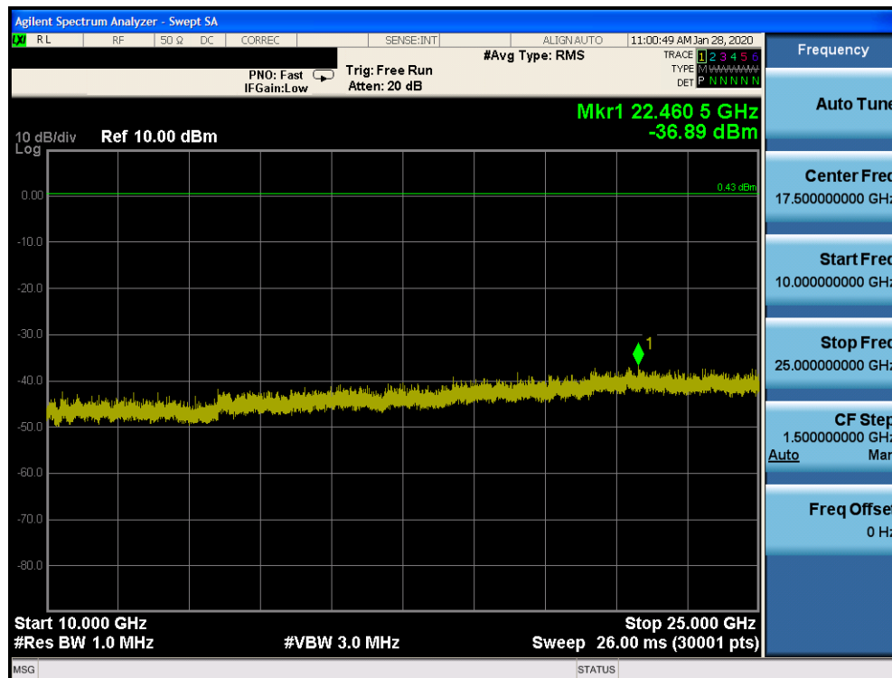
Plot 7-70. Conducted Spurious Plot Ant 4a (Bluetooth (LE), 1Mbps, ePA – Ch. 0)
