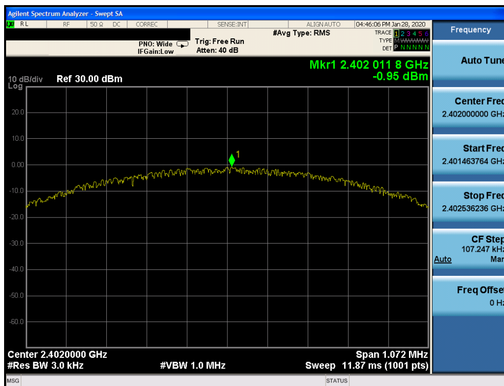
Plot 7-28. Power Spectral Density Plot Ant 2a (Bluetooth (LE), 1Mbps, iPA – Ch. 0)
