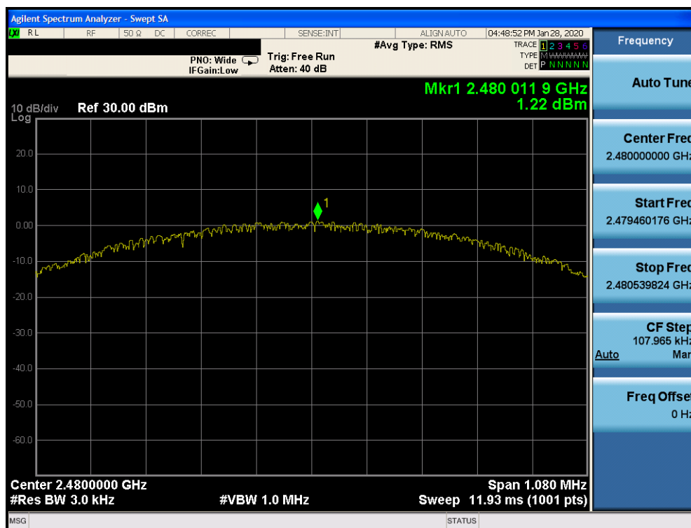
Plot 7-42. Power Spectral Density Plot TxBF Ant 2a (Bluetooth (LE), 1Mbps, ePA – Ch. 39)
