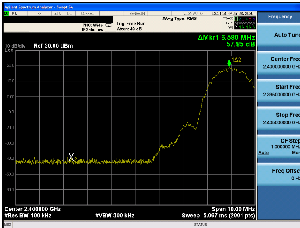
Plot 7-63. Band Edge Plot Ant 4a (Bluetooth (LE), 2Mbps ePA – Ch. 1)
