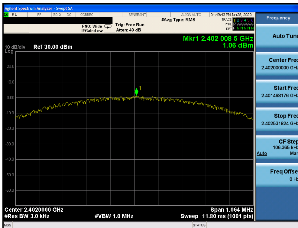
Plot 7-38. Power Spectral Density Plot TxBF Ant 2a (Bluetooth (LE), 1Mbps, ePA – Ch. 0)
