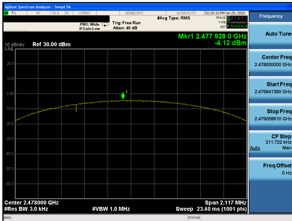
Plot 7-24. Power Spectral Density Plot Ant 4a (Bluetooth (LE), 2Mbps, iPA – Ch. 38)
