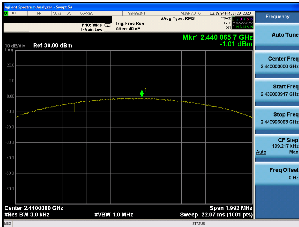
Plot 7-20. Power Spectral Density Plot Ant 4a (Bluetooth (LE), 2Mbps, ePA – Ch. 19)
