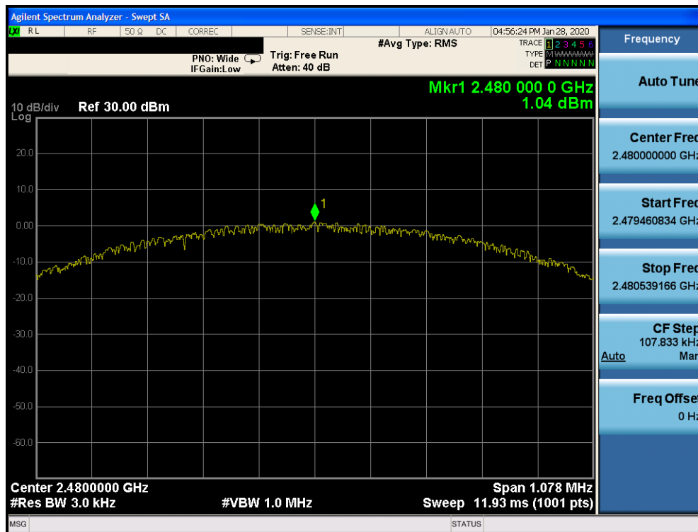
Plot 7-47. Power Spectral Density Plot TxBF Ant 4a (Bluetooth (LE), 1Mbps, iPA – Ch. 39)
