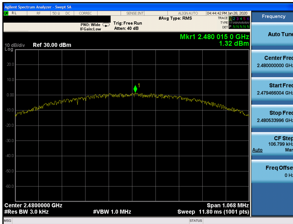
Plot 7-27. Power Spectral Density Plot Ant 2a (Bluetooth (LE), 1Mbps, ePA – Ch. 39)
