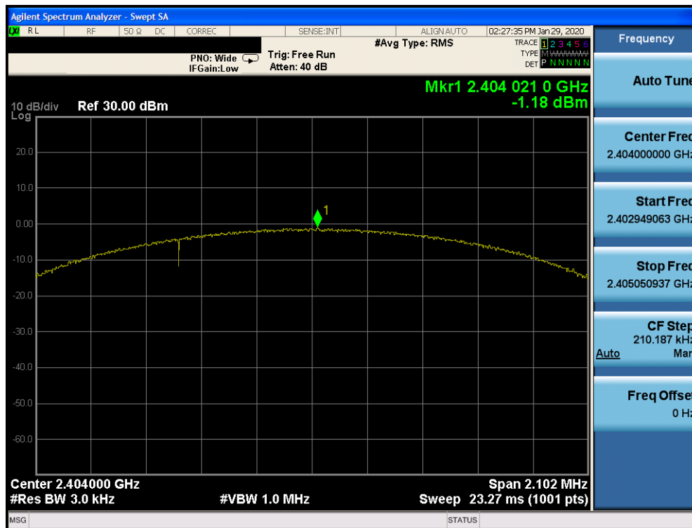
Plot 7-49. Power Spectral Density Plot TxBF Ant 4a (Bluetooth (LE), 2Mbps, ePA – Ch. 1)
