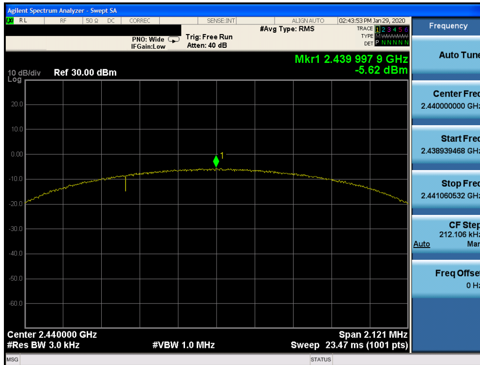
Plot 7-35. Power Spectral Density Plot Ant 2a (Bluetooth (LE), 2Mbps, iPA – Ch. 19)
