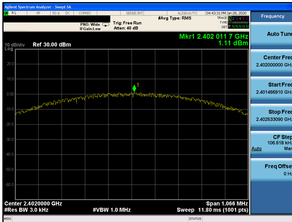
Plot 7-25. Power Spectral Density Plot Ant 2a (Bluetooth (LE), 1Mbps, ePA – Ch. 0)
