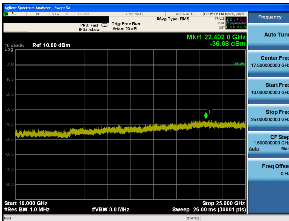
Plot 7-78. Conducted Spurious Plot Ant 2a (Bluetooth (LE), 1Mbps, ePA – Ch. 19)
