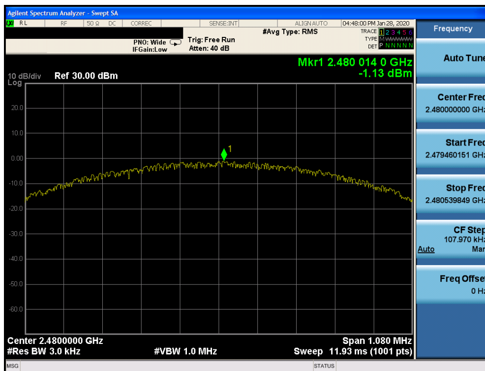
Plot 7-48. Power Spectral Density Plot TxBF Ant 2a (Bluetooth (LE), 1Mbps, iPA – Ch. 39)
