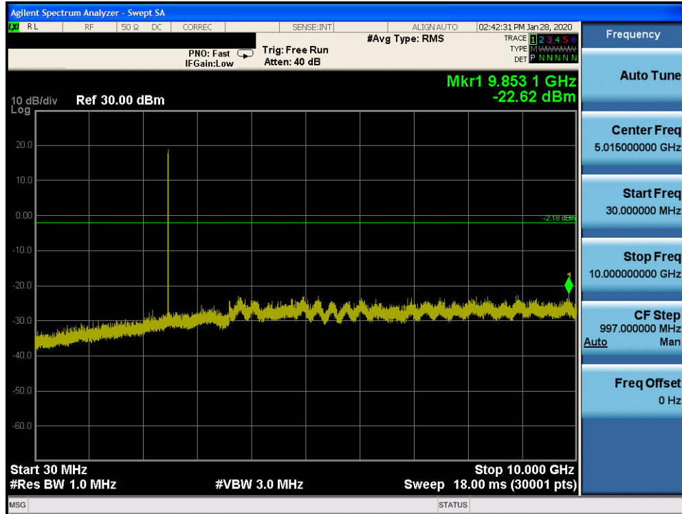
Plot 7-79. Conducted Spurious Plot Ant 2a (Bluetooth (LE), 1Mbps, ePA – Ch. 39)
