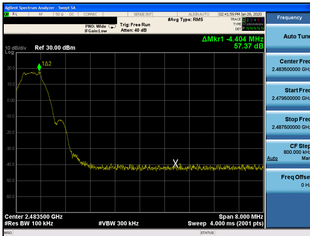
Plot 7-66. Band Edge Plot Ant 2a (Bluetooth (LE), 1Mbps ePA – Ch. 39)
