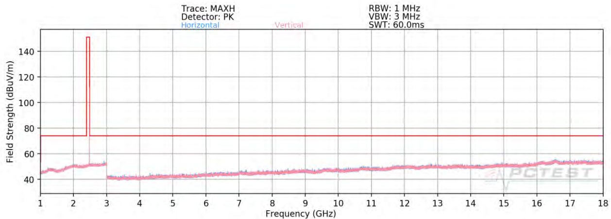
Plot 7-86. Radiated Spurious Plot Above 1GHz Ant 2a (1Mbps, ePA – Ch. 39)
