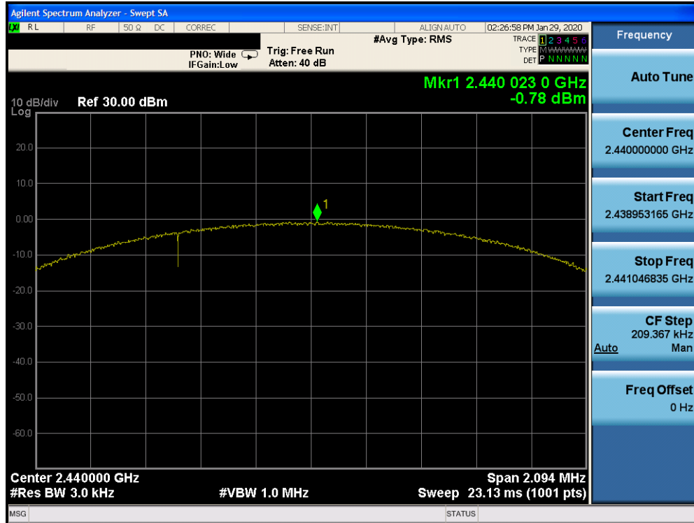
Plot 7-51. Power Spectral Density Plot TxBF Ant 4a (Bluetooth (LE), 2Mbps, ePA – Ch. 19)
