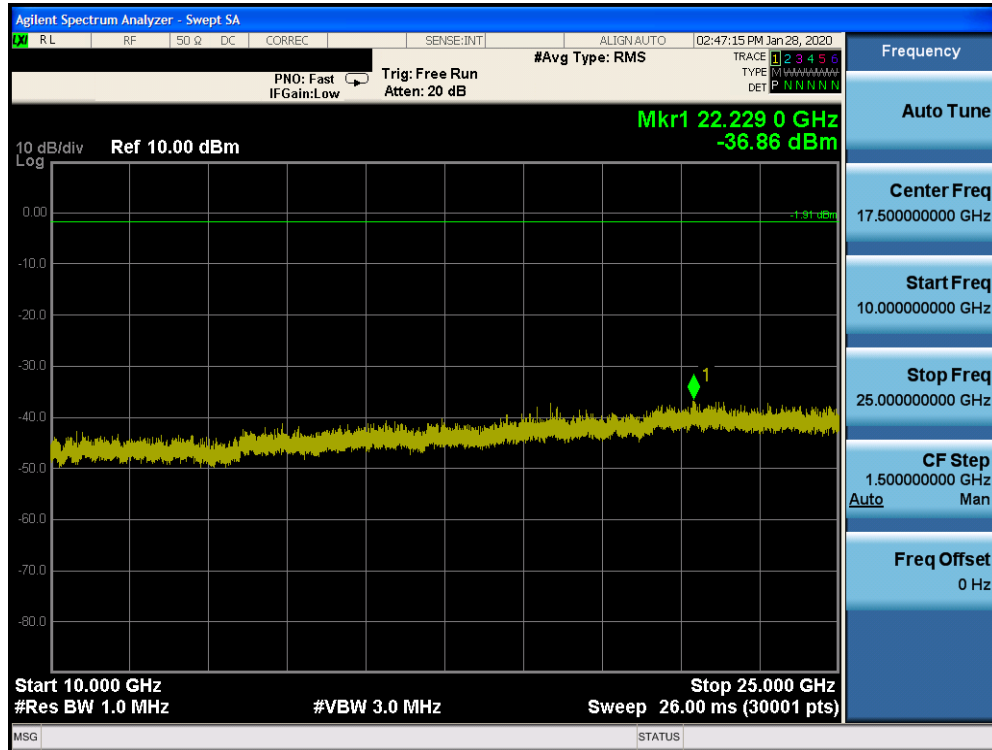
Plot 7-76. Conducted Spurious Plot Ant 2a (Bluetooth (LE), 1Mbps, ePA – Ch. 0)
