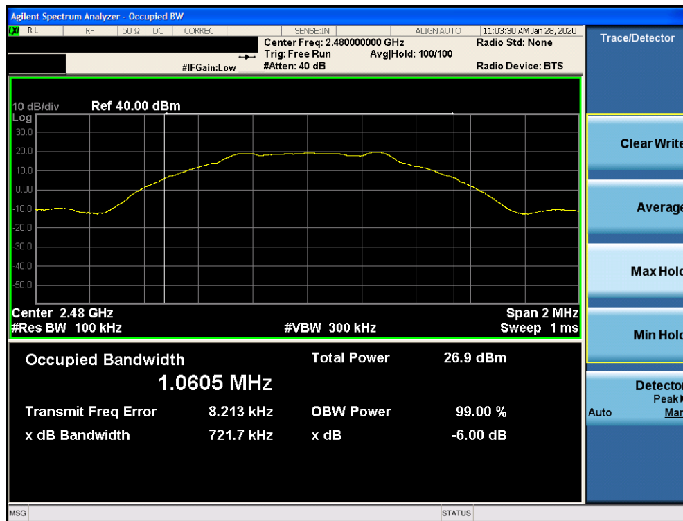
Plot 7-3. 6dB Bandwidth Plot Ant 4a (Bluetooth (LE), 1Mbps, ePA – Ch. 39)
