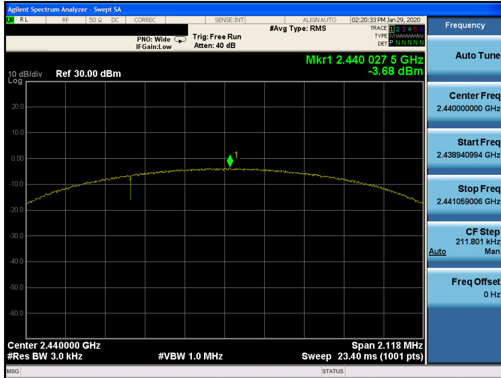
Plot 7-23. Power Spectral Density Plot Ant 4a (Bluetooth (LE), 2Mbps, iPA – Ch. 19)
