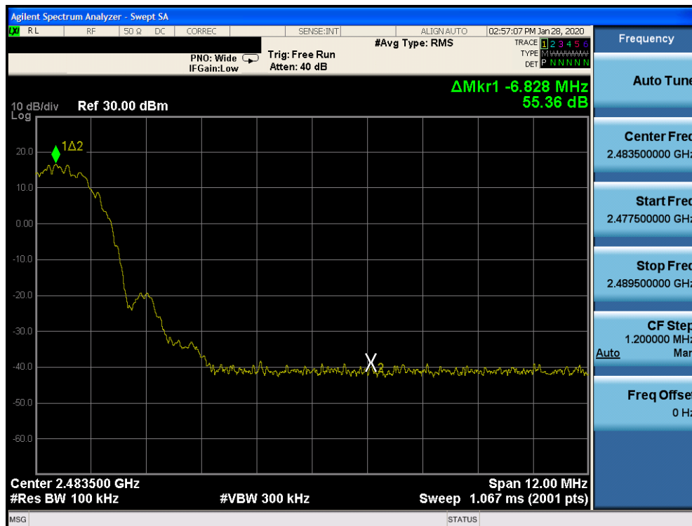
Plot 7-68. Band Edge Plot Ant 2a (Bluetooth (LE), 2Mbps ePA – Ch. 38)
