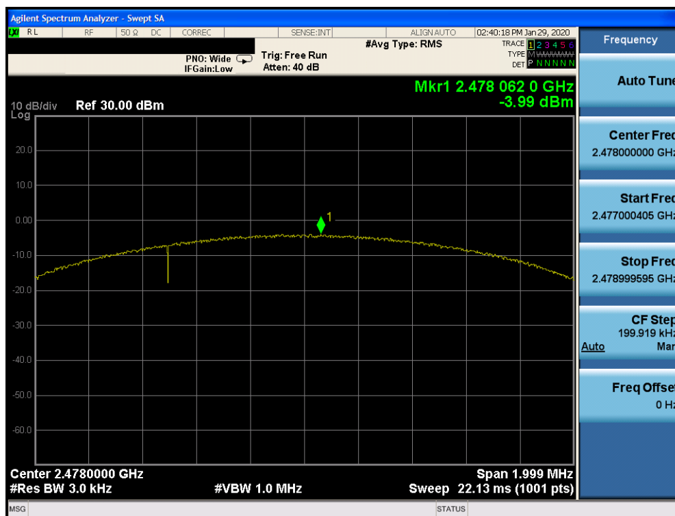
Plot 7-54. Power Spectral Density Plot TxBF Ant 2a (Bluetooth (LE), 2Mbps, ePA – Ch. 38)
