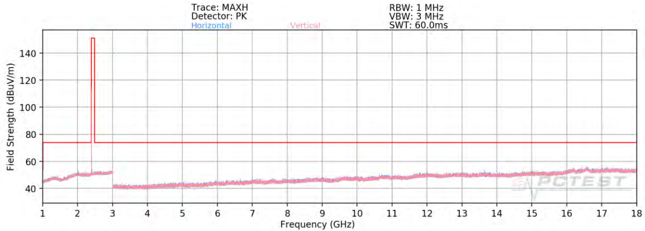
Plot 7-84. Radiated Spurious Plot Above 1GHz Ant 2a (1Mbps, ePA – Ch. 0)
