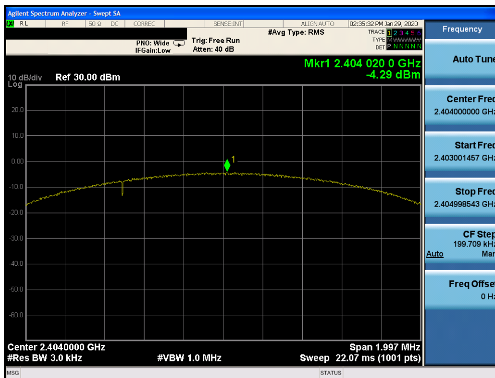
Plot 7-50. Power Spectral Density Plot TxBF Ant 2a (Bluetooth (LE), 2Mbps, ePA – Ch. 1)
