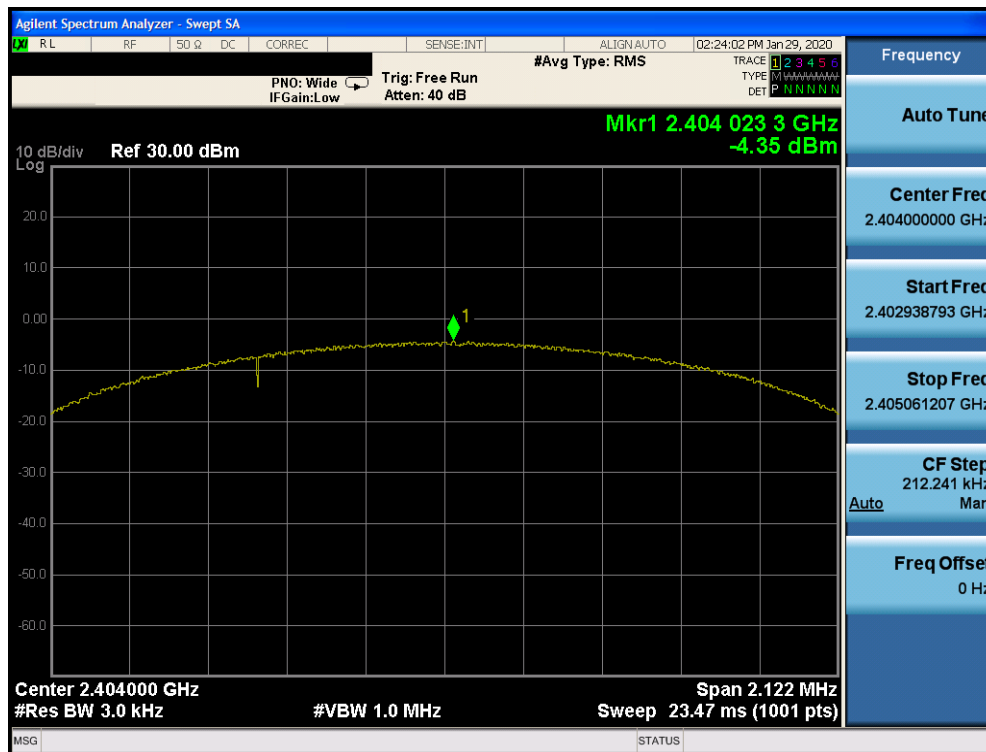
Plot 7-55. Power Spectral Density Plot TxBF Ant 4a (Bluetooth (LE), 2Mbps, iPA – Ch. 1)
