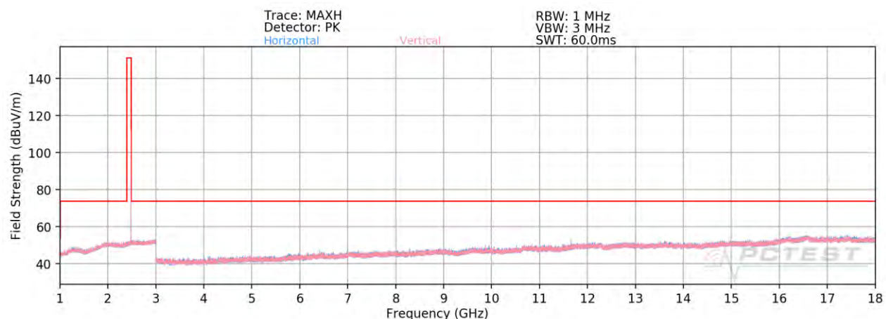
Plot 7-83. Radiated Spurious Plot Above 1GHz Ant 4a (1Mbps, ePA – Ch. 39)
