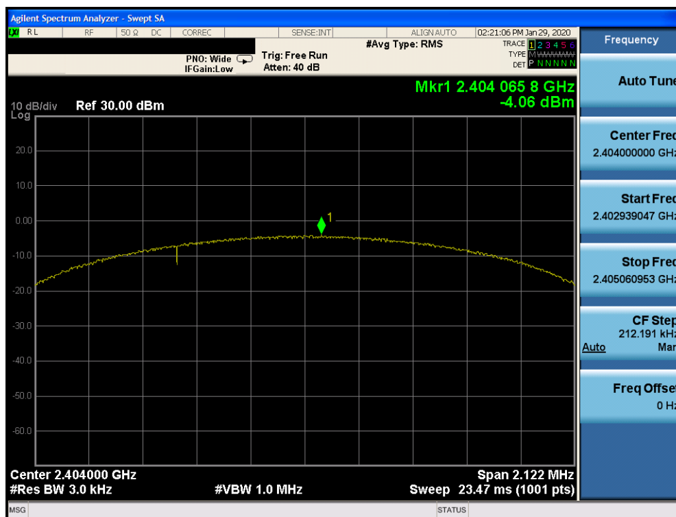
Plot 7-22. Power Spectral Density Plot Ant 4a (Bluetooth (LE), 2Mbps, iPA – Ch. 1)
