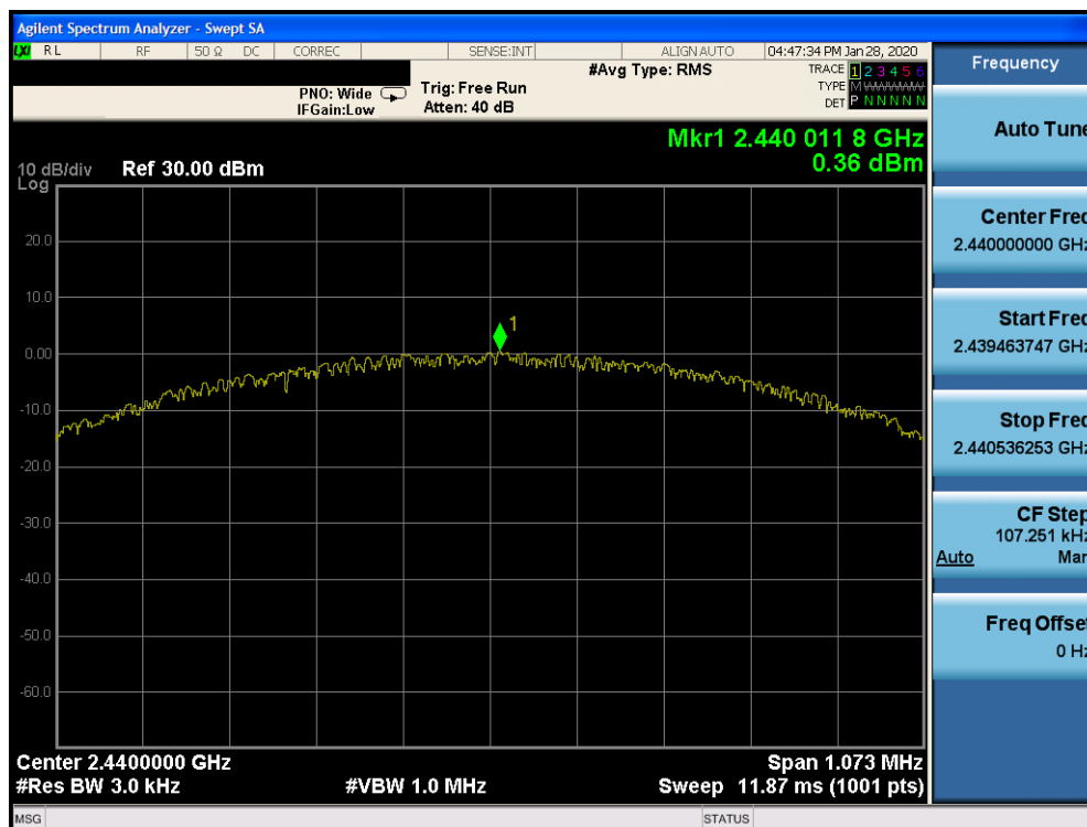
Plot 7-46. Power Spectral Density Plot TxBF Ant 2a (Bluetooth (LE), 1Mbps, iPA – Ch. 19)
