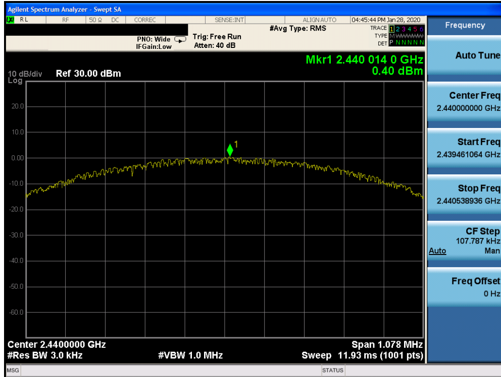
Plot 7-29. Power Spectral Density Plot Ant 2a (Bluetooth (LE), 1Mbps, iPA – Ch. 19)
