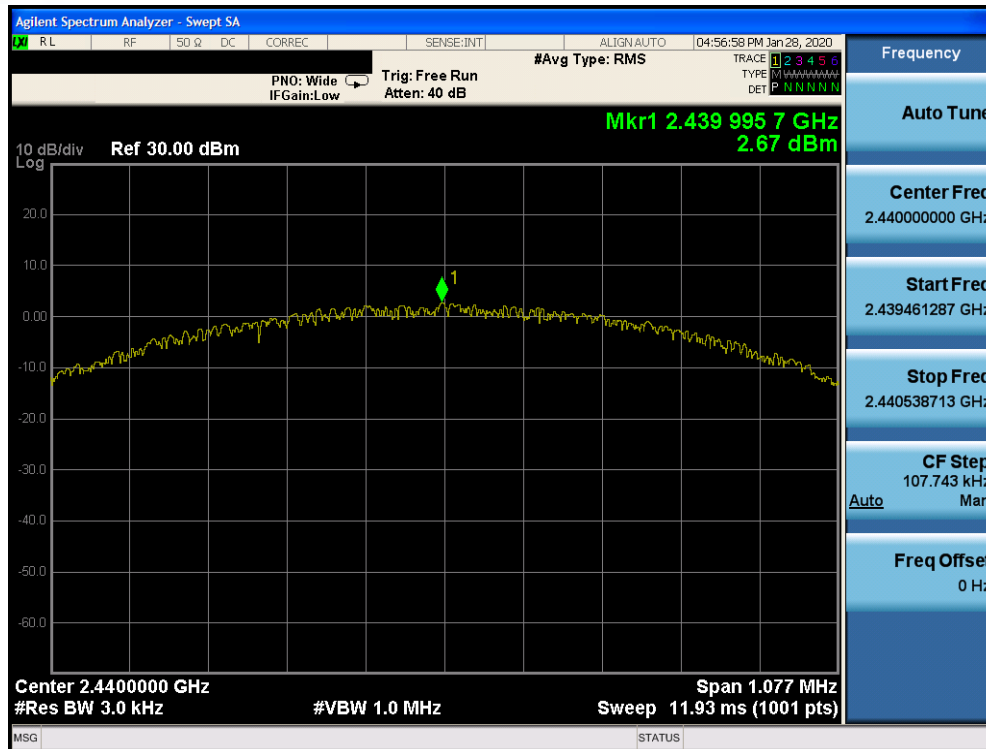
Plot 7-45. Power Spectral Density Plot TxBF Ant 4a (Bluetooth (LE), 1Mbps, iPA – Ch. 19)
