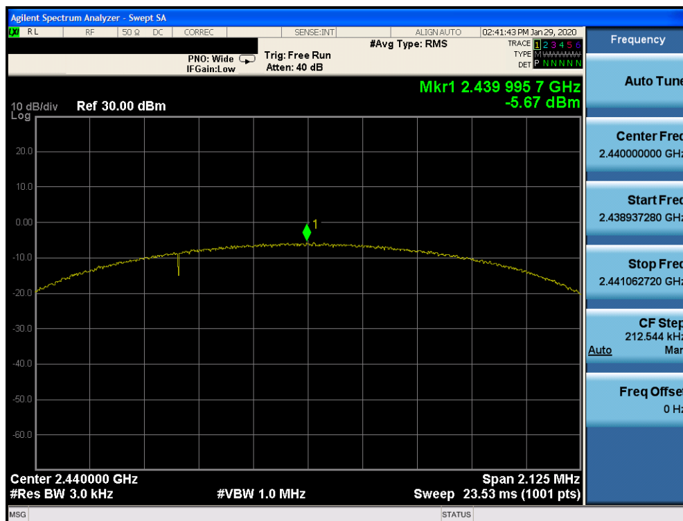
Plot 7-58. Power Spectral Density Plot TxBF Ant 2a (Bluetooth (LE), 2Mbps, iPA – Ch. 19)
