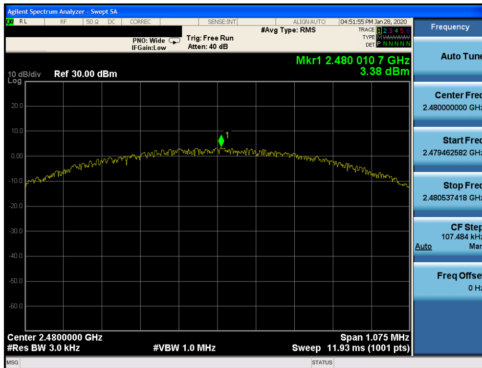
Plot 7-41. Power Spectral Density Plot TxBF Ant 4a (Bluetooth (LE), 1Mbps, ePA – Ch. 39)
