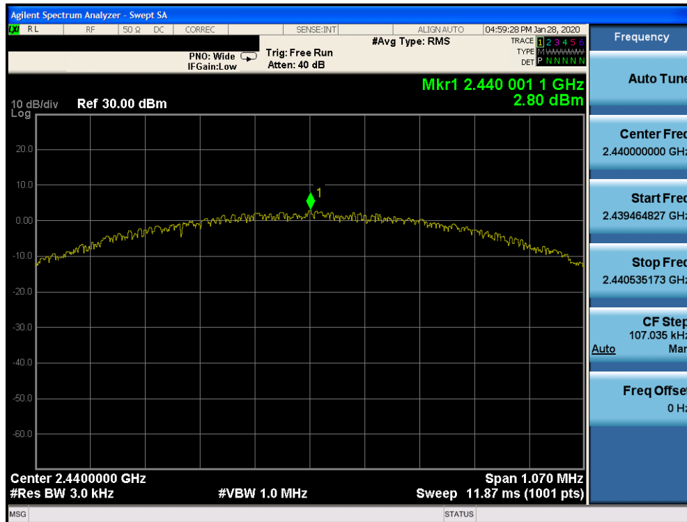
Plot 7-17. Power Spectral Density Plot Ant 4a (Bluetooth (LE), 1Mbps, iPA – Ch. 19)
