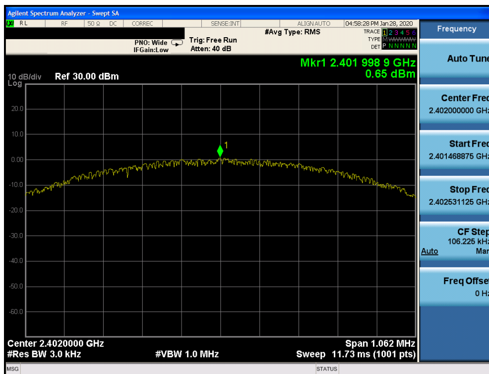
Plot 7-16. Power Spectral Density Plot Ant 4a (Bluetooth (LE), 1Mbps, iPA – Ch. 0)
