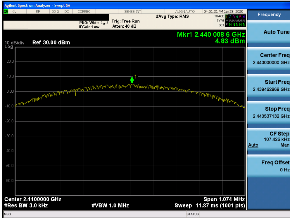
Plot 7-39. Power Spectral Density Plot TxBF Ant 4a (Bluetooth (LE), 1Mbps, ePA – Ch. 19)
