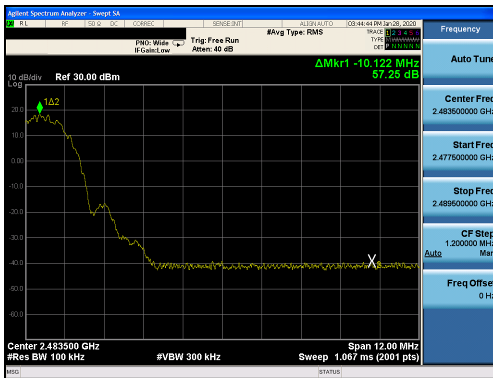
Plot 7-64. Band Edge Plot Ant 4a (Bluetooth (LE), 2Mbps ePA – Ch. 38)
