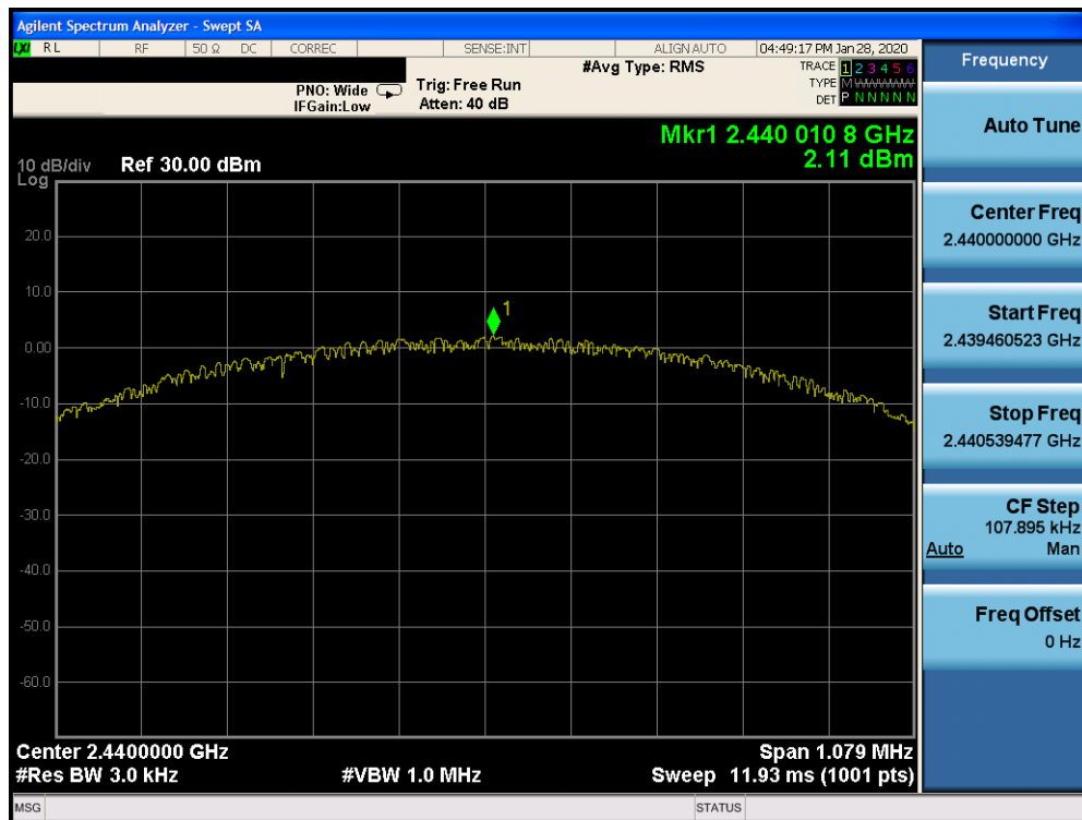
Plot 7-40. Power Spectral Density Plot TxBF Ant 2a (Bluetooth (LE), 1Mbps, ePA – Ch. 19)
