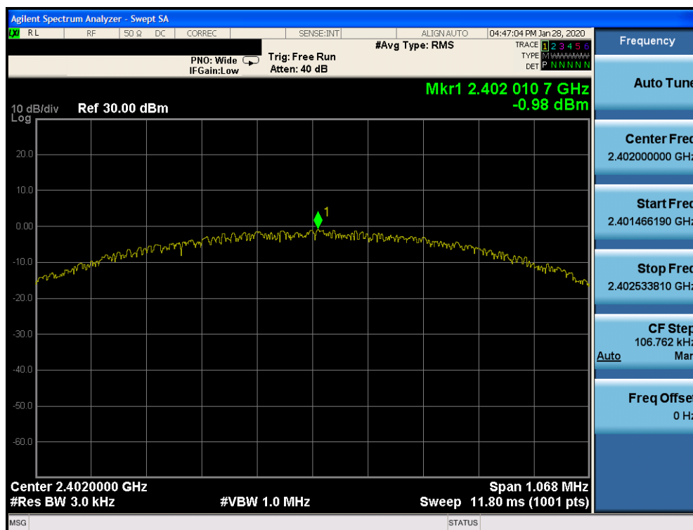
Plot 7-44. Power Spectral Density Plot TxBF Ant 2a (Bluetooth (LE), 1Mbps, iPA – Ch. 0)
