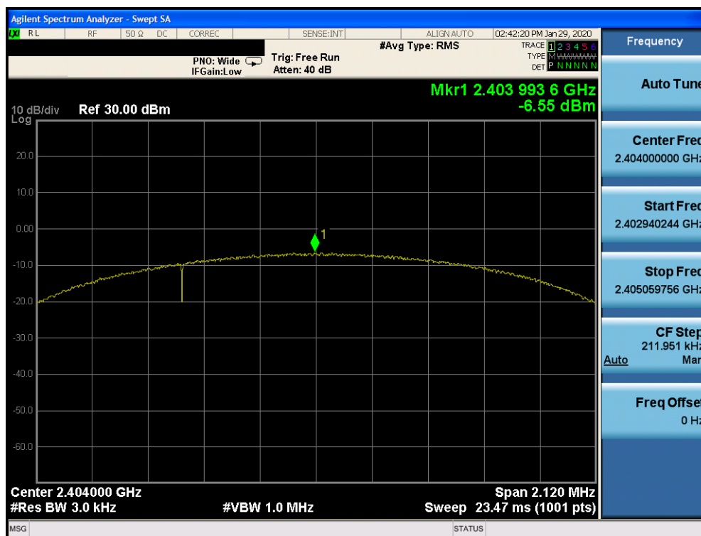
Plot 7-56. Power Spectral Density Plot TxBF Ant 2a (Bluetooth (LE), 2Mbps, iPA – Ch. 1)
