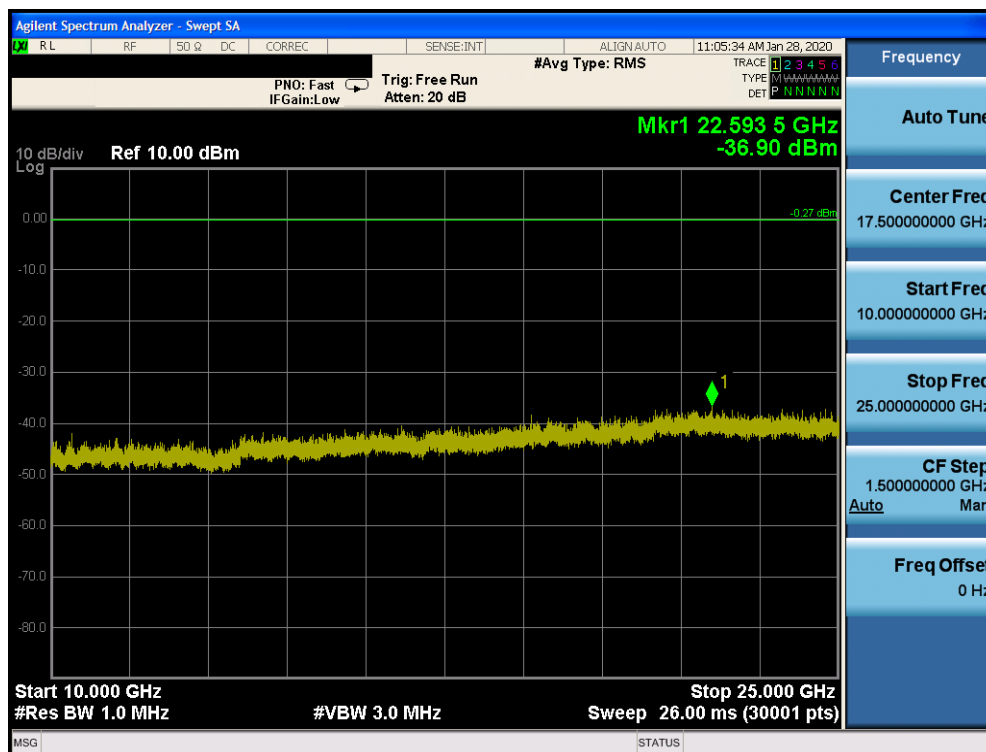
Plot 7-74. Conducted Spurious Plot Ant 4a (Bluetooth (LE), 1Mbps, ePA – Ch. 39)
