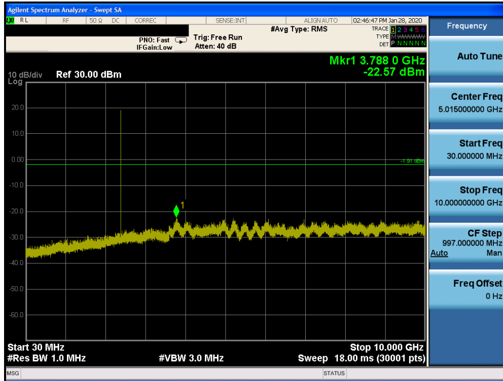
Plot 7-75. Conducted Spurious Plot Ant 2a (Bluetooth (LE), 1Mbps, ePA – Ch. 0)
