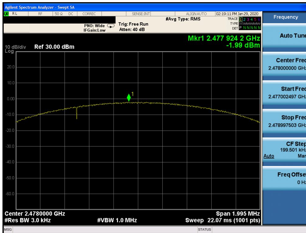
Plot 7-21. Power Spectral Density Plot Ant 4a (Bluetooth (LE), 2Mbps, ePA – Ch. 38)
