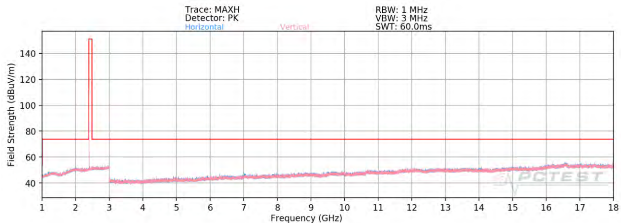
Plot 7-81. Radiated Spurious Plot Above 1GHz Ant 4a (1Mbps, ePA – Ch. 0)
