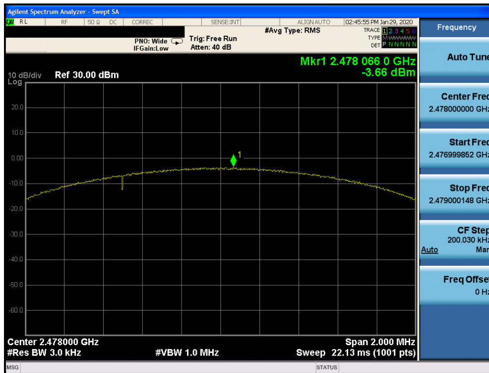
Plot 7-33. Power Spectral Density Plot Ant 2a (Bluetooth (LE), 2Mbps, ePA – Ch. 38)
