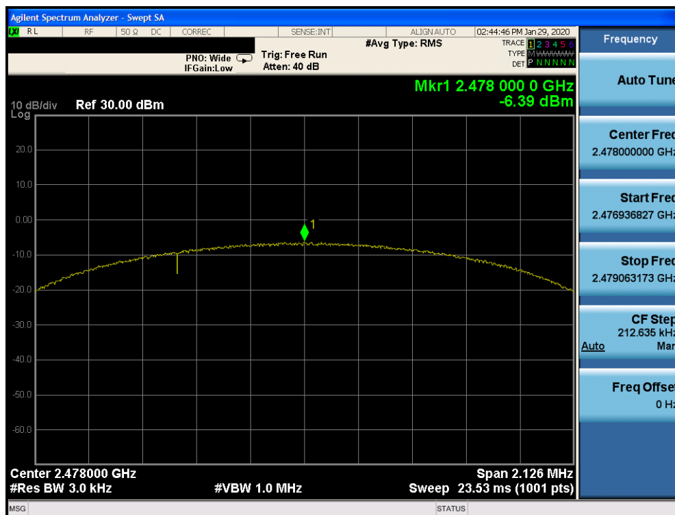
Plot 7-36. Power Spectral Density Plot Ant 2a (Bluetooth (LE), 2Mbps, iPA – Ch. 38)
