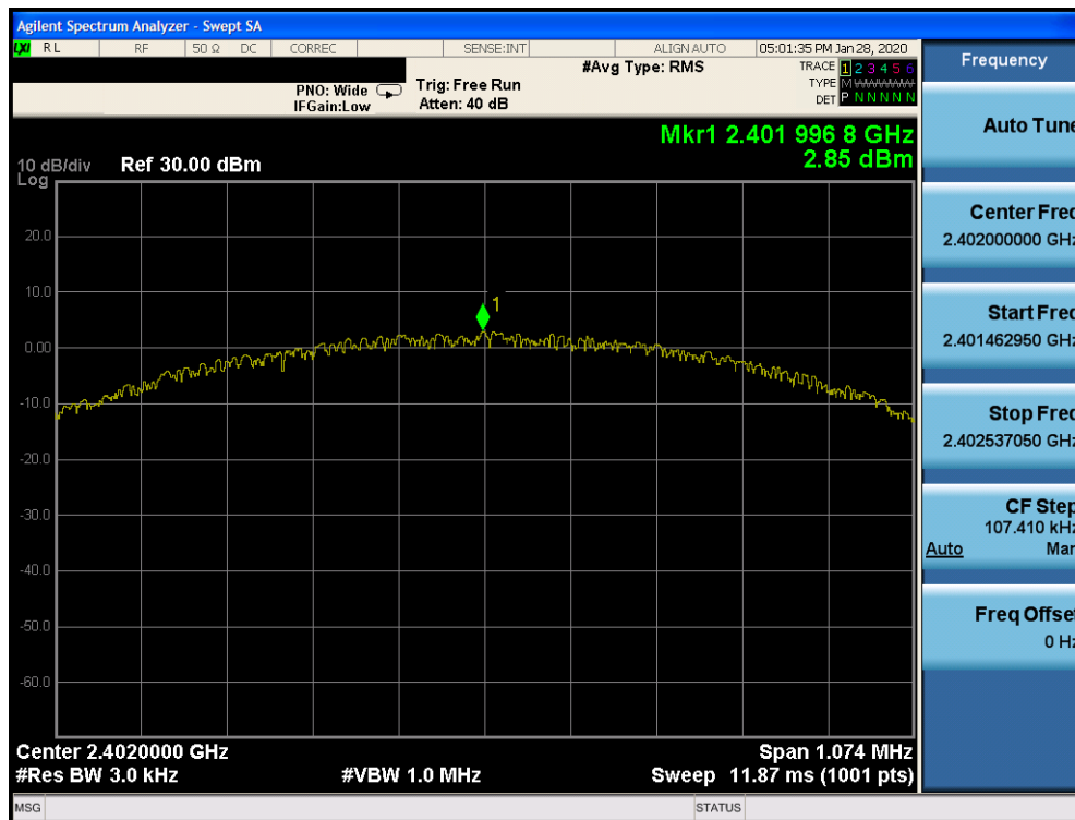
Plot 7-13. Power Spectral Density Plot Ant 4a (Bluetooth (LE), 1Mbps, ePA – Ch. 0)
