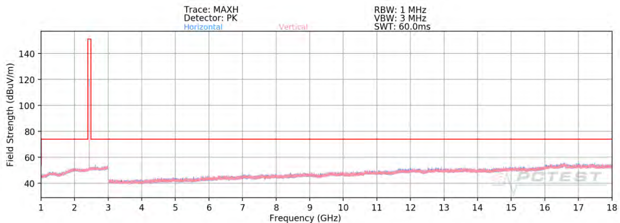
Plot 7-88. Radiated Spurious Plot Above 1GHz TXBF (1Mbps, ePA – Ch. 19)
