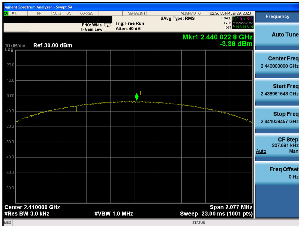
Plot 7-52. Power Spectral Density Plot TxBF Ant 2a (Bluetooth (LE), 2Mbps, ePA – Ch. 19)
