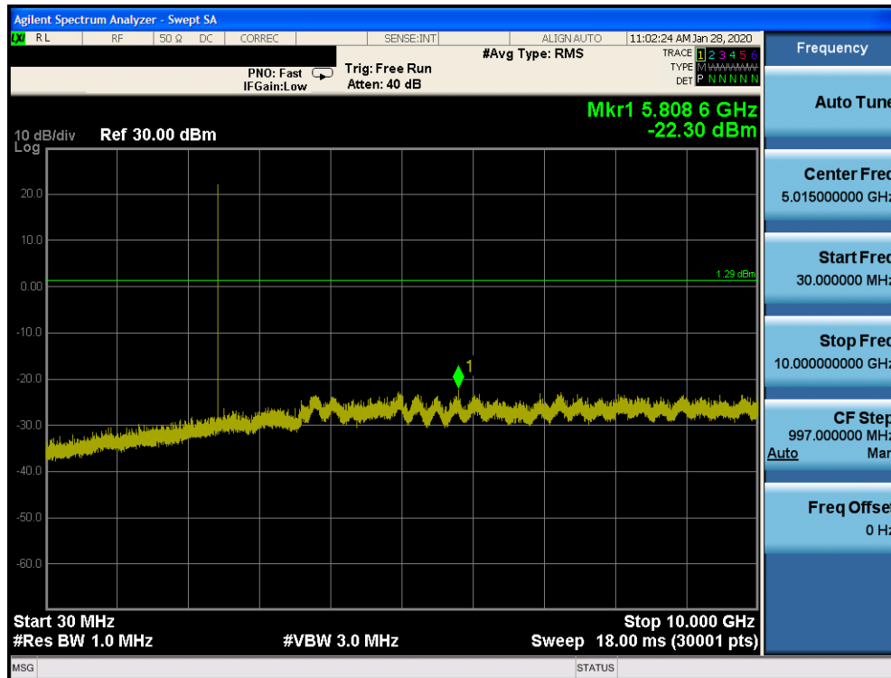
Plot 7-71. Conducted Spurious Plot Ant 4a (Bluetooth (LE), 1Mbps, ePA – Ch. 19)
