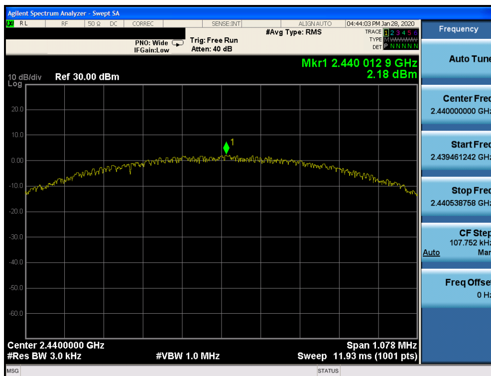
Plot 7-26. Power Spectral Density Plot Ant 2a (Bluetooth (LE), 1Mbps, ePA – Ch. 19)
