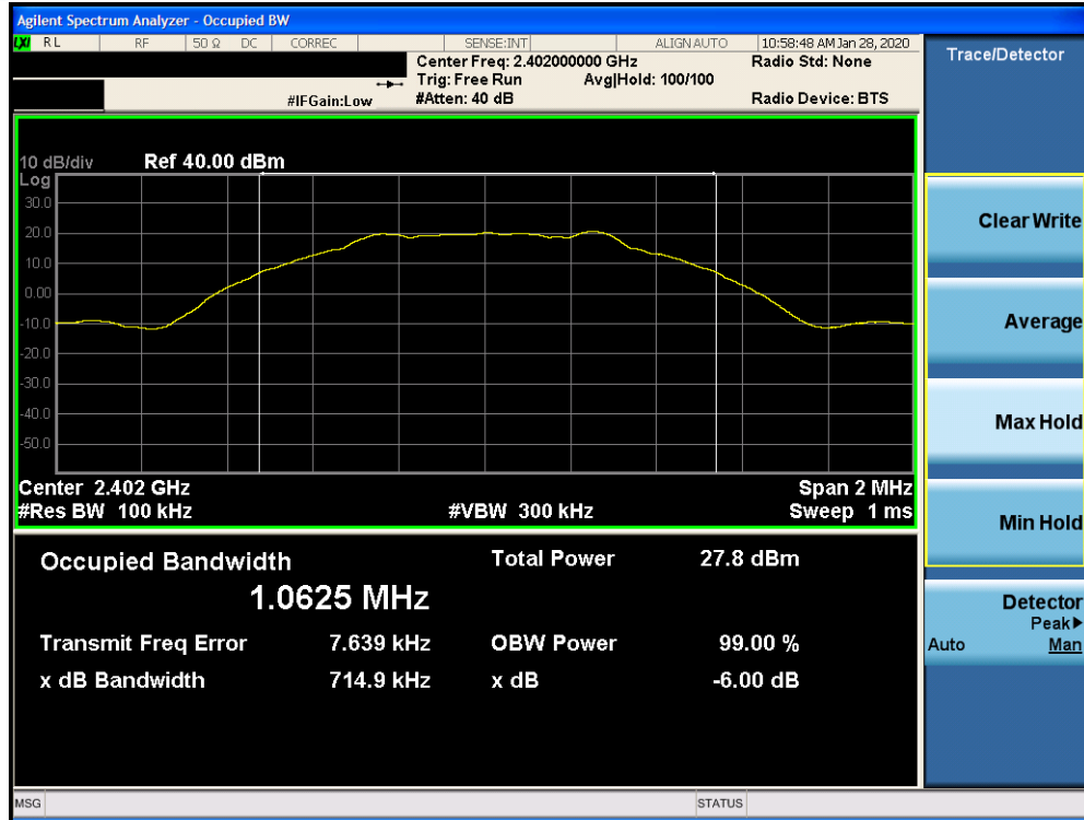
Plot 7-1. 6dB Bandwidth Plot Ant 4a (Bluetooth (LE), 1Mbps, ePA – Ch. 0)
