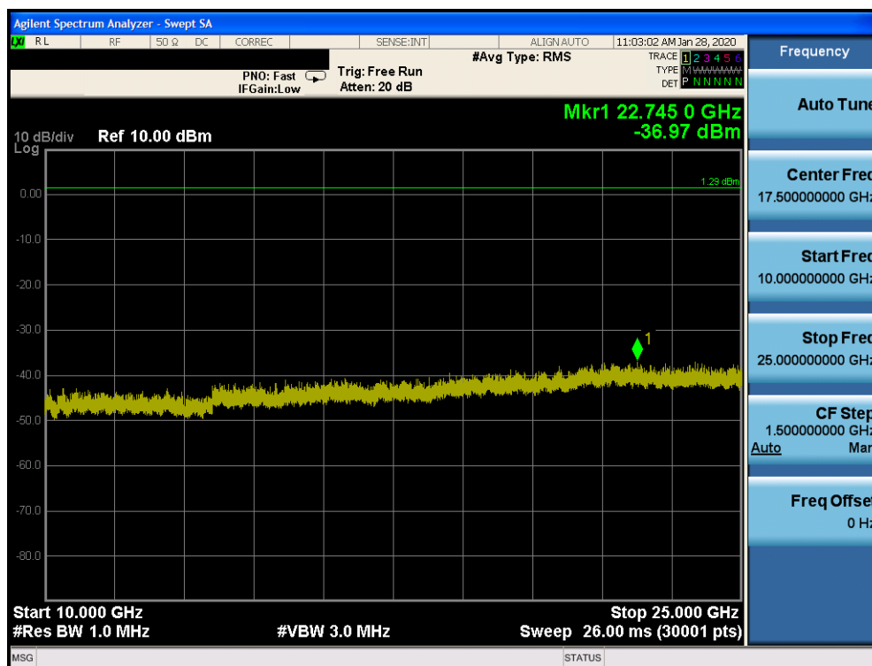
Plot 7-72. Conducted Spurious Plot Ant 4a (Bluetooth (LE), 1Mbps, ePA – Ch. 19)
