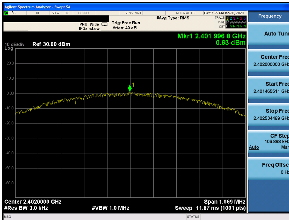
Plot 7-43. Power Spectral Density Plot TxBF Ant 4a (Bluetooth (LE), 1Mbps, iPA – Ch. 0)
