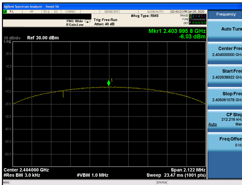
Plot 7-34. Power Spectral Density Plot Ant 2a (Bluetooth (LE), 2Mbps, iPA – Ch. 1)
