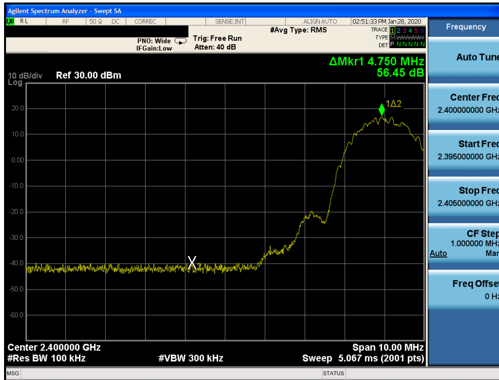
Plot 7-67. Band Edge Plot Ant 2a (Bluetooth (LE), 2Mbps ePA – Ch. 1)
