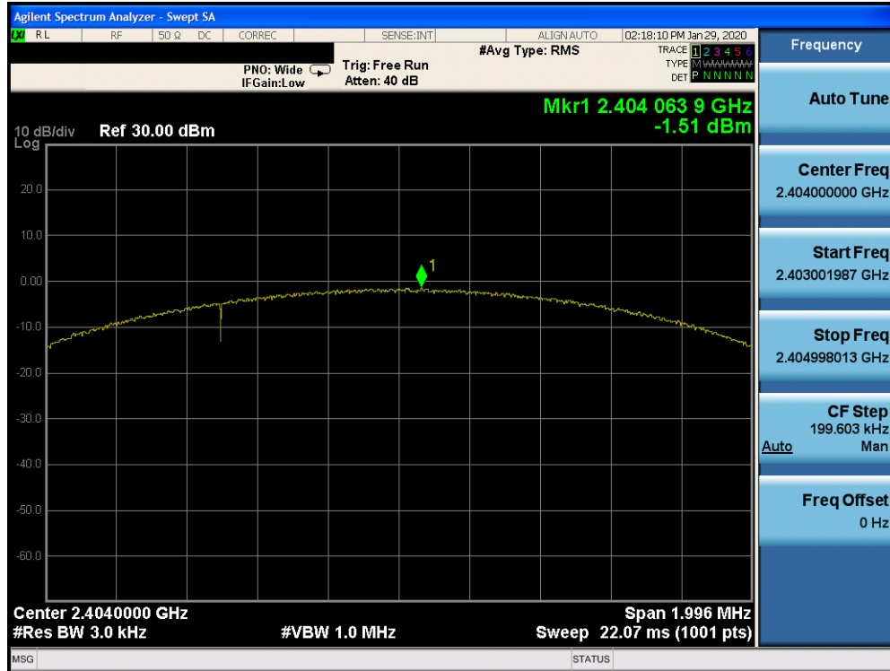
Plot 7-19. Power Spectral Density Plot Ant 4a (Bluetooth (LE), 2Mbps, ePA – Ch. 1)
