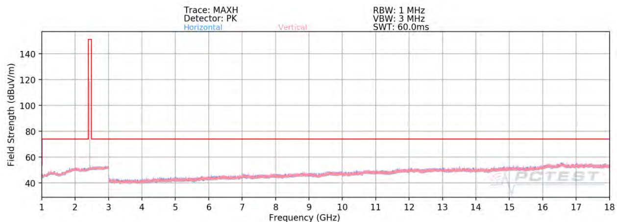
Plot 7-82. Radiated Spurious Plot Above 1GHz Ant 4a (1Mbps, ePA – Ch. 19)
