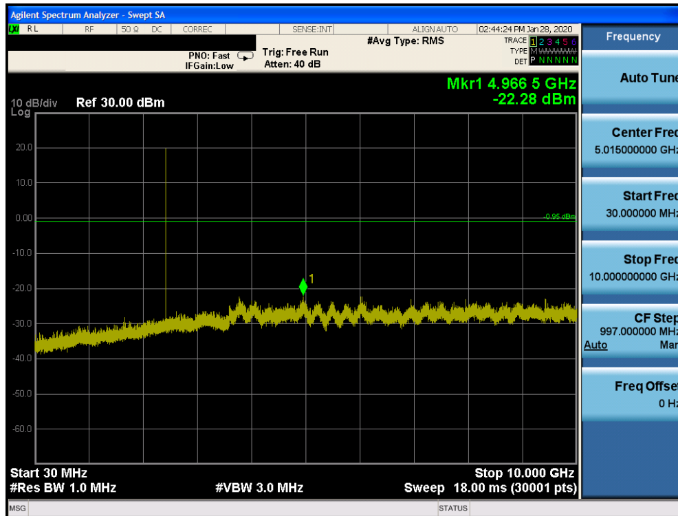
Plot 7-77. Conducted Spurious Plot Ant 2a (Bluetooth (LE), 1Mbps, ePA – Ch. 19)
