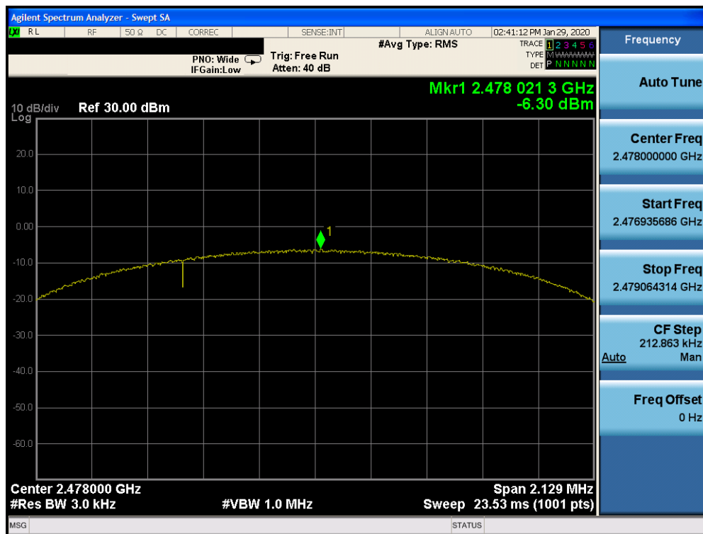
Plot 7-60. Power Spectral Density Plot TxBF Ant 2a (Bluetooth (LE), 2Mbps, iPA – Ch. 38)
