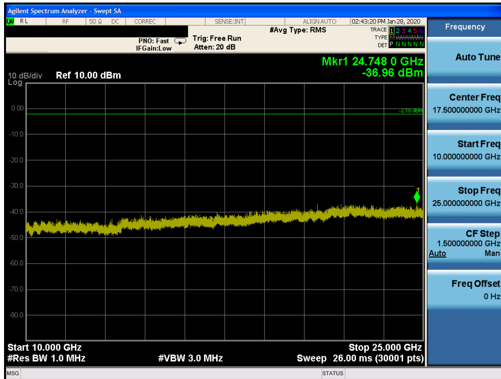
Plot 7-80. Conducted Spurious Plot Ant 2a (Bluetooth (LE), 1Mbps, ePA – Ch. 39)
