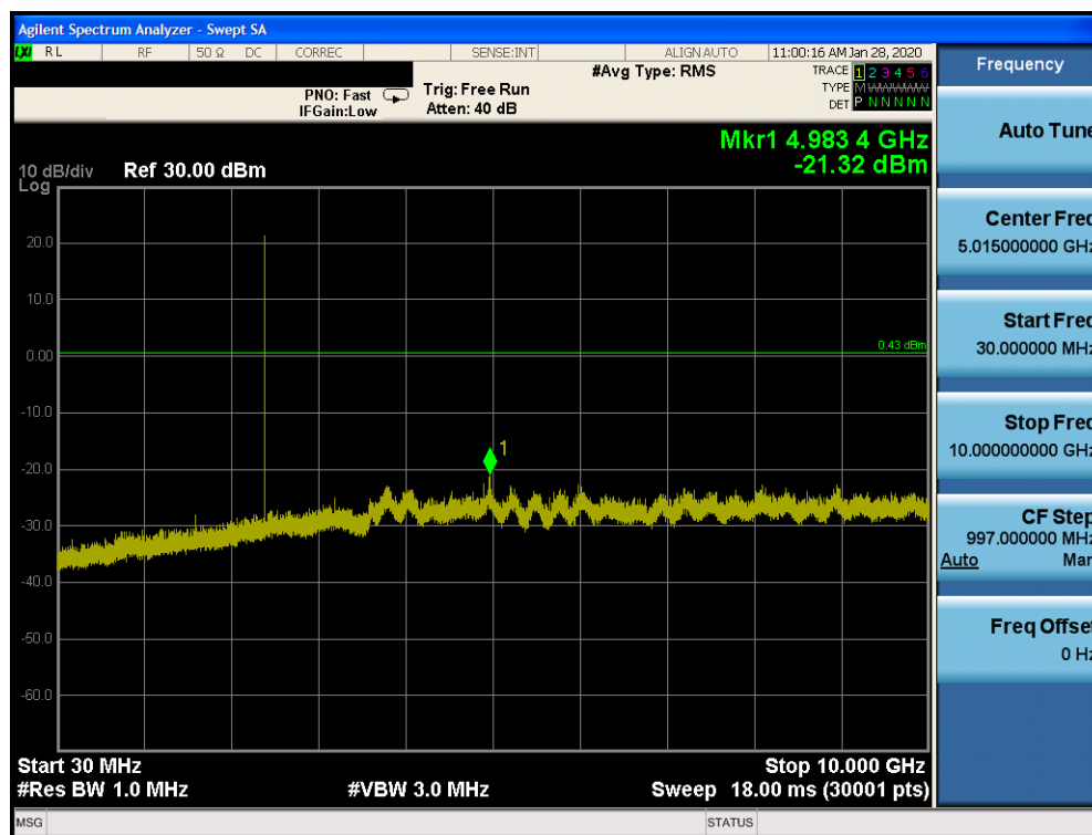
Plot 7-69. Conducted Spurious Plot Ant 4a (Bluetooth (LE), 1Mbps, ePA – Ch. 0)
