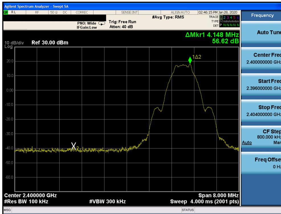
Plot 7-65. Band Edge Plot Ant 2a (Bluetooth (LE), 1Mbps ePA – Ch. 0)
