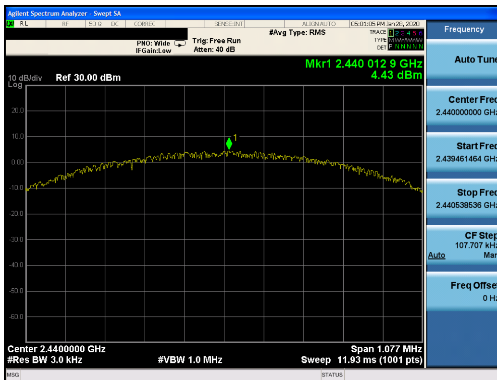
Plot 7-14. Power Spectral Density Plot Ant 4a (Bluetooth (LE), 1Mbps, ePA – Ch. 19)
