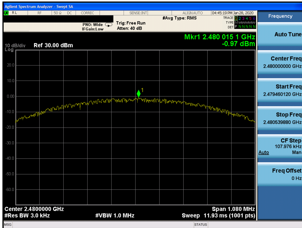
Plot 7-30. Power Spectral Density Plot Ant 2a (Bluetooth (LE), 1Mbps, iPA – Ch. 39)
