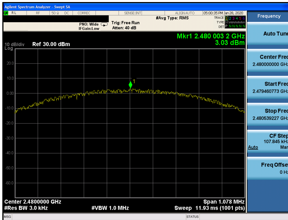
Plot 7-15. Power Spectral Density Plot Ant 4a (Bluetooth (LE), 1Mbps, ePA – Ch. 39)
