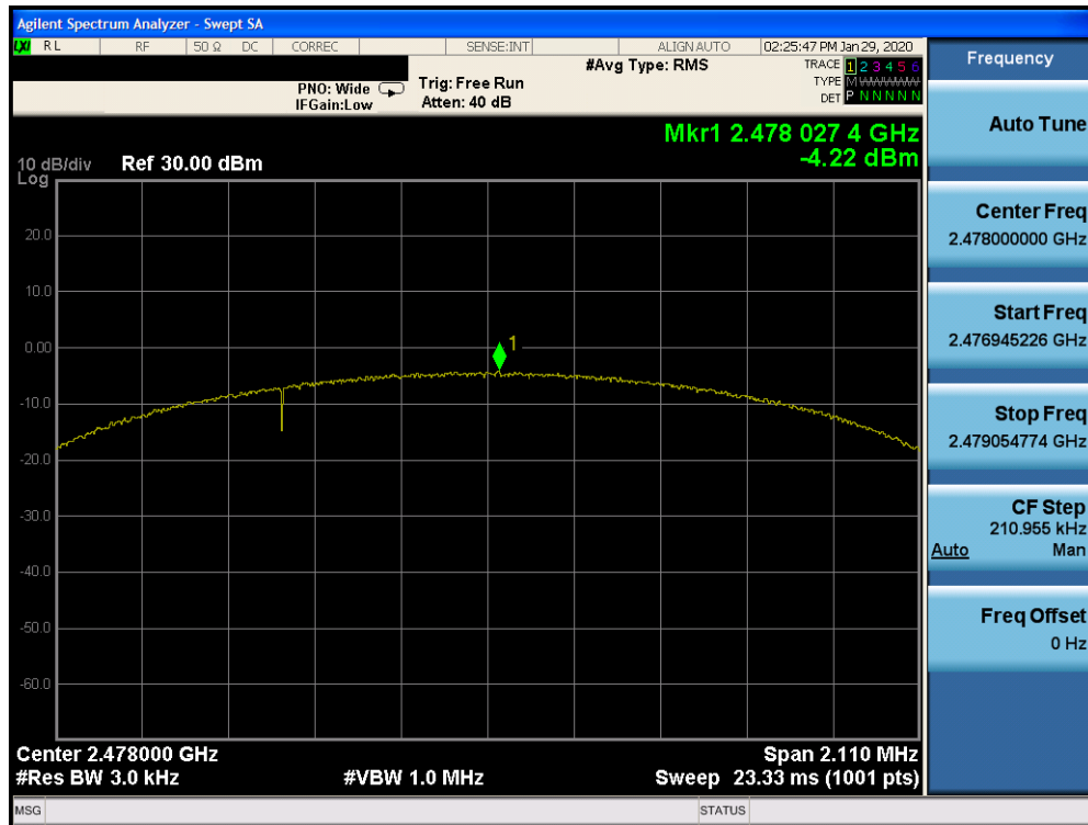
Plot 7-59. Power Spectral Density Plot TxBF Ant 4a (Bluetooth (LE), 2Mbps, iPA – Ch. 38)
