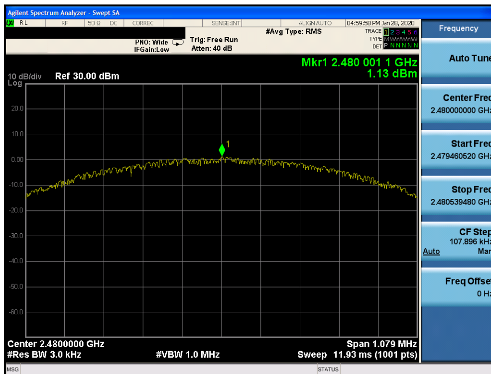
Plot 7-18. Power Spectral Density Plot Ant 4a (Bluetooth (LE), 1Mbps, iPA – Ch. 39)
