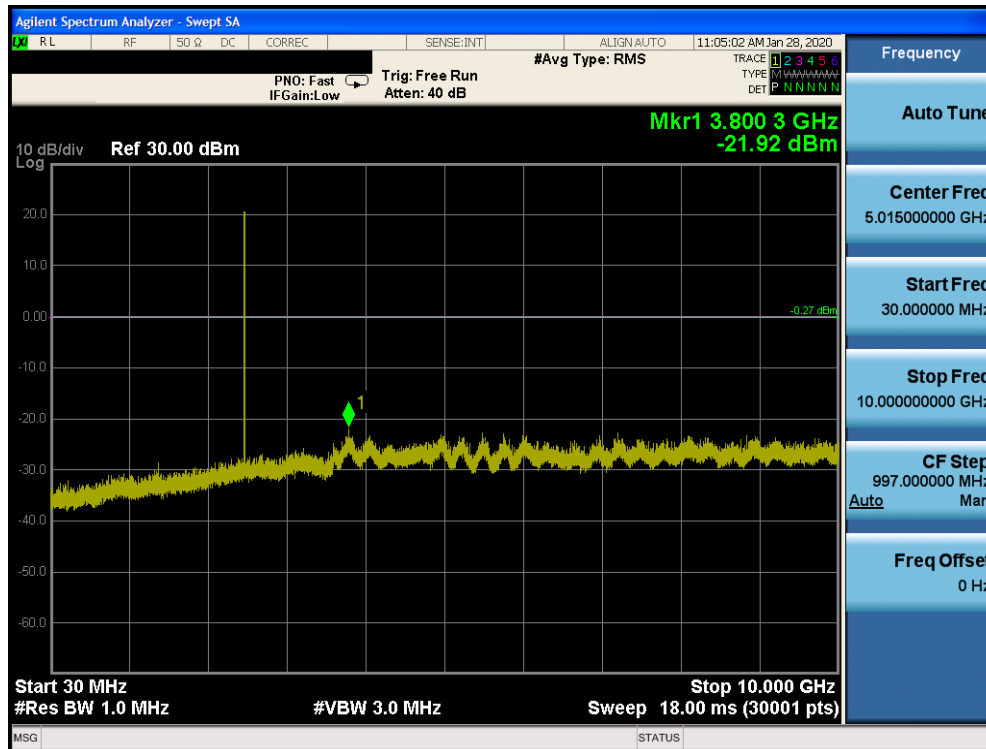
Plot 7-73. Conducted Spurious Plot Ant 4a (Bluetooth (LE), 1Mbps, ePA – Ch. 39)
