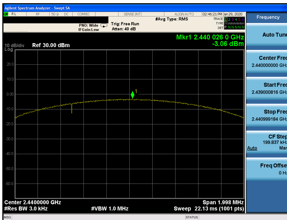
Plot 7-32. Power Spectral Density Plot Ant 2a (Bluetooth (LE), 2Mbps, ePA – Ch. 19)
