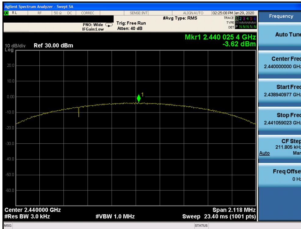
Plot 7-57. Power Spectral Density Plot TxBF Ant 4a (Bluetooth (LE), 2Mbps, iPA – Ch. 19)
