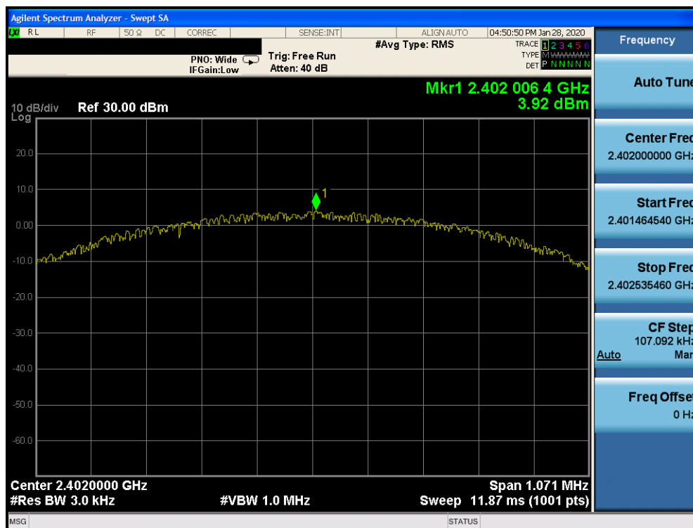
Plot 7-37. Power Spectral Density Plot TxBF Ant 4a (Bluetooth (LE), 1Mbps, ePA – Ch. 0)
