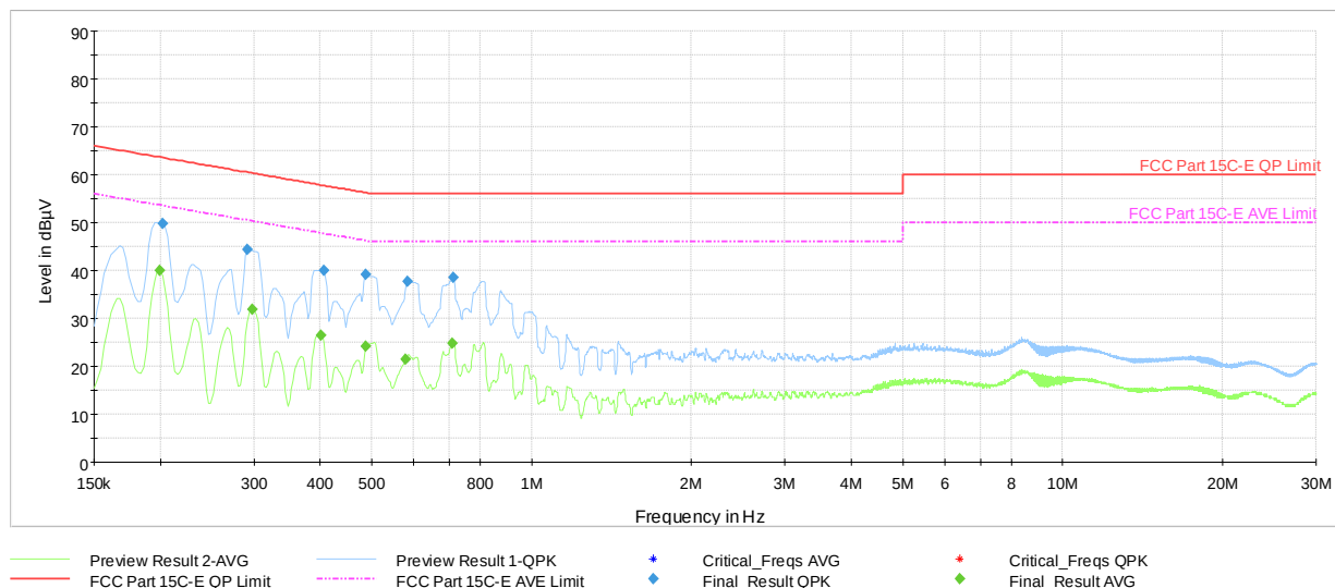
Plot 7-85. Line-Conducted Test Plot- Ch.39 TxBF (L1, with AC/DC Adapter)
