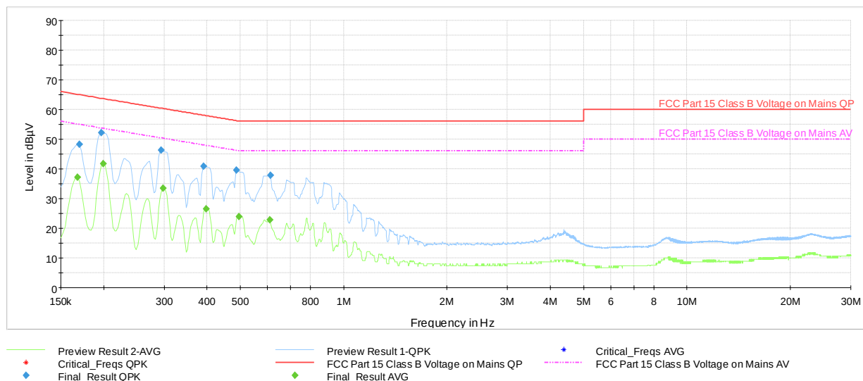
Plot 7-86. Line-Conducted Test Plot- Ch.39 TxBF (N, with AC/DC Adapter)
