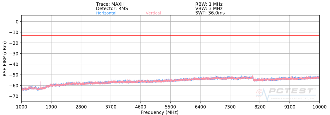
Plot 7-54. Radiated Spurious Plot Above 1GHz (Band 14)
