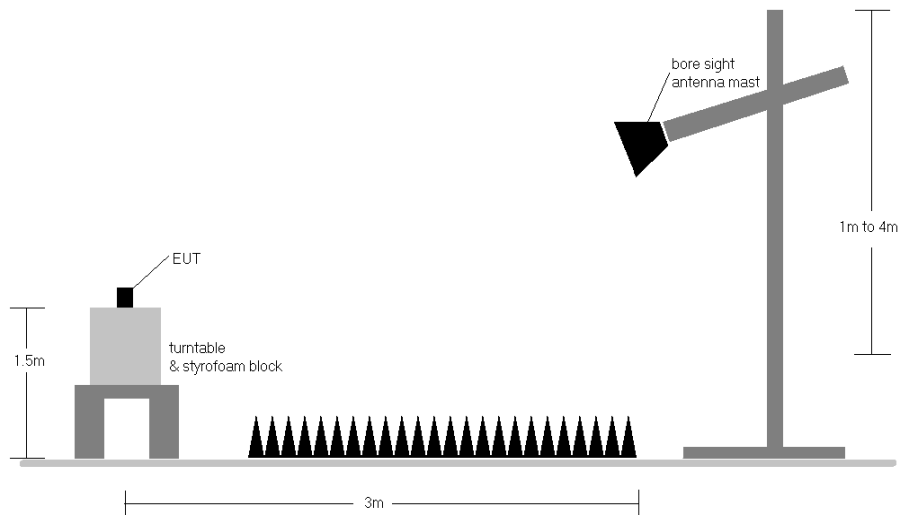
Figure 7-7. Test Instrument & Measurement Setup > 1GHz
