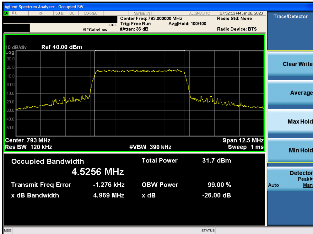
Plot 7-18. Occupied Bandwidth Plot (LTE Band 14 - 5MHz 64-QAM - Full RB Configuration)
