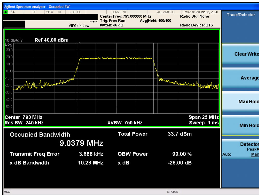
Plot 7-13. Occupied Bandwidth Plot (LTE Band 14 - 10MHz QPSK - Full RB Configuration)
