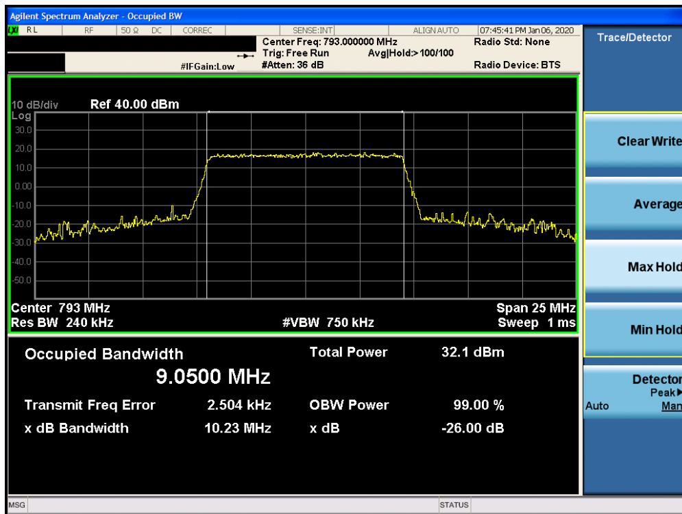
Plot 7-15. Occupied Bandwidth Plot (LTE Band 14 - 10MHz 64-QAM - Full RB Configuration)
