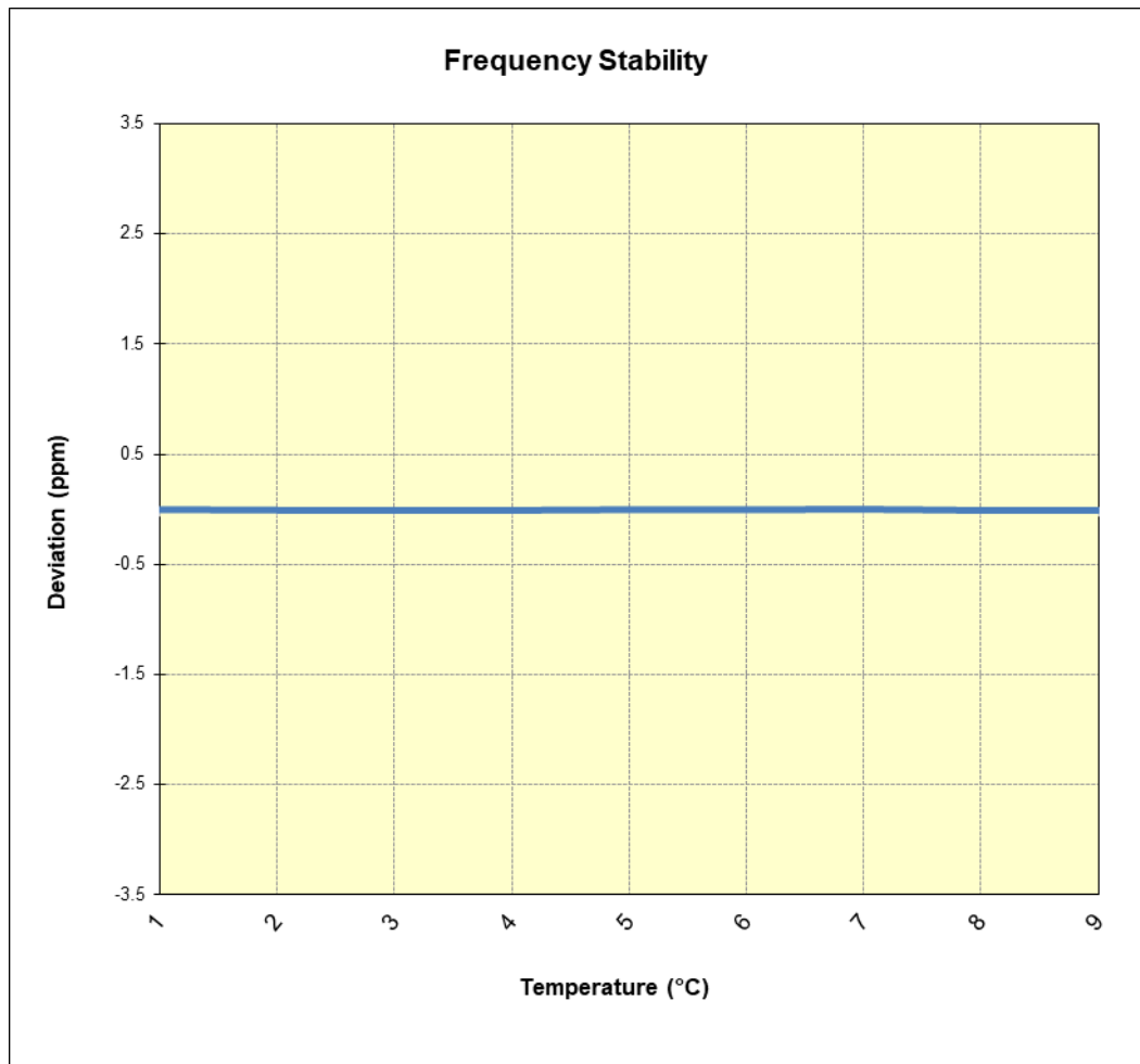
Figure 7-9. LTE Band 26 Frequency Stability Chart
