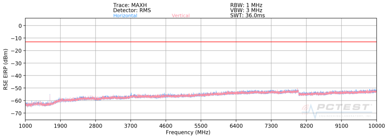
Plot 7-52. Radiated Spurious Plot Above 1GHz (Band 26)
