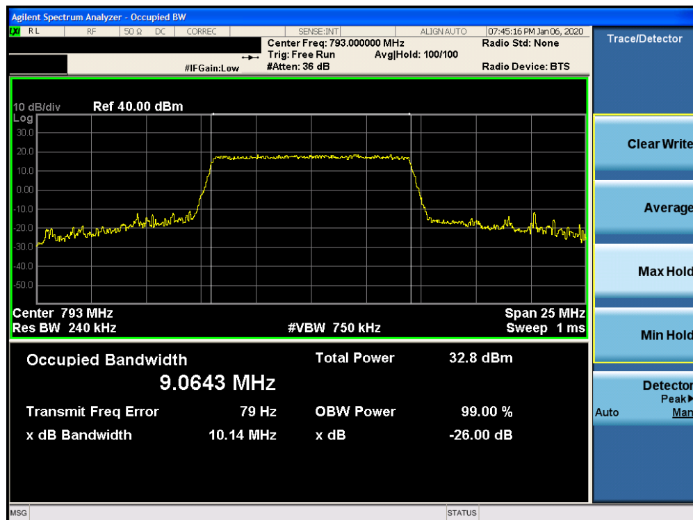
Plot 7-14. Occupied Bandwidth Plot (LTE Band 14 - 10MHz 16-QAM - Full RB Configuration)
