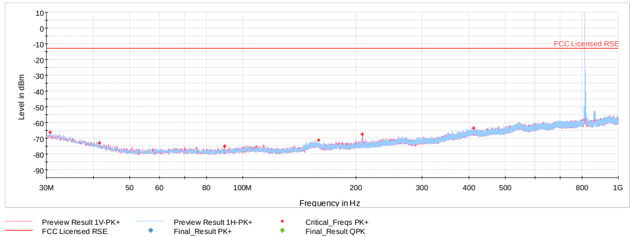
Plot 7-51. Radiated Spurious Plot Below 1GHz (Band 26)
