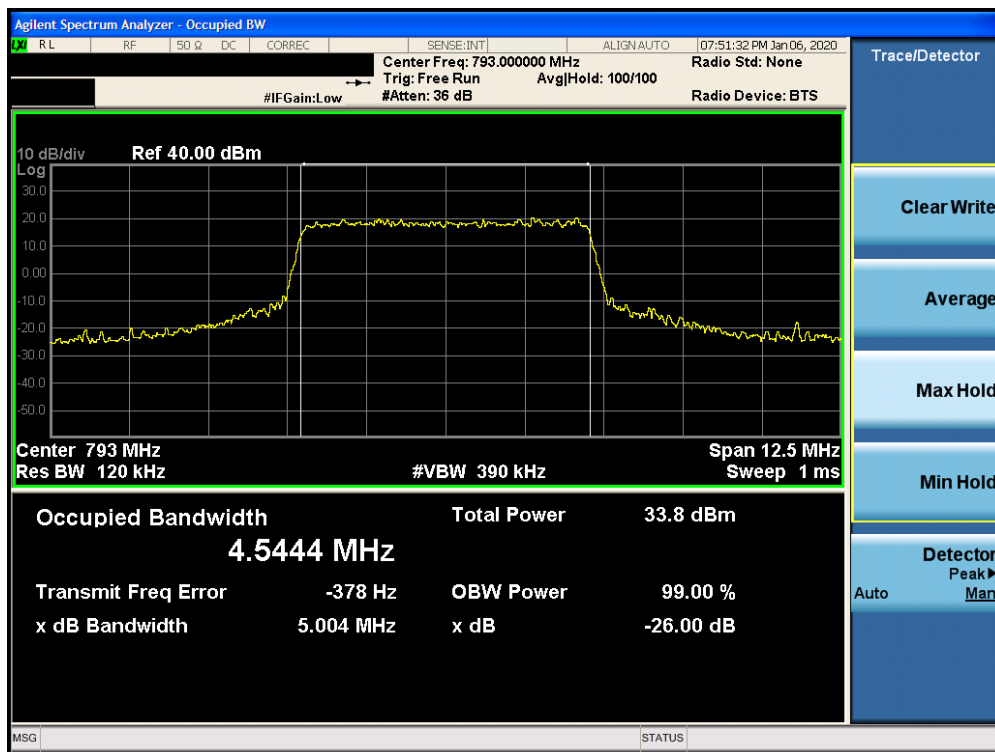
Plot 7-16. Occupied Bandwidth Plot (LTE Band 14 - 5MHz QPSK - Full RB Configuration)
