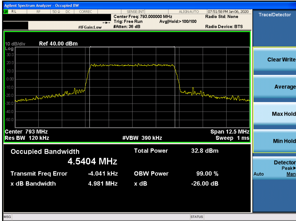
Plot 7-17. Occupied Bandwidth Plot (LTE Band 14 - 5MHz 16-QAM - Full RB Configuration)
