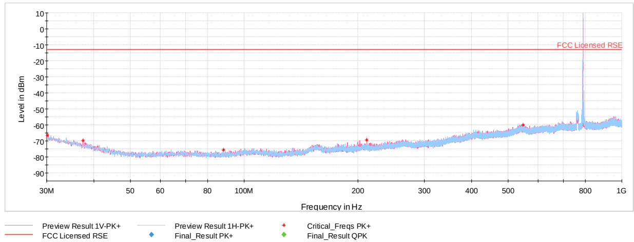
Plot 7-53. Radiated Spurious Plot Below 1GHz (Band 14)
