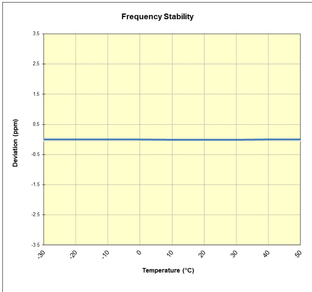
Figure 7-10. LTE Band 14 Frequency Stability Chart
