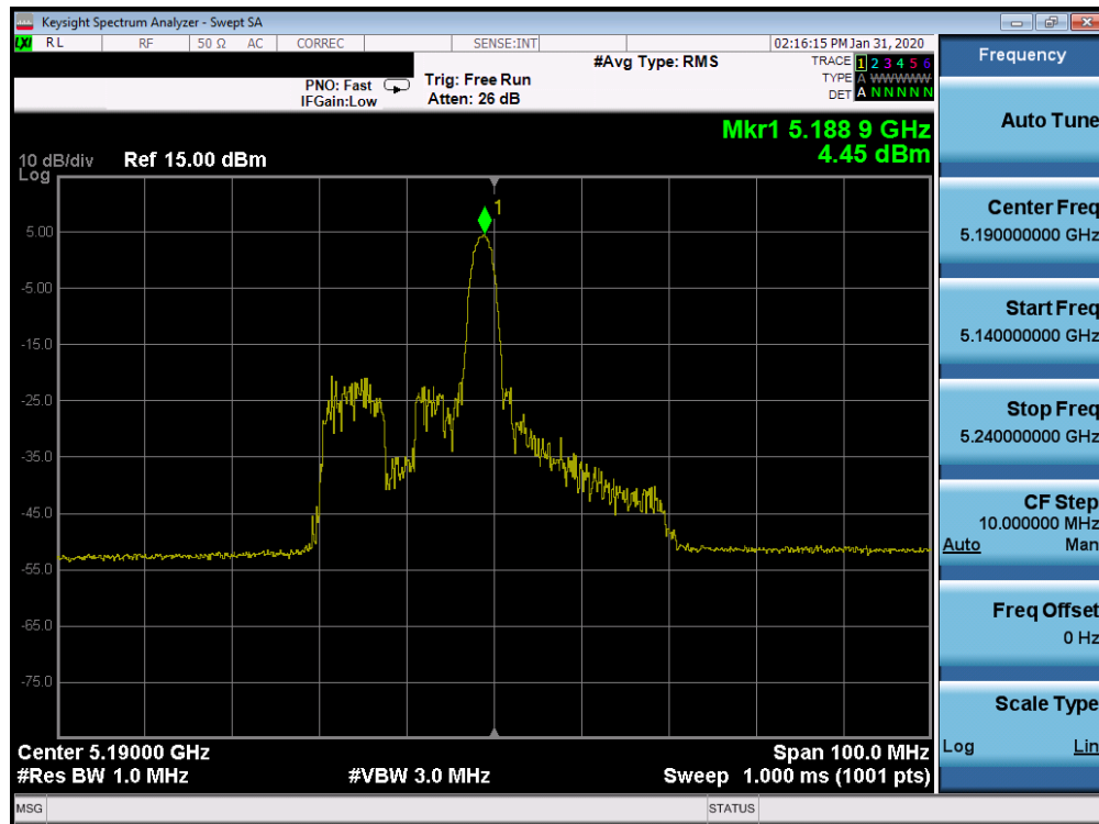
Plot 7-430. Power Spectral Density Plot ISSED SISO CORE 1 (40MHz BW 802.11ax Index 8 – RU26 (UNII Band 1) – Ch. 38)
