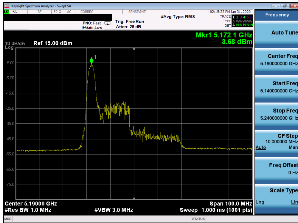
Plot 7-429. Power Spectral Density Plot ISSED SISO CORE 1 (40MHz BW 802.11ax Index 0 – RU26 (UNII Band 1) – Ch. 38)
