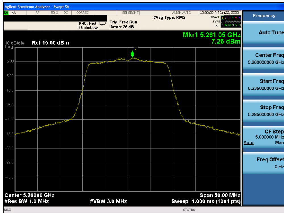
Plot 7-132. Power Spectral Density Plot CDD CORE 1 (20MHz BW 802.11n (UNII Band 2A) – Ch. 52)
