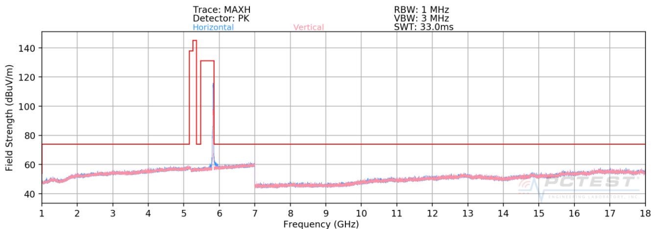
Plot 7-182. Radiated Spurious Plot above 1GHz SISO CORE0 (802.11n - U3 Ch. 165)
