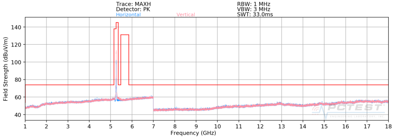
Plot 7-186. Radiated Spurious Plot above 1GHz SISO CORE1 (802.11n – U2A Ch. 52)
