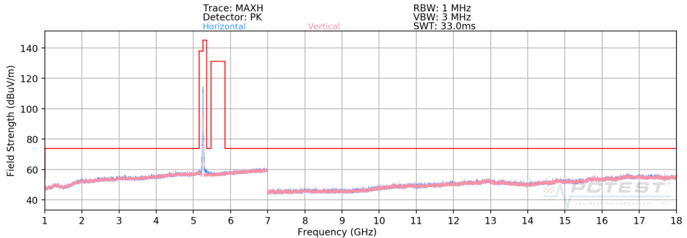
Plot 7-174. Radiated Spurious Plot above 1GHz SISO CORE0 (802.11n – U2A Ch. 52)
