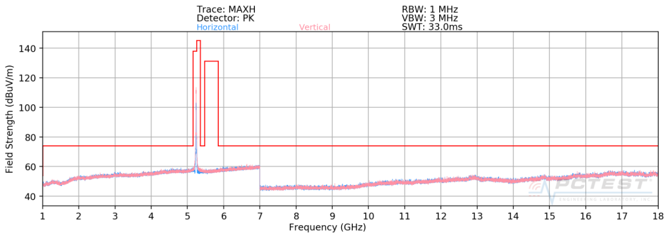
Plot 7-185. Radiated Spurious Plot above 1GHz SISO CORE1 (802.11n – U1 Ch. 48)
