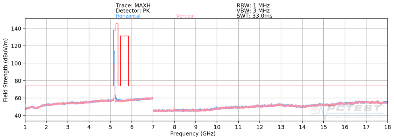
Plot 7-172. Radiated Spurious Plot above 1GHz SISO CORE0 (802.11n – U1 Ch. 40)
