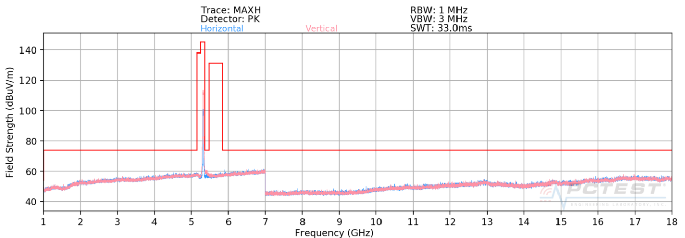
Plot 7-188. Radiated Spurious Plot above 1GHz SISO CORE1 (802.11n – U2A Ch. 64)
