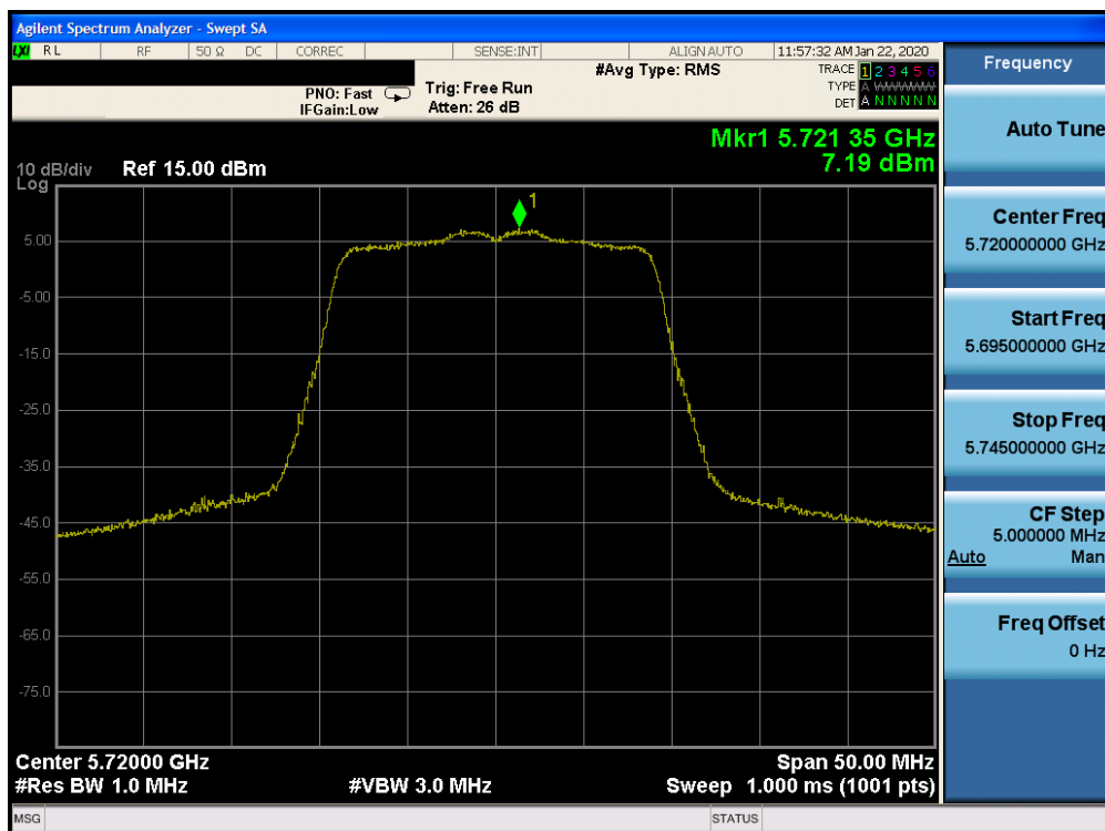
Plot 7-148. Power Spectral Density Plot CDD CORE 1 (20MHz BW 802.11n (UNII Band 2C) – Ch. 144)
