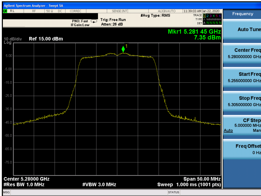
Plot 7-133. Power Spectral Density Plot CDD CORE 0 (20MHz BW 802.11n (UNII Band 2A) – Ch. 56)
