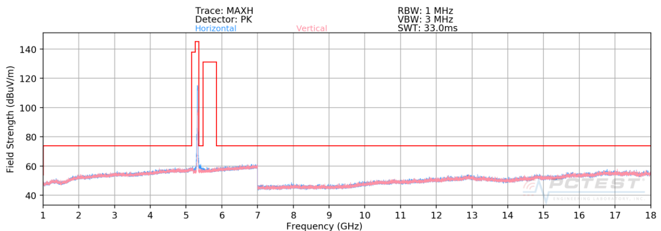
Plot 7-176. Radiated Spurious Plot above 1GHz SISO CORE0 (802.11n – U2A Ch. 64)
