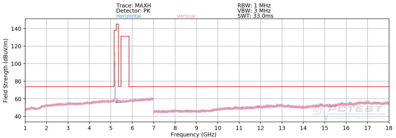
Plot 7-184. Radiated Spurious Plot above 1GHz SISO CORE1 (802.11n – U1 Ch. 40)
