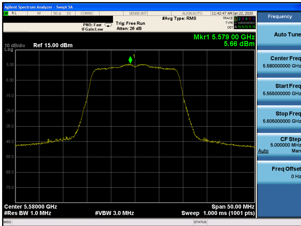
Plot 7-145. Power Spectral Density Plot CDD CORE 0 (20MHz BW 802.11n (UNII Band 2C) – Ch. 116)
