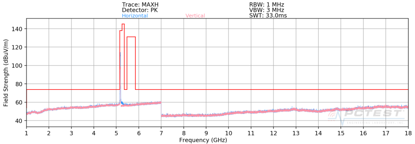
Plot 7-171. Radiated Spurious Plot above 1GHz SISO CORE0 (802.11n – U1 Ch. 36)
