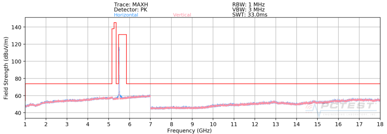
Plot 7-177. Radiated Spurious Plot above 1GHz SISO CORE0 (802.11n – U2C Ch. 100)
