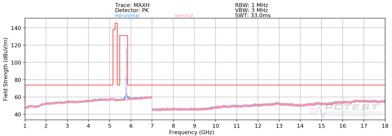
Plot 7-181. Radiated Spurious Plot above 1GHz SISO CORE0 (802.11n - U3 Ch. 157)
