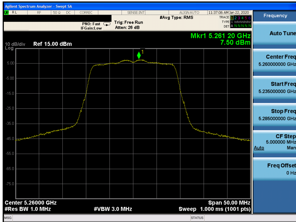
Plot 7-131. Power Spectral Density Plot CDD CORE 0 (20MHz BW 802.11n (UNII Band 2A) – Ch. 52)
