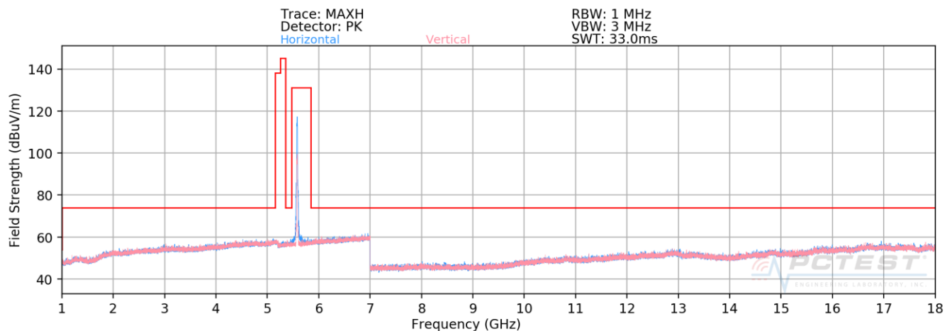
Plot 7-178. Radiated Spurious Plot above 1GHz SISO CORE0 (802.11n – U2C Ch. 116)
