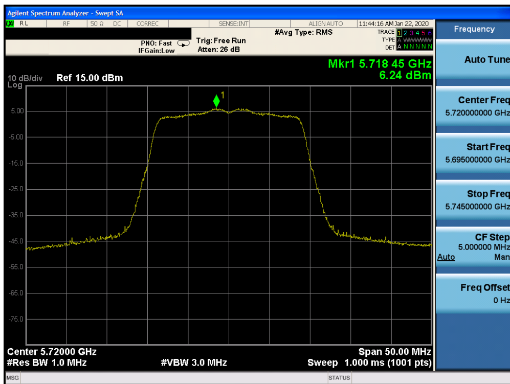
Plot 7-147. Power Spectral Density Plot CDD CORE 0 (20MHz BW 802.11n (UNII Band 2C) – Ch. 144)
