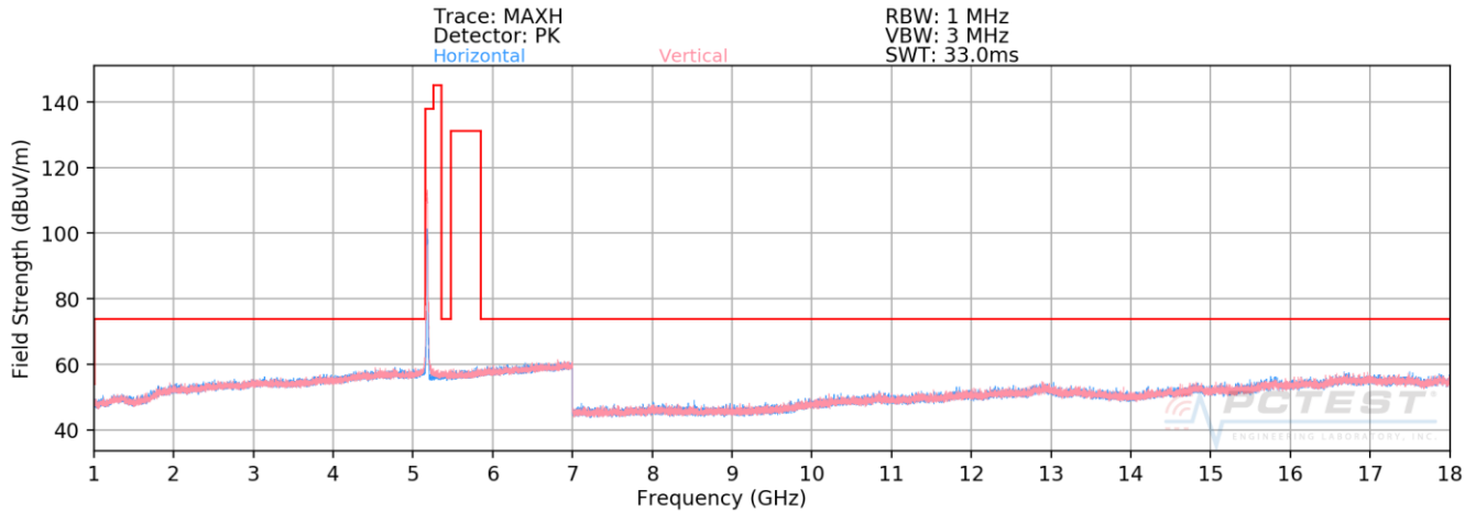
Plot 7-183. Radiated Spurious Plot above 1GHz SISO CORE1 (802.11n – U1 Ch. 36)
