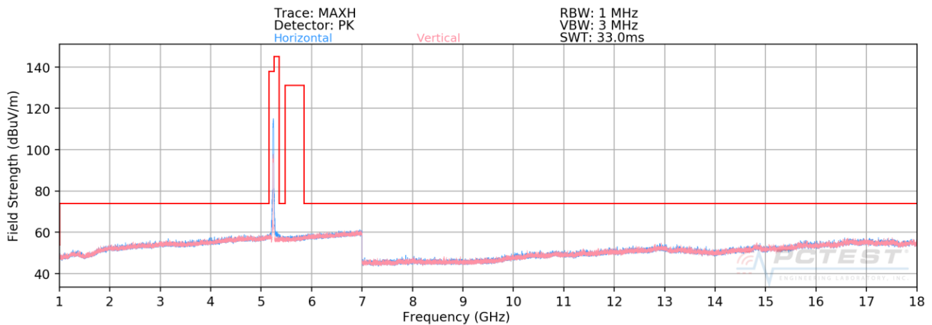
Plot 7-173. Radiated Spurious Plot above 1GHz SISO CORE0 (802.11n – U1 Ch. 48)
