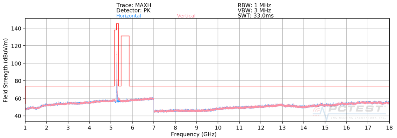
Plot 7-187. Radiated Spurious Plot above 1GHz SISO CORE1 (802.11n – U2A Ch. 60)
