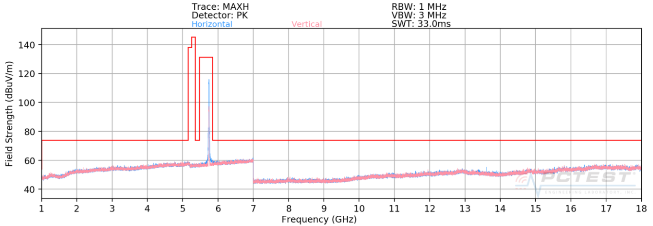
Plot 7-180. Radiated Spurious Plot above 1GHz SISO CORE0 (802.11n - U3 Ch. 149)
