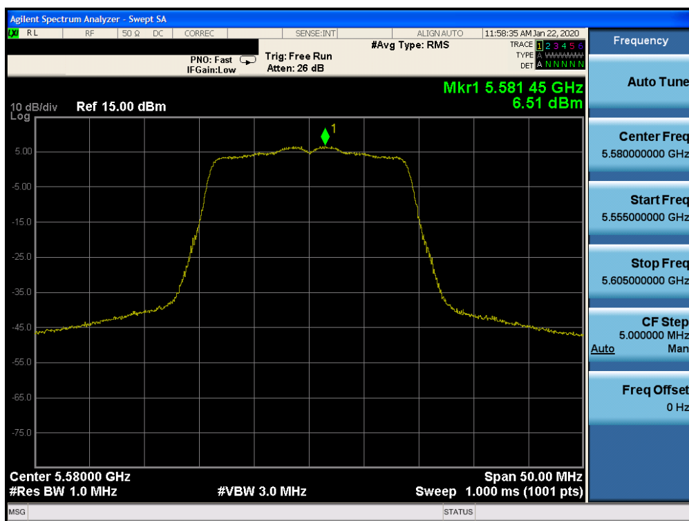
Plot 7-146. Power Spectral Density Plot CDD CORE 1 (20MHz BW 802.11n (UNII Band 2C) – Ch. 116)
