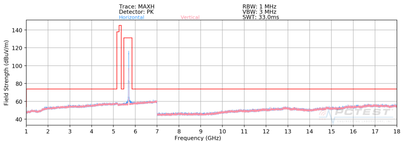
Plot 7-179. Radiated Spurious Plot above 1GHz SISO CORE0 (802.11n – U2C Ch. 144)
