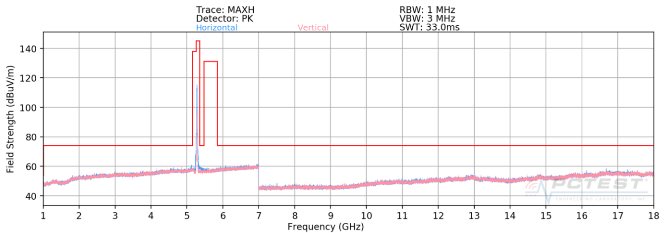
Plot 7-175. Radiated Spurious Plot above 1GHz SISO CORE0 (802.11n – U2A Ch. 60)
