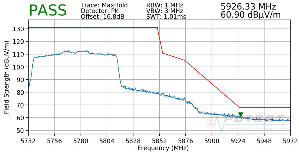
Plot 7-255. Radiated Upper Band Edge Plot SISO CORE1 (Peak – UNII Band 3)
