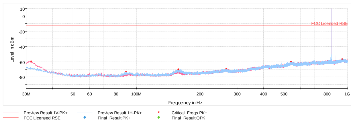
Plot 7-76. Radiated Spurious Plot Below 1GHz (Cellular GPRS Mode) with AC/DC Adapter
