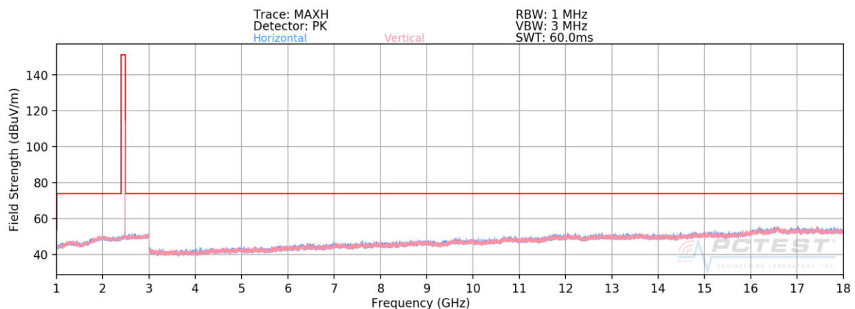
Plot 7-59. Radiated Spurious Plot above 1GHz Ant 4a (BT GFSK ePA – Ch. 78)
