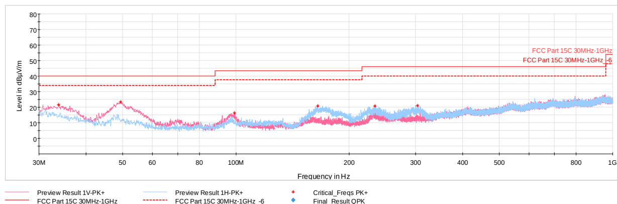
Plot 7-83. Radiated Spurious Plot below 1GHz GFSK ePA Tx BF – Ch.39 , with AC/DC Adapter)
