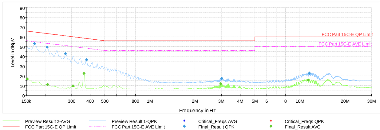
Plot 7-85. Line-Conducted Test Plot- Ch.39 TxBF (L1, with Laptop)
