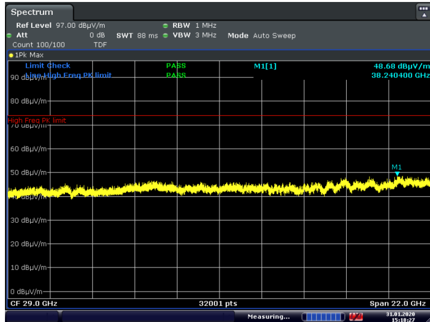
Plot 7-69. Radiated Spurious Plot Simultaneous Tx 18GHz– 40GHz Pol. H
