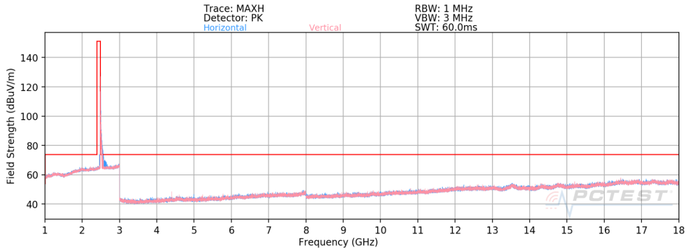
Plot 7-68. Radiated Spurious Plot above 1GHz Simultaneous Tx
