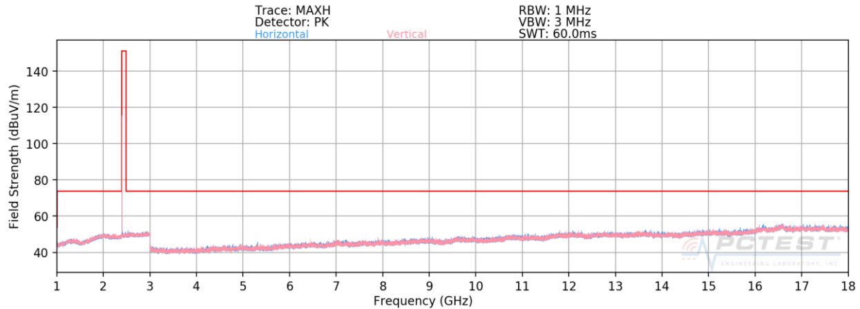
Plot 7-57. Radiated Spurious Plot above 1GHz Ant 4a (BT GFSK ePA – Ch. 0)
