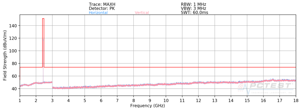
Plot 7-58. Radiated Spurious Plot above 1GHz Ant 4a (BT GFSK ePA – Ch. 39)
