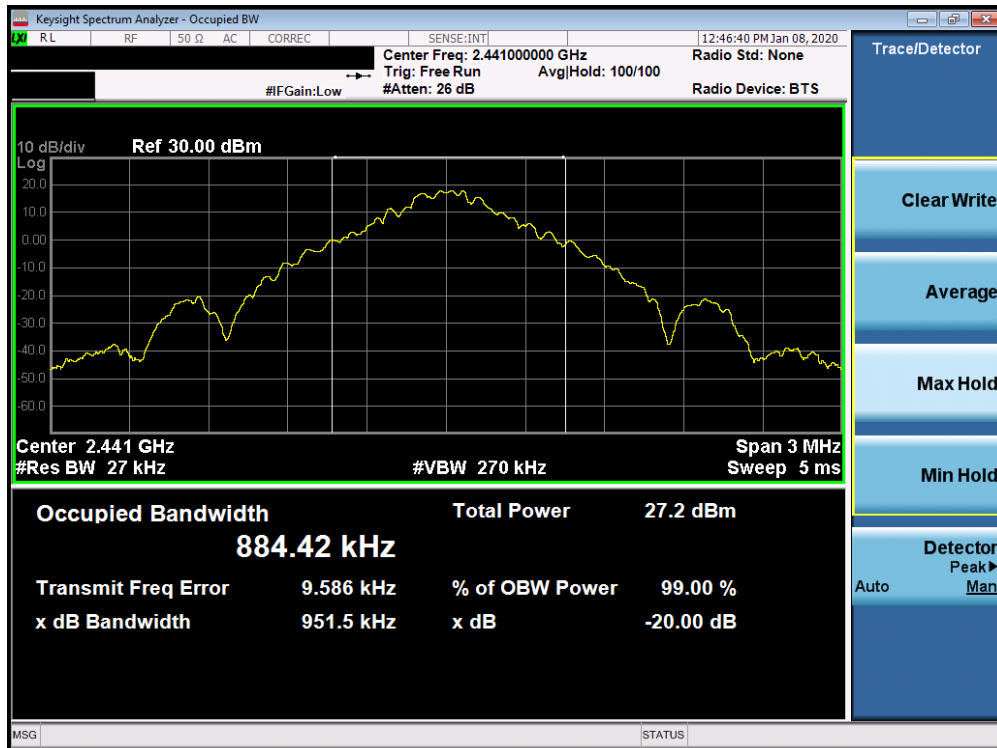
Plot 7-2. 20dB Bandwidth Plot Ant 4a (Bluetooth, GFSK, ePA – Ch. 39)
