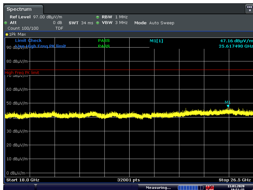
Plot 7-67. Radiated Spurious Plot above 18GHz TxBF (GFSK ePA, Pol. H)
