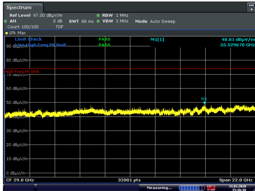
Plot 7-70. Radiated Spurious Plot Simultaneous Tx 18GHz– 40GHz Pol. V
