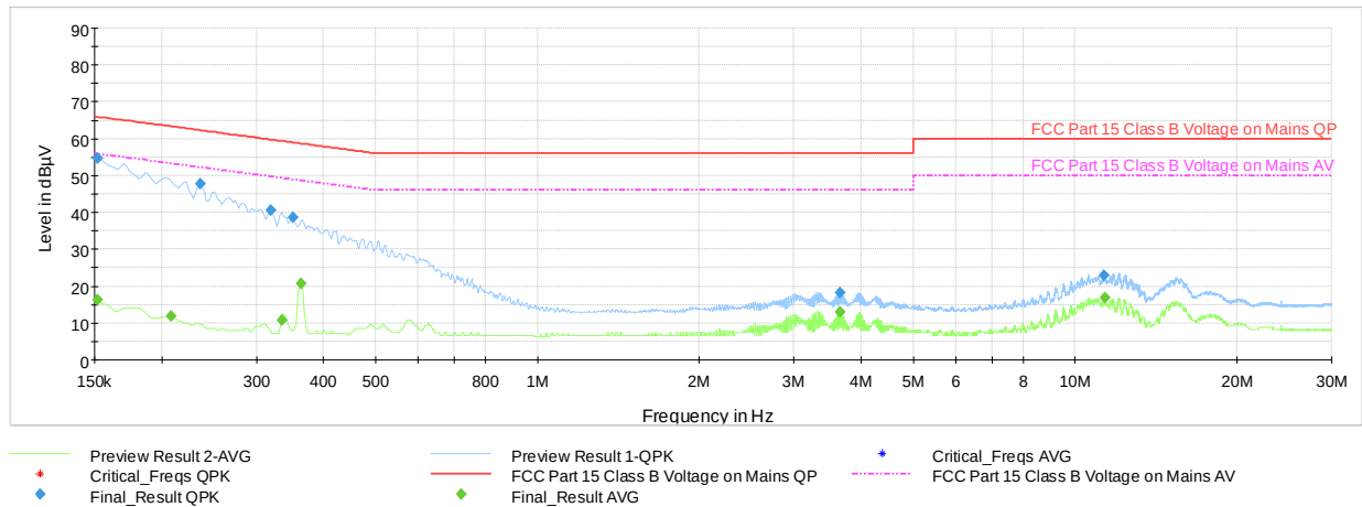
Plot 7-86. Line-Conducted Test Plot- Ch.39 TxBF (N, with Laptop)
