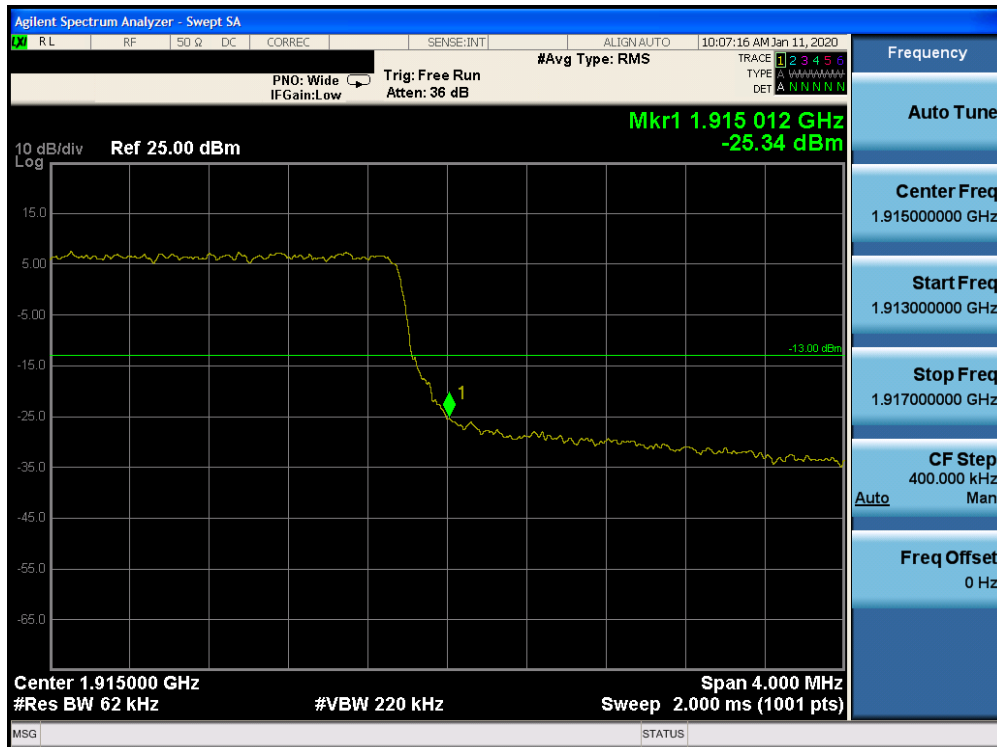
Plot 7-316. Upper Band Edge Plot (Band 25 – 5.0MHz QPSK – RB Size 25)
