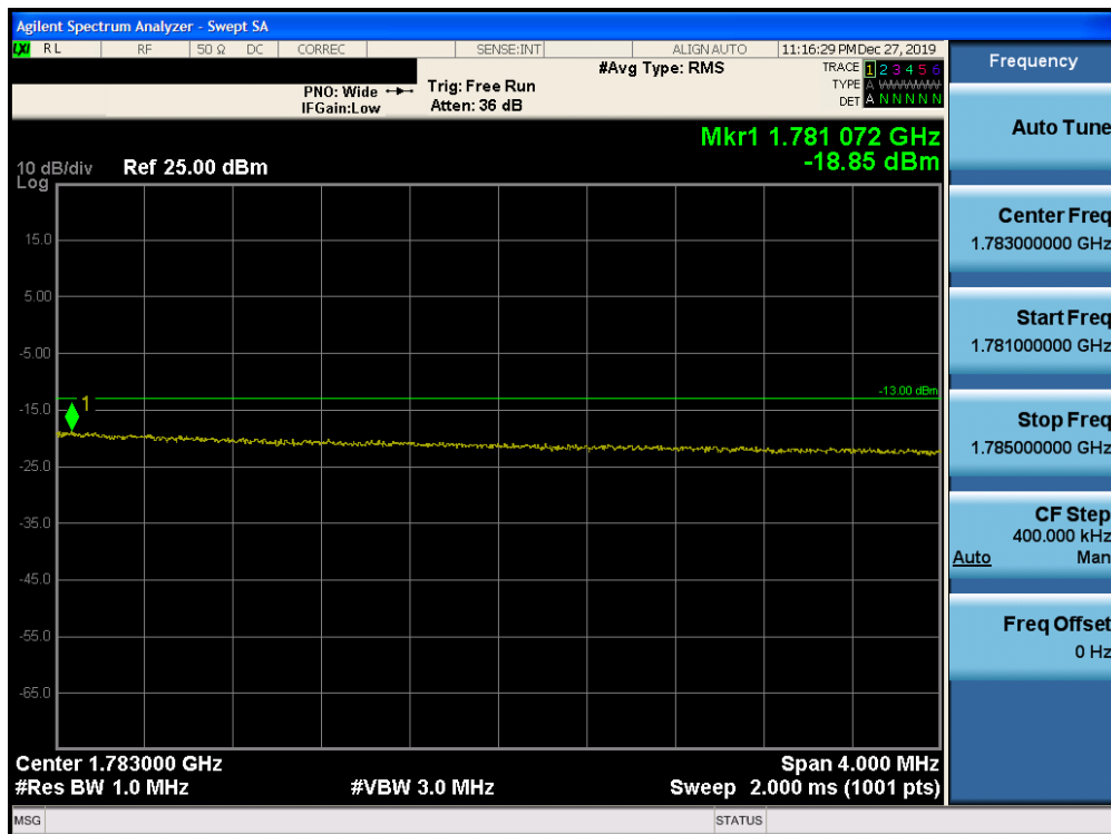
Plot 7-281. Upper Extended Band Edge Plot (Band 66 – 20.0MHz QPSK – RB Size 100)
