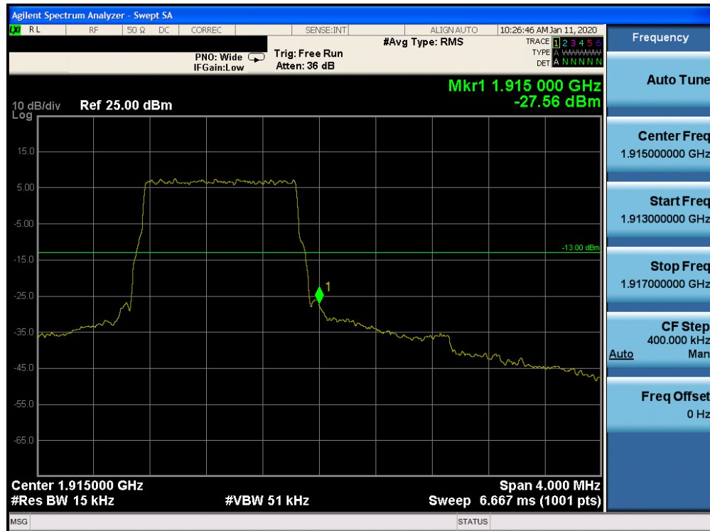
Plot 7-308. Upper Band Edge Plot (Band 25 – 1.4MHz QPSK – RB Size 6)
