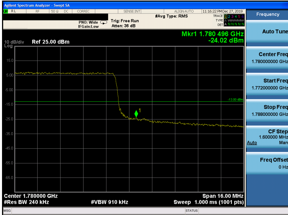
Plot 7-280. Upper Band Edge Plot (Band 66 – 20.0MHz QPSK – RB Size 100)
