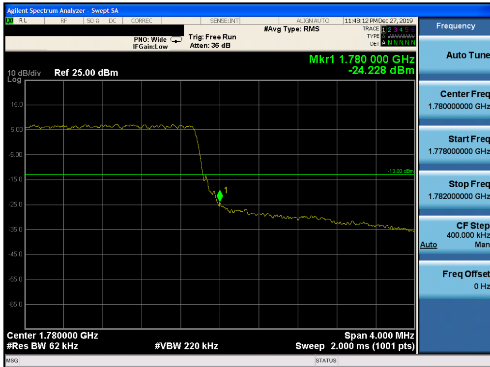
Plot 7-268. Upper Band Edge Plot (Band 66 – 5.0MHz QPSK – RB Size 25)
