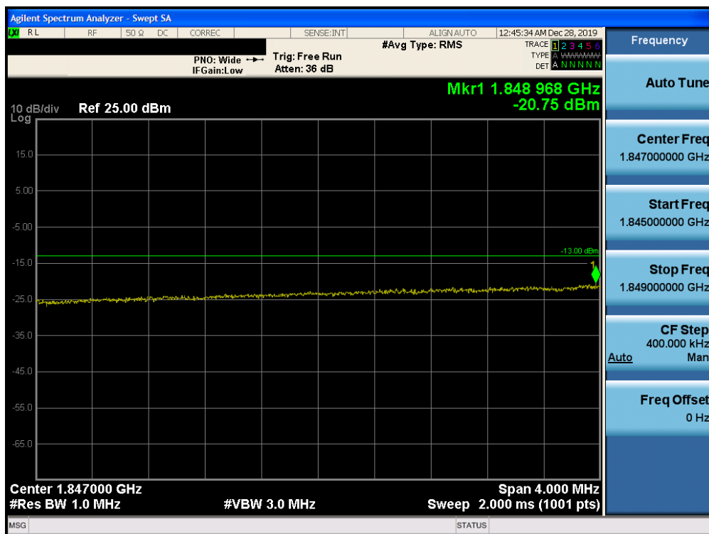
Plot 7-303. Lower Extended Band Edge Plot (Band 2 – 20.0MHz QPSK – RB Size 100)
