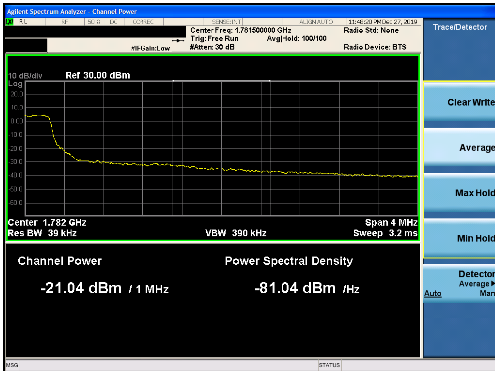
Plot 7-269. Upper Extended Band Edge Plot (Band 66 – 5.0MHz QPSK – RB Size 25)
