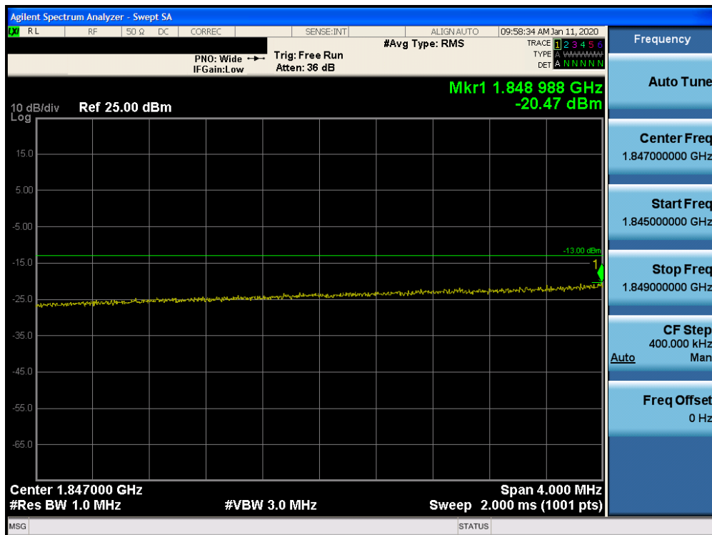
Plot 7-323. Lower Extended Band Edge Plot (Band 25 – 15.0MHz QPSK – RB Size 75)
