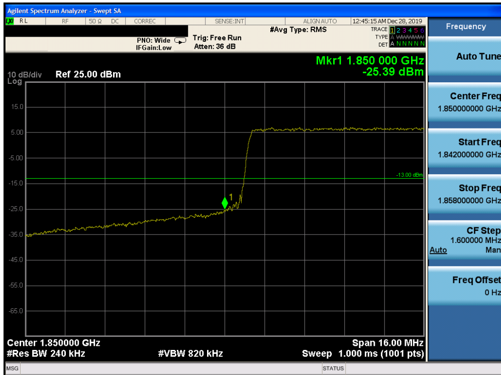
Plot 7-302. Lower Band Edge Plot (Band 2 – 20.0MHz QPSK – RB Size 100)
