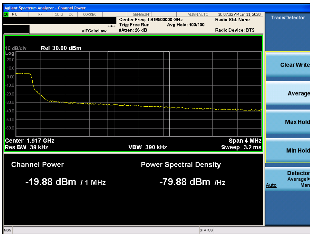
Plot 7-317. Upper Extended Band Edge Plot (Band 25 – 5.0MHz QPSK – RB Size 25)
