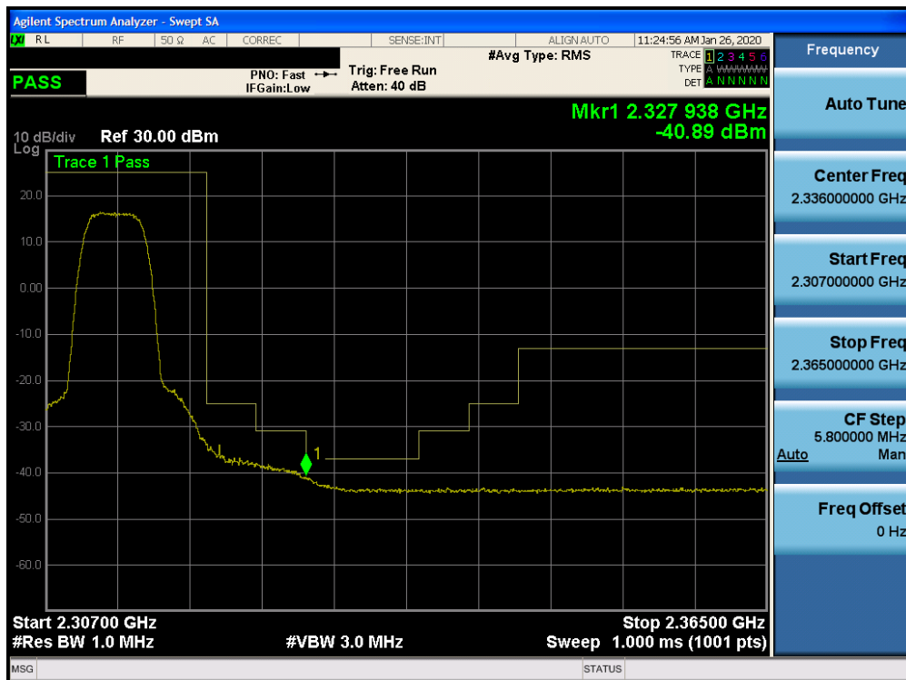
Plot 7-333. Upper Extended Band Edge Plot (Band 30 – 5.0MHz QPSK – RB Size 25)
