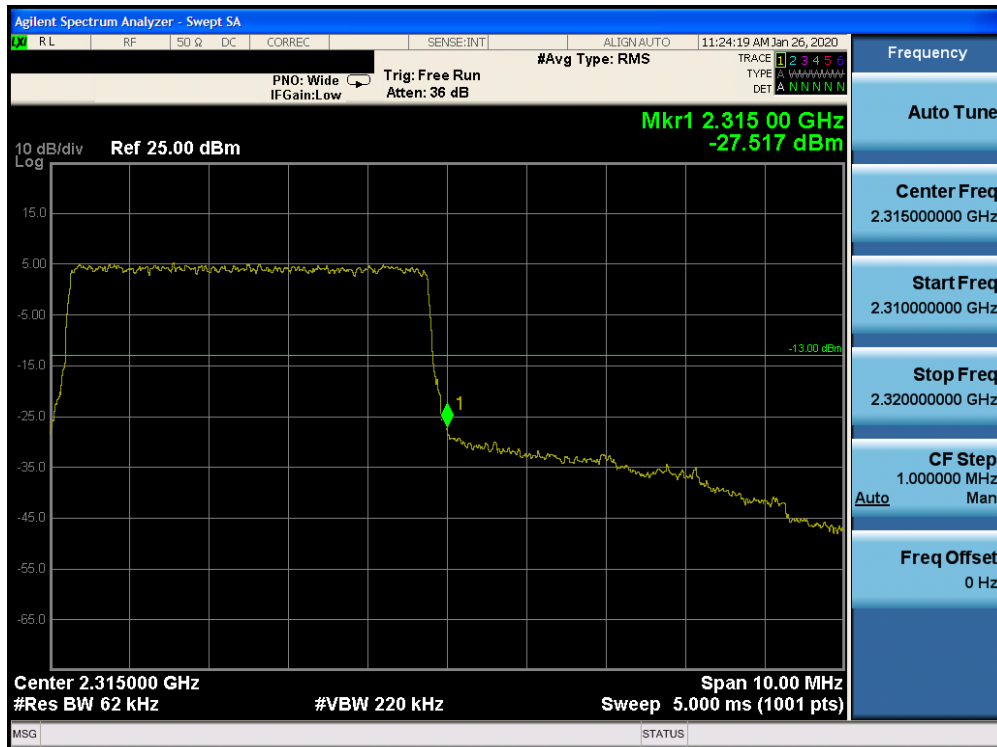
Plot 7-332. Upper Band Edge Plot (Band 30 – 5.0MHz QPSK – RB Size 25)
