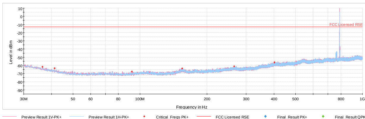
Plot 7-53. Radiated Spurious Plot Below 1GHz (Band 14)
