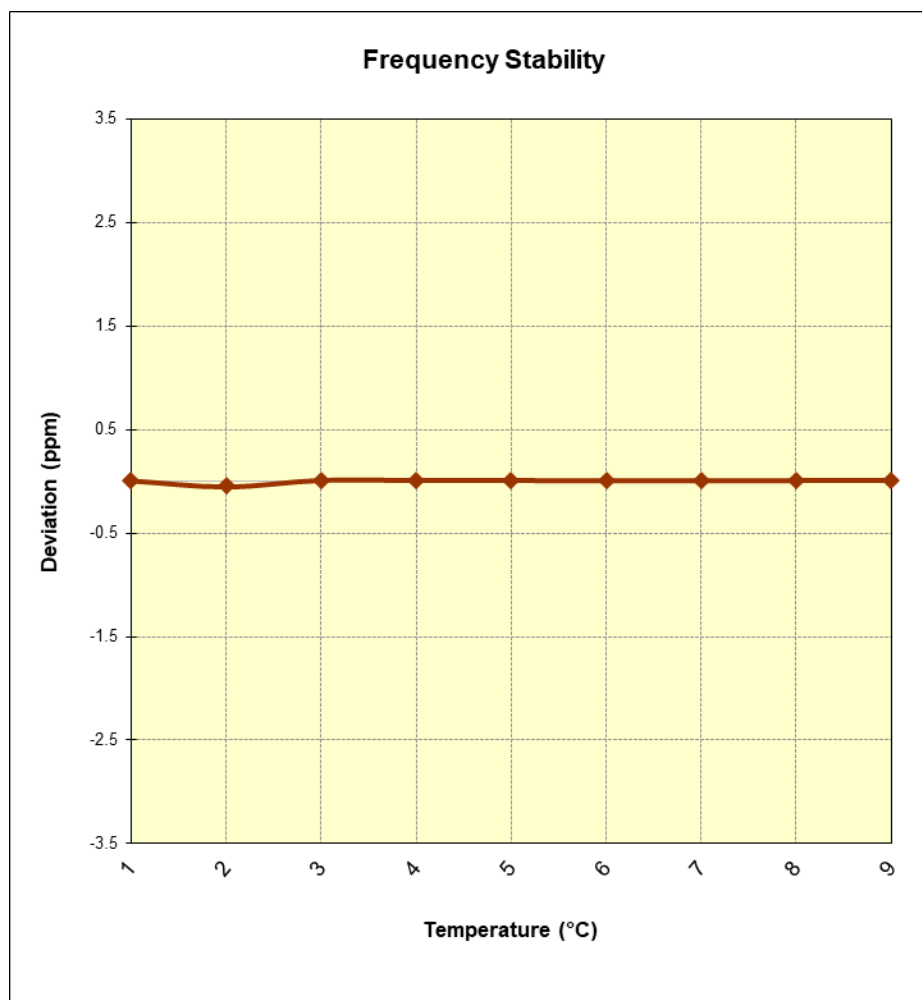
Figure 7-9. LTE Band 26 Frequency Stability Chart
