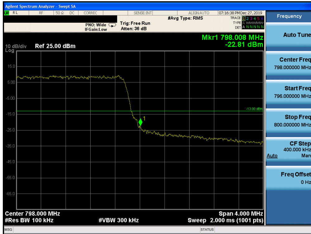
Plot 7-47. Upper Band Edge Plot (LTE Band 14 - 5MHz QPSK)
