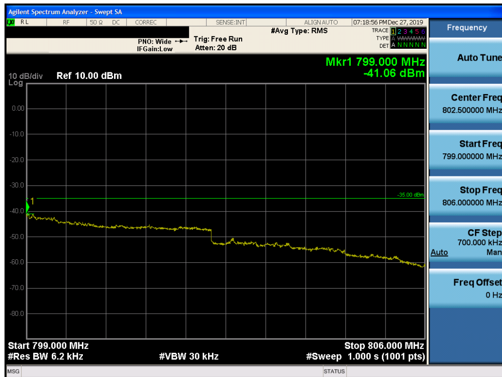
Plot 7-48. Upper Emission Mask Plot (LTE Band 14 - 5MHz QPSK)
