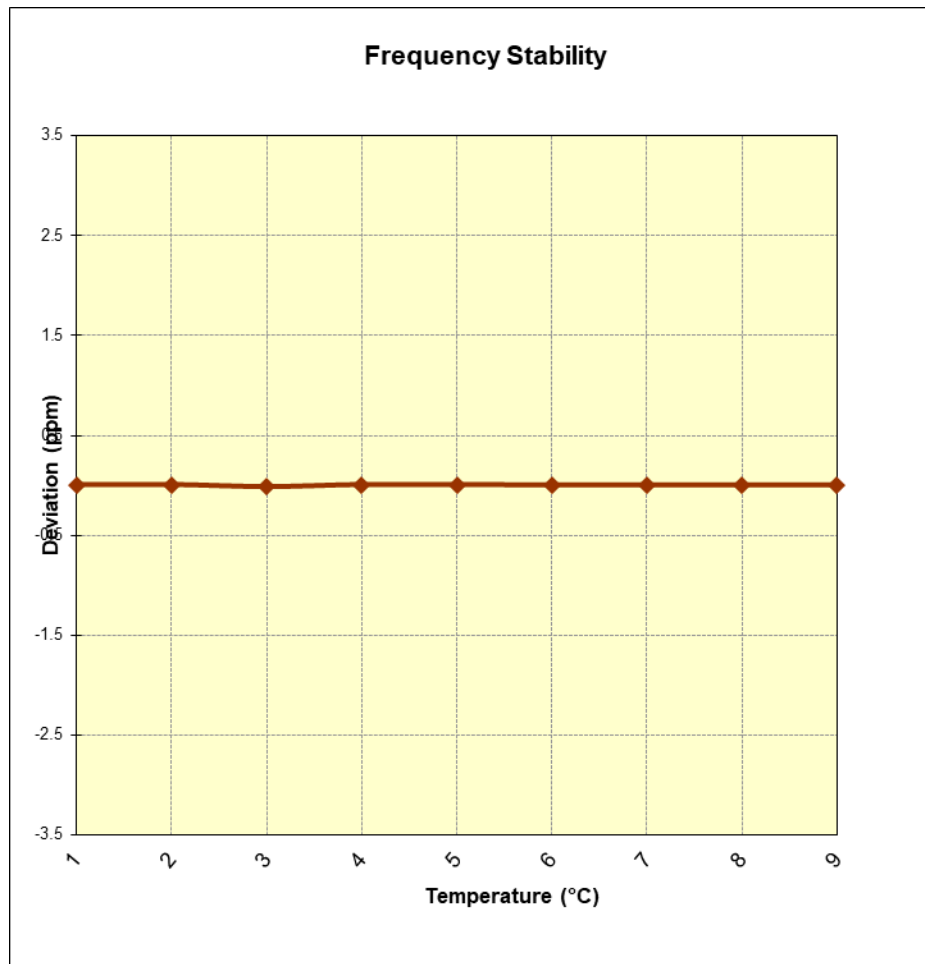
Figure 7-10. LTE Band 14 Frequency Stability Chart
