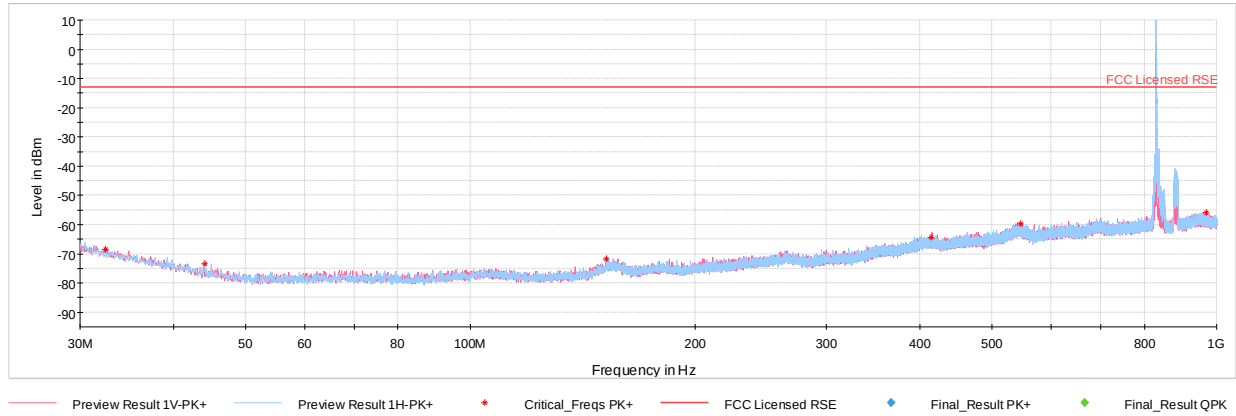
Plot 7-51. Radiated Spurious Plot Below 1GHz (Band 26)
