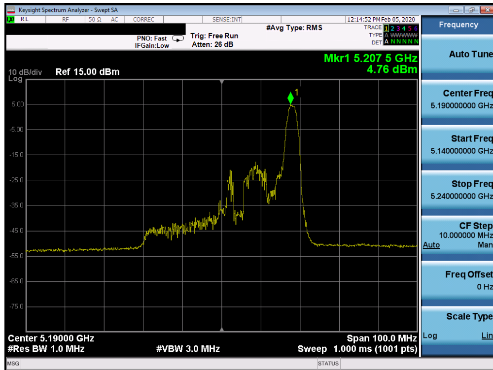
Plot 7-431. Power Spectral Density Plot ISSED SISO CORE 1 (40MHz BW 802.11ax Index 17 – RU26 (UNII Band 1) – Ch. 38)
