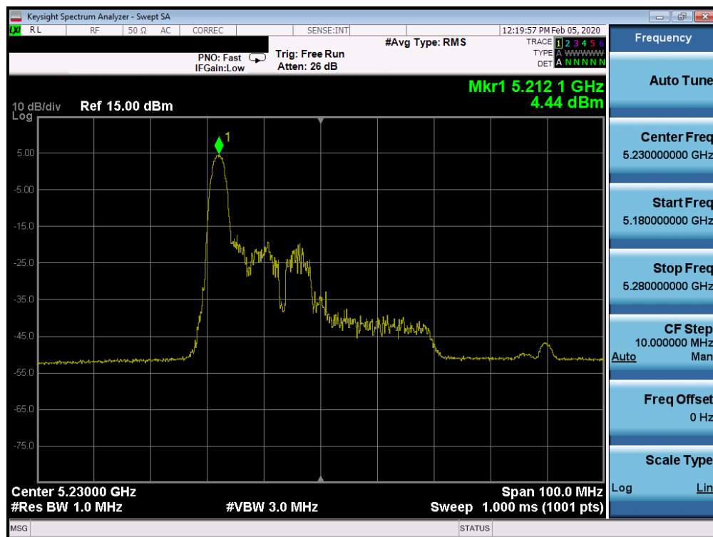
Plot 7-432. Power Spectral Density Plot ISSED SISO CORE 1 (40MHz BW 802.11ax Index 0 – RU26 (UNII Band 1) – Ch. 46)
