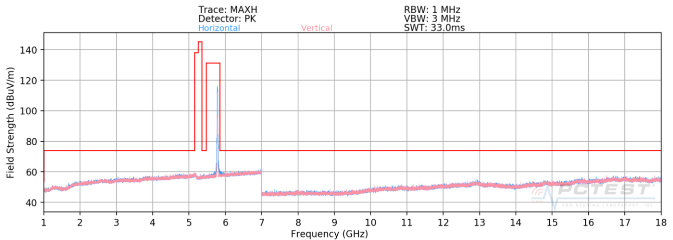
Plot 7-195. Radiated Spurious Plot above 1GHz SISO CORE1 (802.11n – U3 Ch. 157)
