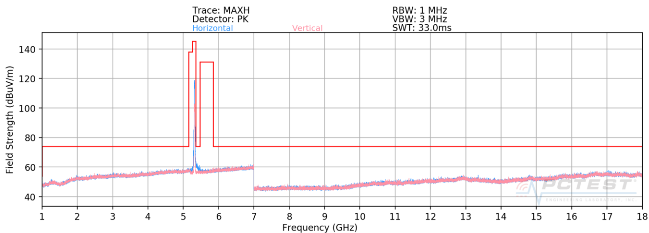
Plot 7-202. Radiated Spurious Plot above 1GHz CDD (802.11n – U2A Ch. 64)
