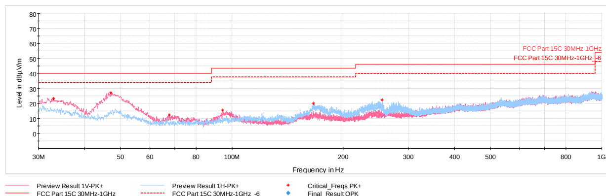
Plot 7-283. Radiated Spurious Plot below 1GHz CDD – Ch.36 with AC/DC Adapter
