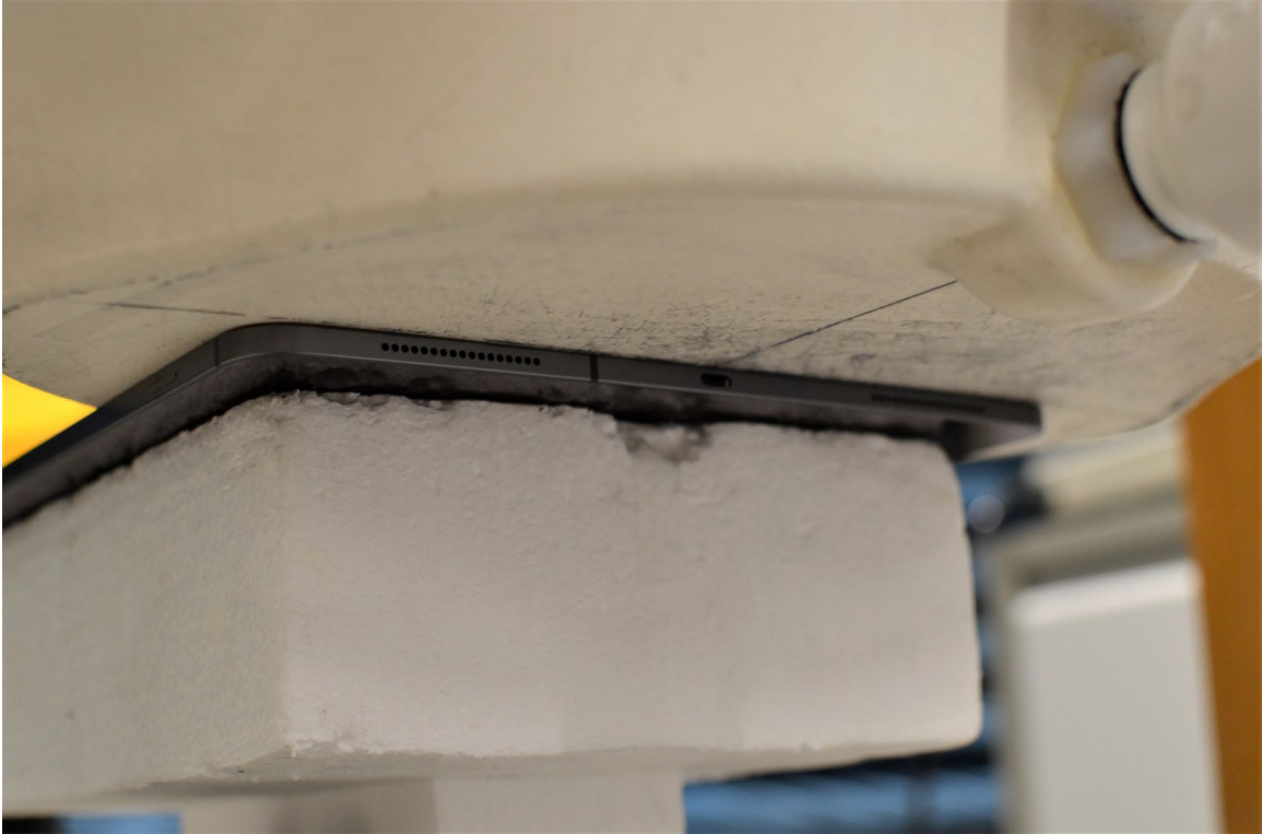
SAR Test Setup Photo 3: Back Side at 0.0 cm – Ant 1/2a/2b
