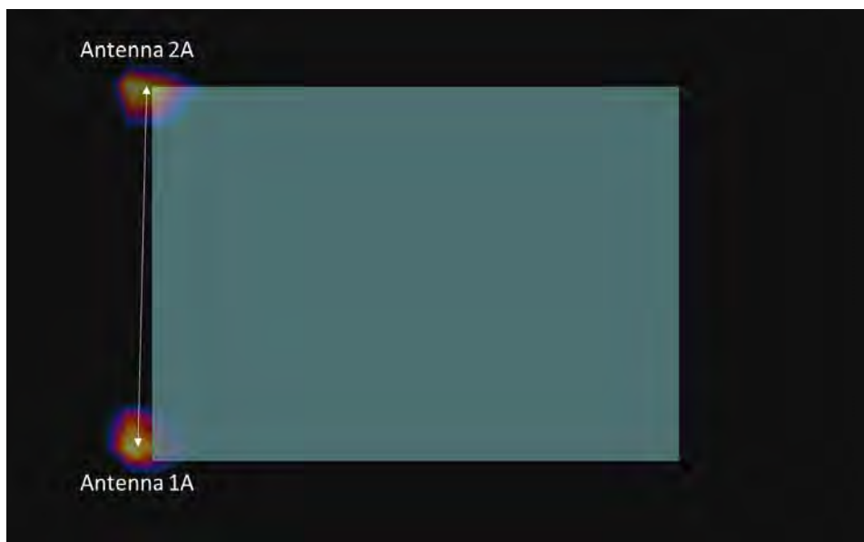
Figure 11-11 Back Side Spatial Separation for Antenna 1A and Antenna 2A
