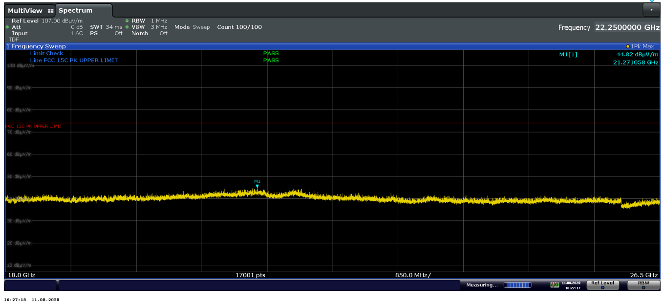
Plot 7-66. Radiated Spurious Emissions above 18GHz TxBF (GFSK ePA – Ch.0, Pol. H)
