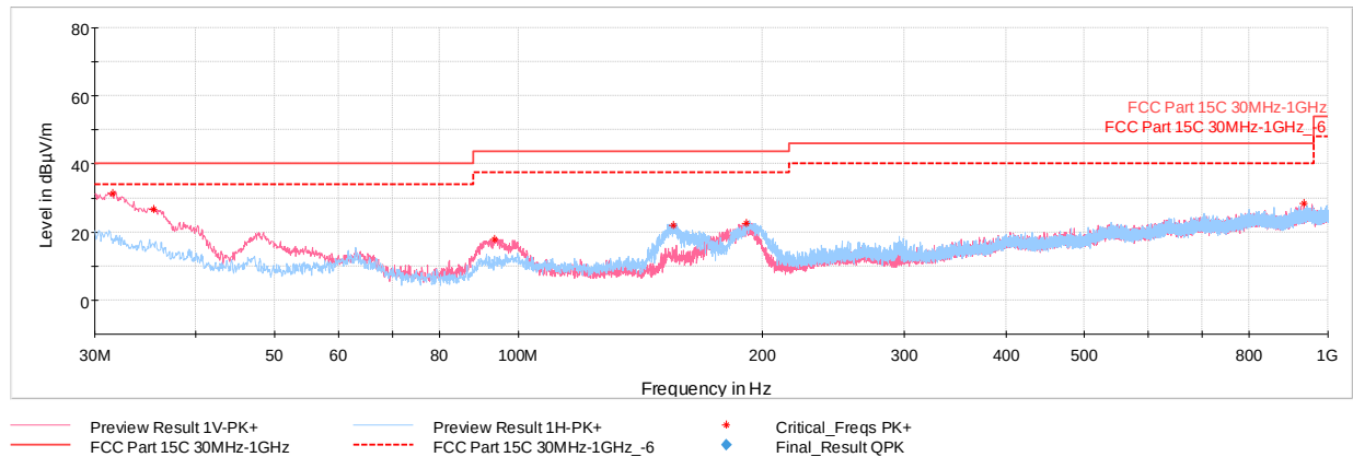
Plot 7-80. Radiated Spurious Emissions below 1GHz TxBF (GFSK ePA – Ch.0, with AC/DC Adapter)
