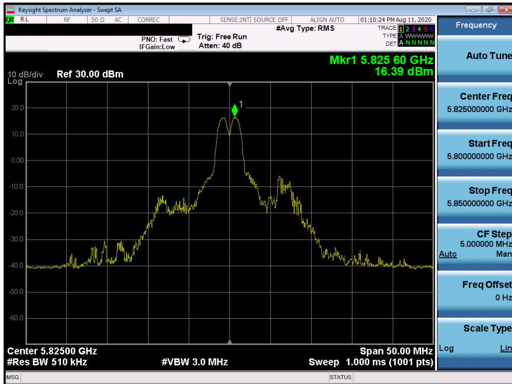
Plot 7-1142. Power Spectral Density Plot CDD Diversity Antenna 1b (20MHz BW 802.11ax Index 4 – RU26 (UNII Band 3) – Ch. 165)
