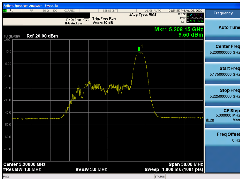
Plot 7-448. Power Spectral Density Plot Antenna 2a (20MHz BW 802.11ax Index 8– RU26 (UNII Band 1) – Ch. 40)
