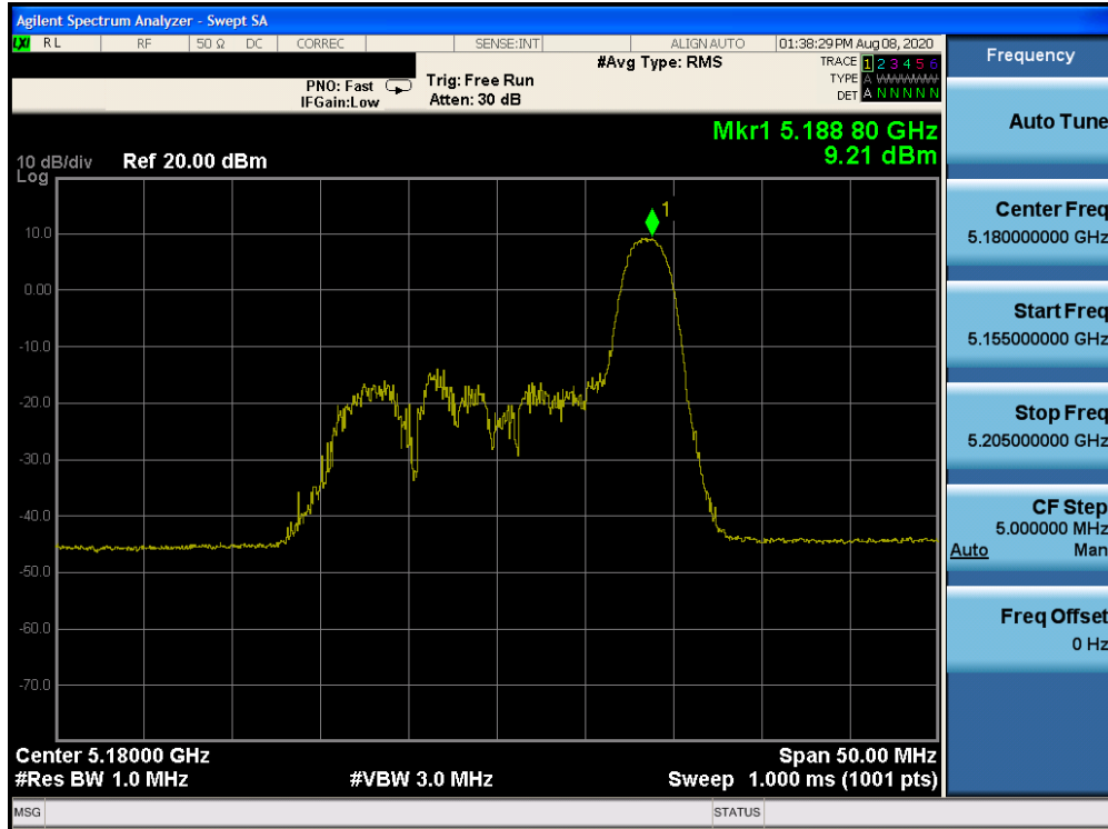
Plot 7-445. Power Spectral Density Plot Antenna 2a (20MHz BW 802.11ax Index 8 – RU26 (UNII Band 1) – Ch. 36)
