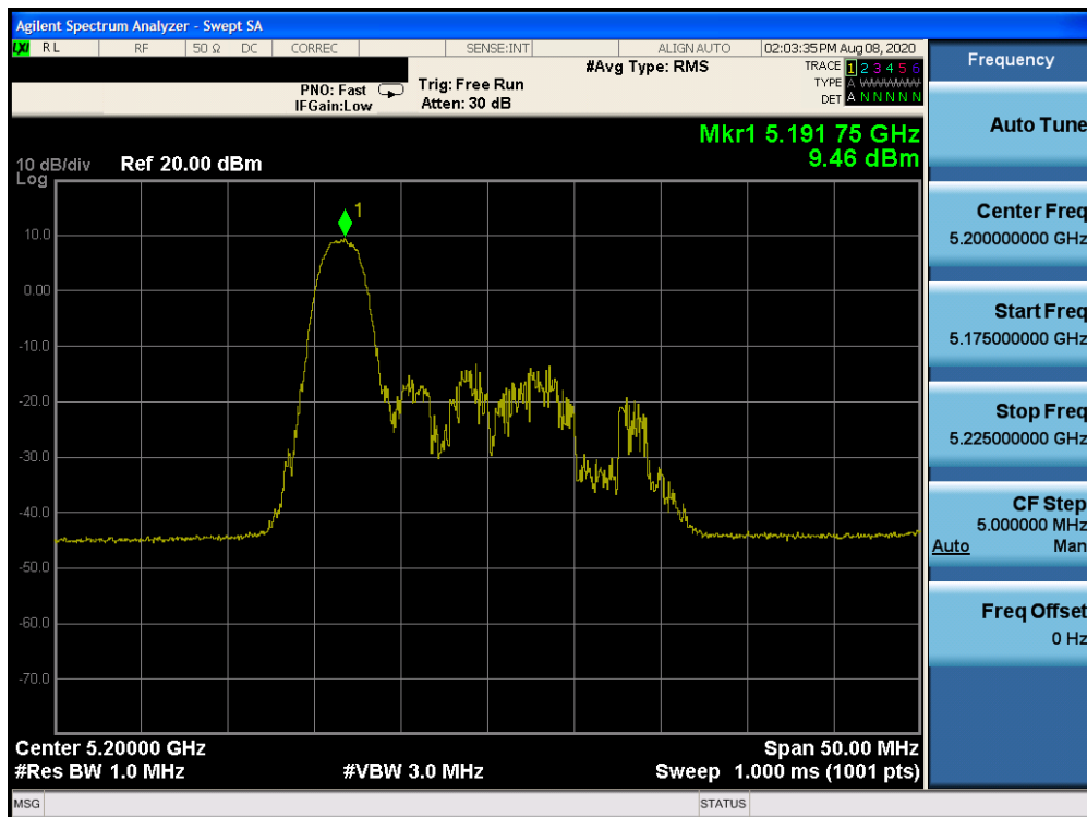
Plot 7-446. Power Spectral Density Plot Antenna 2a (20MHz BW 802.11ax Index 0 – RU26 (UNII Band 1) – Ch. 40)
