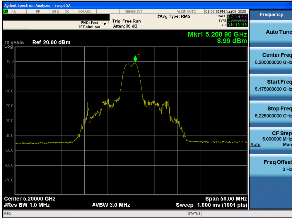
Plot 7-447. Power Spectral Density Plot Antenna 2a (20MHz BW 802.11ax Index 4 – RU26 (UNII Band 1) – Ch. 40)
