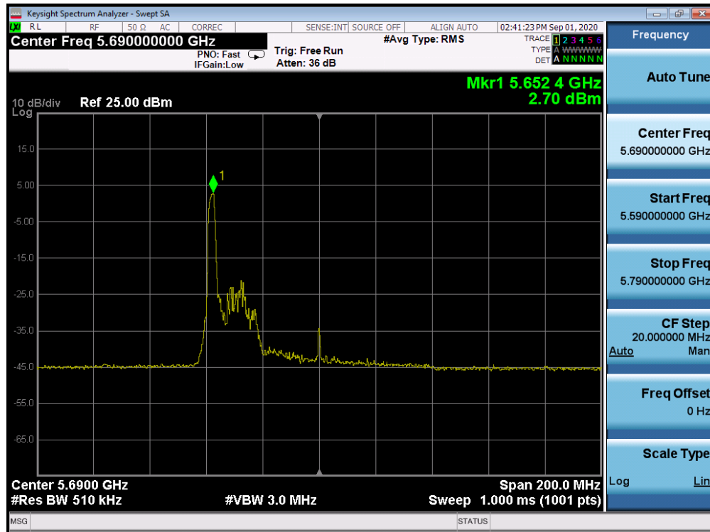
Plot 7-519. Power Spectral Density Plot Antenna 2a (80MHz BW 802.11ax Index 0 – RU26 (UNII Band 2C) – Ch. 138)
