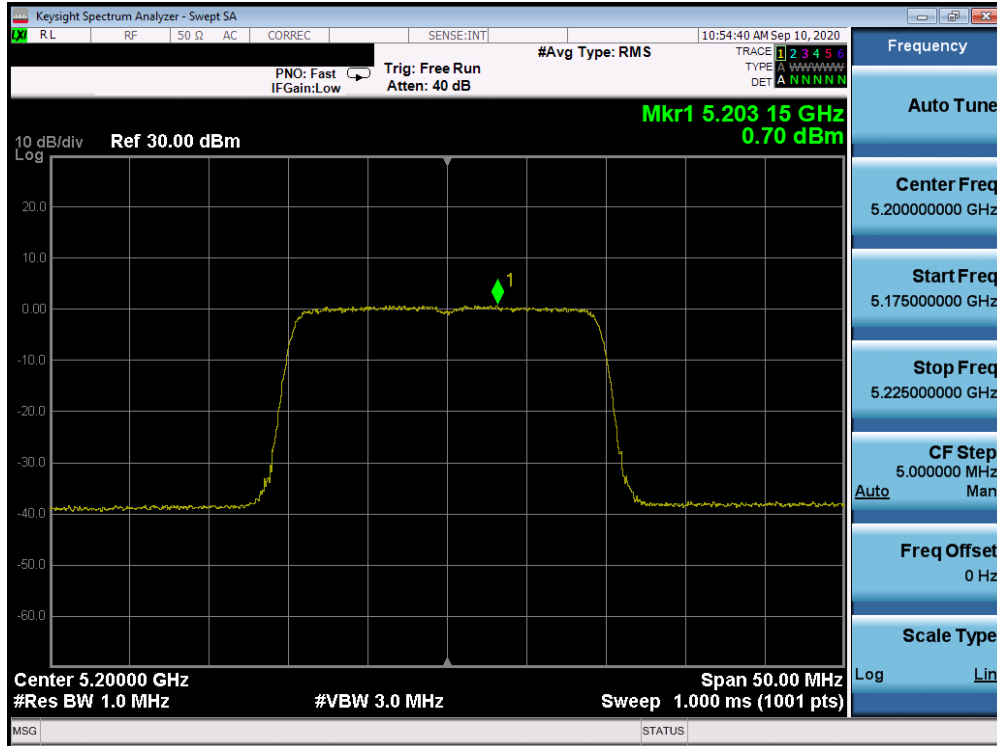
Plot 7-559. ISD Power Spectral Density Plot Antenna 2a (20MHz BW 802.11ax- RU242 (UNII Band 1) – Ch. 40)
