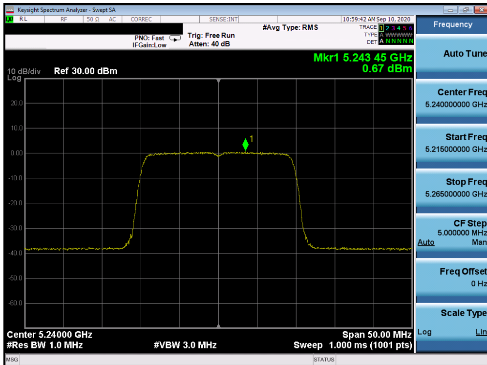
Plot 7-560. ISD Power Spectral Density Plot Antenna 2a (20MHz BW 802.11ax- RU242 (UNII Band 1) – Ch. 48)
