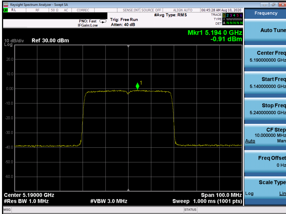
Plot 7-697. ISD Power Spectral Density Plot Antenna 1b (40MHz BW 802.11ax – RU484 (UNII Band 1) – Ch. 38)
