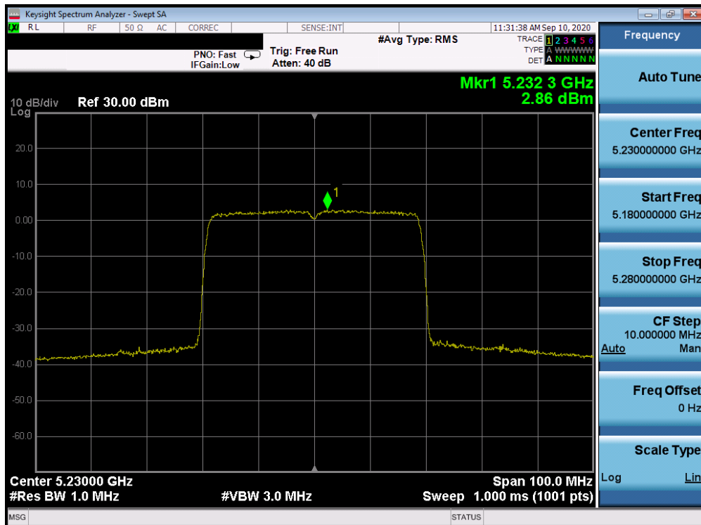
Plot 7-698. ISD Power Spectral Density Plot Antenna 1b (40MHz BW 802.11ax – RU484 (UNII Band 1) – Ch. 46)
