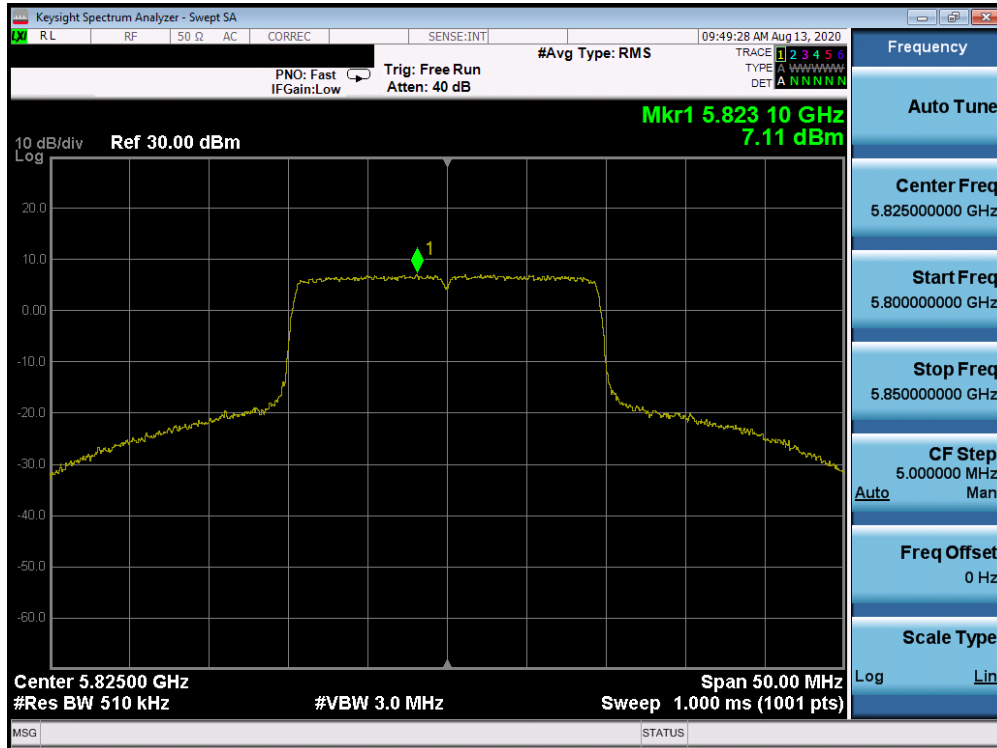
Plot 7-899. Power Spectral Density Plot CDD Primary Antenna 2b (20MHz BW 802.11ax- RU242 (UNII Band 3) – Ch. 165)
