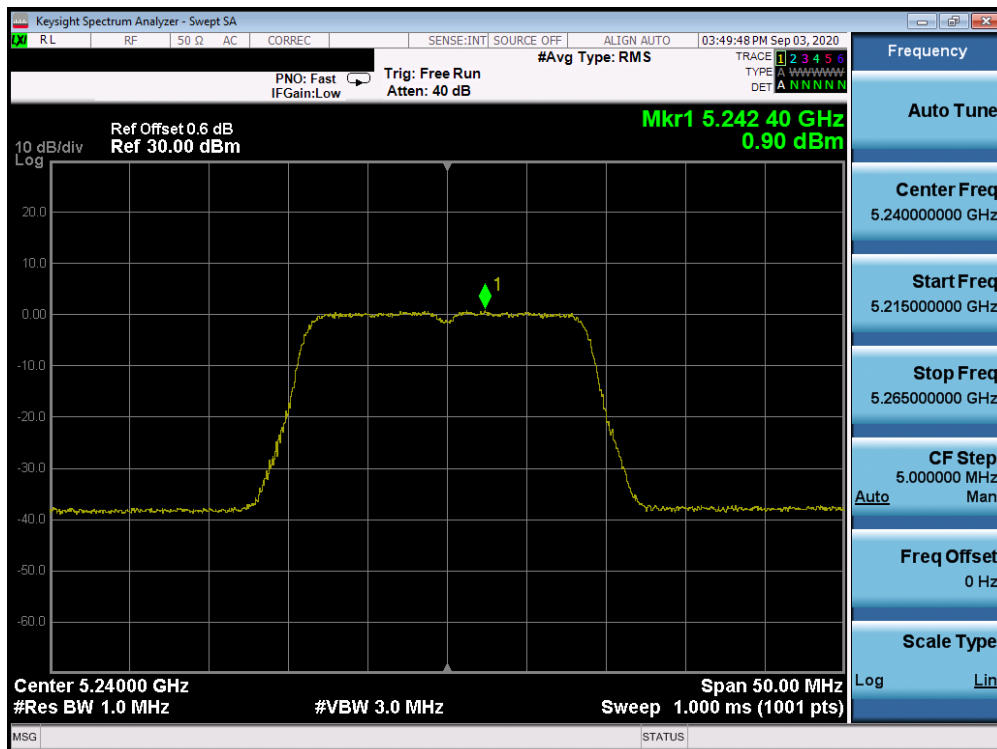
Plot 7-252. ISED Power Spectral Density Plot SDM Diversity Antenna 1b (20MHz BW 802.11n (UNII Band 1) – Ch. 48)
