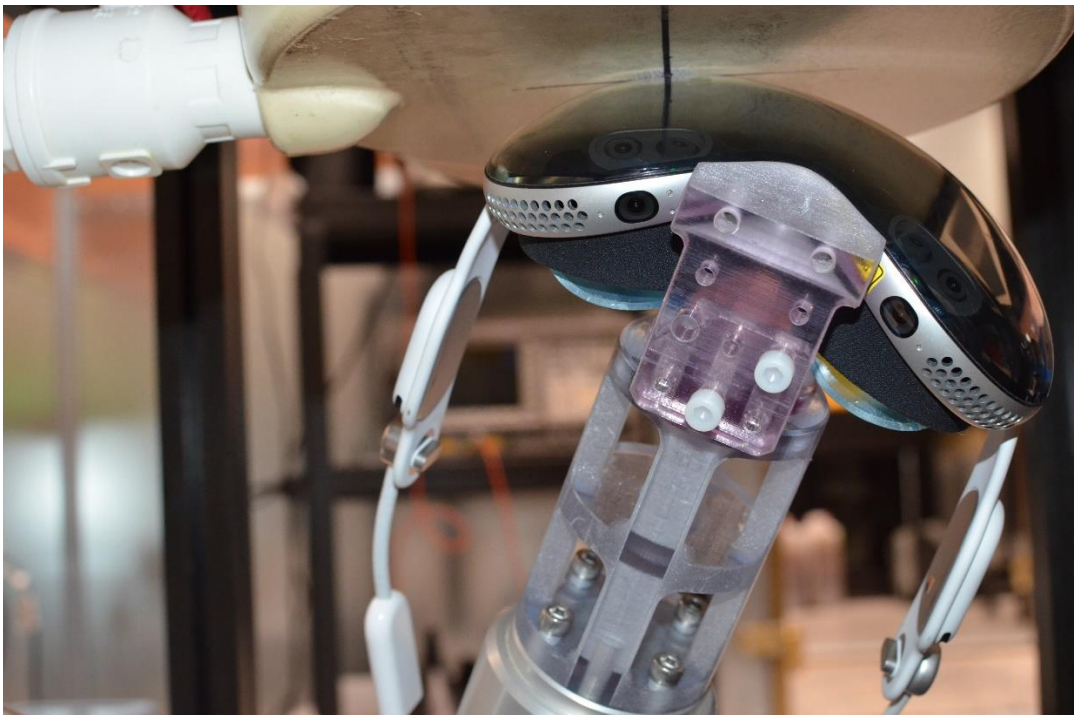
SAR Test Setup Photo 18: Antenna 1 Point 34 Extremity SAR at 0.0 cm
