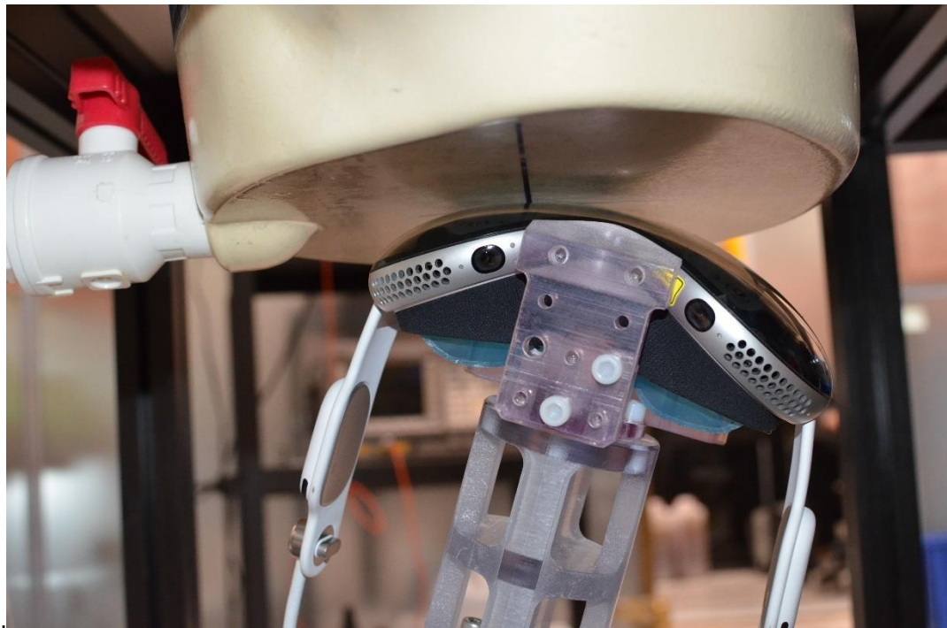
SAR Test Setup Photo 20: Antenna 1 Point 39 Extremity SAR at 0.0 cm
