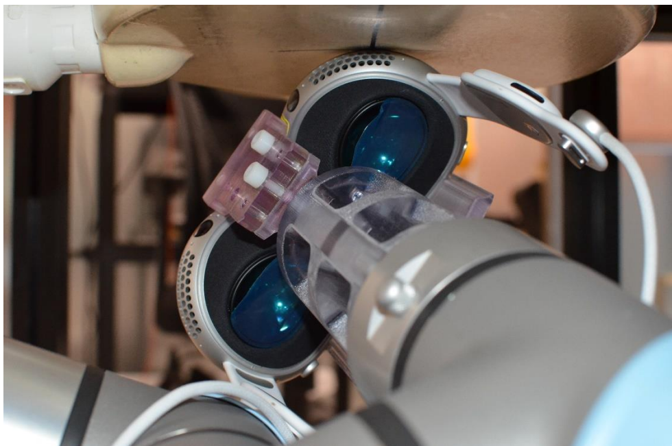
SAR Test Setup Photo 11: Antenna NB UNII_L Point 10 Extremity SAR at 0.0 cm
