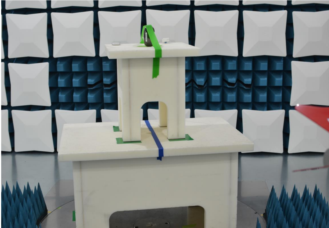
Figure 7: Above 1GHz Test Setup (Front View)
