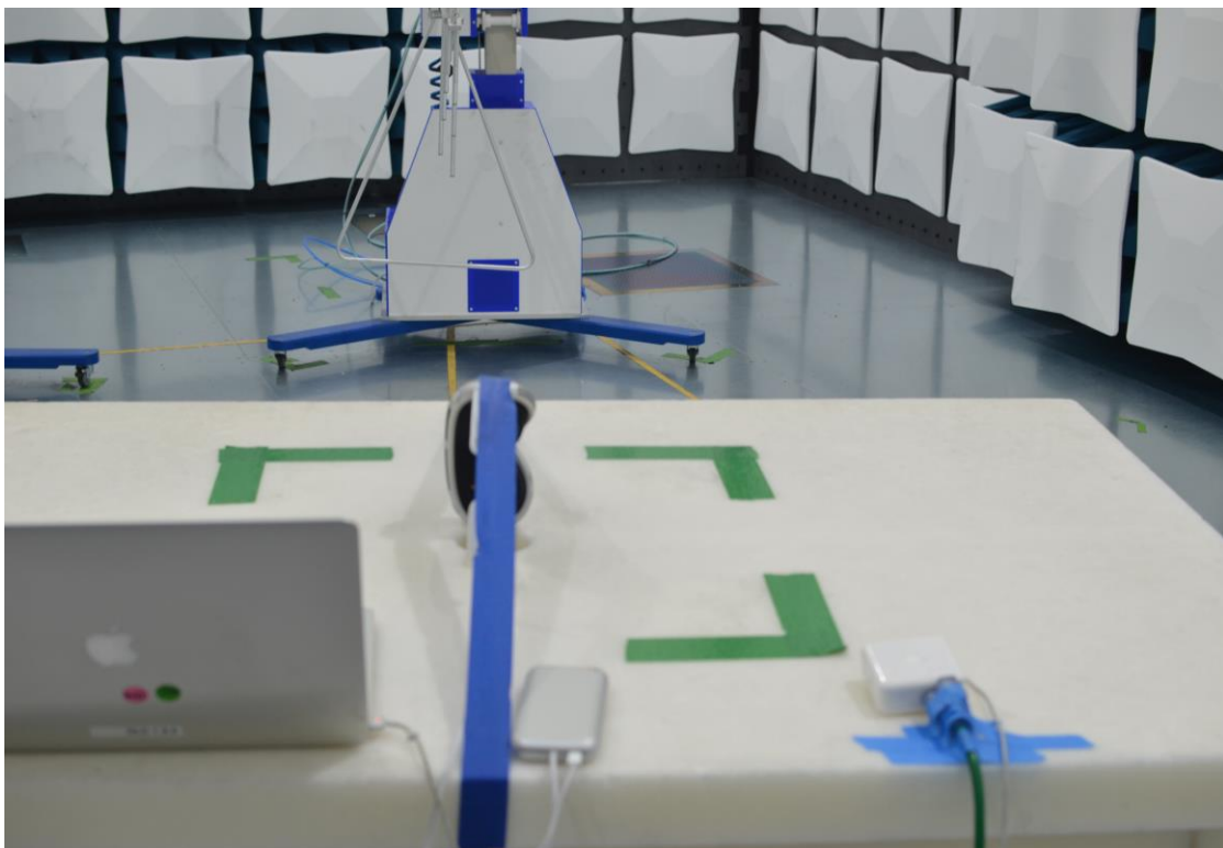
Figure 16: 30MHz-1GHz Test Setup (Rear View)
