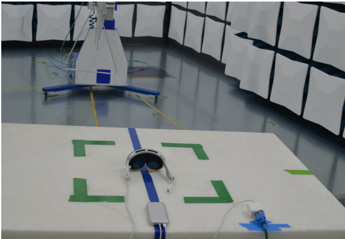
Figure 10: 30MHz-1GHz Test Setup (Rear View)
