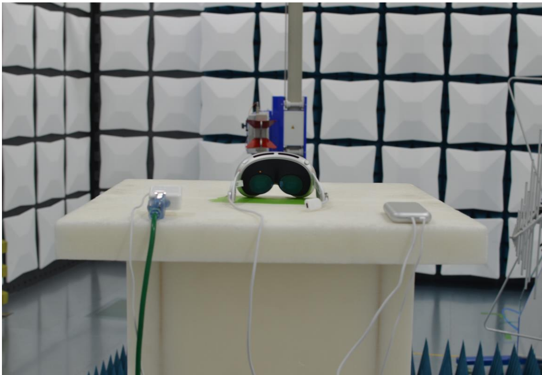
Figure 6: Above 1GHz Test Setup (Rear View)
