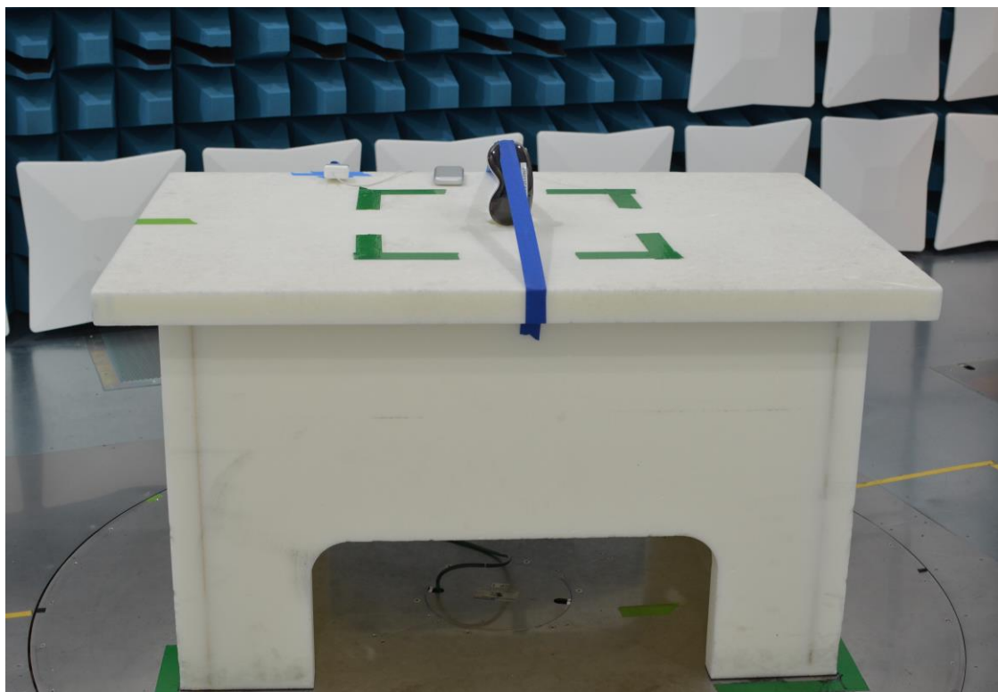
Figure 11: 30MHz-1GHz Test Setup (Front View)
