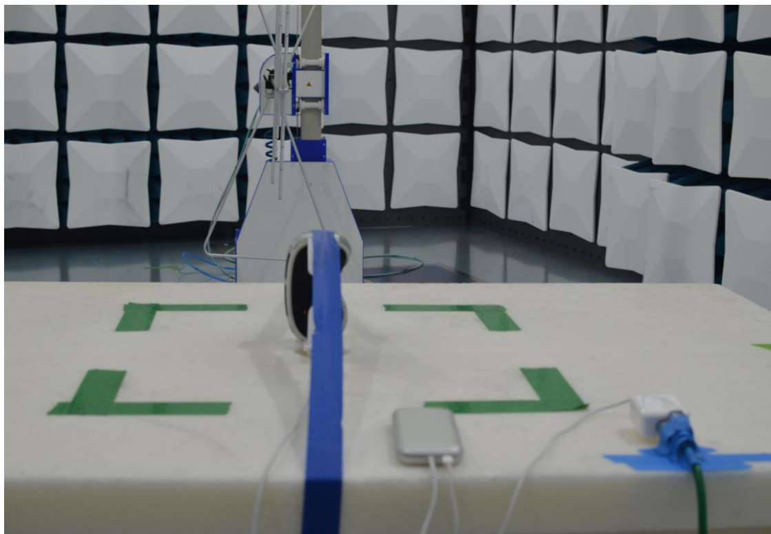
Figure 12: 30MHz-1GHz Test Setup (Rear View)
