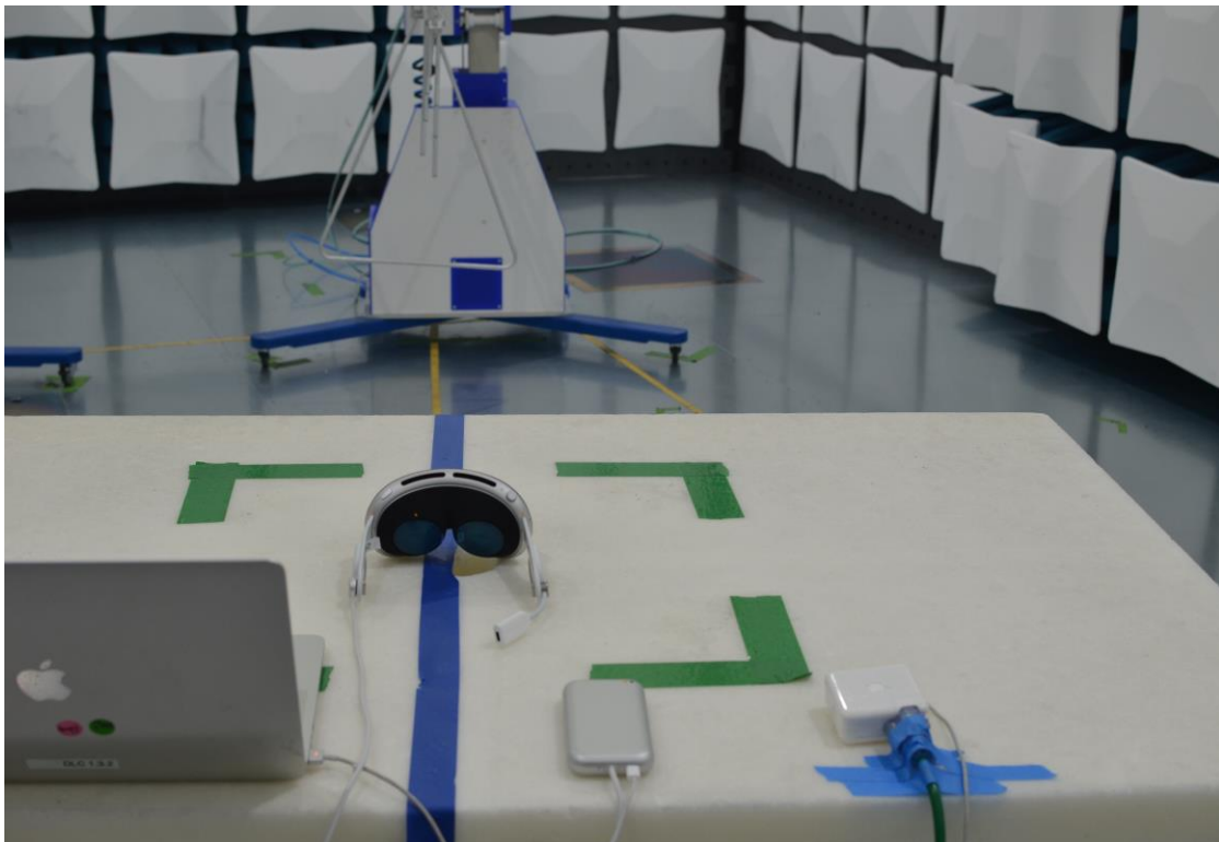
Figure 14: 30MHz-1GHz Test Setup (Rear View)
