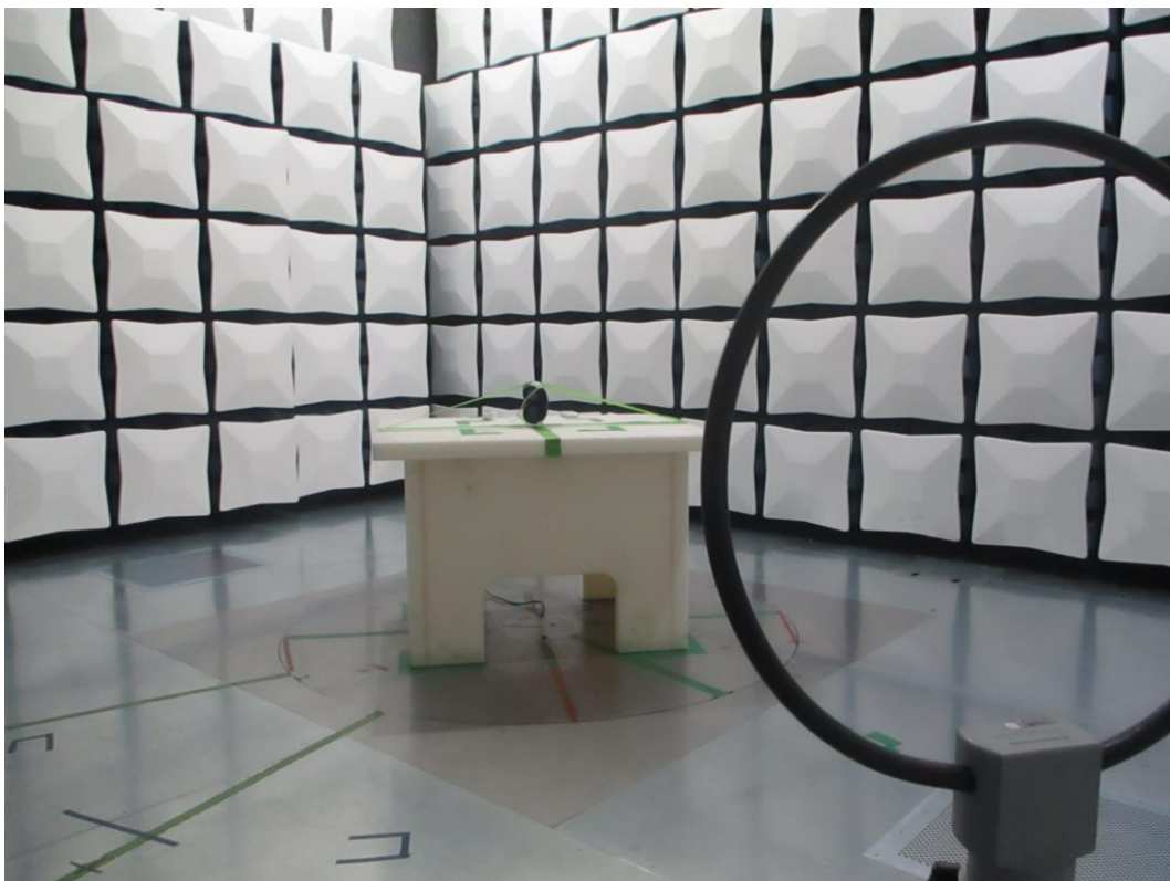
Figure 18: 9kHz-30MHz Test Setup (Front View)
