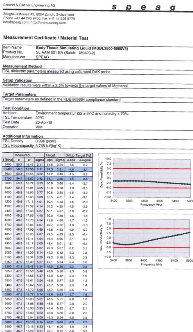
Figure D-4 5 GHz Body Tissue Equivalent Matter
