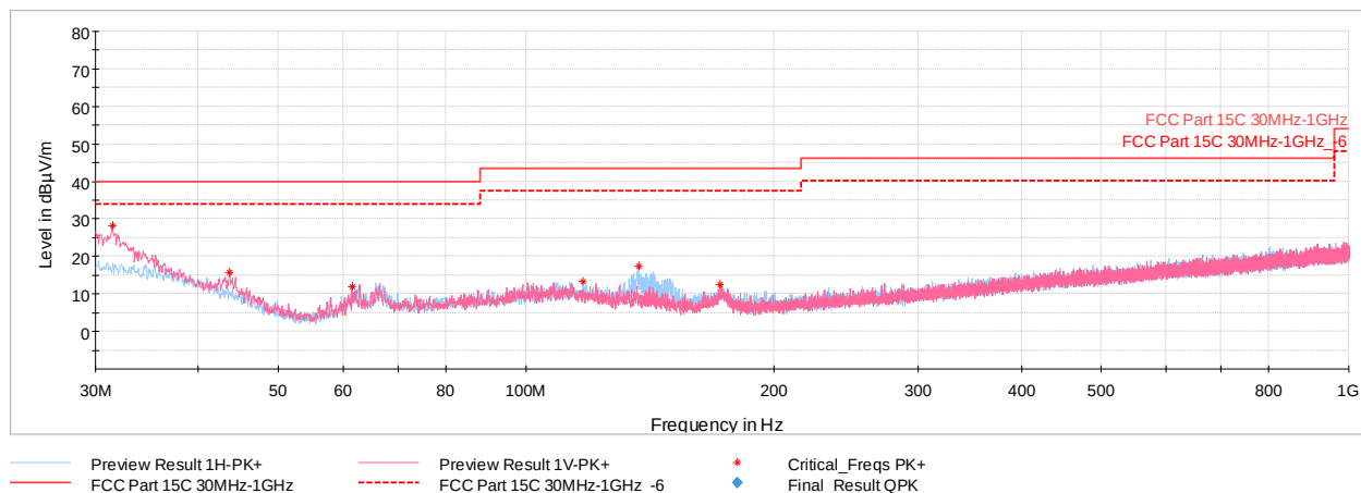
Plot 7-73. Radiated Spurious Plot below 1GHz (4Mbps, HDR4 ePA – Ch.38, Pol. H & V, with Charger)
