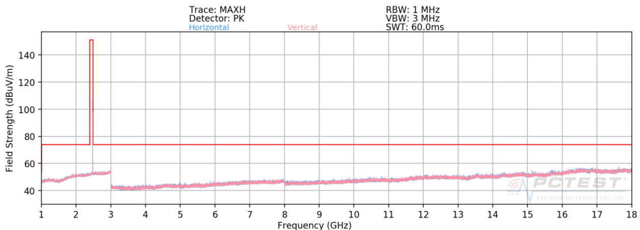
Plot 7-62. Radiated Spurious Plot Above 1GHz Ant-1 (4Mbps, HDR4, ePA – Ch. 75, Ant. Pol. H & V)
