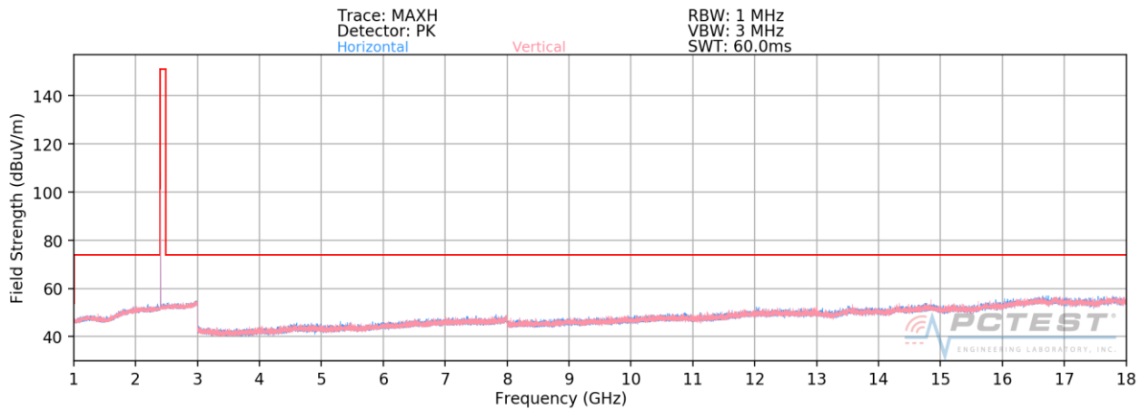
Plot 7-57. Radiated Spurious Plot Above 1GHz Ant-0 (4Mbps, HDR4, ePA – Ch. 1, Ant. Pol. H & V)
