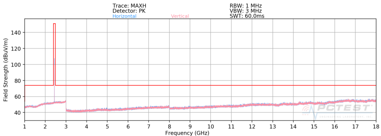
Plot 7-61. Radiated Spurious Plot Above 1GHz Ant-1 (4Mbps, HDR4, ePA – Ch. 38, Ant. Pol. H & V)
