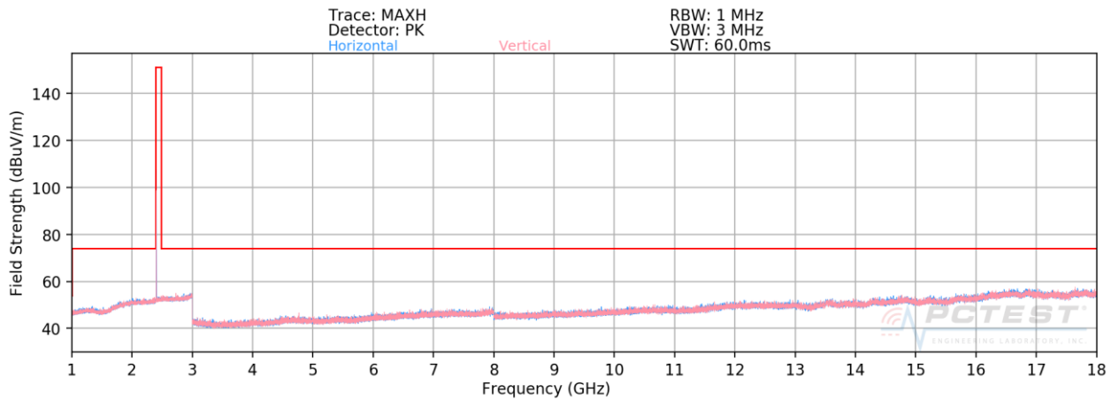
Plot 7-60. Radiated Spurious Plot Above 1GHz Ant-1 (4Mbps, HDR4, ePA – Ch. 1, Ant. Pol. H & V)
