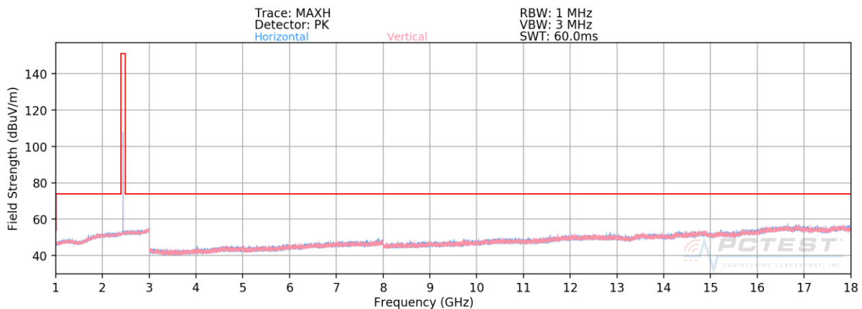
Plot 7-58. Radiated Spurious Plot Above 1GHz Ant-0 (4Mbps, HDR4, ePA – Ch. 38, Ant. Pol. H & V)
