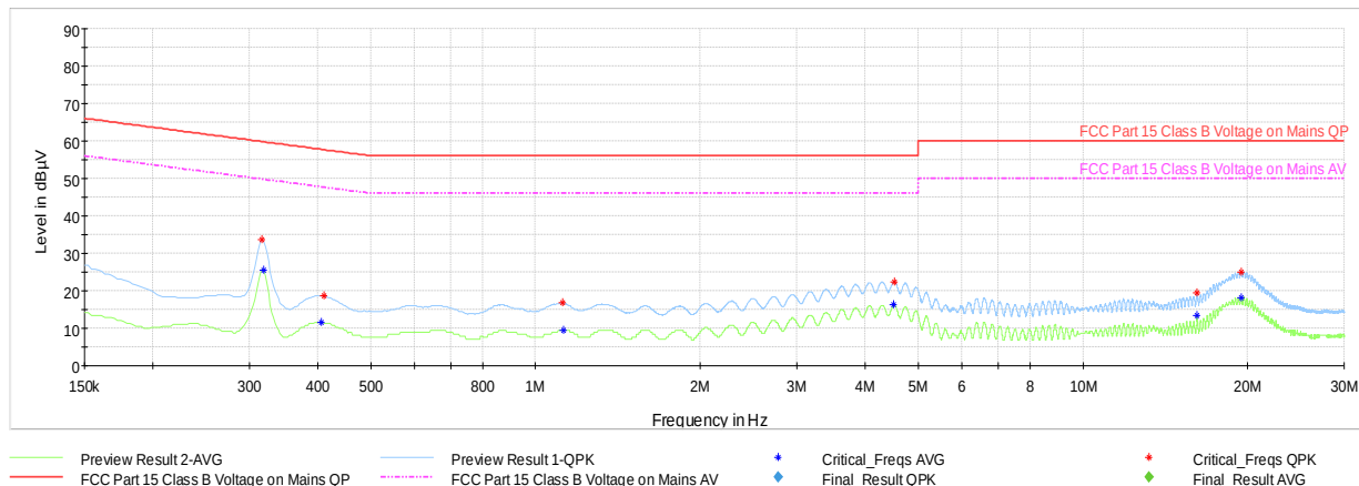
Plot 7-75. AC Line Conducted Plot with Bluetooth LE – 1Mbps ePA Ch.19 (N, with Laptop)
