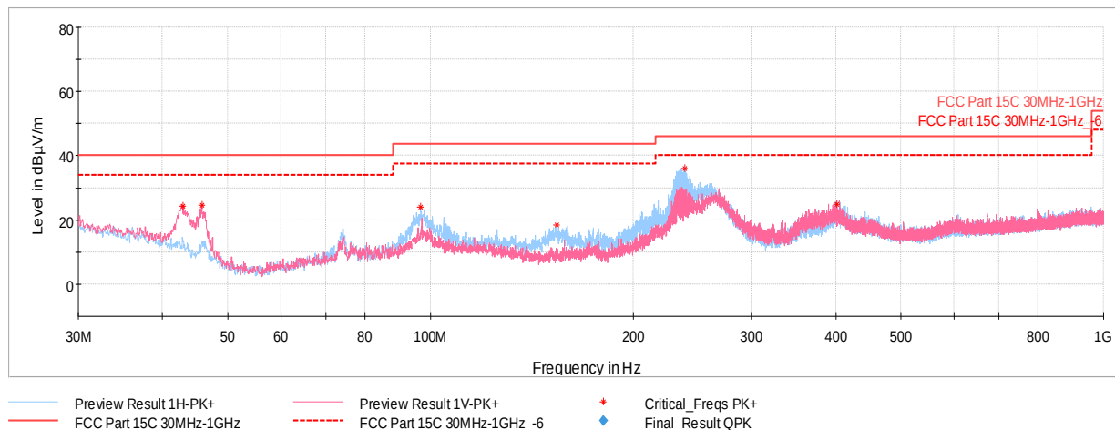
Plot 7-73. Radiated Spurious Plot below 1GHz (1Mbps, ePA – Ch.19, Pol. H & V, with Laptop)
