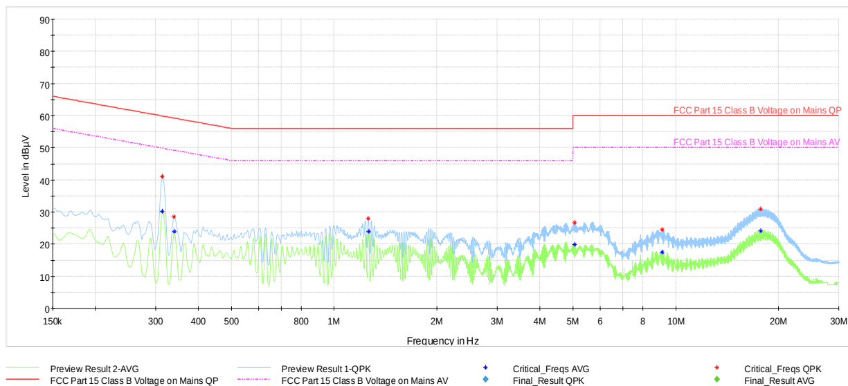
Plot 7-74. AC Line Conducted Plot with Bluetooth LE – 1Mbps ePA Ch.19 (L1, with Laptop)
