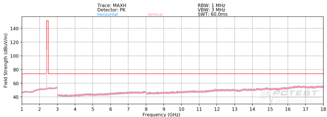
Plot 7-72. Radiated Spurious Plot above 1GHz ANT 1 (BT GFSK ePA – Ch. 0)
